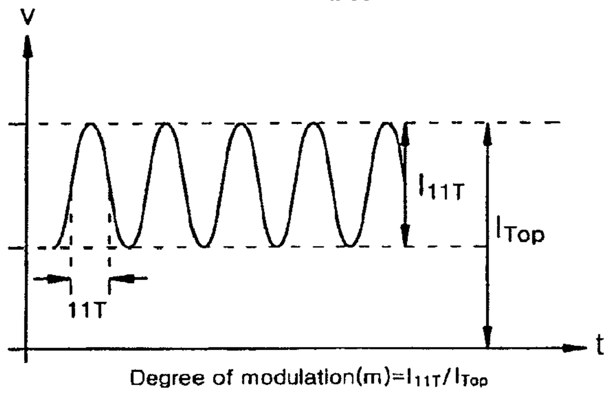
Fig. 5 PRIOR ART
