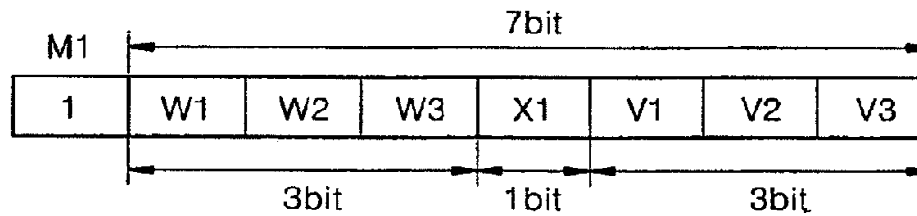
Fig. 2 PRIOR ART
