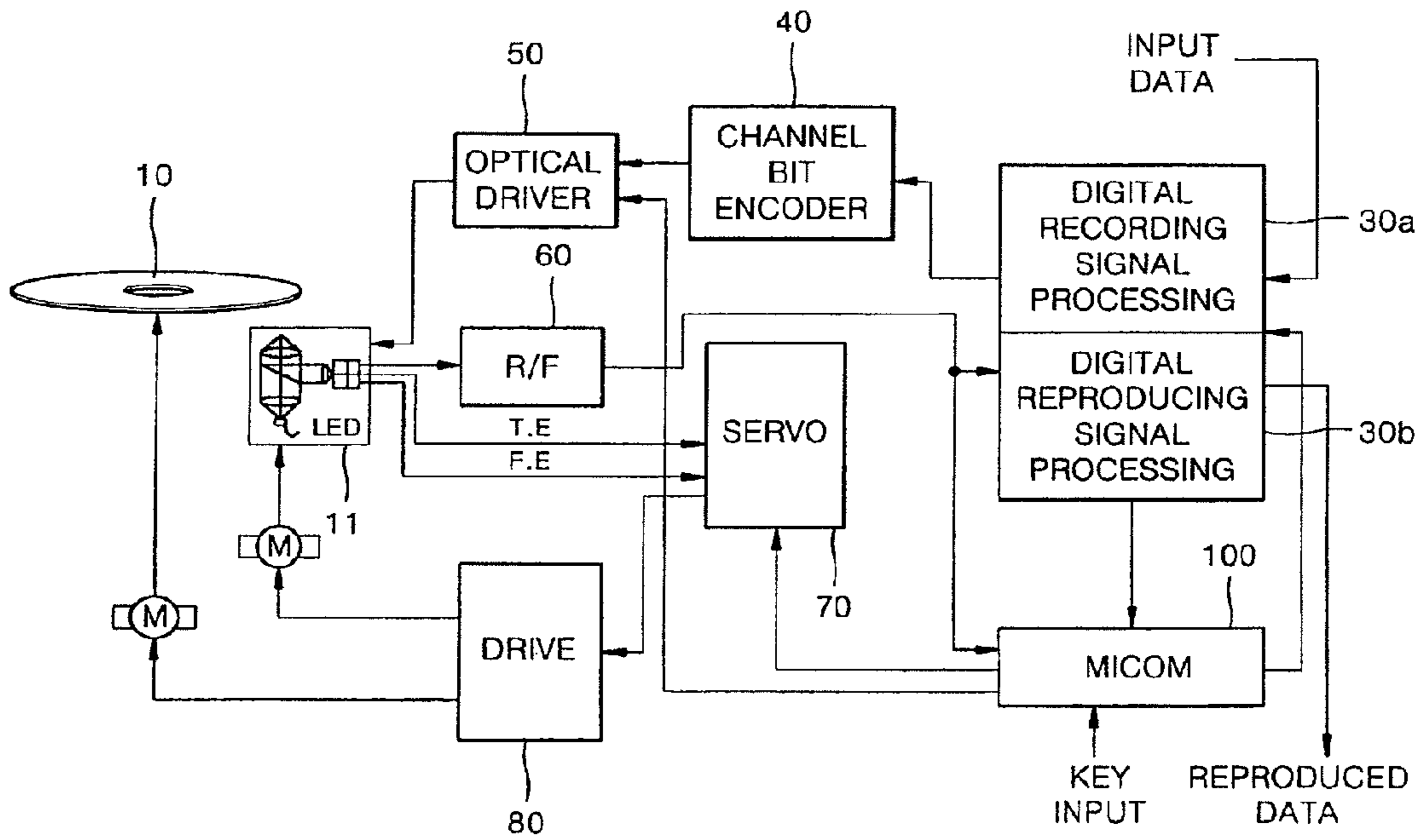
Fig. 1 PRIOR ART
