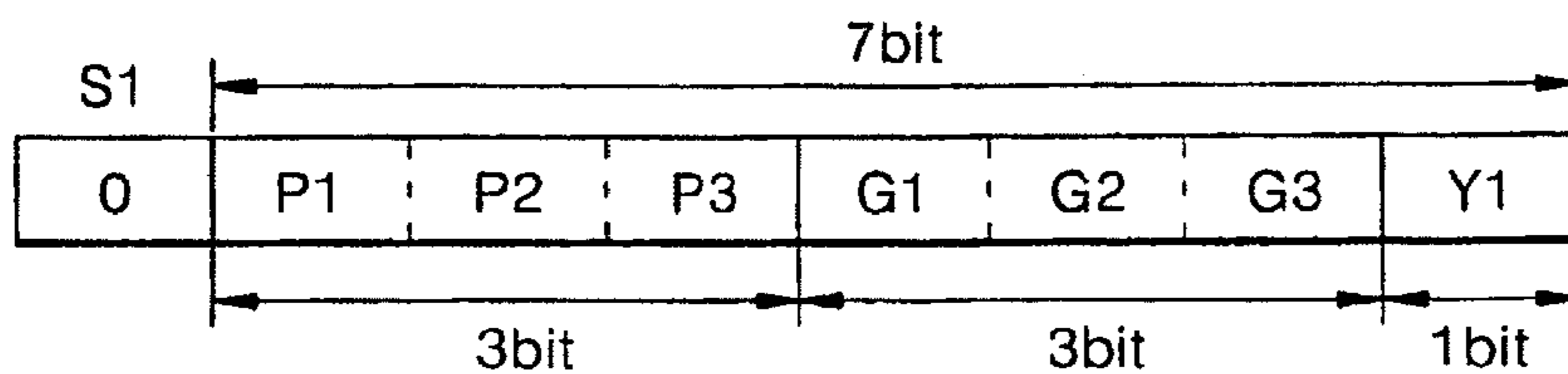
Fig. 7 PRIOR ART
