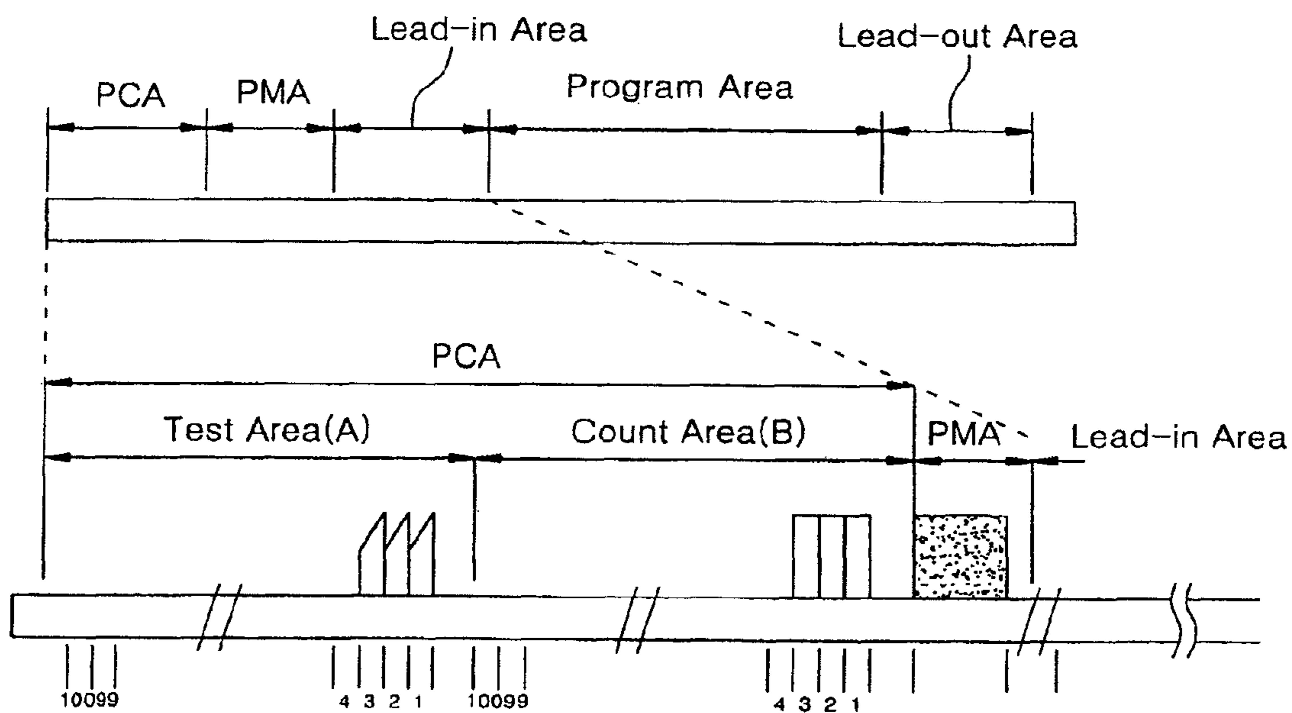
Fig. 4 PRIOR ART
