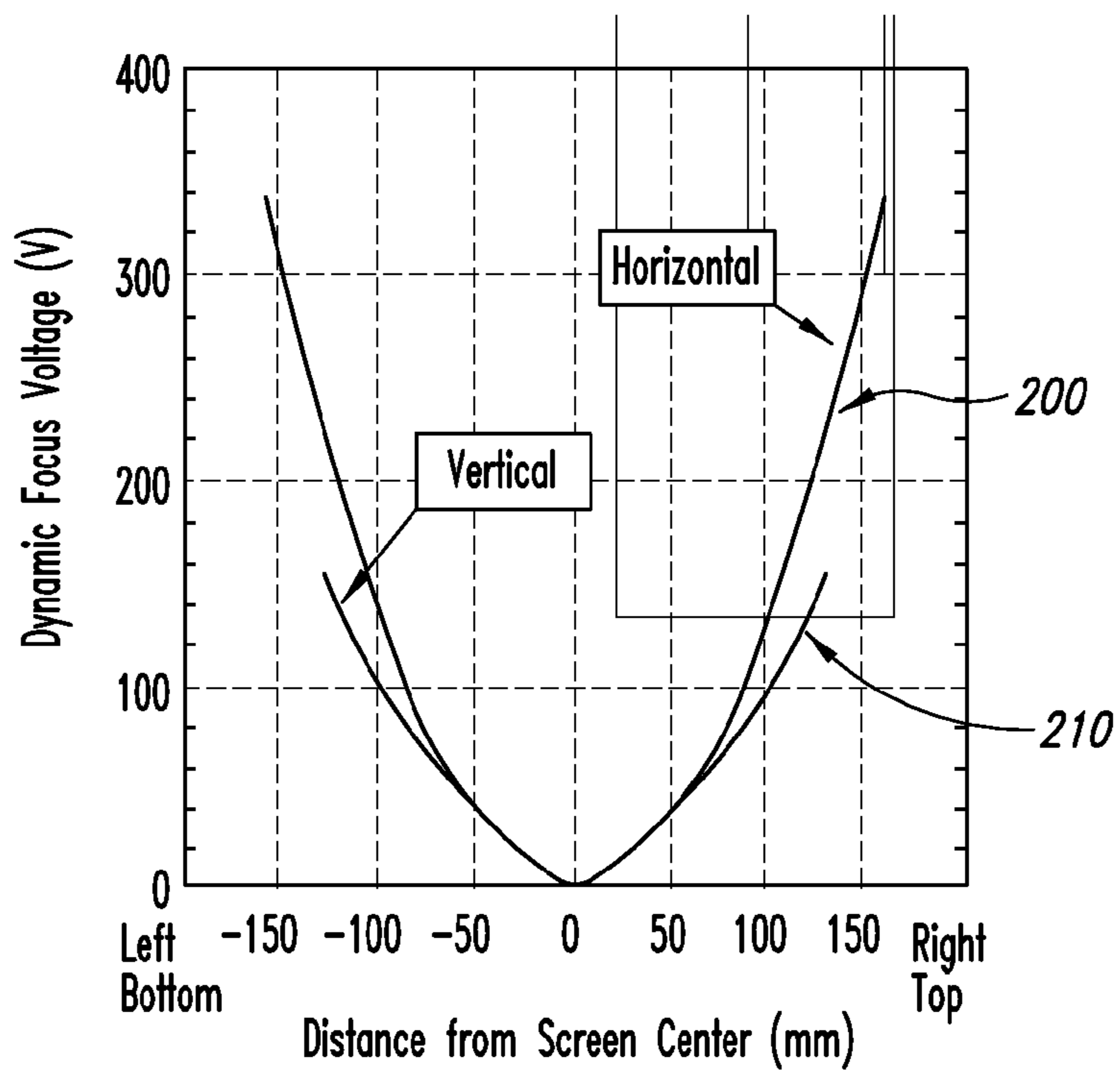
FIG. 3 (Prior Art)
