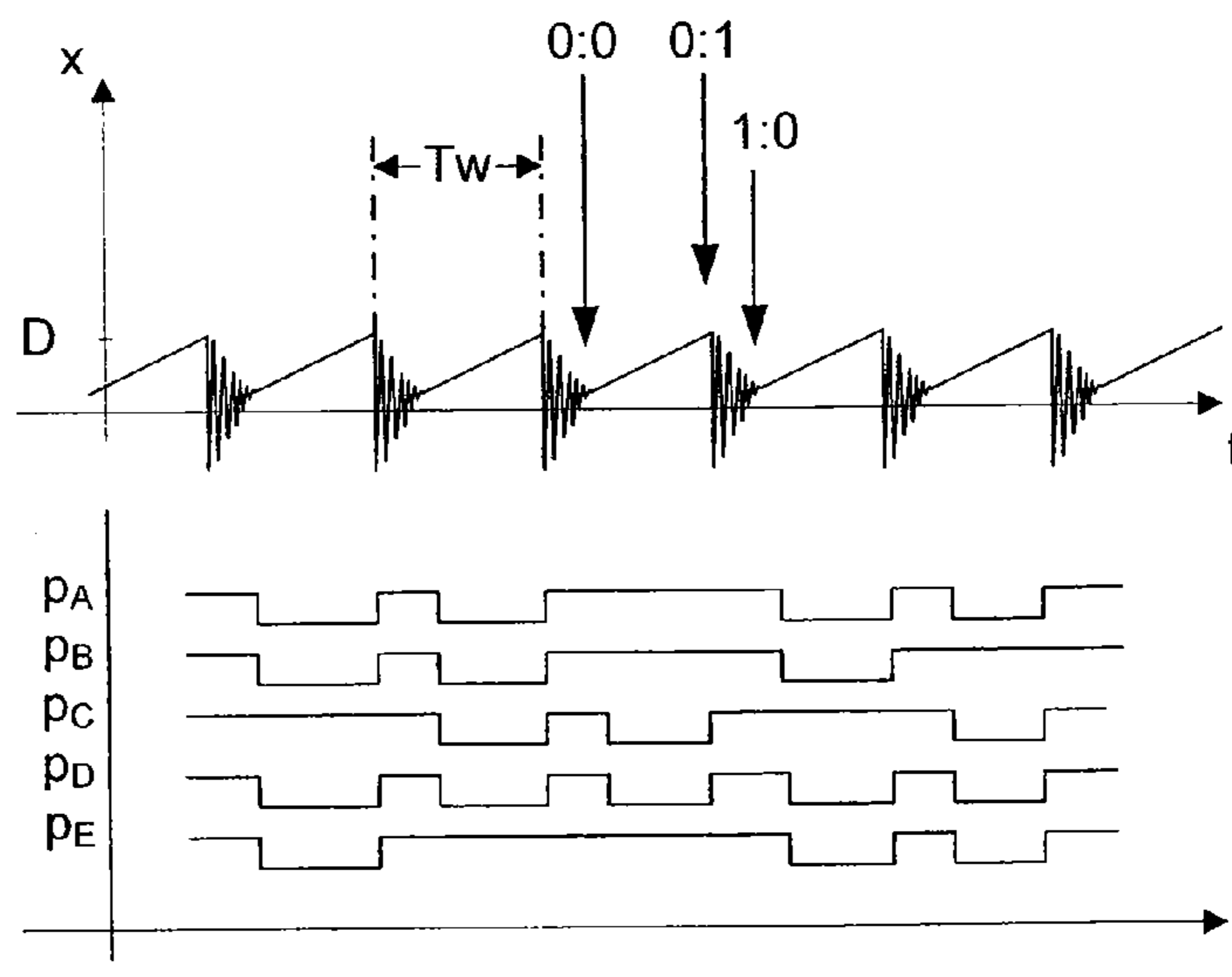
Fig. 20 (prior art)
