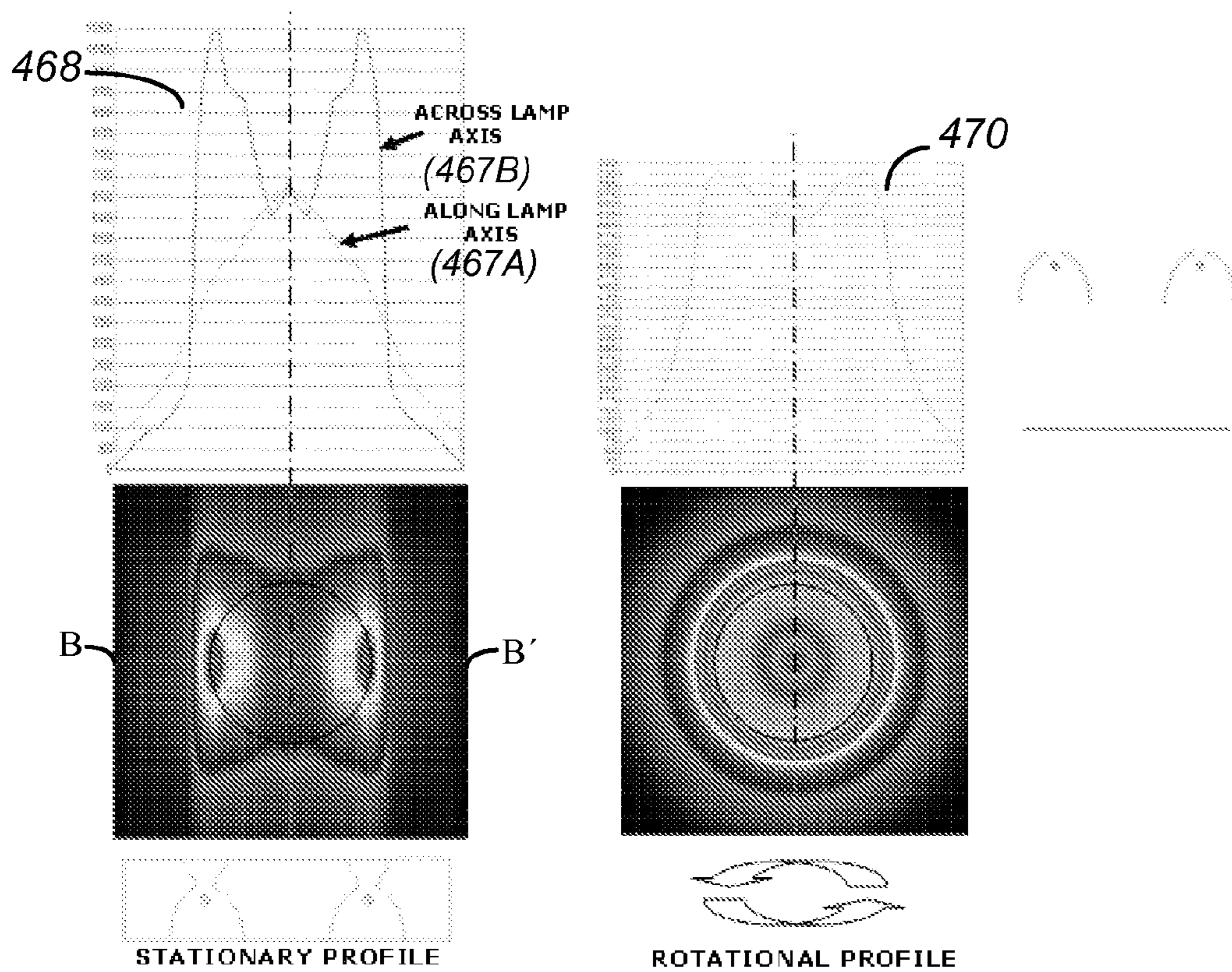
Primary Reflector (asymmetric) - dual lamp
