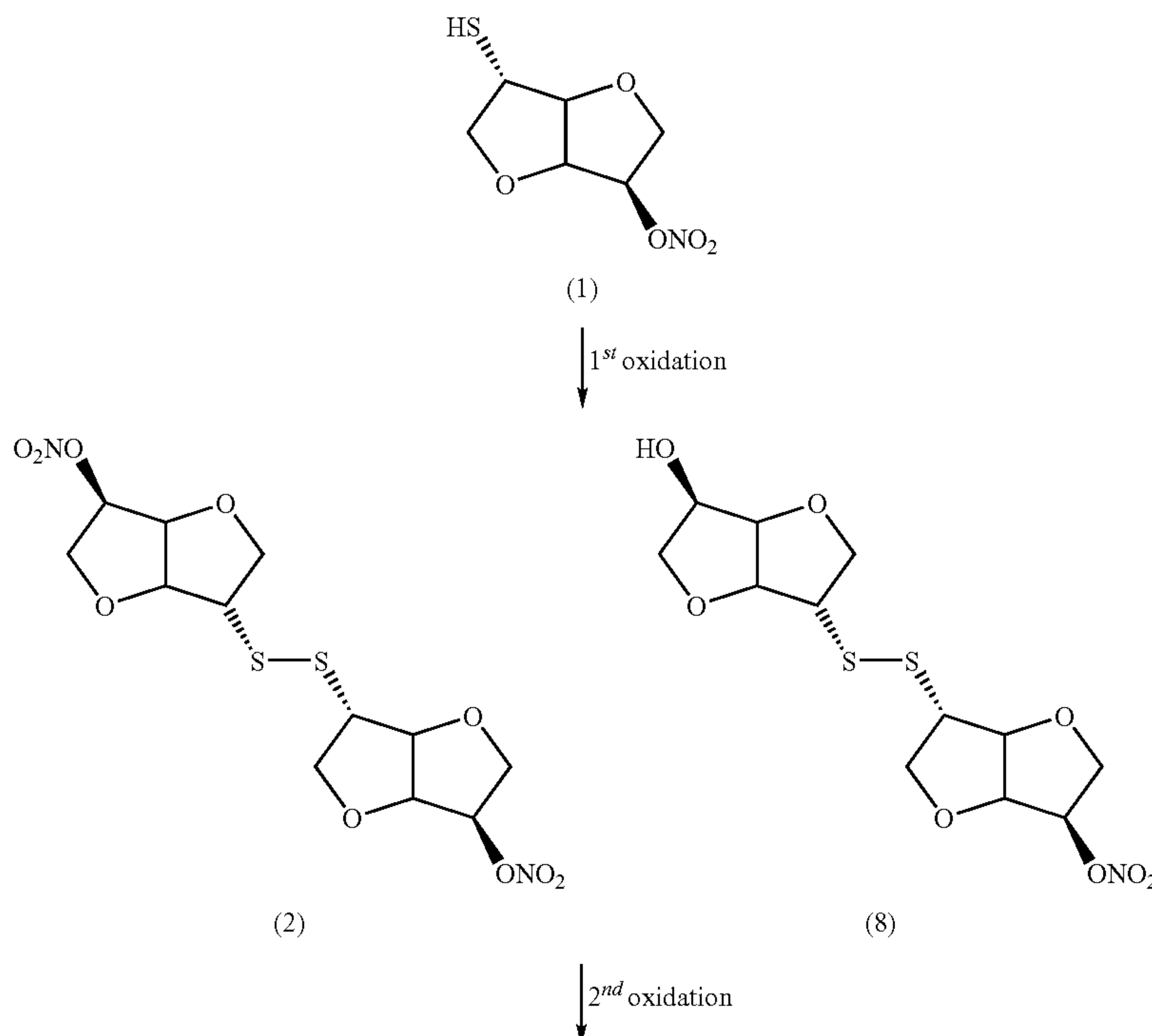
Scheme 1:
