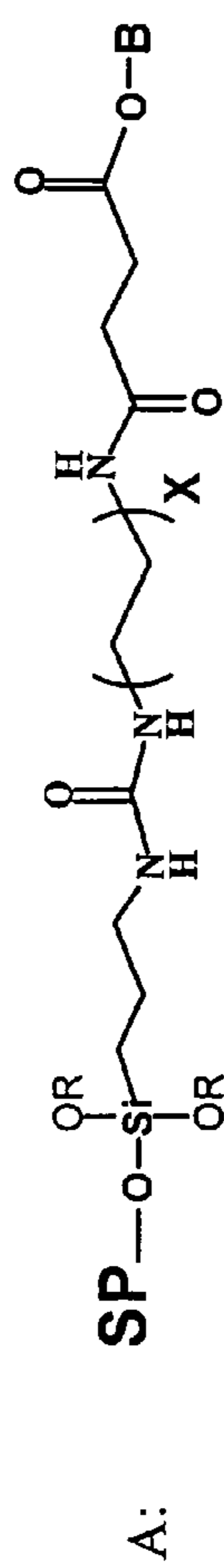
Figure 8. General Chemical formulae for Spacers
