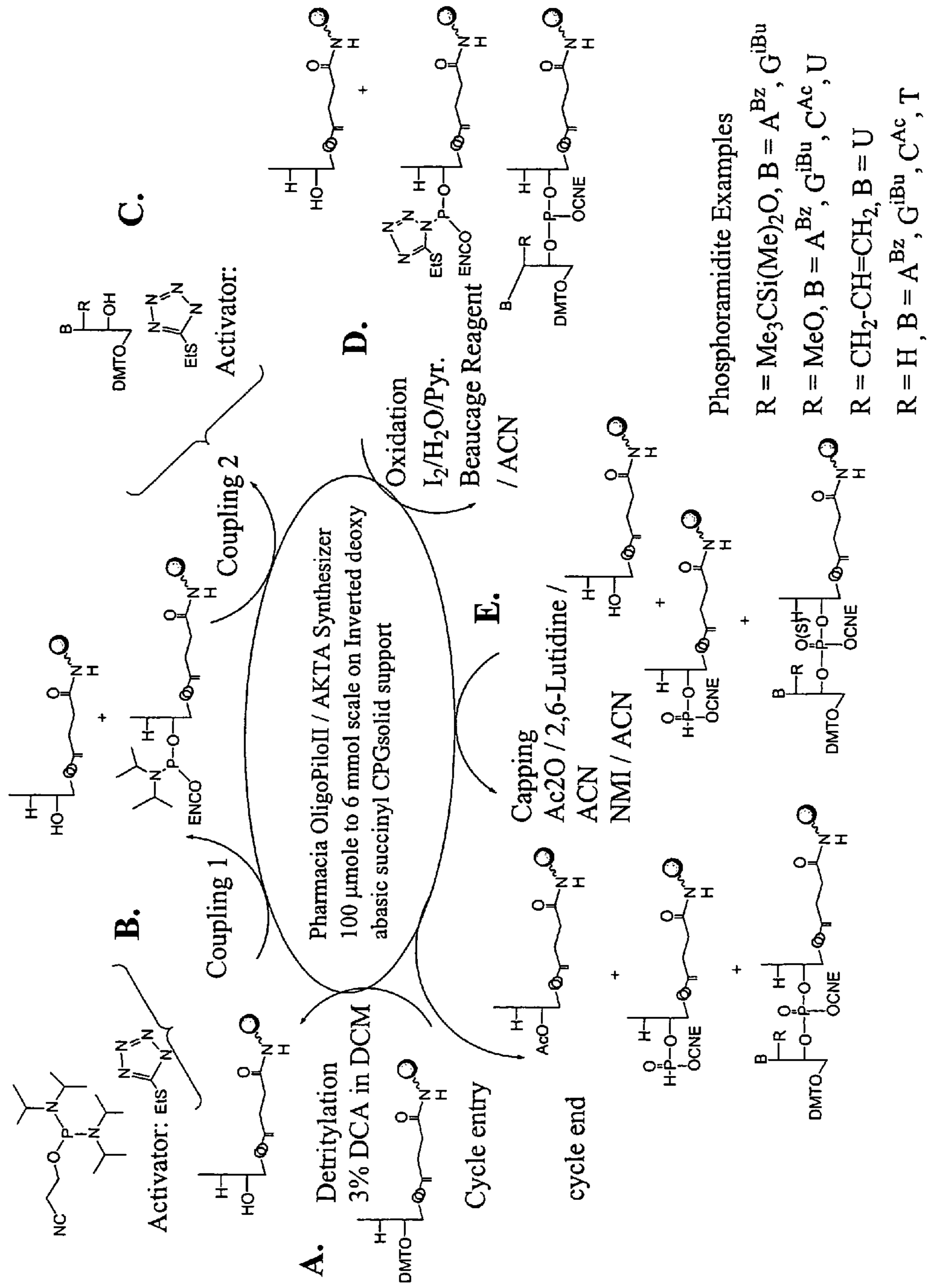
Figure 11: Chemical Synthesis of Oligonucleotides, in situ Phosphoramidite
