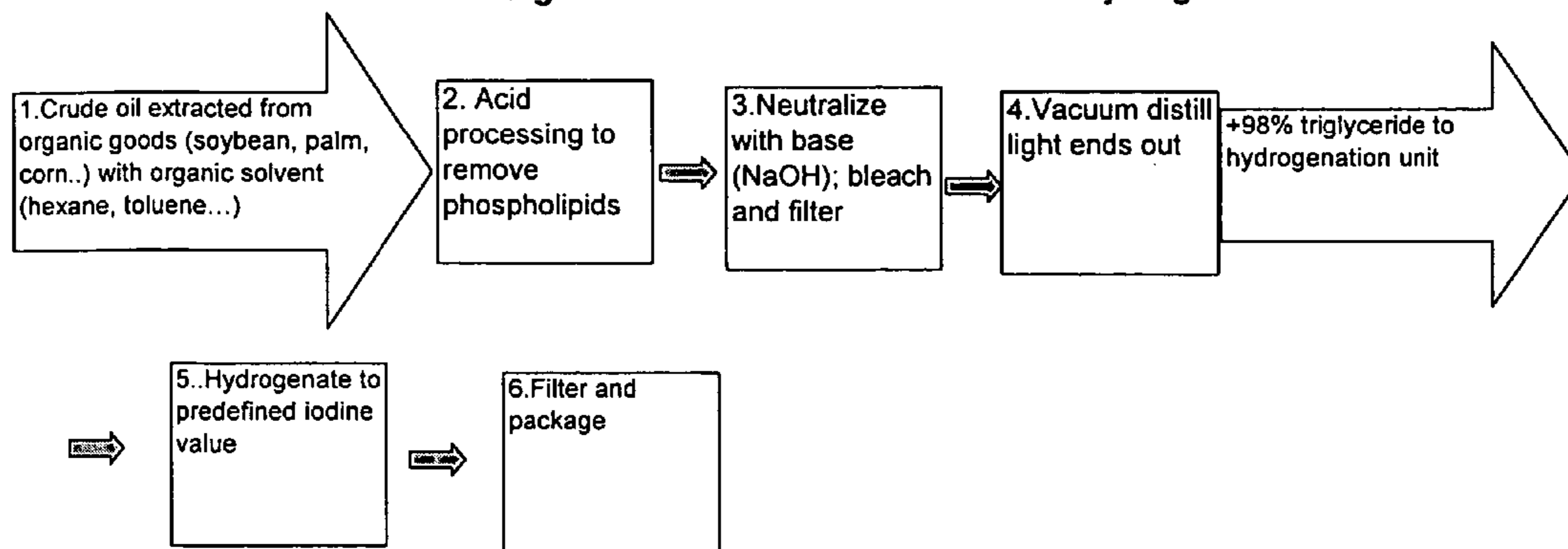
Fig. 1 Process for the manufacture of Hydrogenated oils
