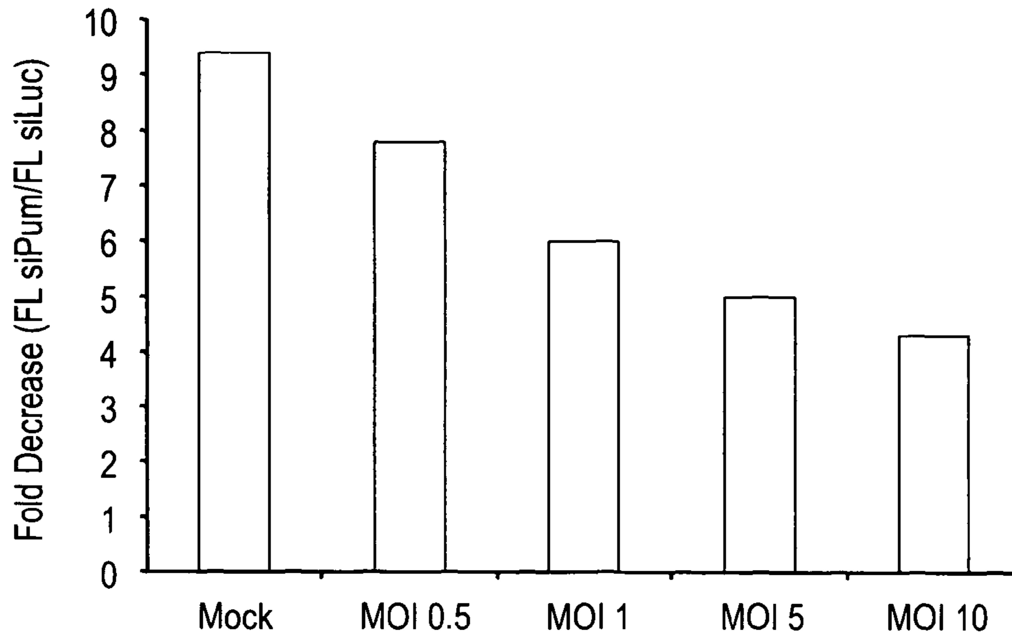
WT Ad-5- Induced Reduction in siRNA Activity
