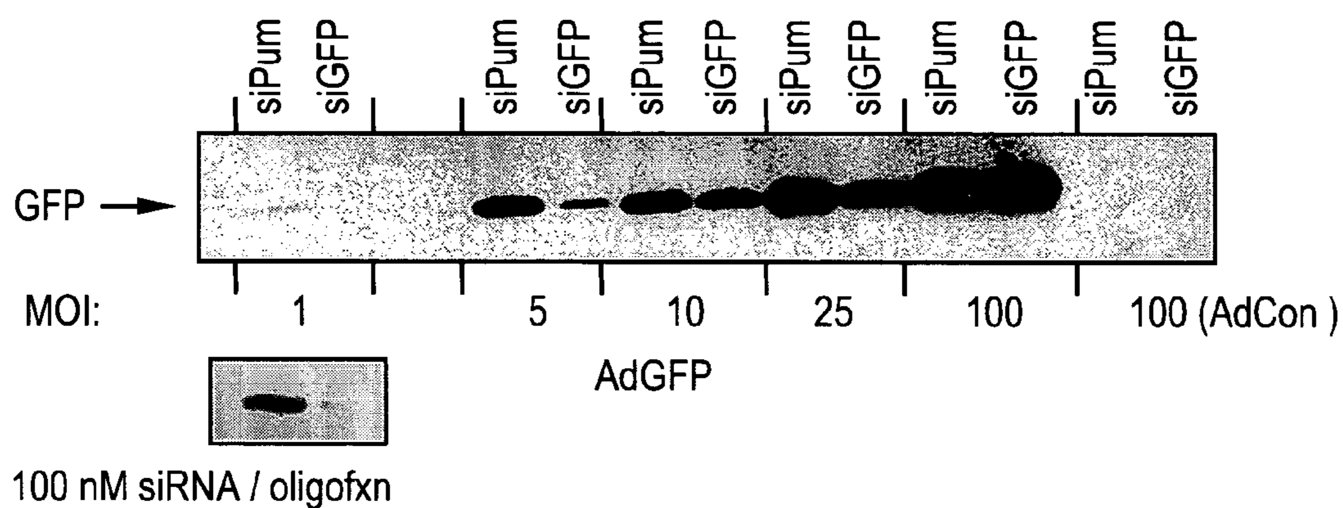
siRNA-Induced Reduction in Virally Encoded Reporter Gene Expression (Non-Replicating)
