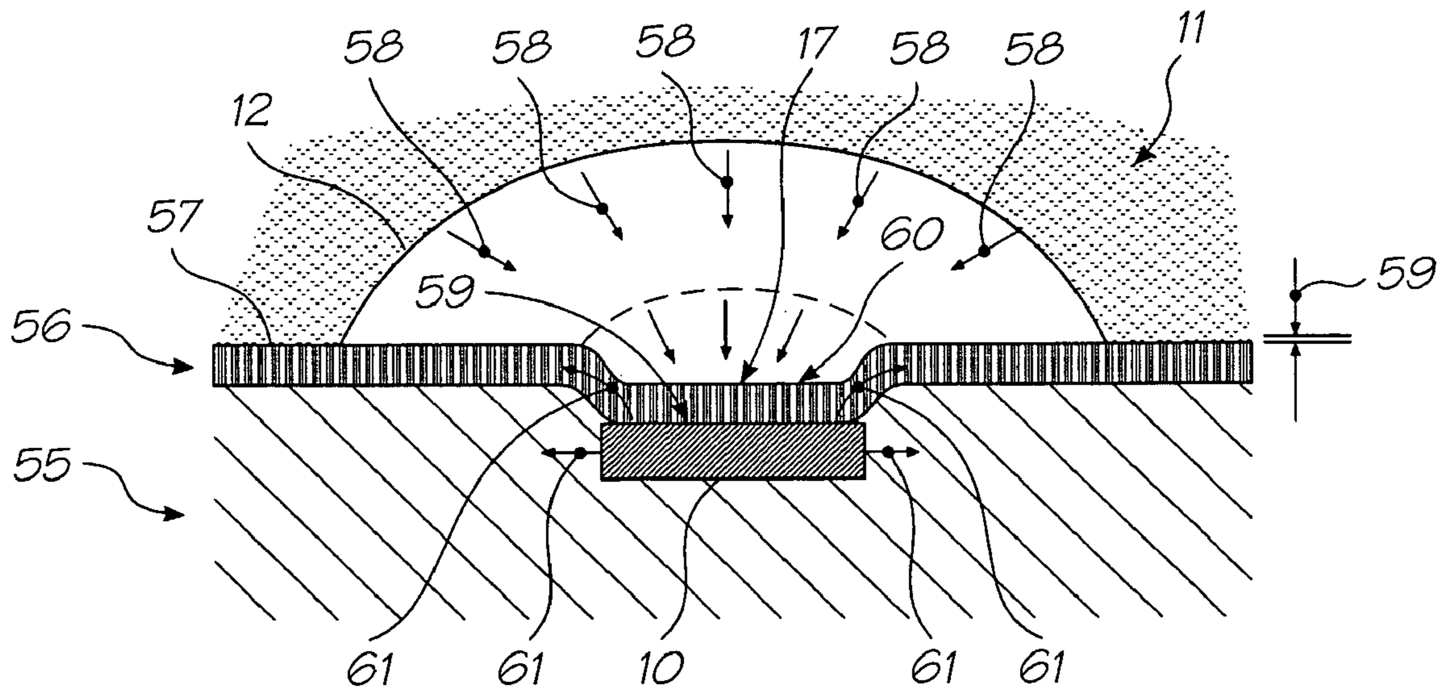
FIG. 47 (PRIOR ART)
