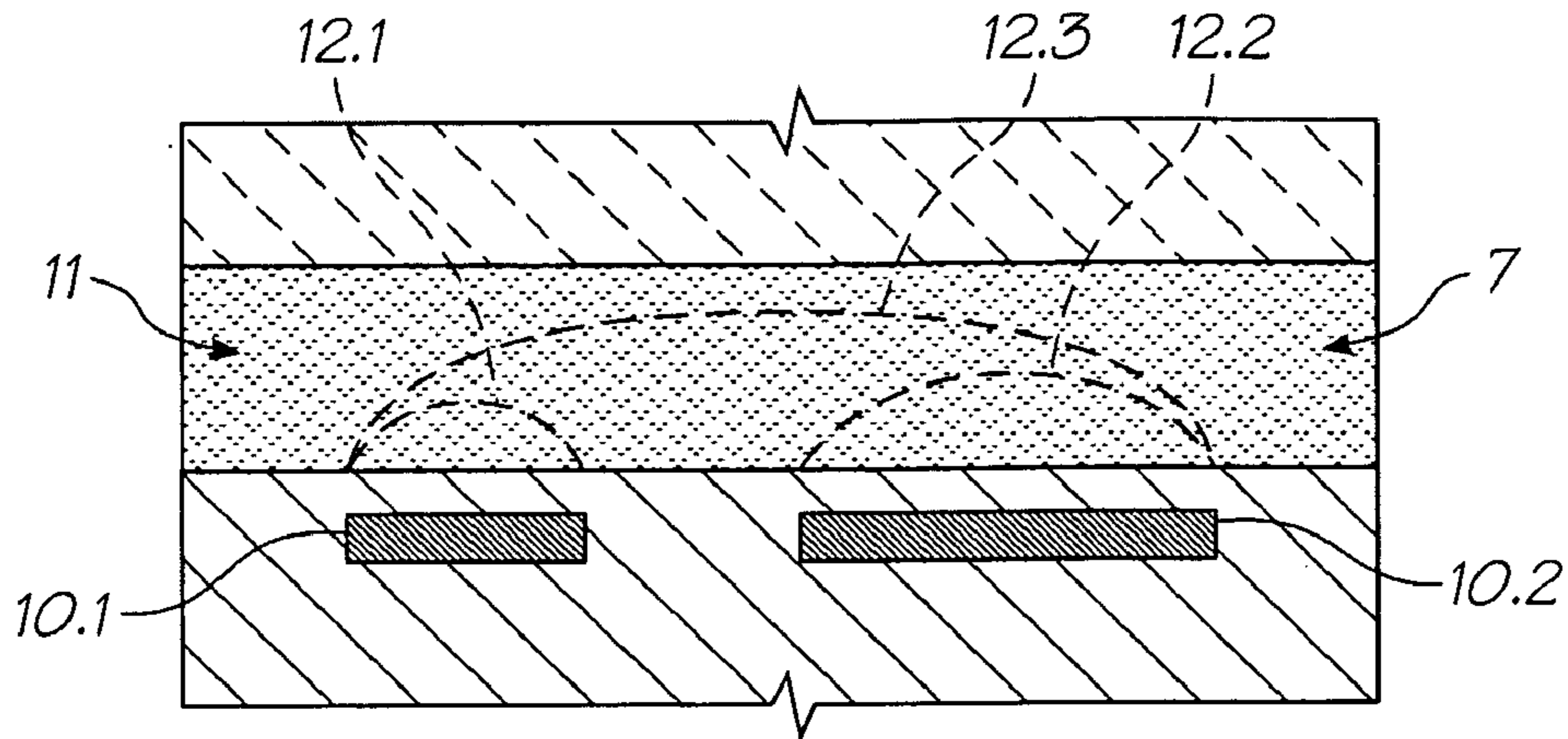
FIG. 52 (PRIOR ART)
