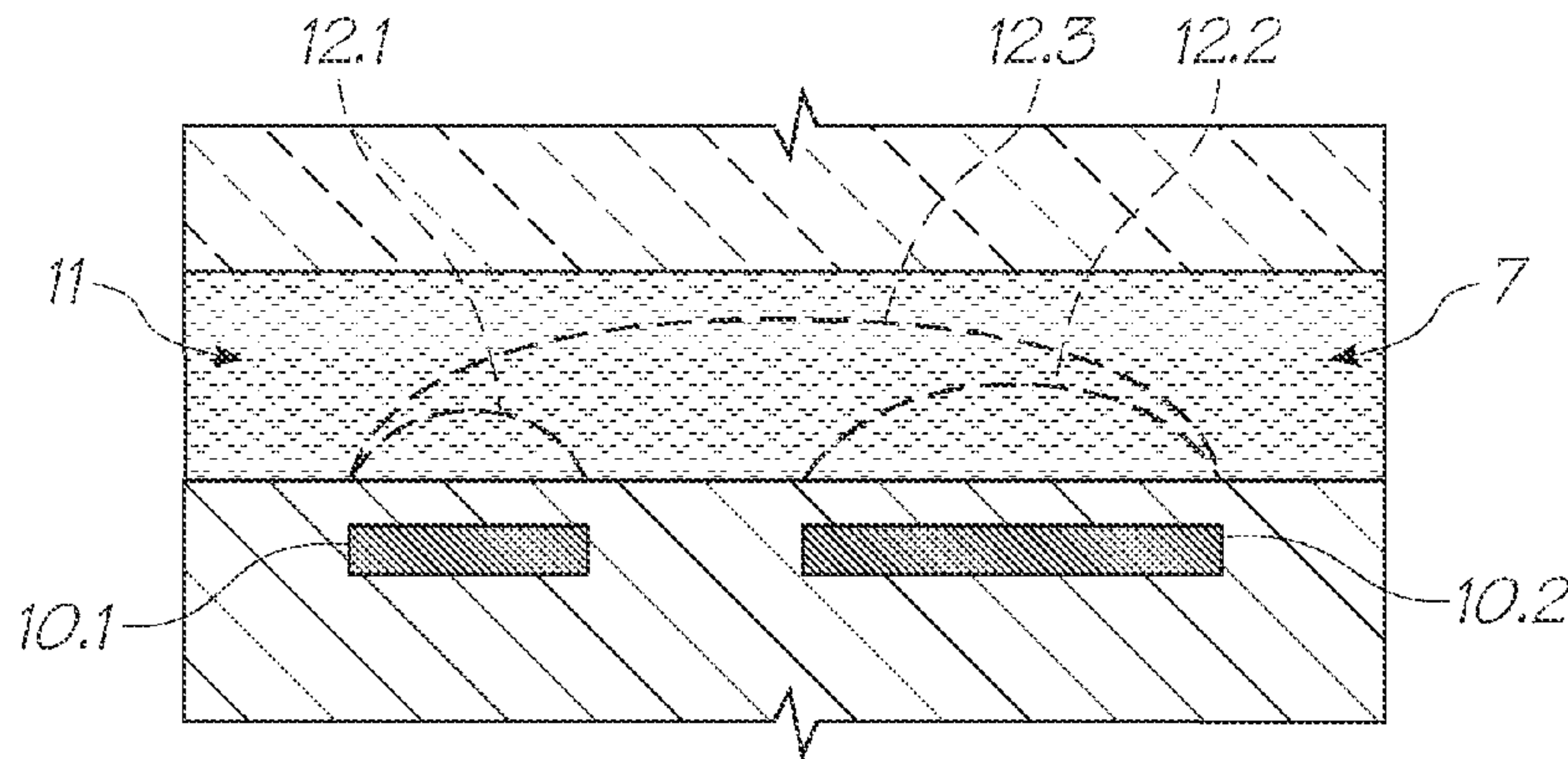
FIG. 52 (PRIOR ART)
