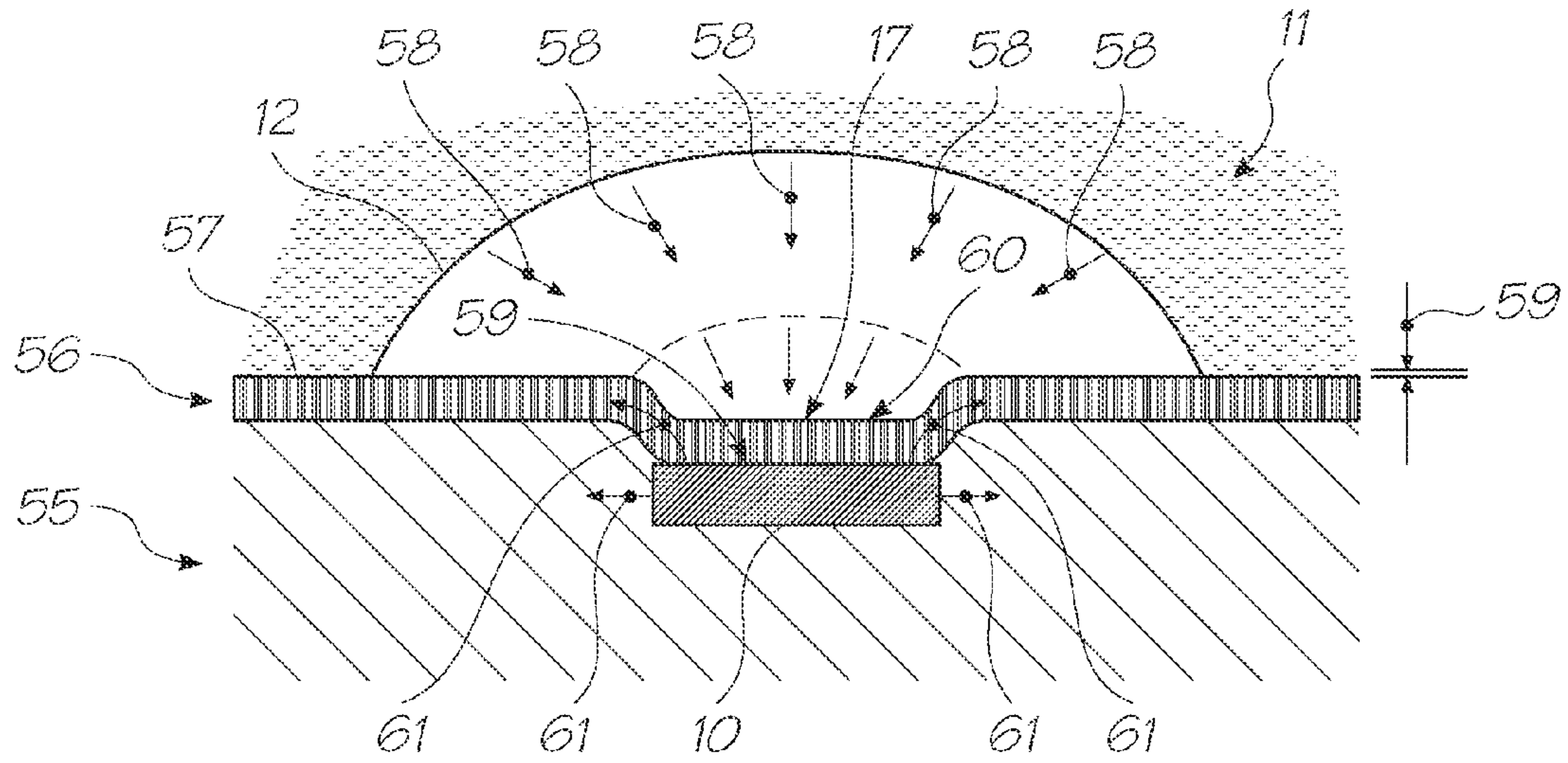
FIG. 47 (PRIOR ART)
