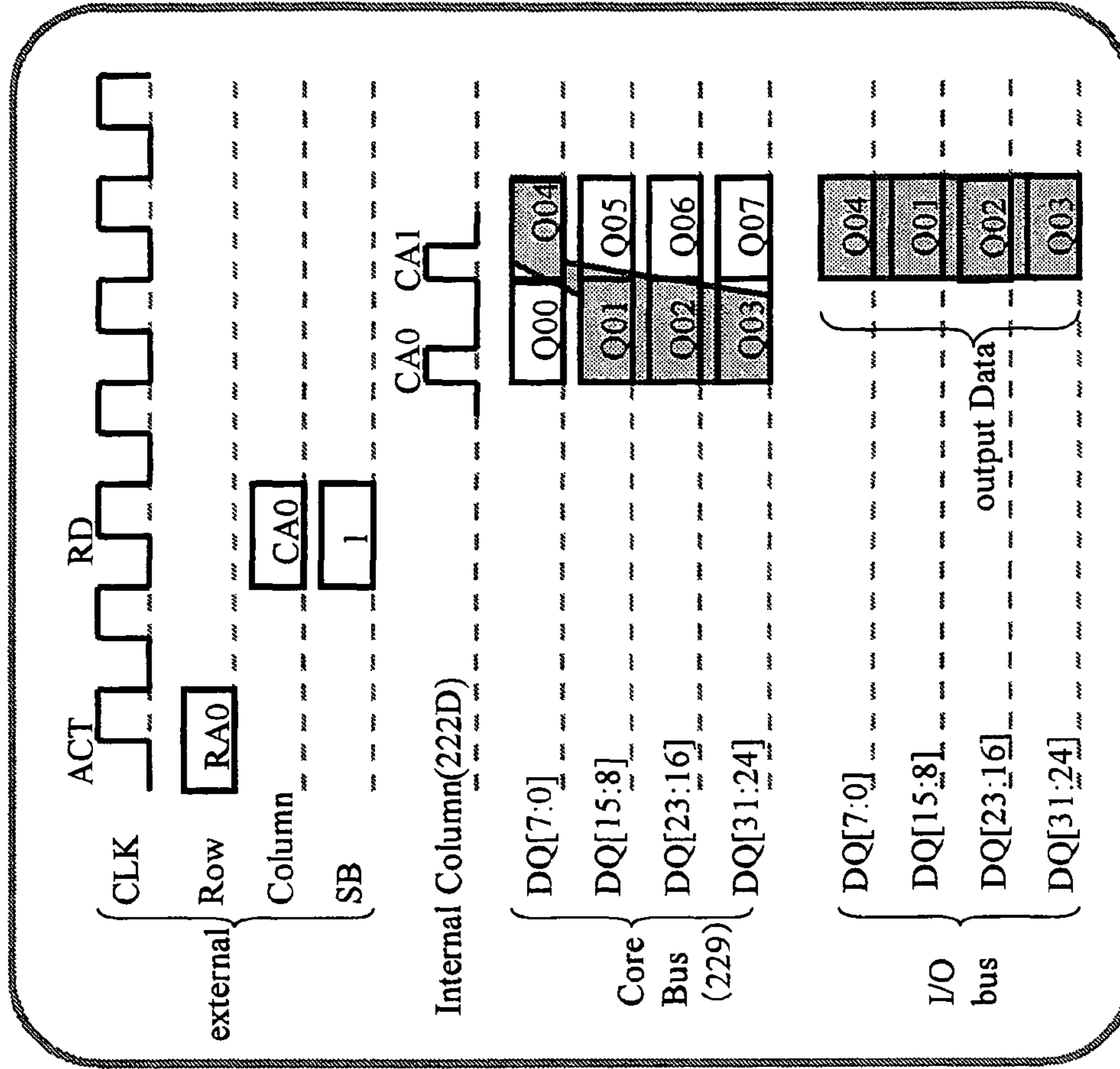
Read Operation [SB="1"]
