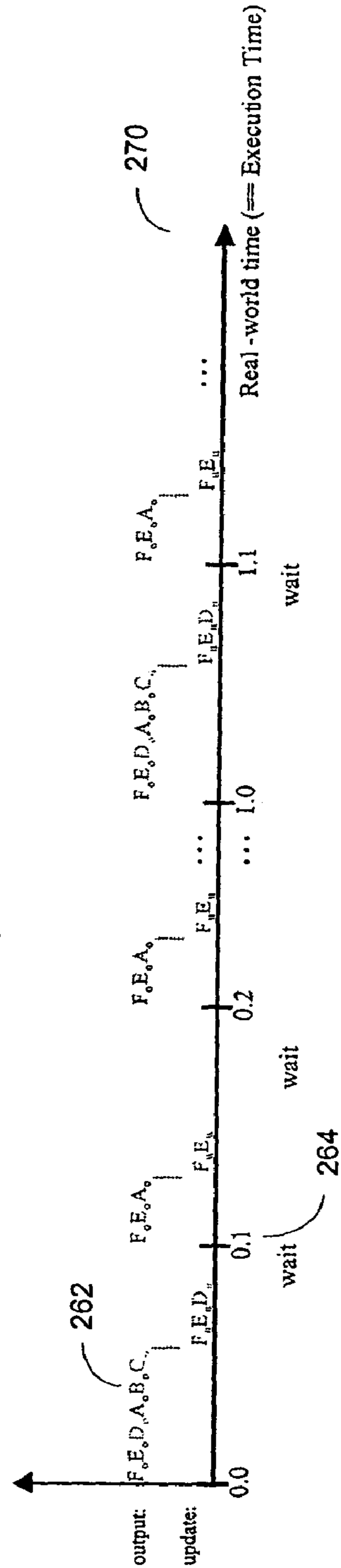
Single tasking execution in a real-time system
