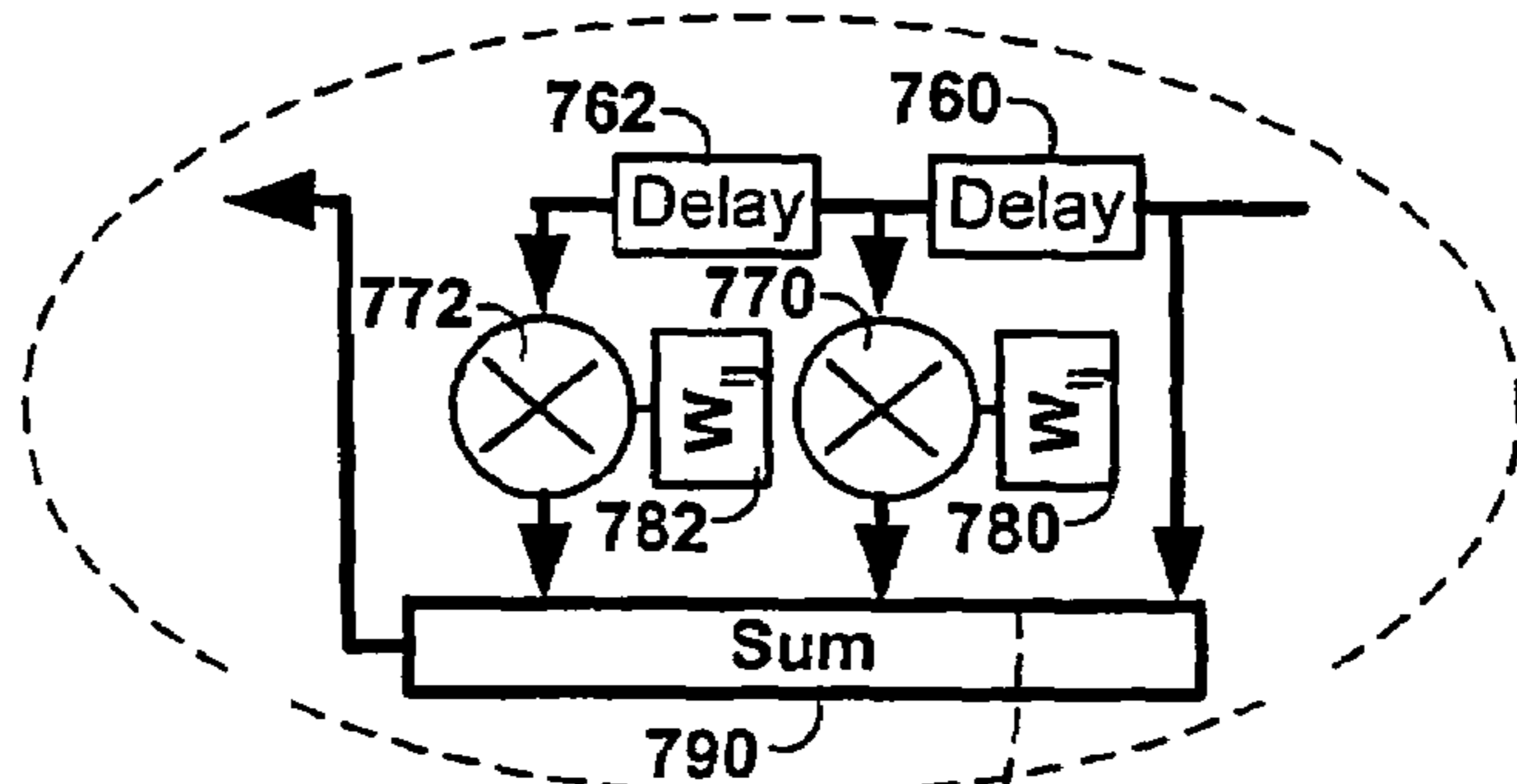
Space-Time Processor FIG. 7C
