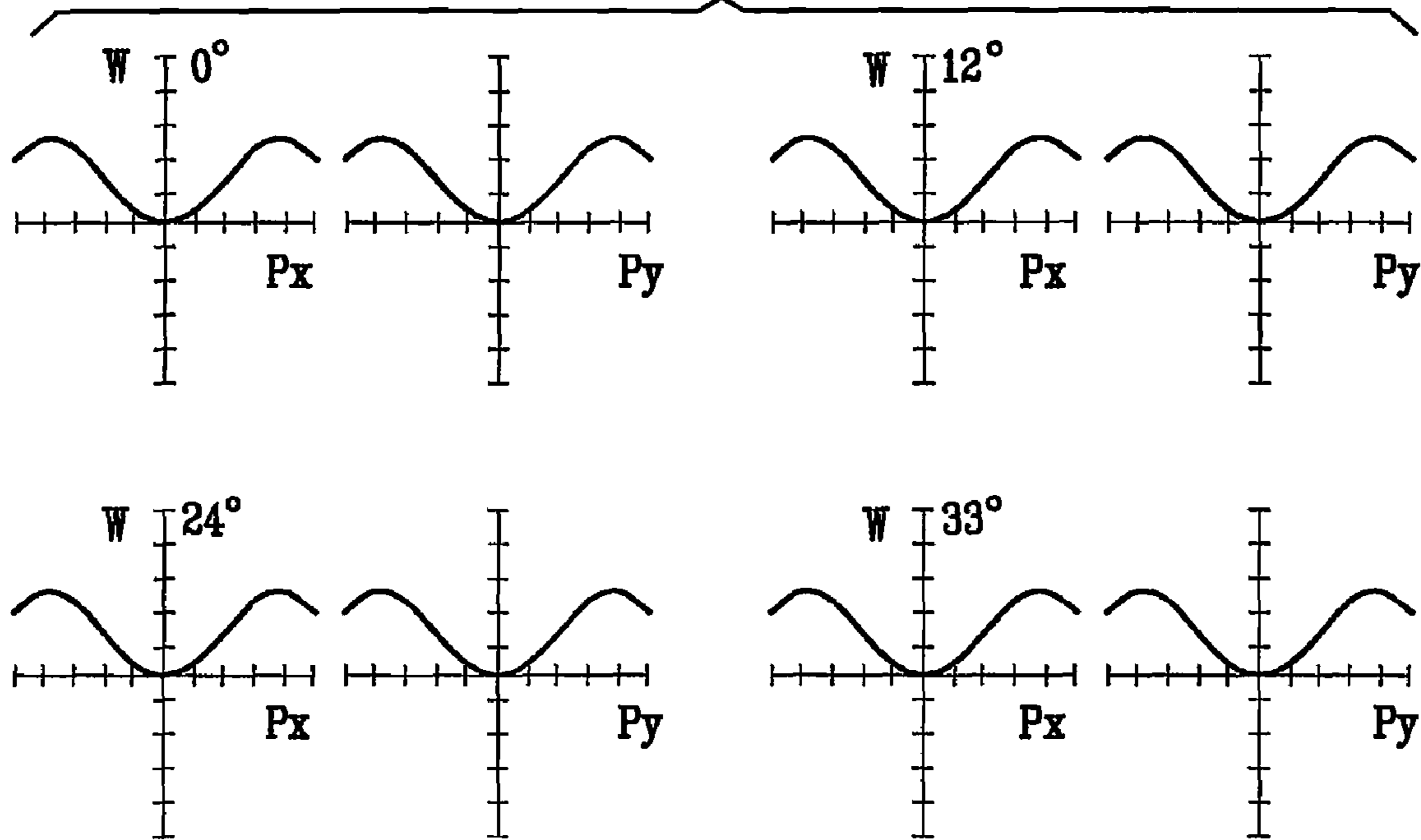
OPTICAL PATH DIFFERENCE AT DIFFERENT FIELDS OF VIEW (FOV)
