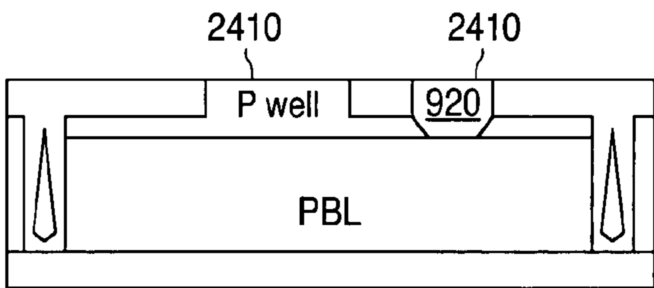
PNP
