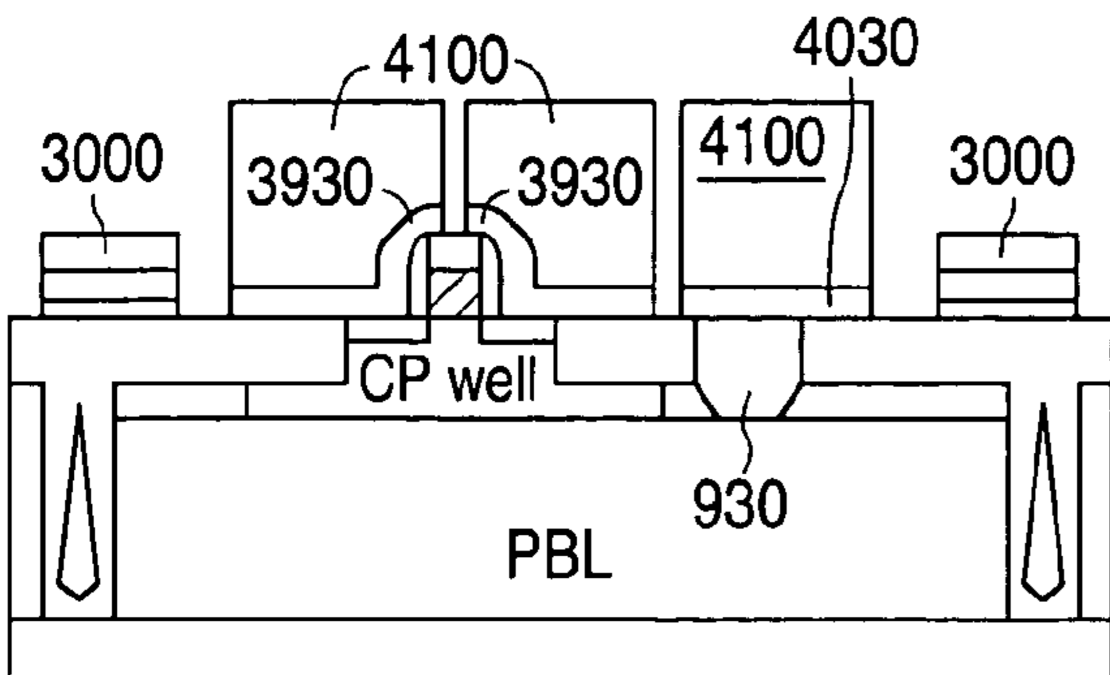
NMOS FIG. 41C
