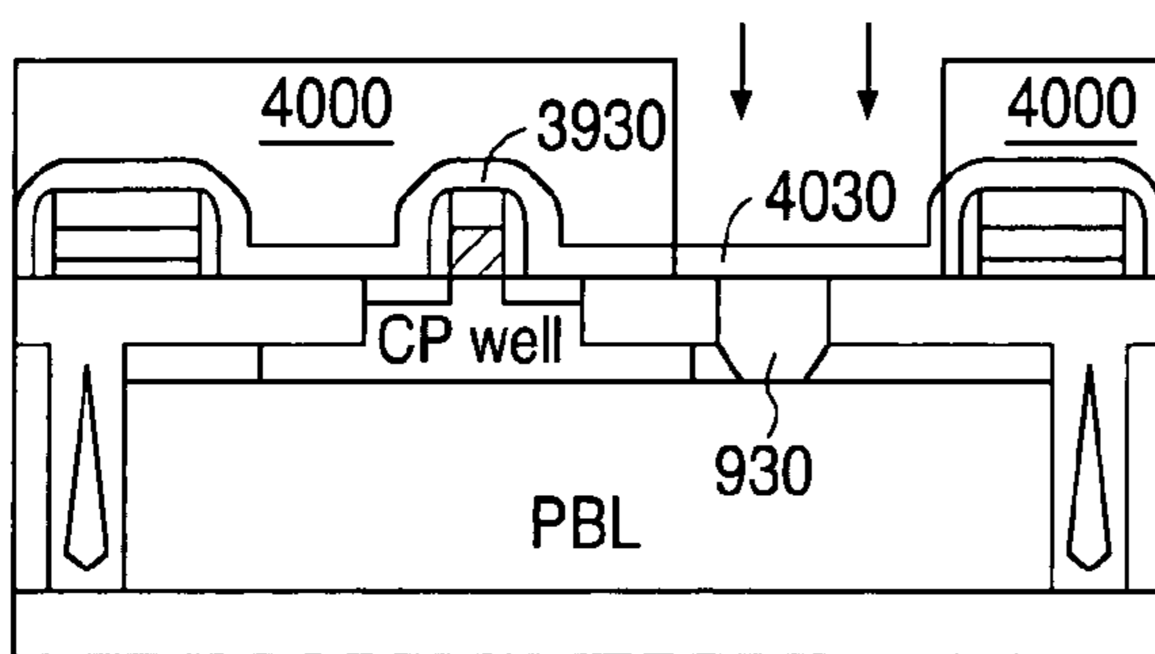
NMOS FIG. 40C
