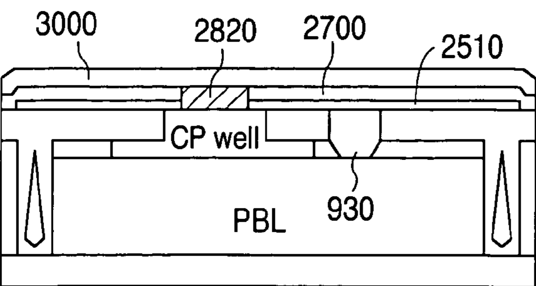
NMOS FIG. 30C
