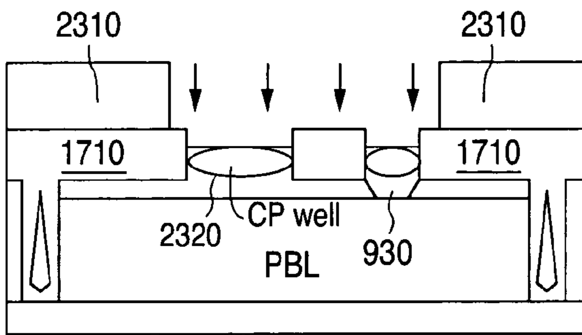
NMOS
