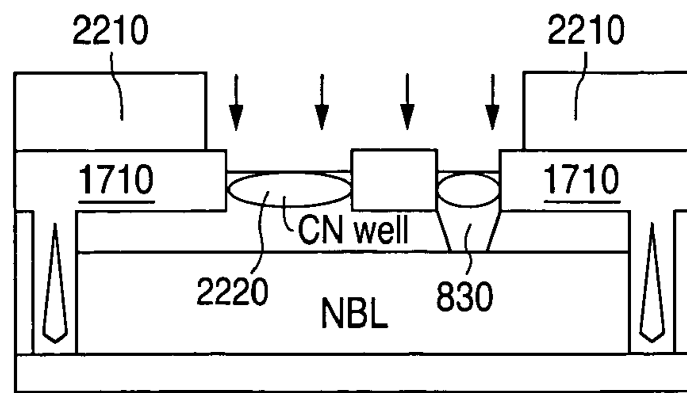
PMOS FIG. 22D
