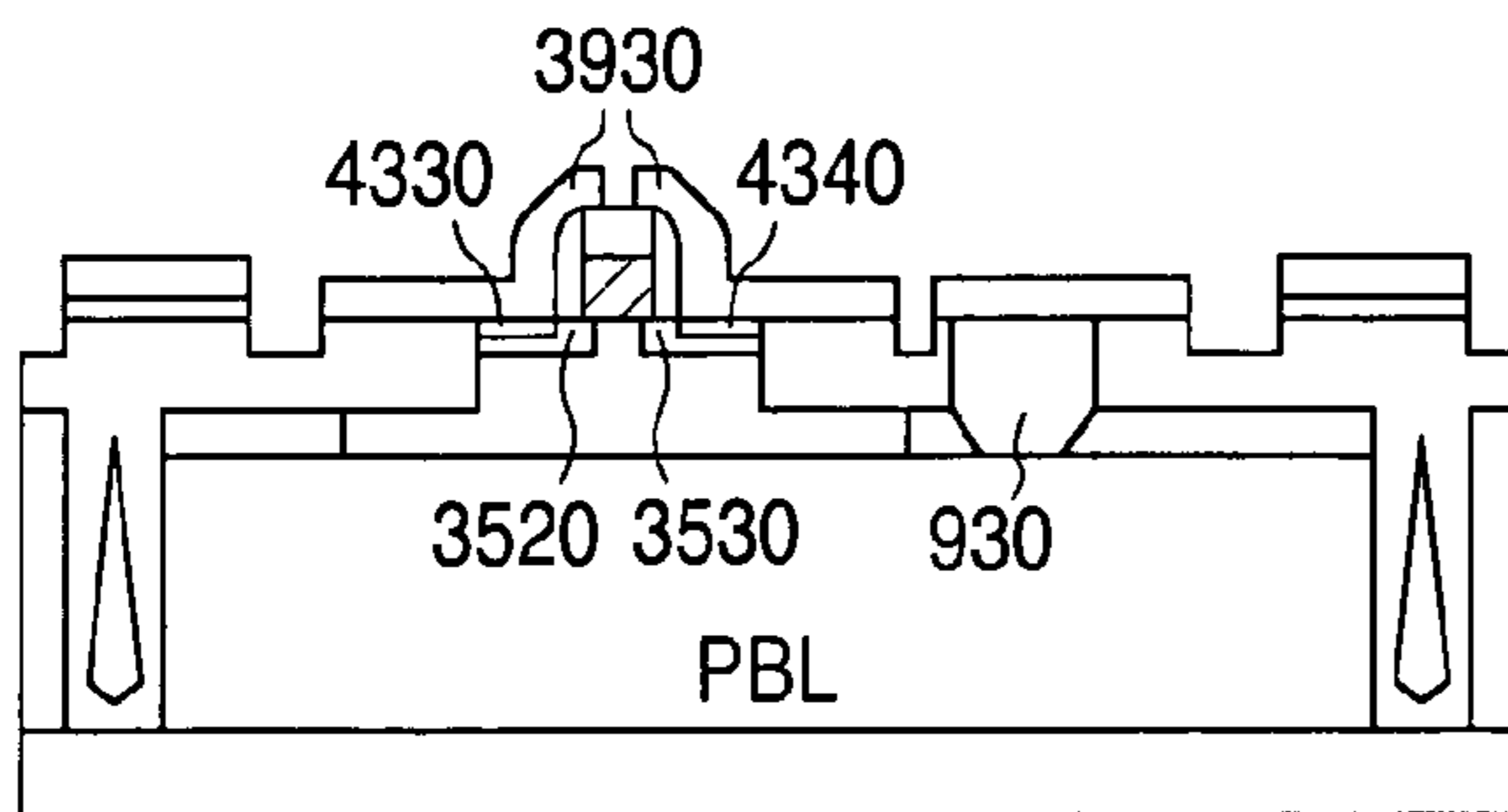
NMOS
