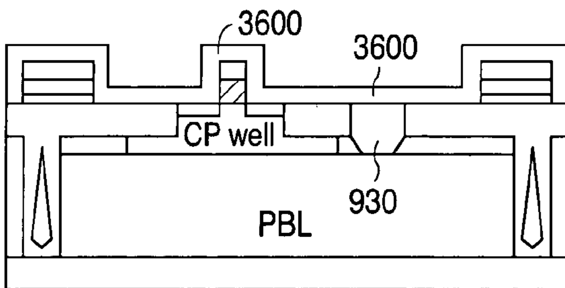
NMOS FIG. 36C
