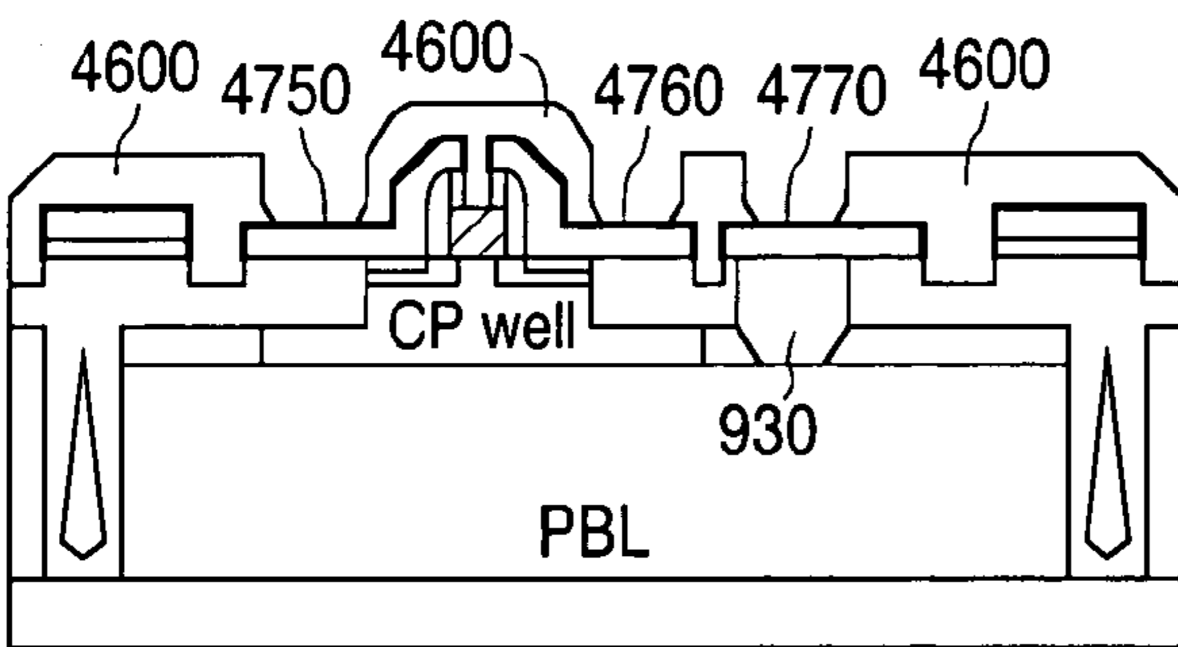
NMOS
