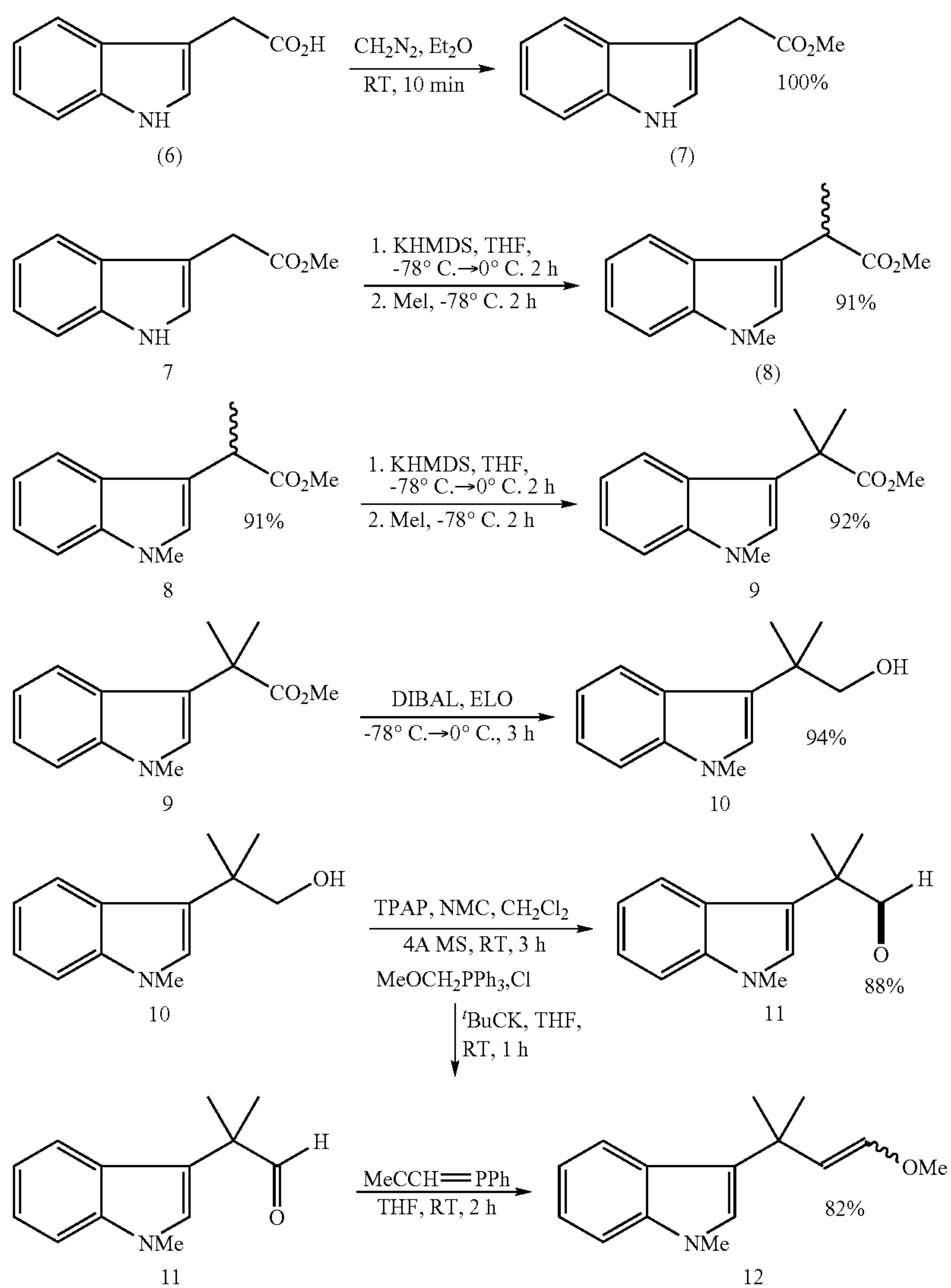
Scheme 2
