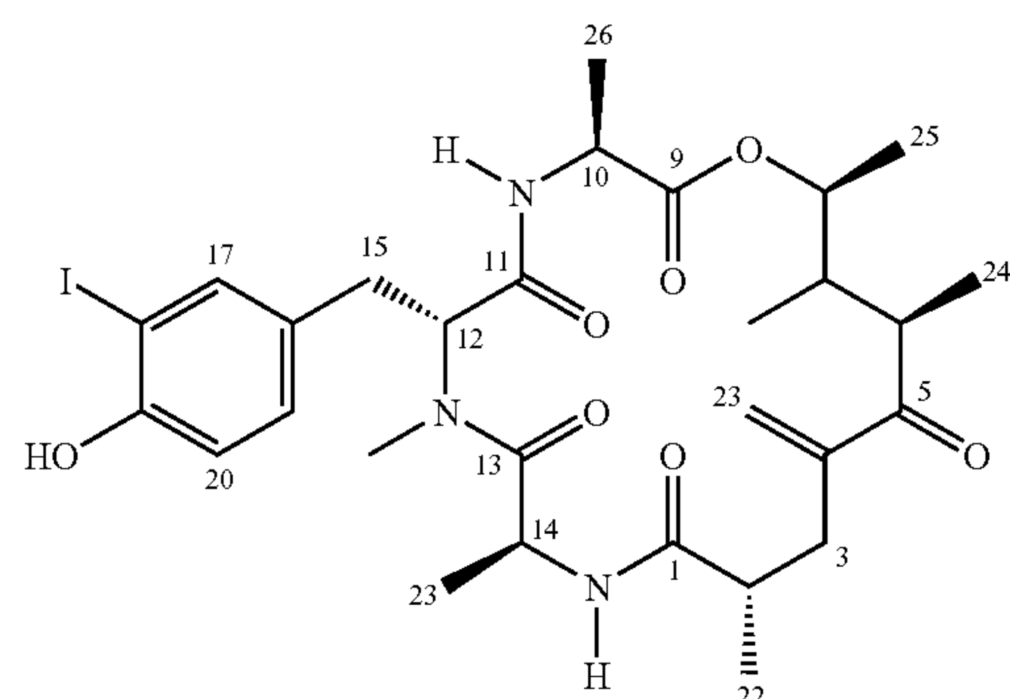
Compound 1
