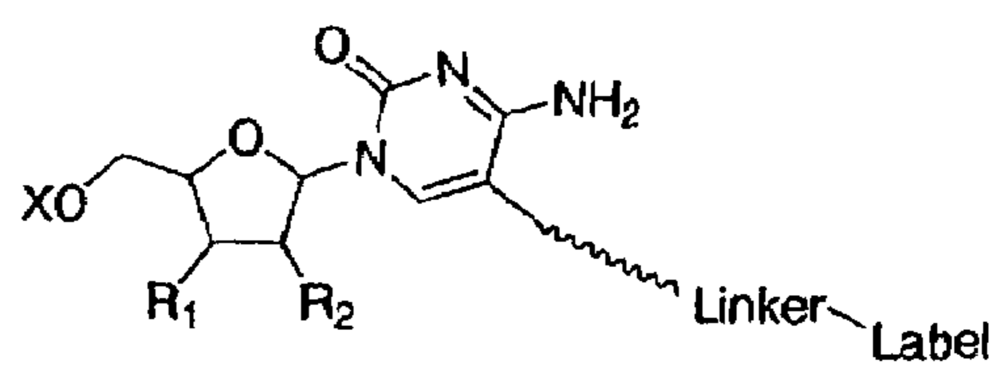
Cytidine C5-linker
