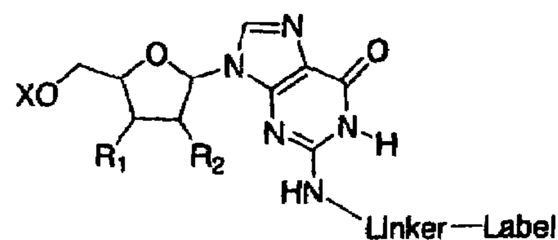
Guanosine N2-linker
