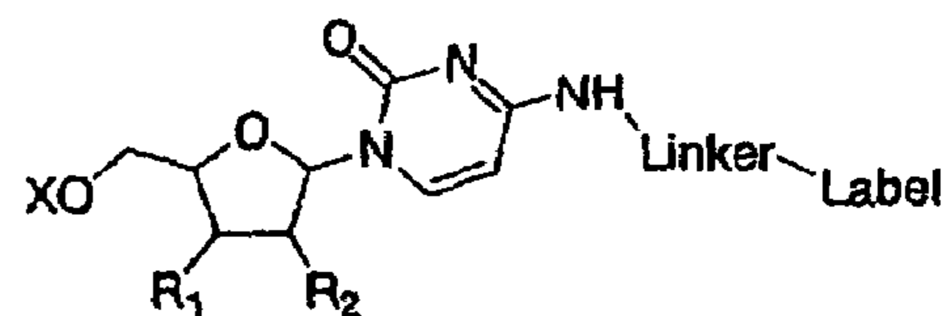
Cytidine N4-linker
