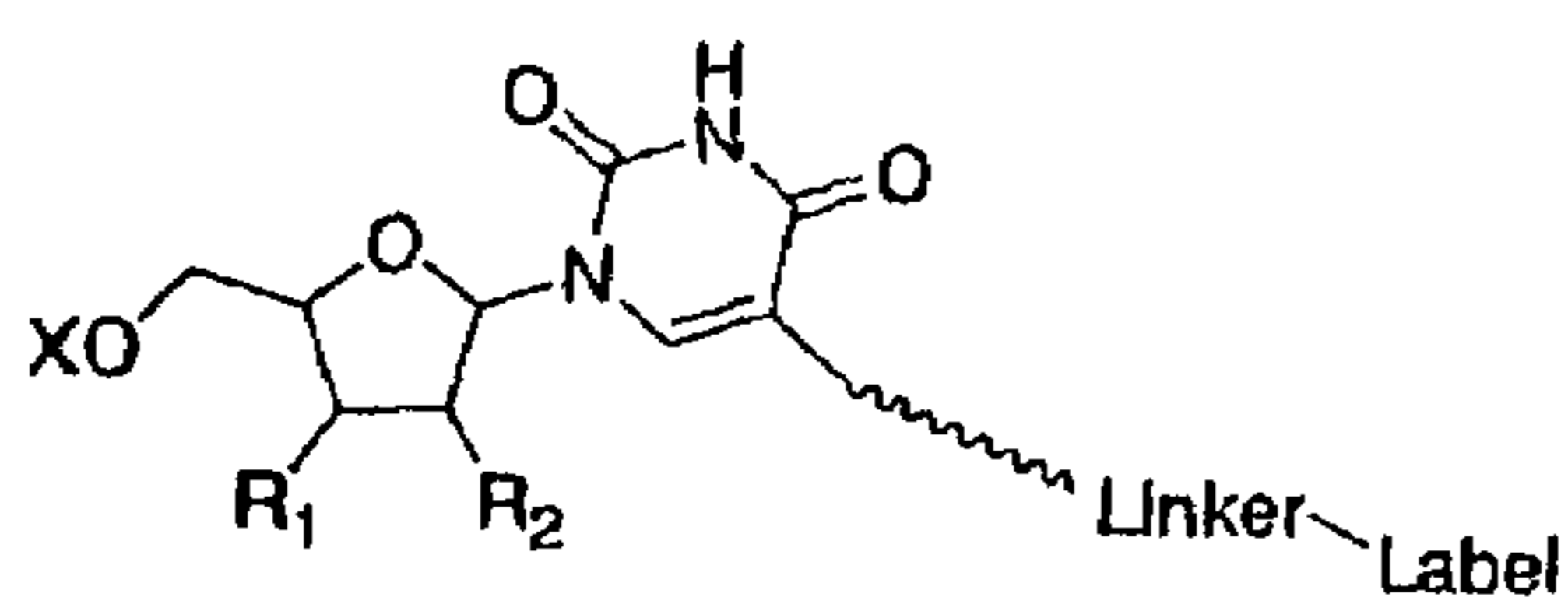
Uridine C5-linker
