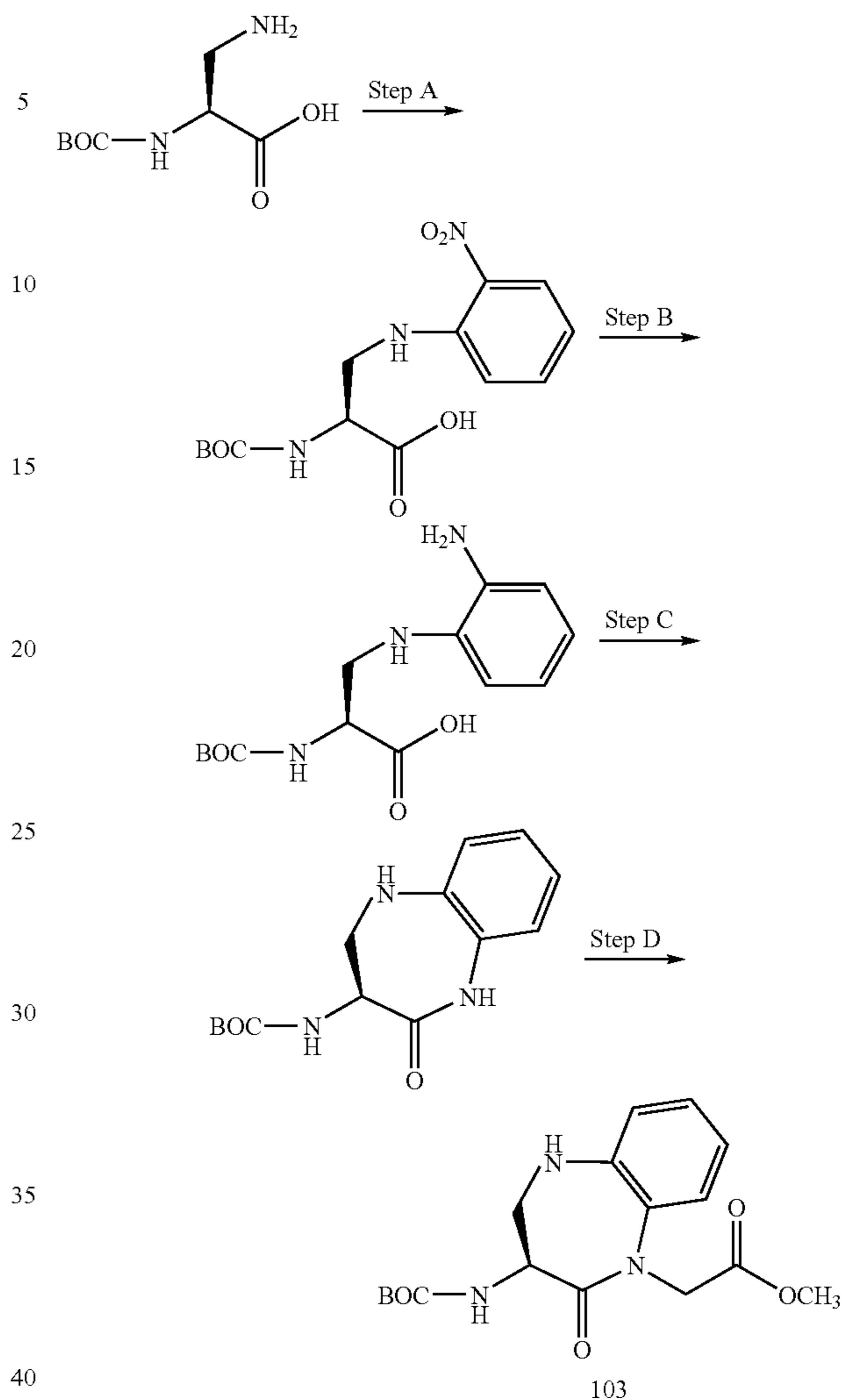
(3-tert-Butoxycarbonylamino-2-oxo-2,3,4,5-tetrahydro-benzo[b][1,4]diazepin-1-yl)acetic Acid Methyl Ester
