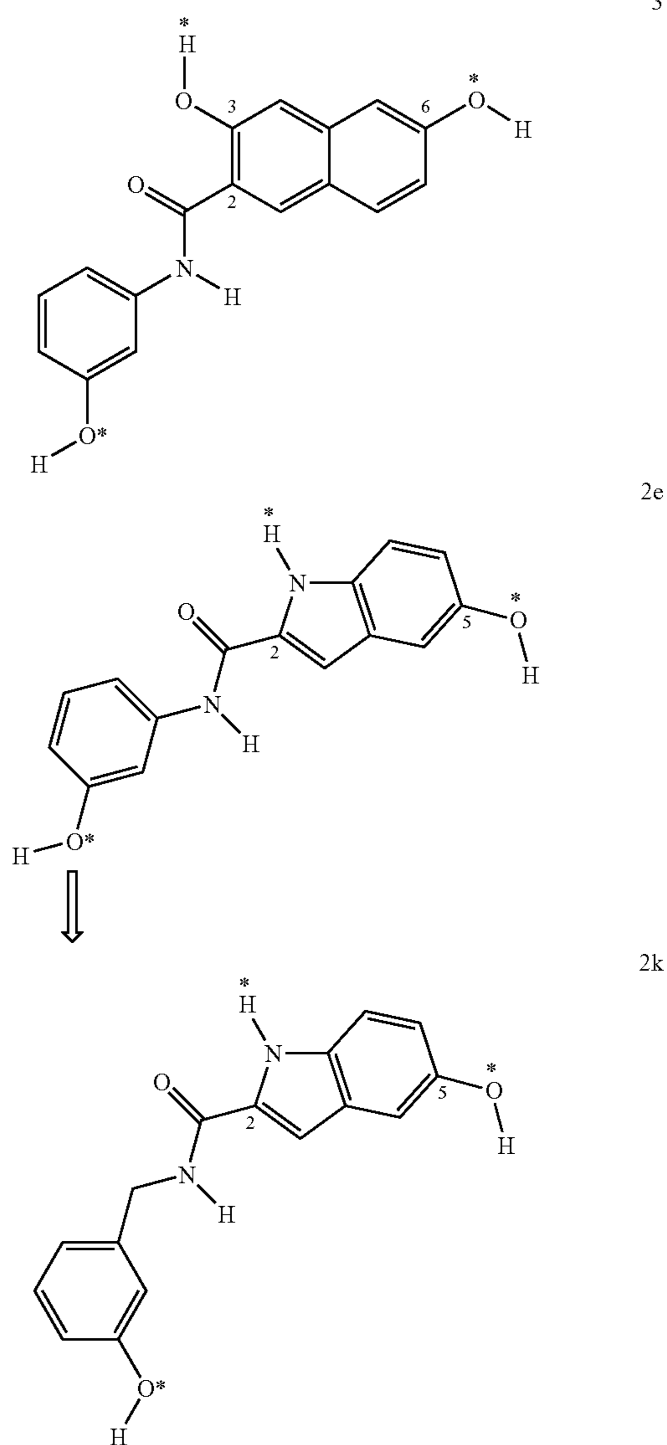
Scheme 3
