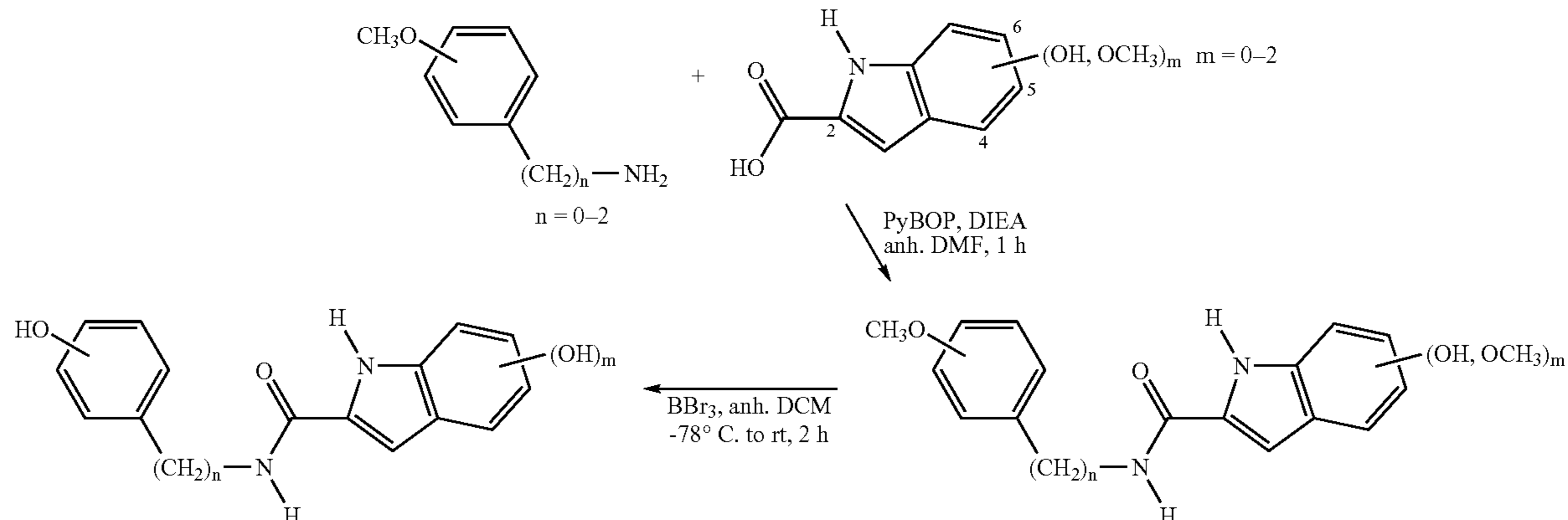
Scheme 2
