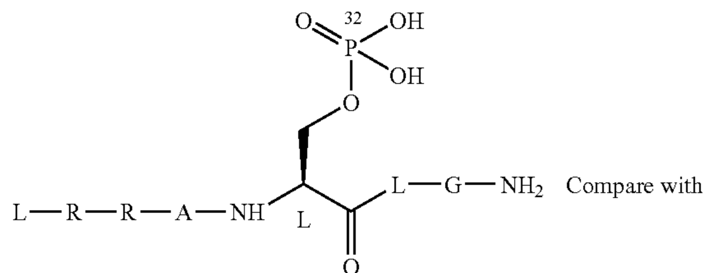
Phosphorylated Kemptamide
