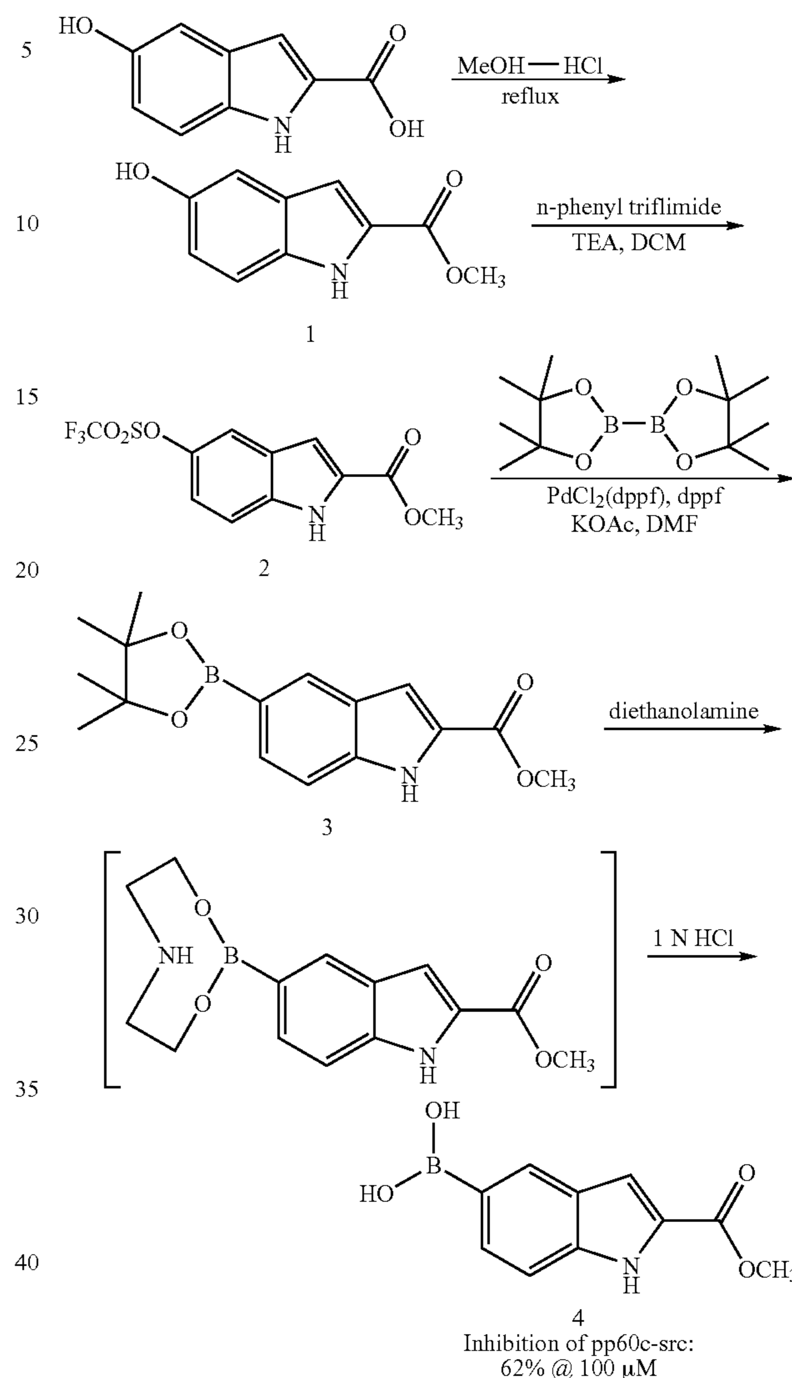
Scheme 1
