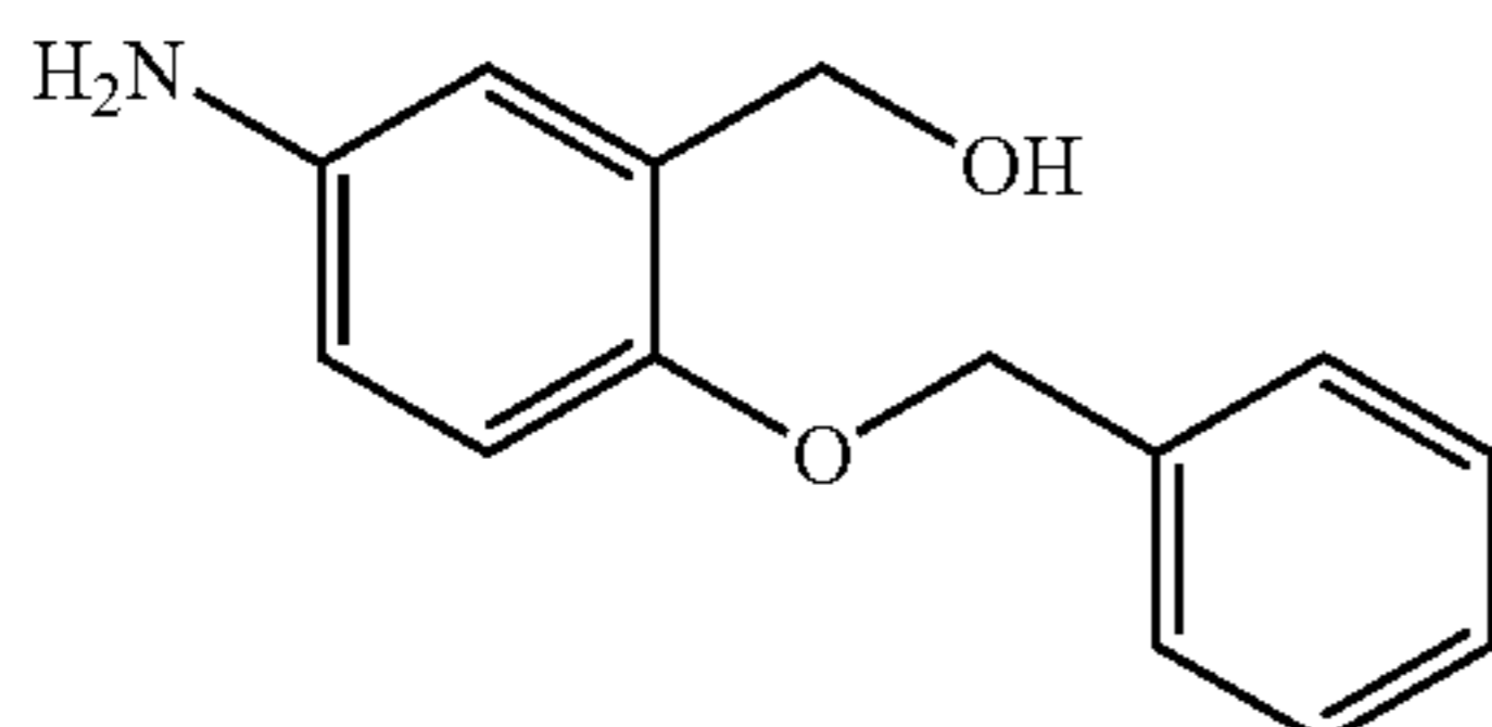
4-benzyloxy-3-hydroxymethylaniline
