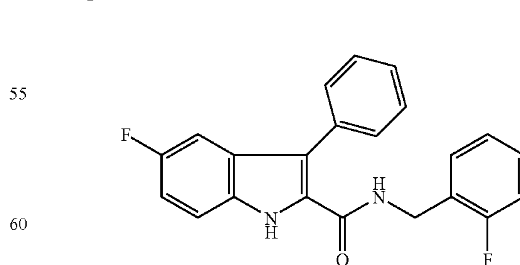
Compound 2s
