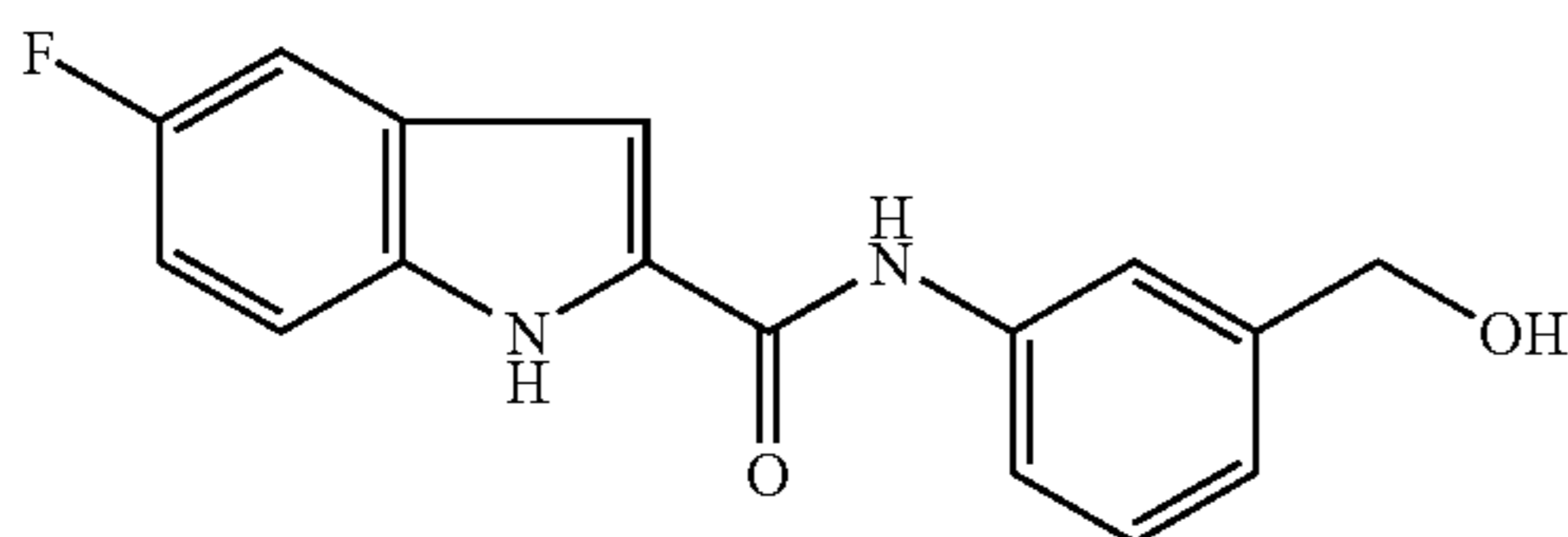
Compound 1yyy
