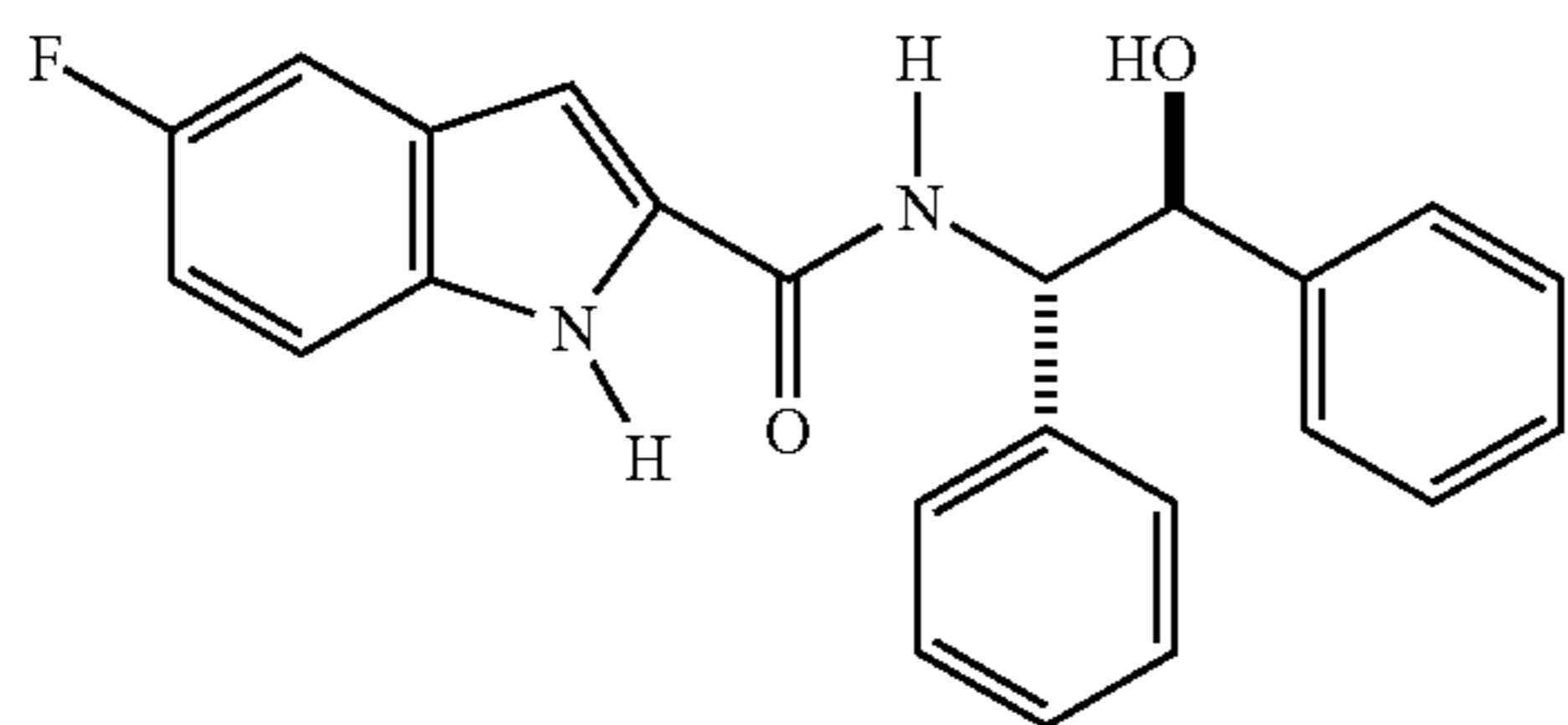
Compound 1dd
