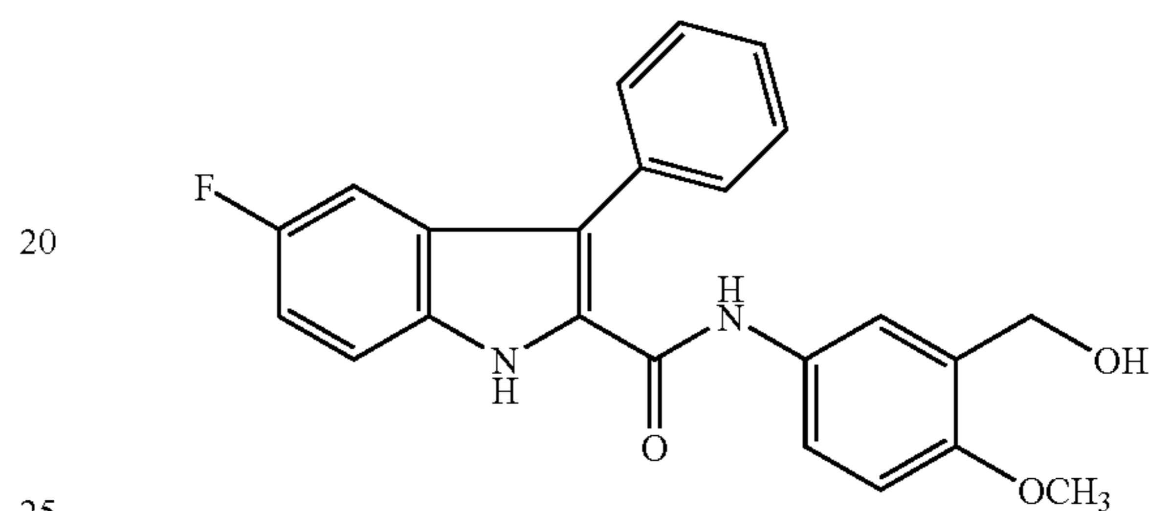
Compound 2f
