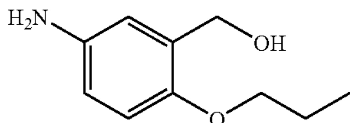
3-hydroxymethyl-4-propyloxyaniline
