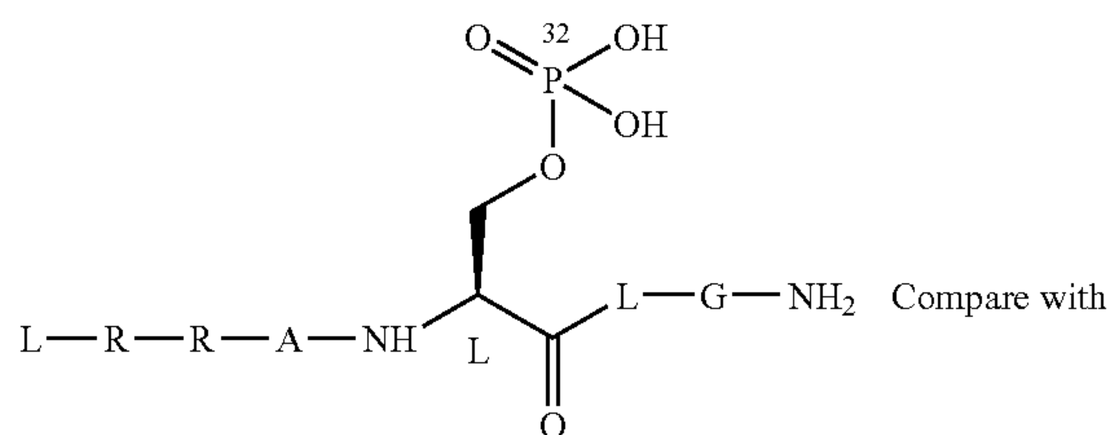
Phosphorylated Kemptamide
