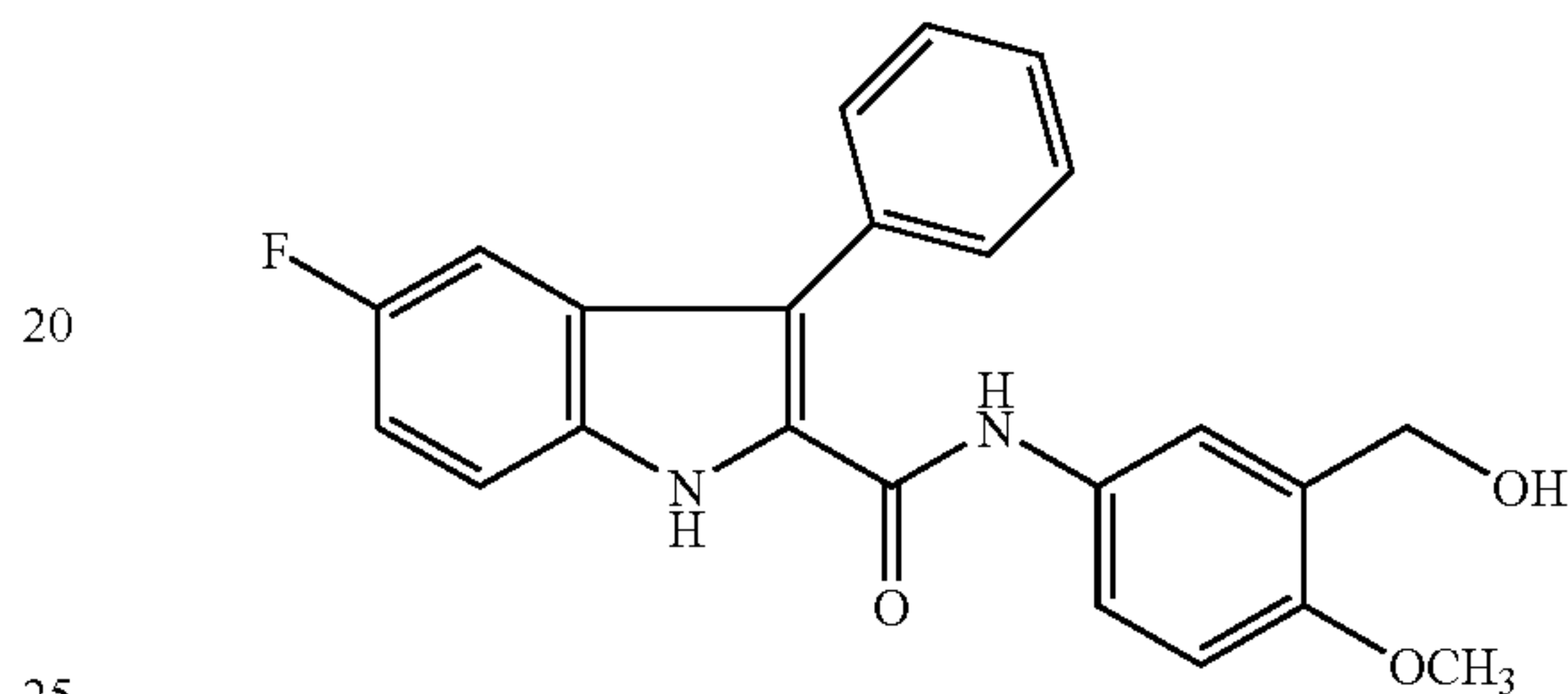
Compound 2f
