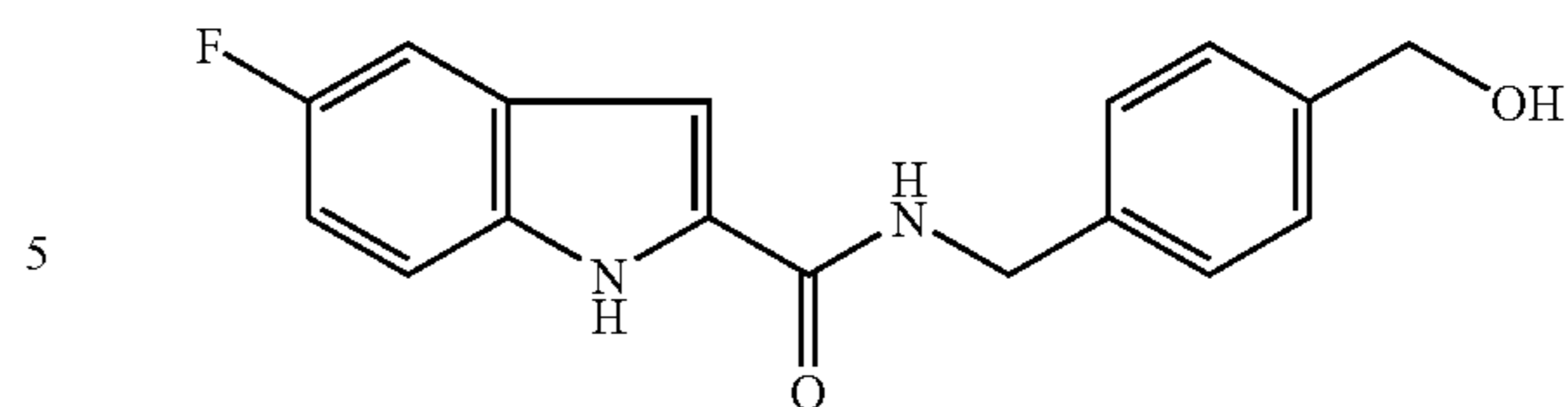
Compound 1oooo
