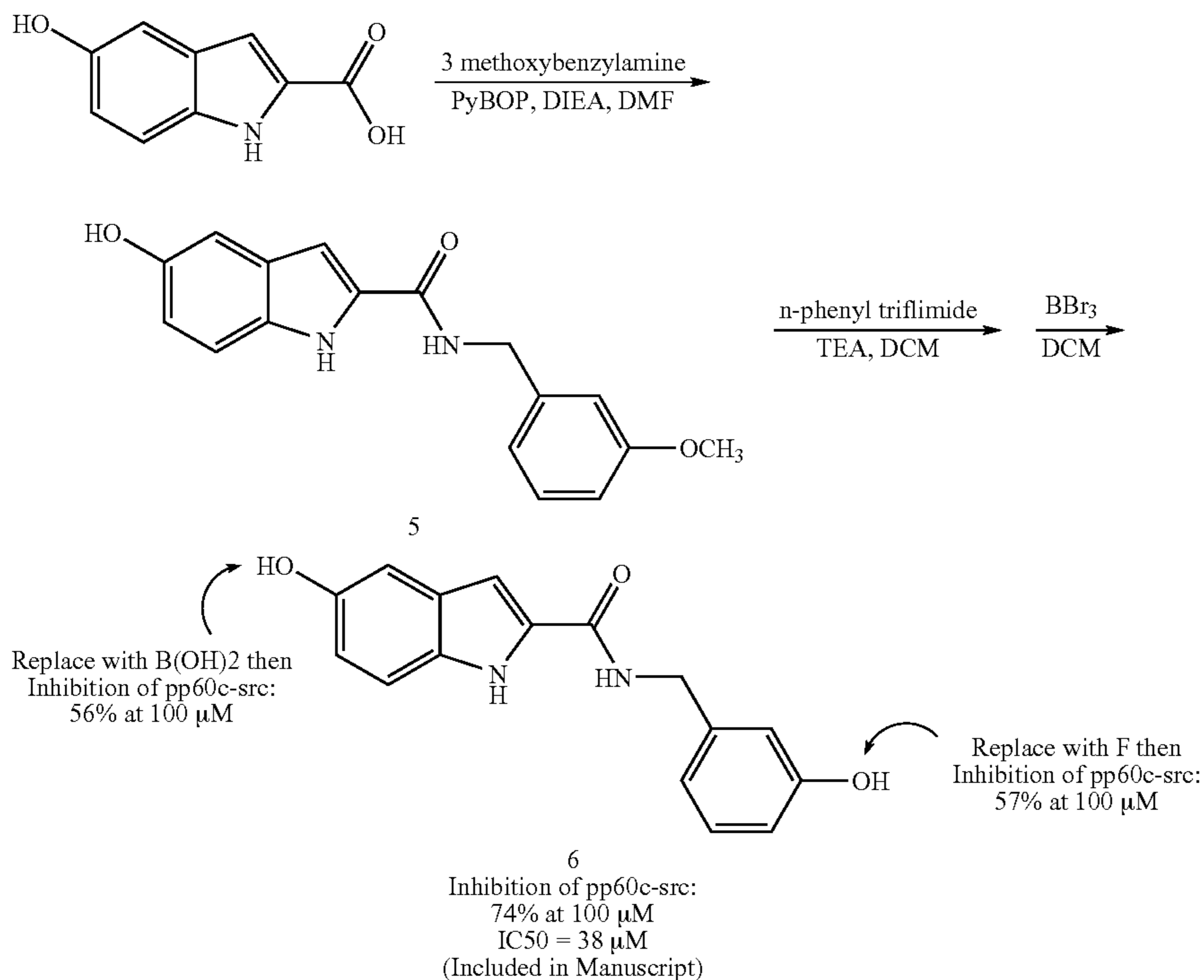
Scheme 2
