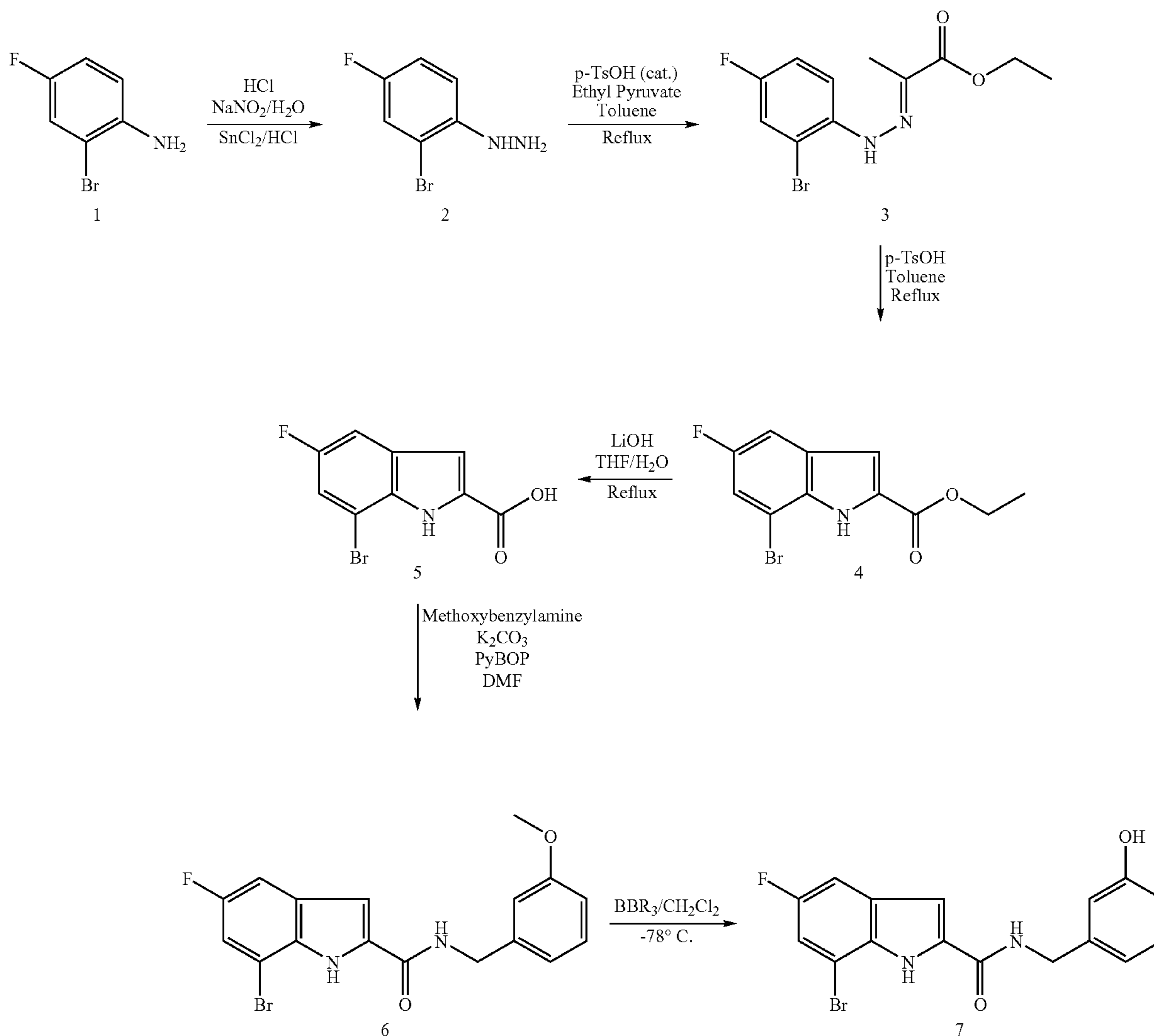
Scheme 1
