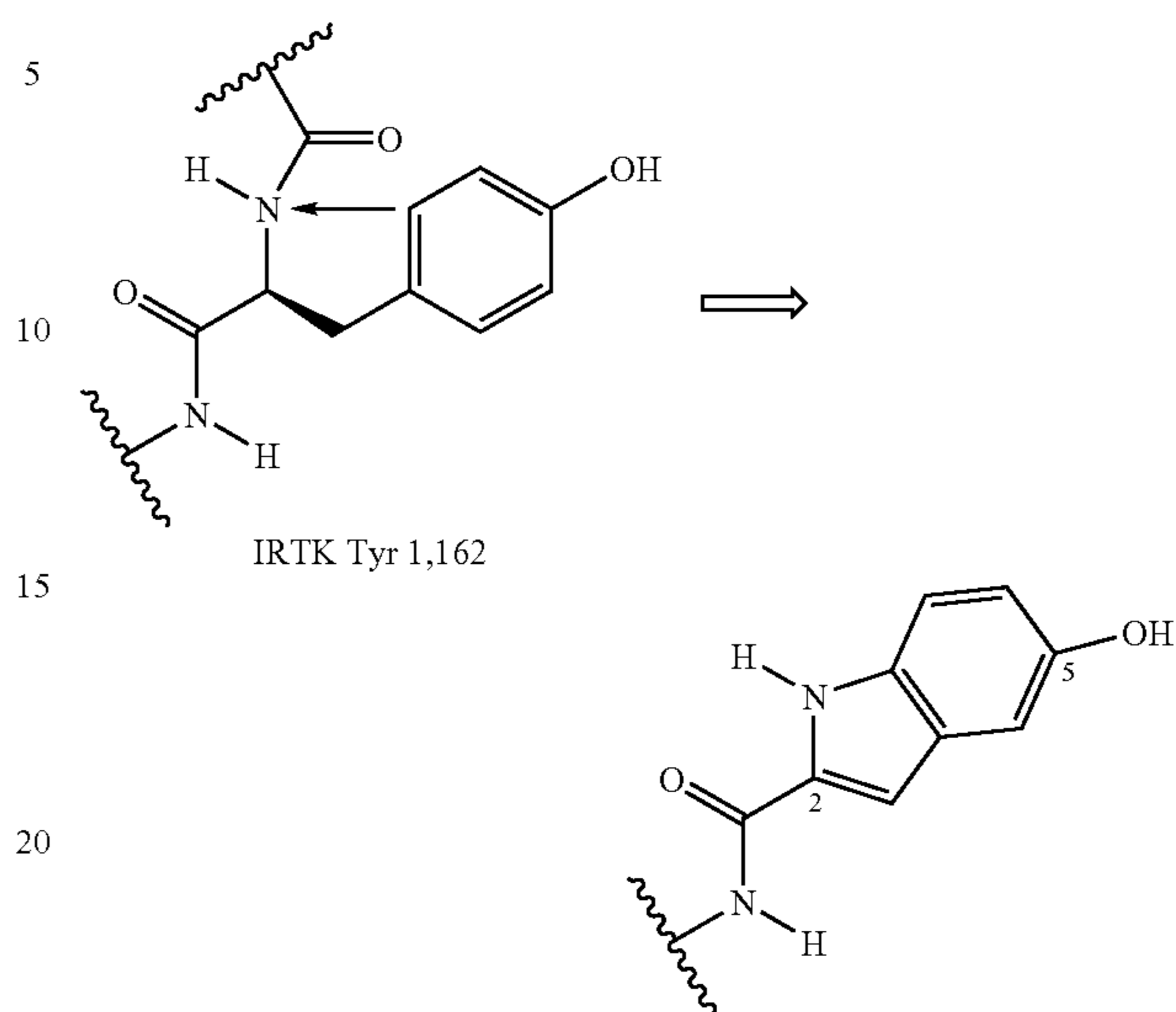
Scheme 1
