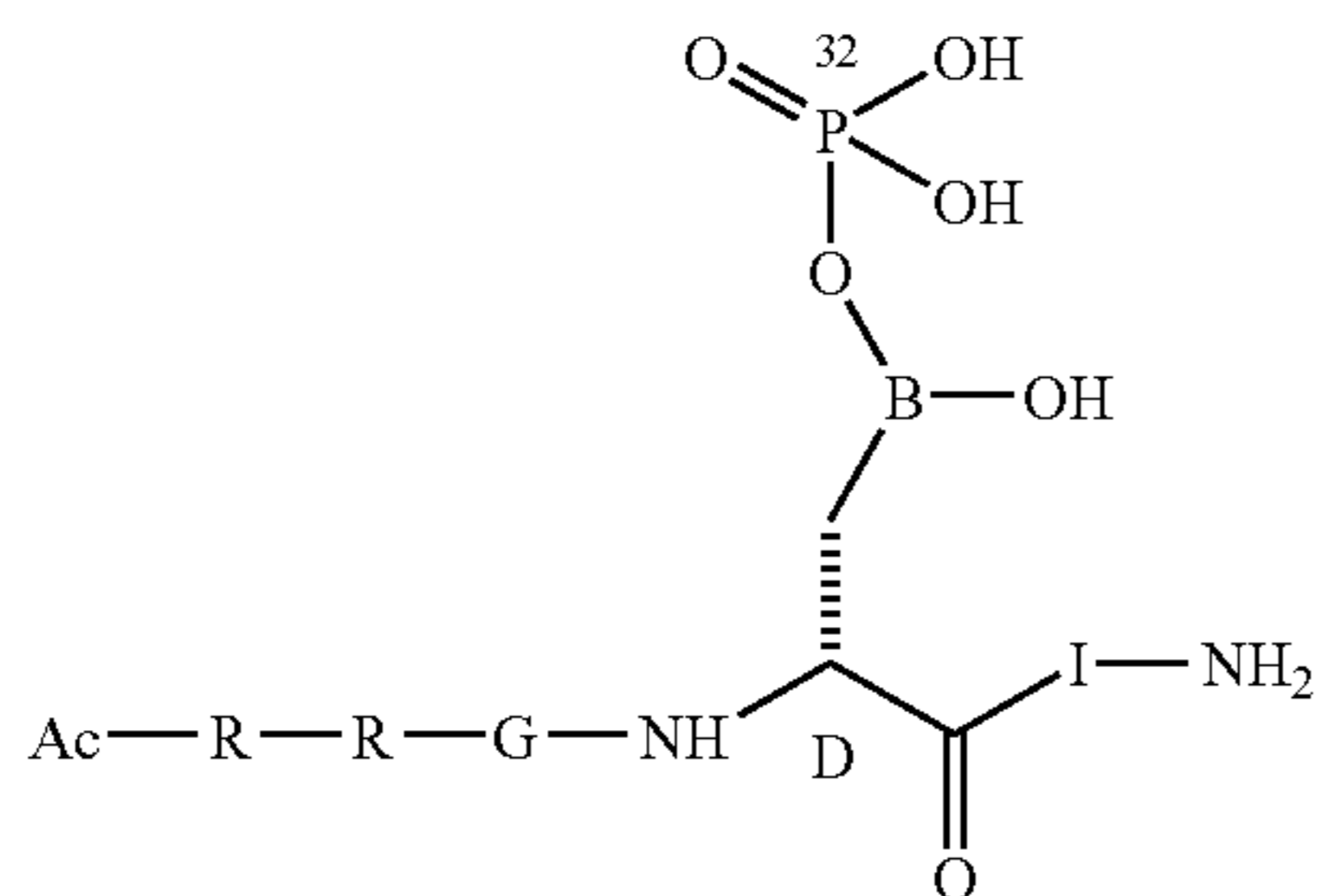
Phosphorylated 22
