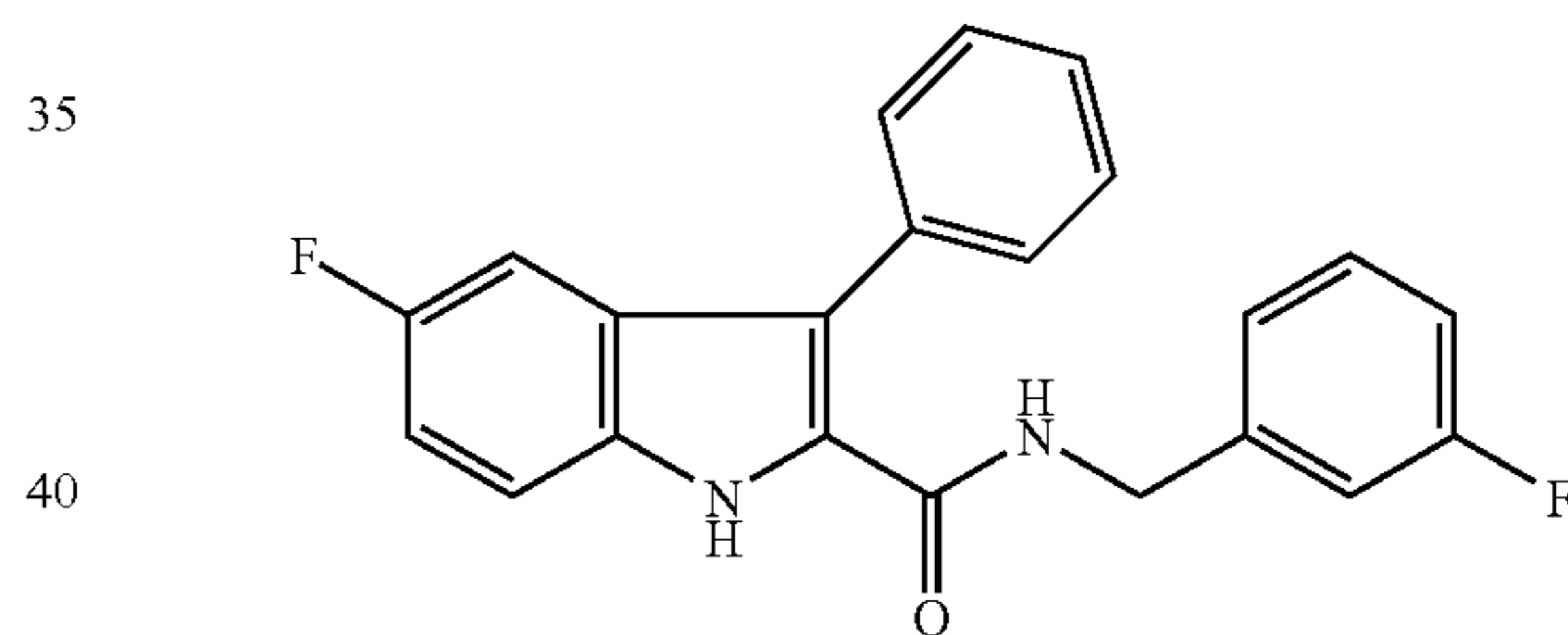
Compound 2g
