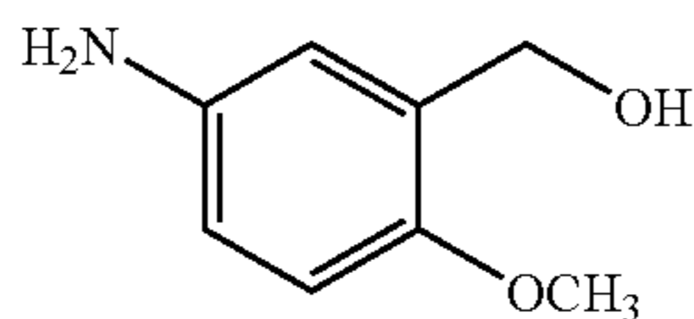
3-hydroxymethyl-4-methoxyaniline
