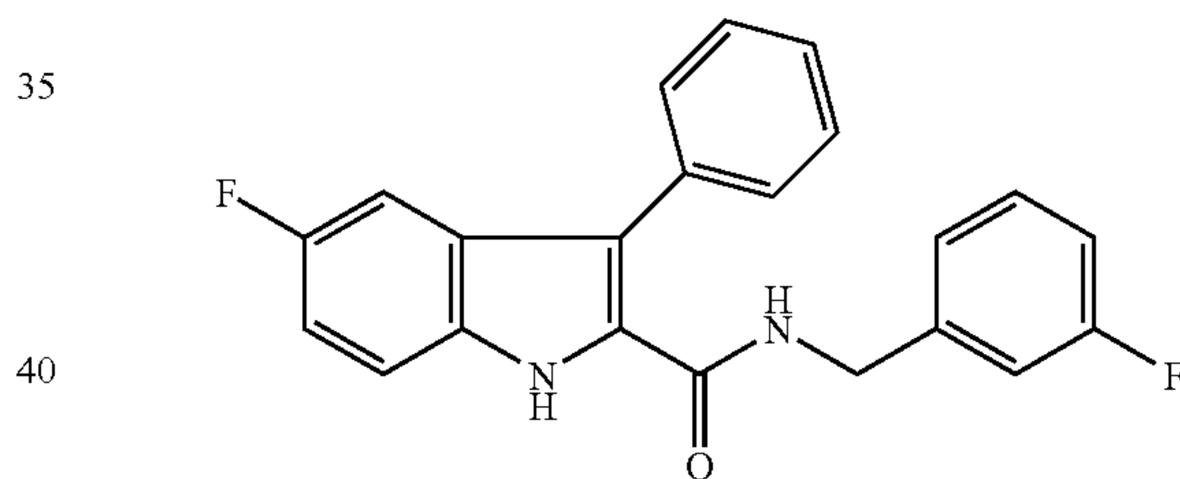
Compound 2g
