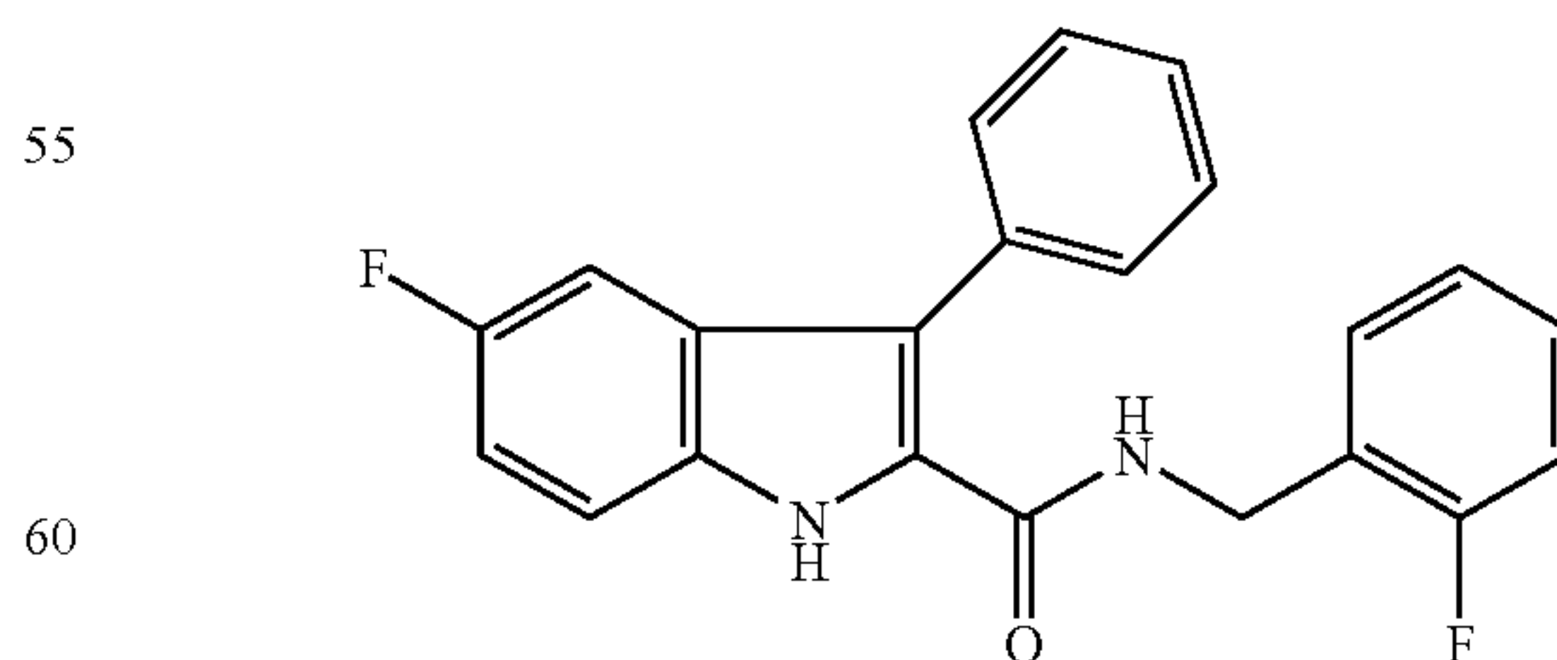
Compound 2s
