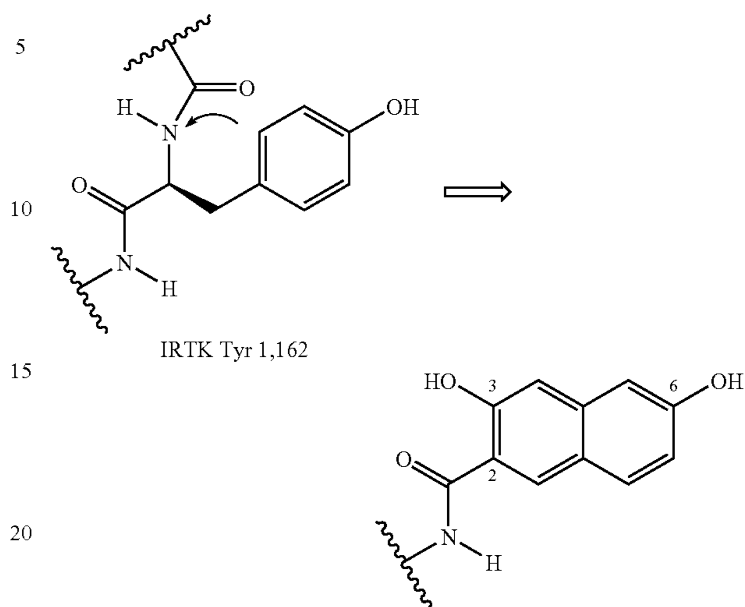
Scheme 1
