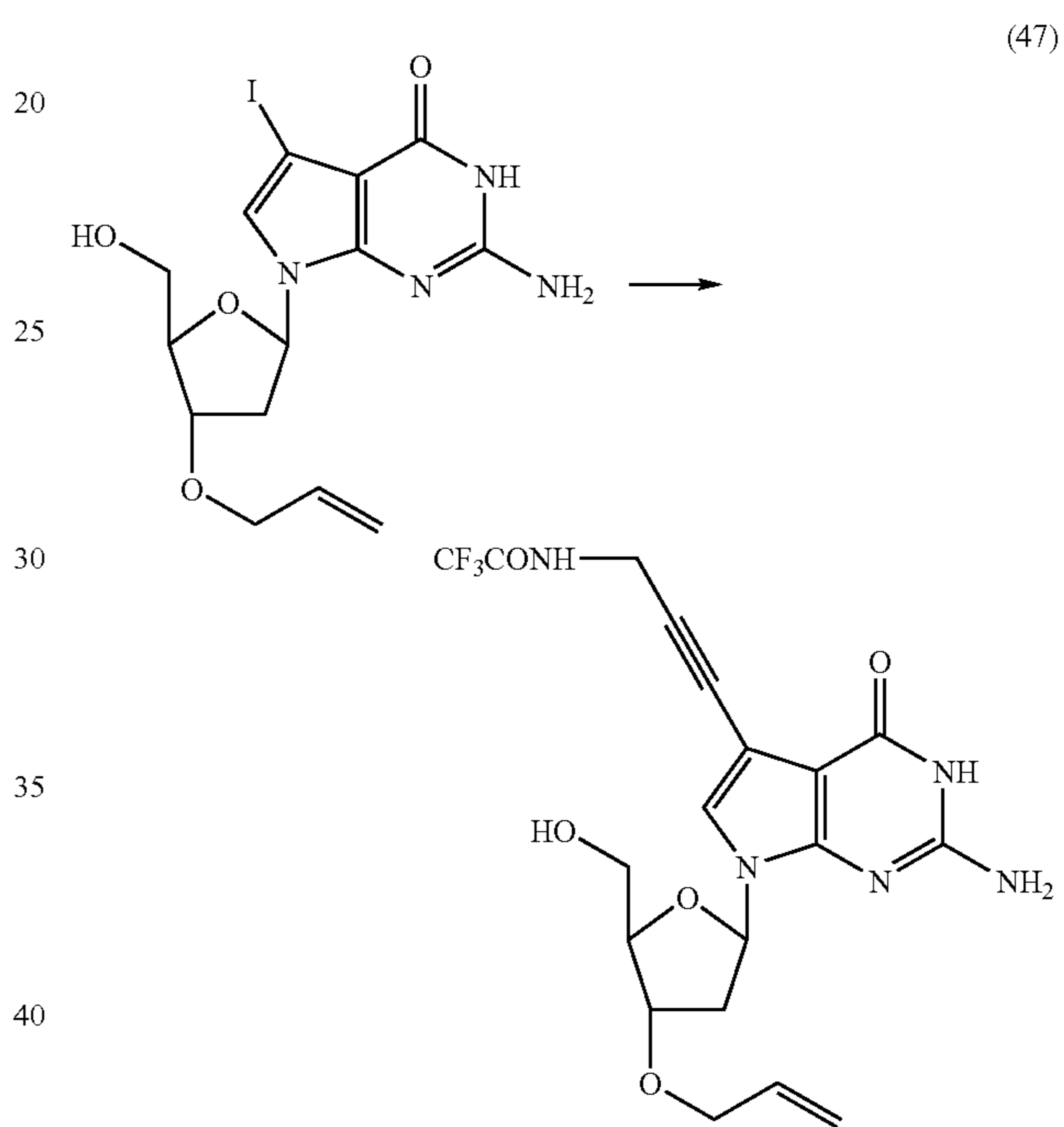
3'-O-Allyl-5'-O-(tert-butyltrimethylsilyl)-7-deaza-7-[3-(2,2,2-trifluoroacetamido)-prop-1-ynyl]-2'-deoxyguanosine (47)
