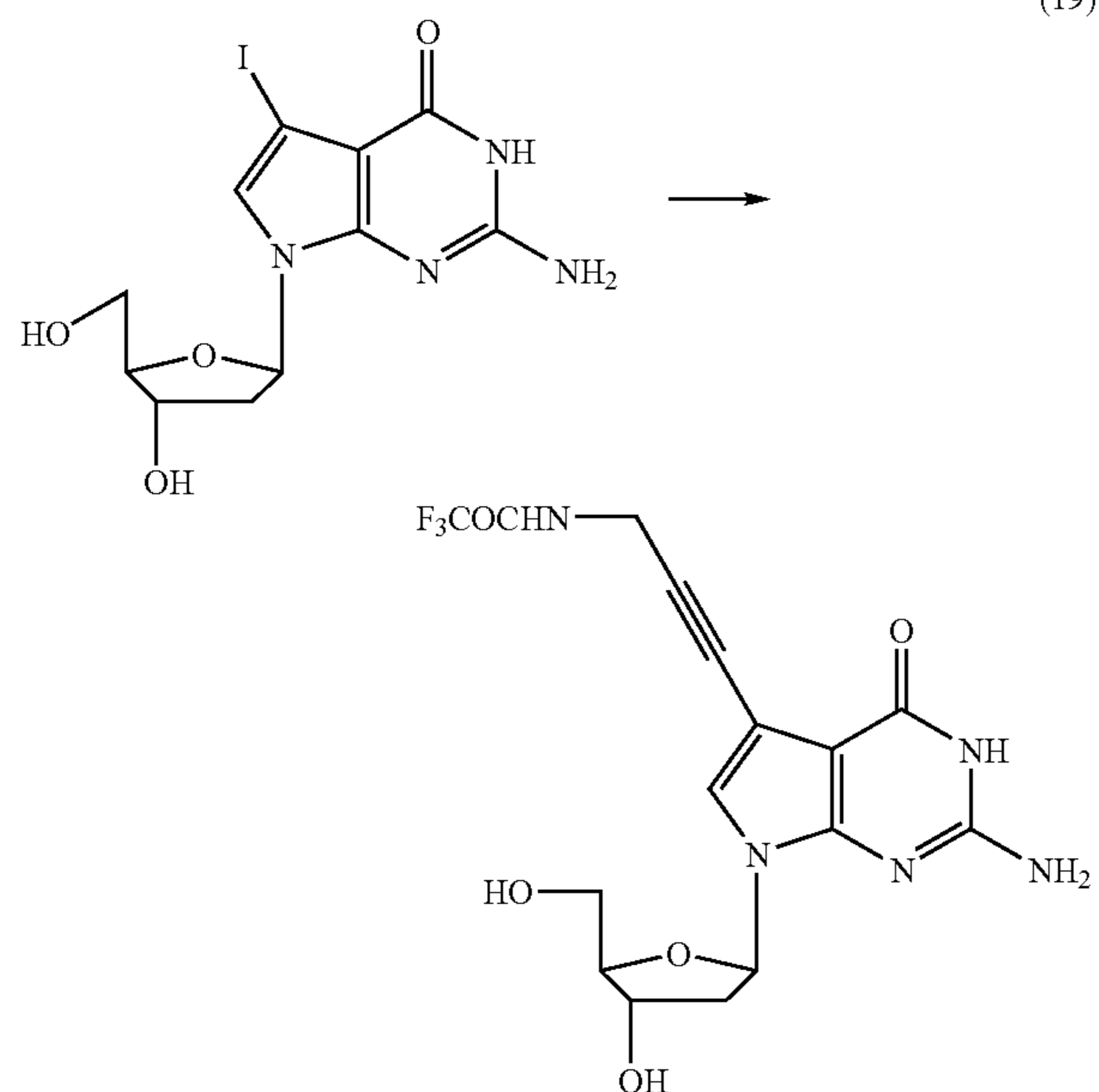
7-Deaza-[3-(2,2,2-trifluoroacetamido)-prop-1-ynyl]- 2'-deoxyguanosine (19)
