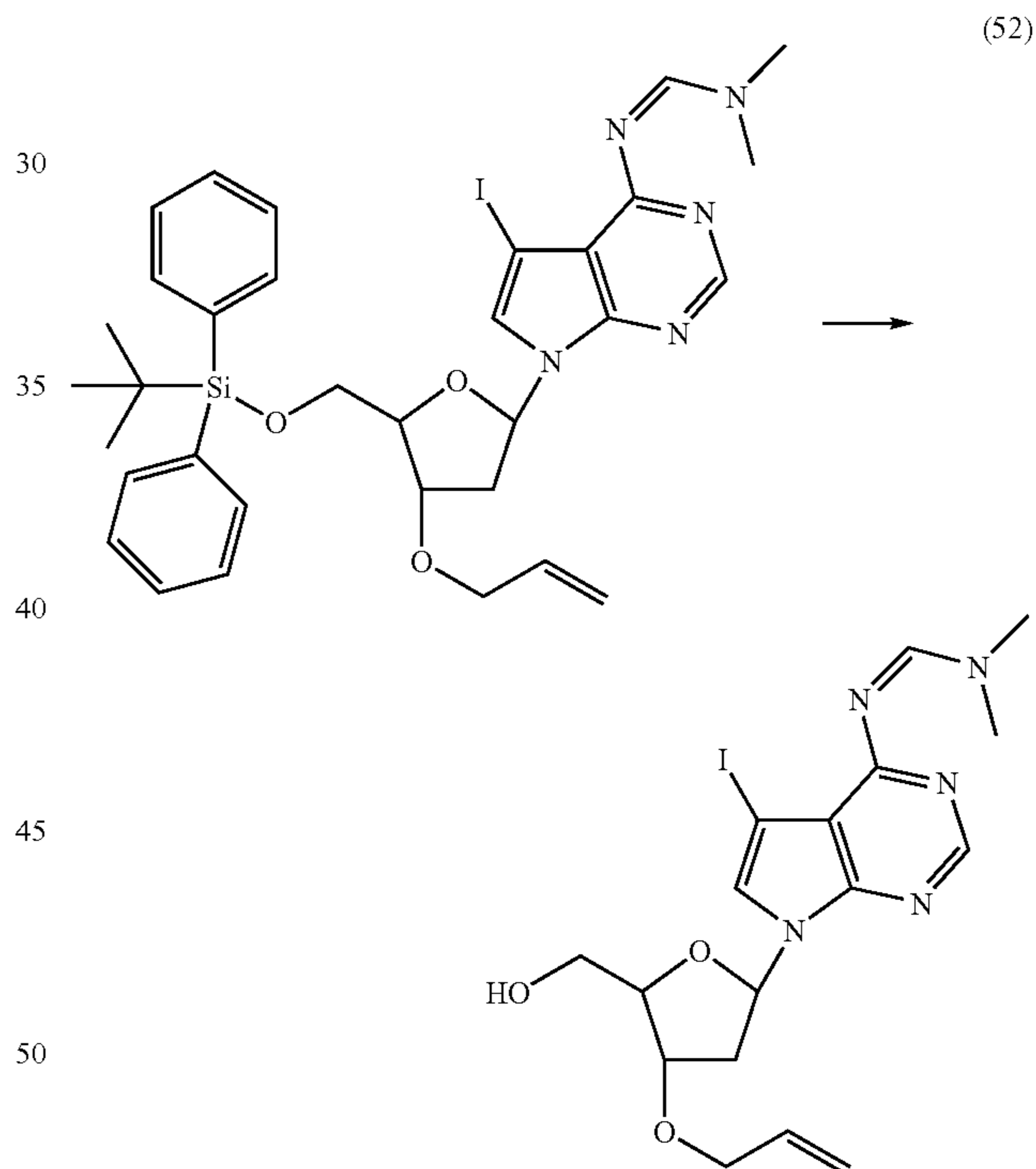
3'-O-Allyl-7-deaza-6-N,N-dimethylformadine-7-iodo-2'-deoxyadenosine (52)
