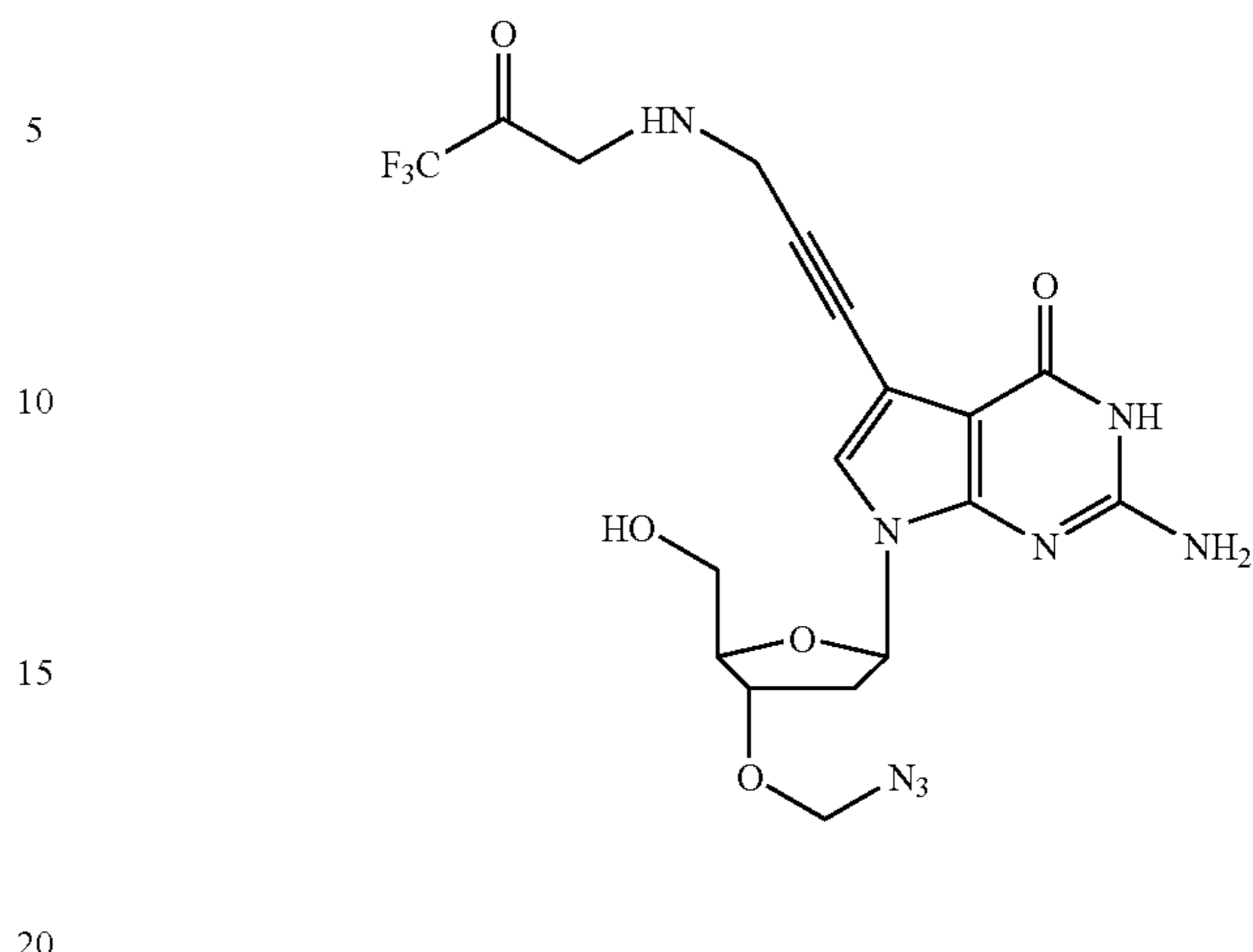
3'-O-Azidomethyl-7-deaza-7-[3-(2,2,2-trifluoroacetamido)-prop-1-ynyl]-2'-deoxyguanosine (22)
