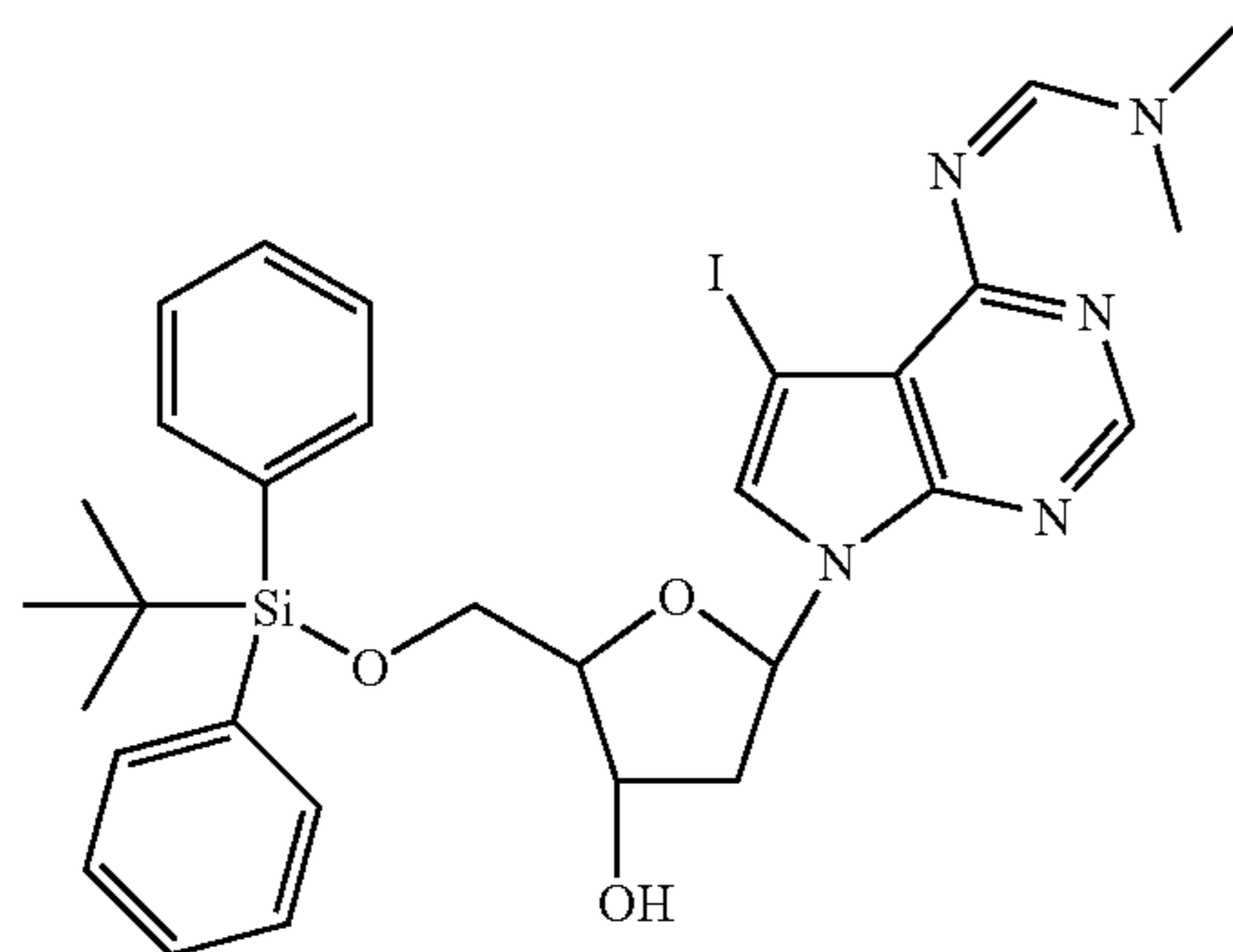
7-Deaza-6-N,N-dimethylformadine-5'-O-diphenylsilyl-7-iodo-2'-deoxyadenosine (50)
