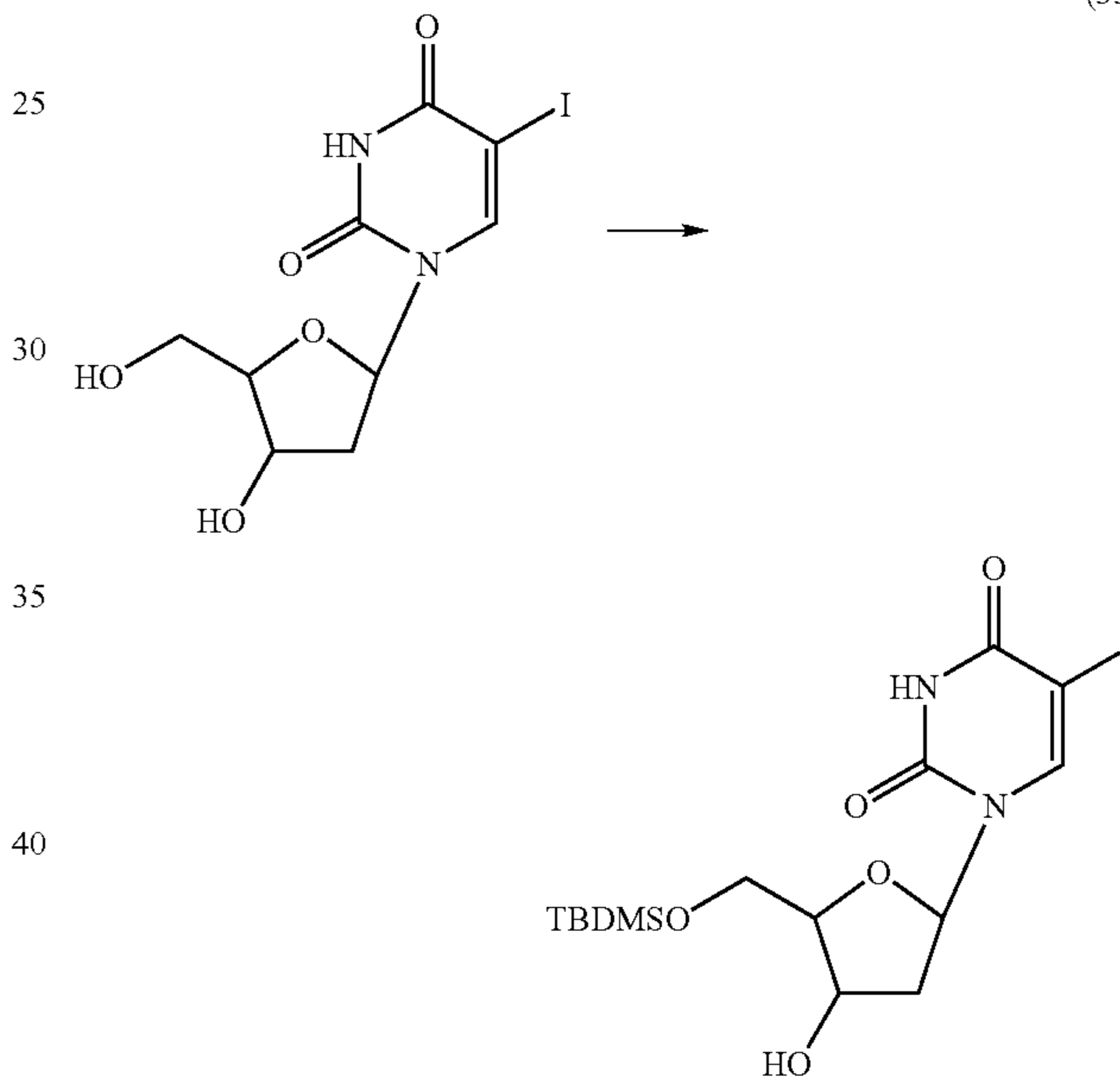
5'-O-(t-Butyldimethylsilyl)-5-iodo-2'-deoxyuridine (33)
