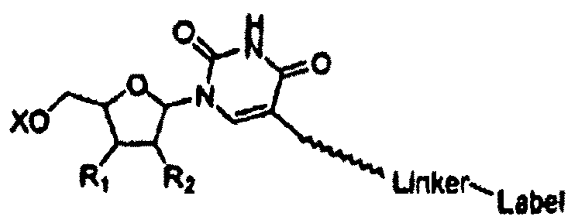
Uridine C5-linker
