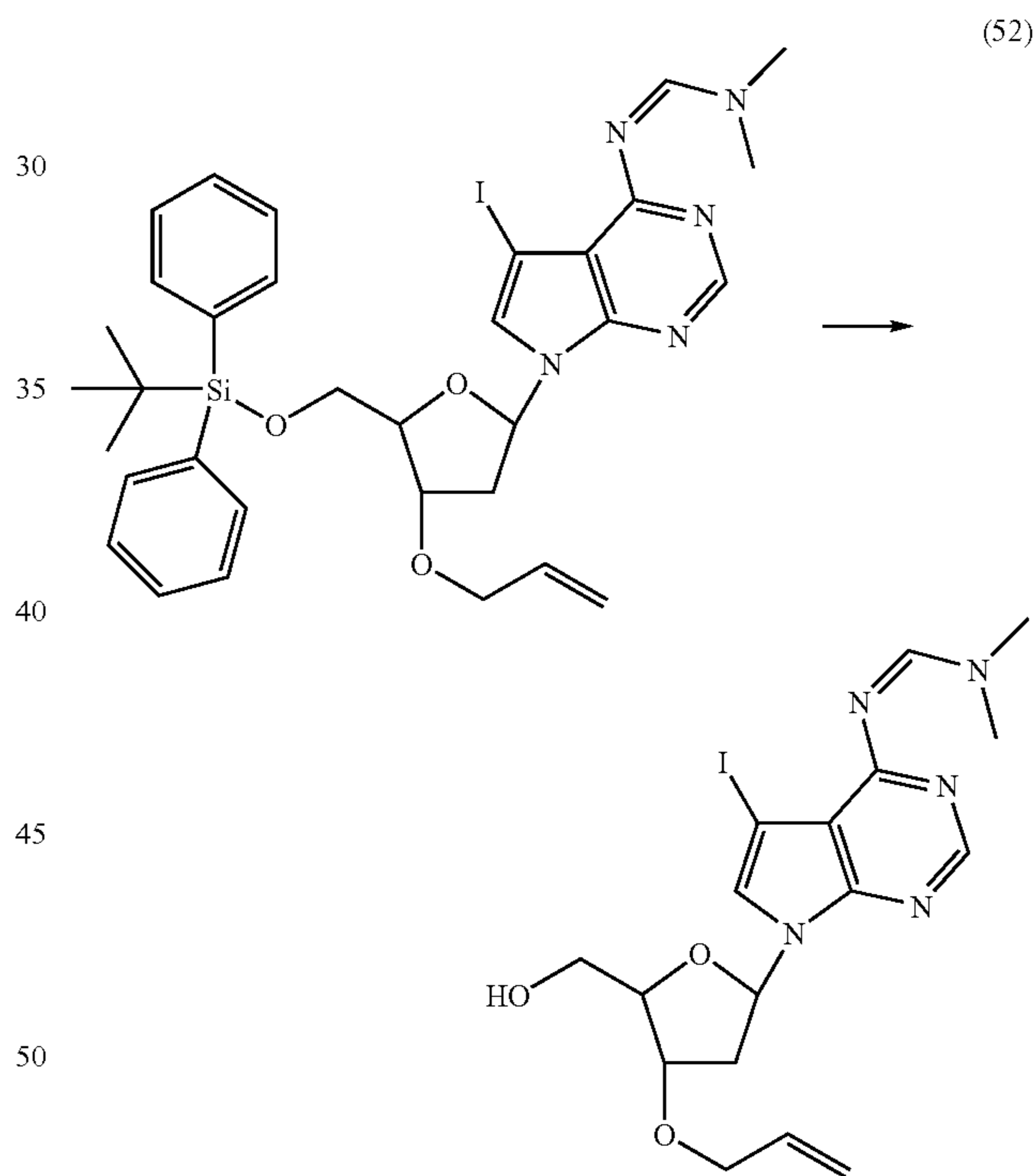
3'-O-Allyl-7-deaza-6-N,N-dimethylformadine-7-iodo-2'-deoxyadenosine (52)
