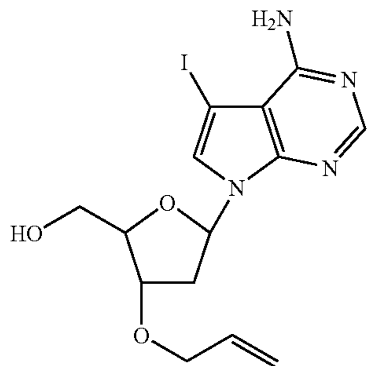
3'-O-Allyl-7-deaza-7-iodo-2'-deoxyadenosine (53)
