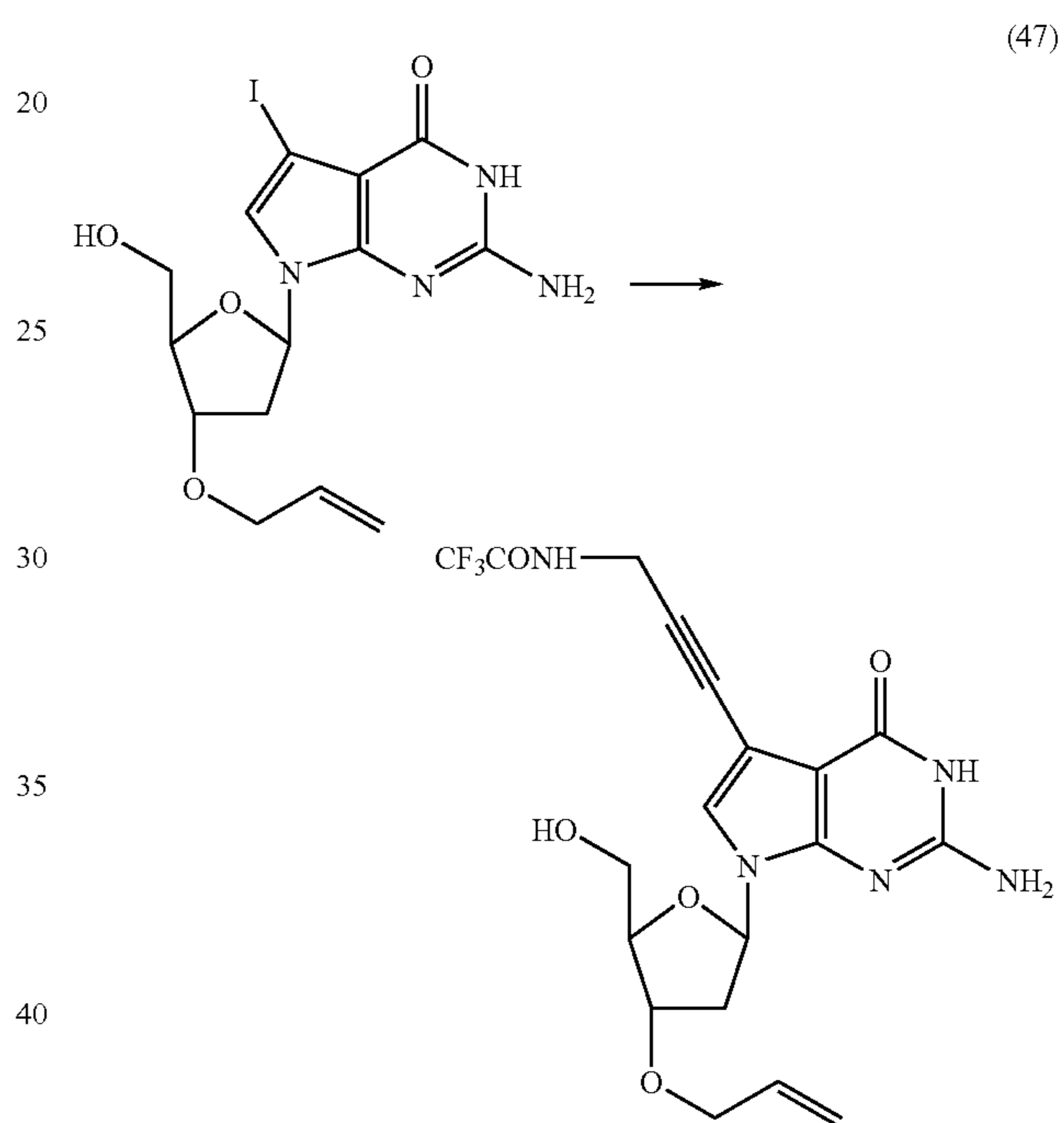
3'-O-Allyl-5'-O-(tert-butyltrimethylsilyl)-7-deaza-7-[3-(2,2,2-trifluoroacetamido)-prop-1-ynyl]-2'-deoxyguanosine (47)
