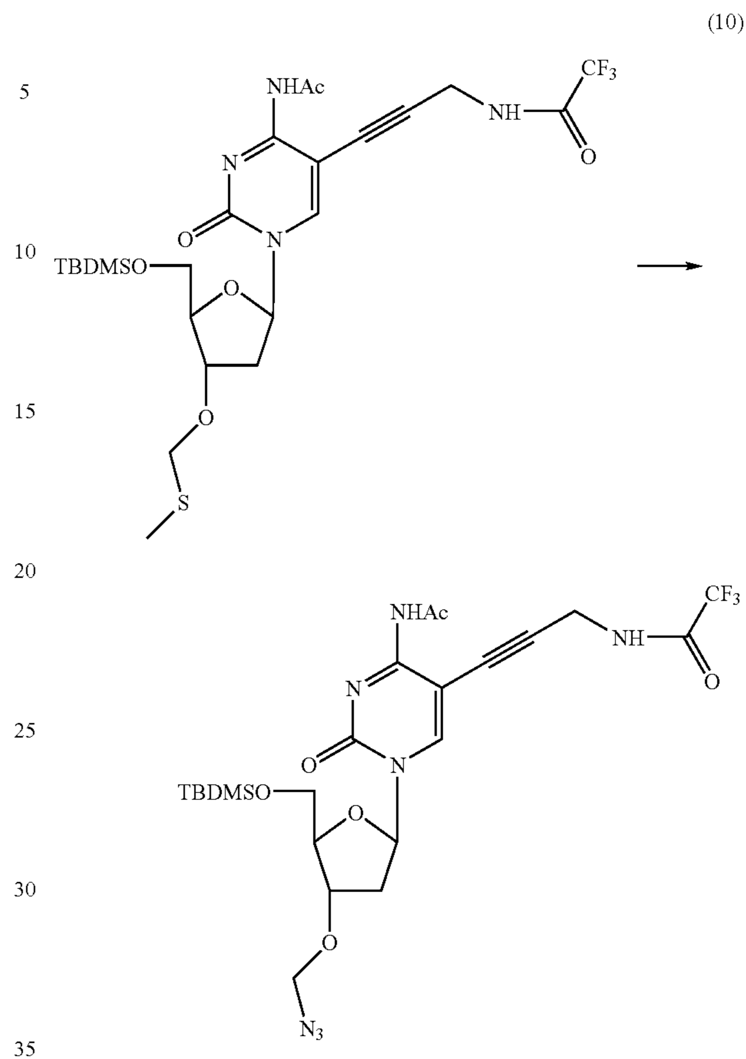
4-N-Acetyl-3'-O-(azidomethyl)-5'-O-(tert-butyldimethylsilyl)-5-[3-(2,2,2-trifluoroacetamide)-prop-1-ynyl]-2'-deoxycytidine (10)
