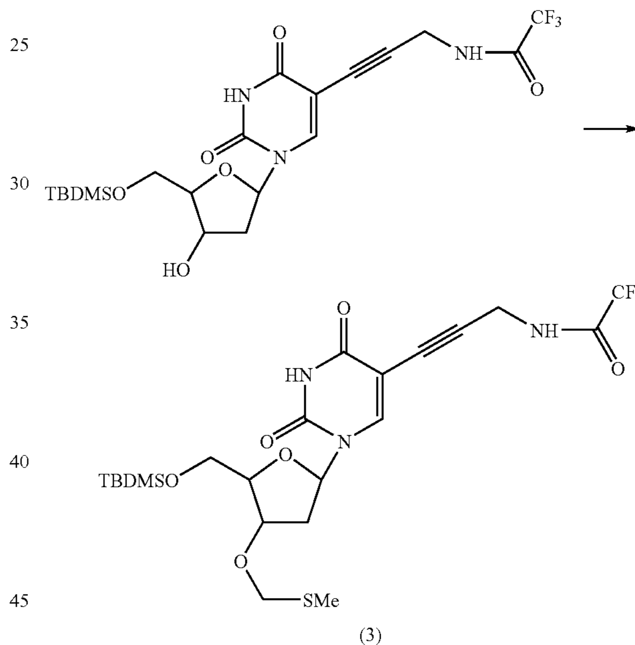
5'-O-(tert-butyl dimethylsilyl)-3'-O-methylthiomethyl-5-[3-(2,2,2-trifluoroacetamido)-prop-1-ynyl]-2'-deoxyuridine (3)
