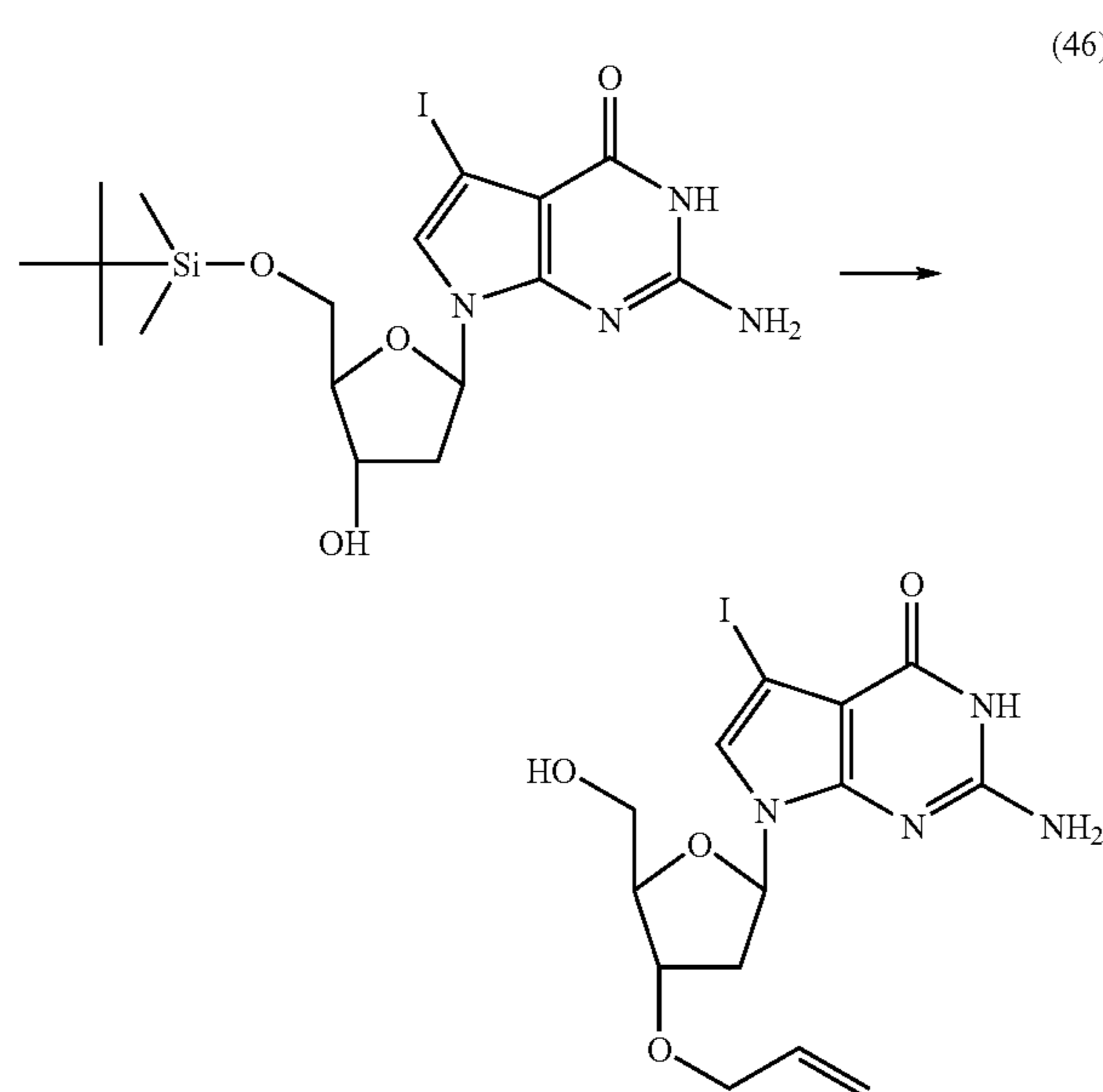
3'-O-Allyl-5'-O-(tert-butyltrimethylsilyl)-7-deaza-7-iodo-2'-deoxyguanosine (46)
