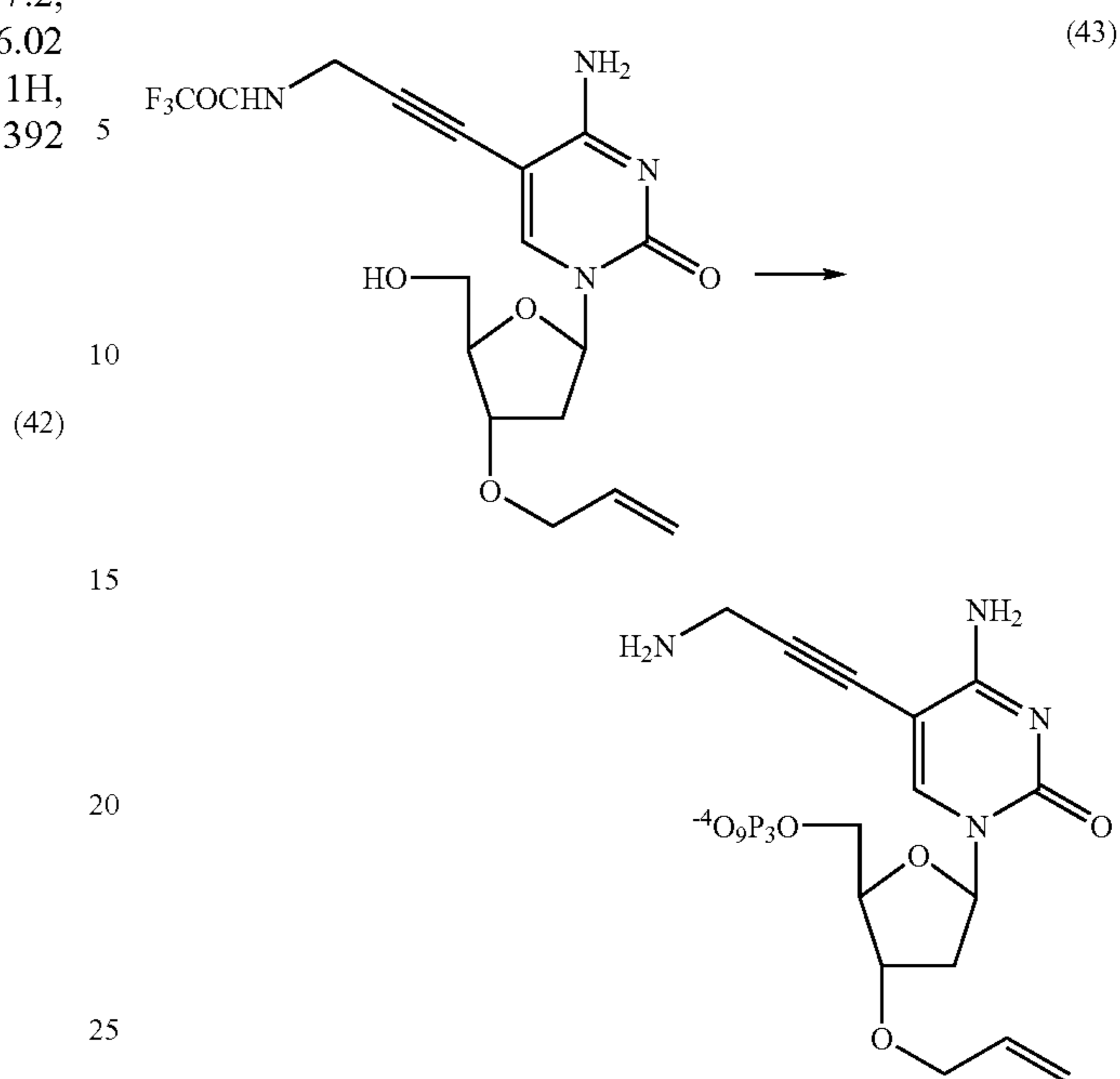
3'-O-Allyl-5-(3-amino-prop-1-ynyl)-5'-O-triphosphate-2'-deoxycytidine (43)
