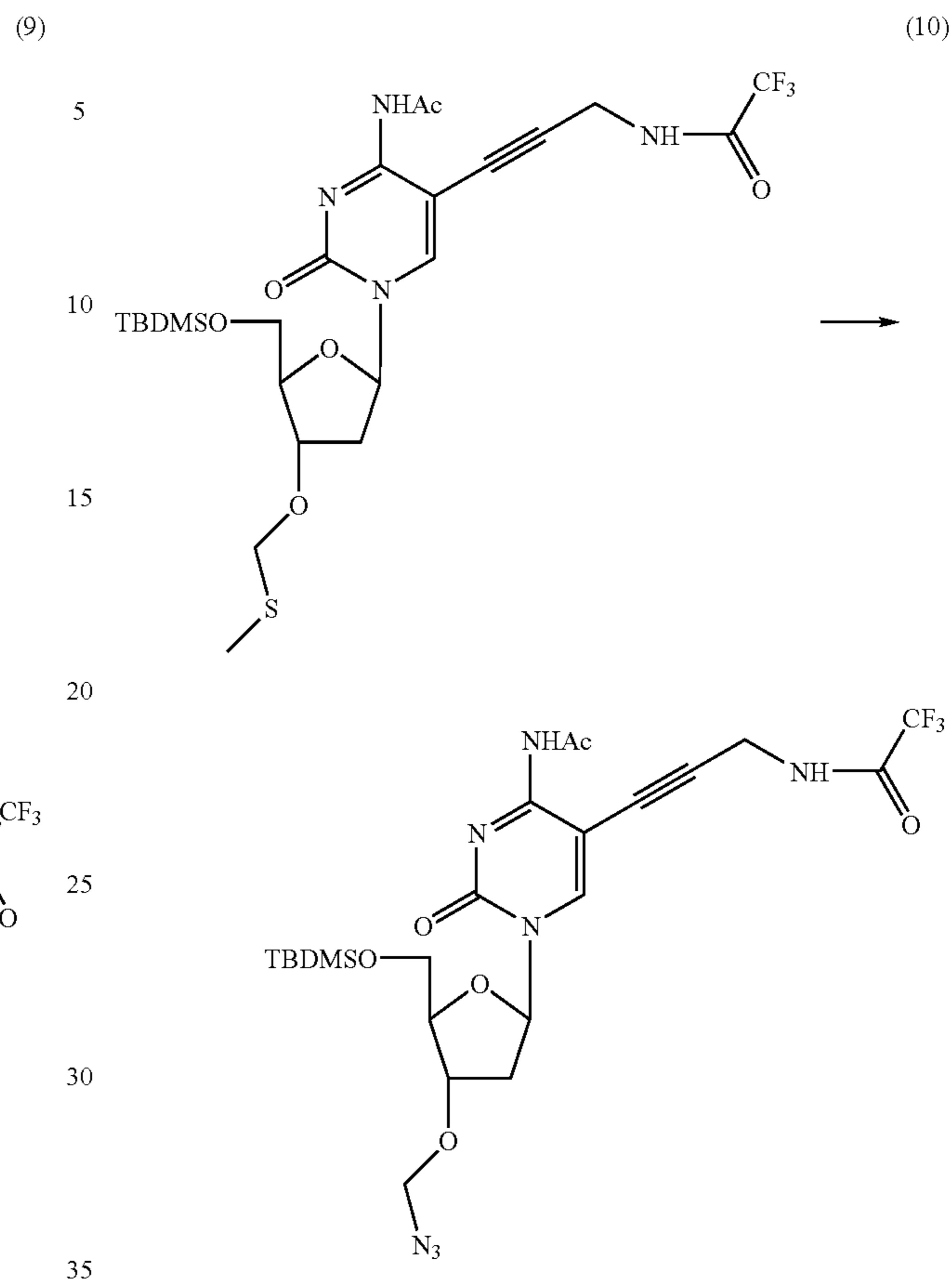
4-N-Acetyl-3'-O-(azidomethyl)-5'-O-(tert-butyldimethylsilyl)-5-[3-(2,2,2-trifluoroacetamide)-prop-1-ynyl]-2'-deoxycytidine (10)
