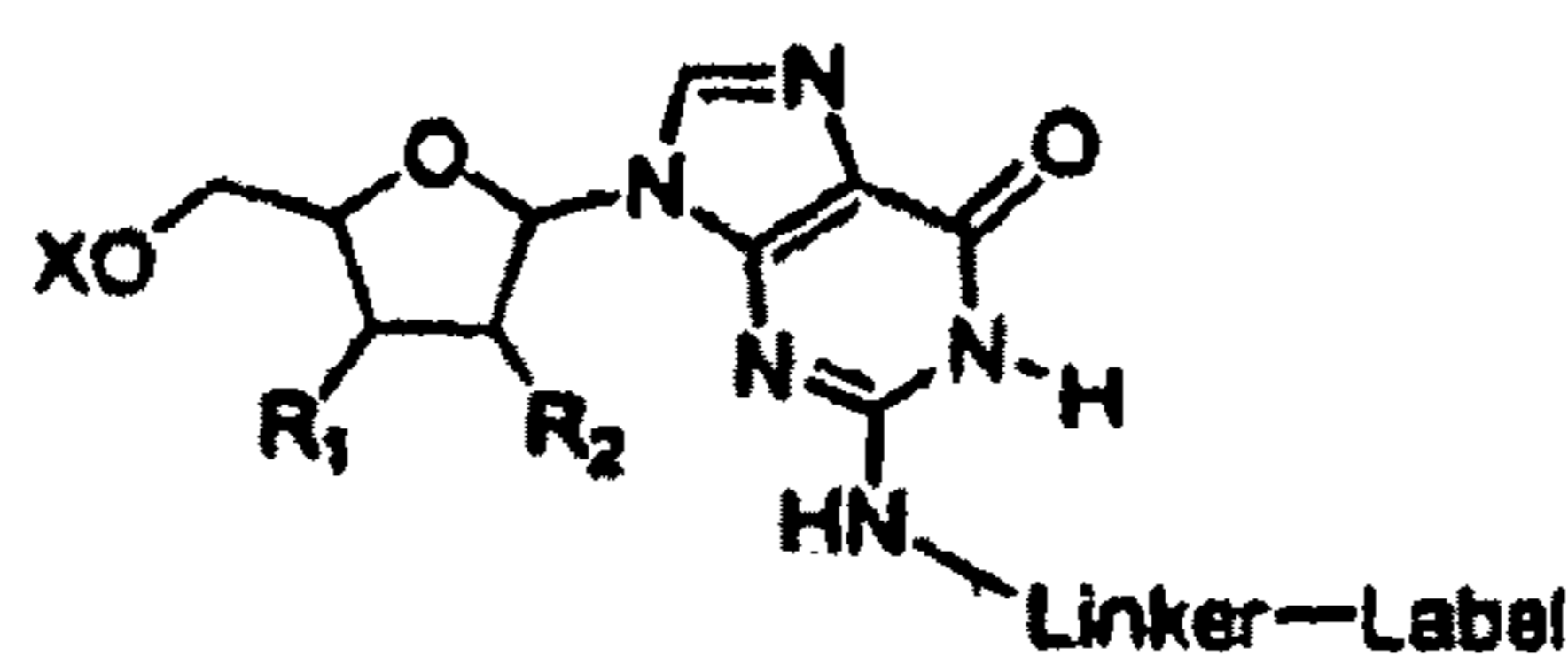
Guanosine N2-linker
