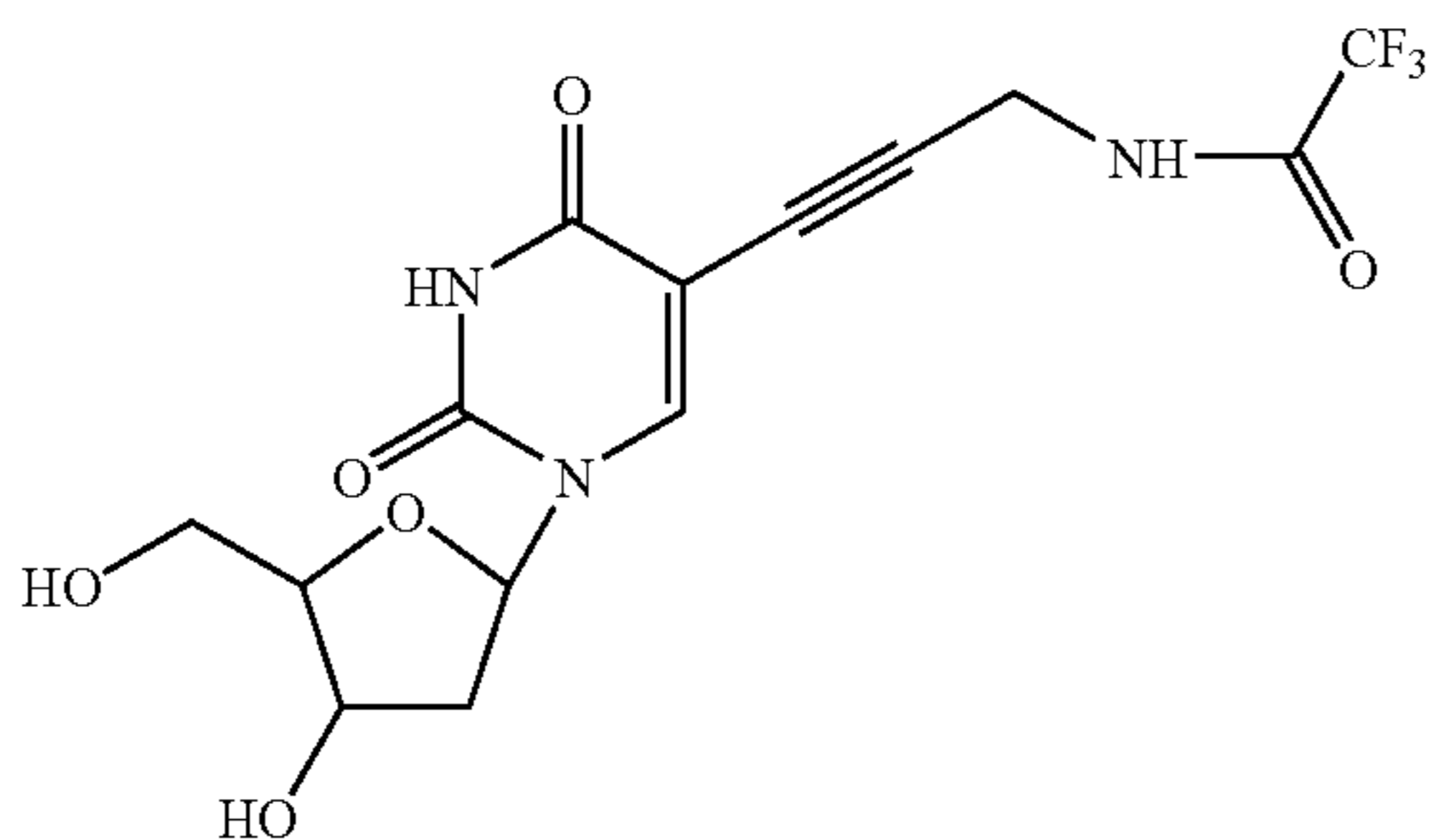
5-[3-(2,2,2-trifluoroacetamido)-prop-1-ynyl]-2'-deoxyuridine (1)
