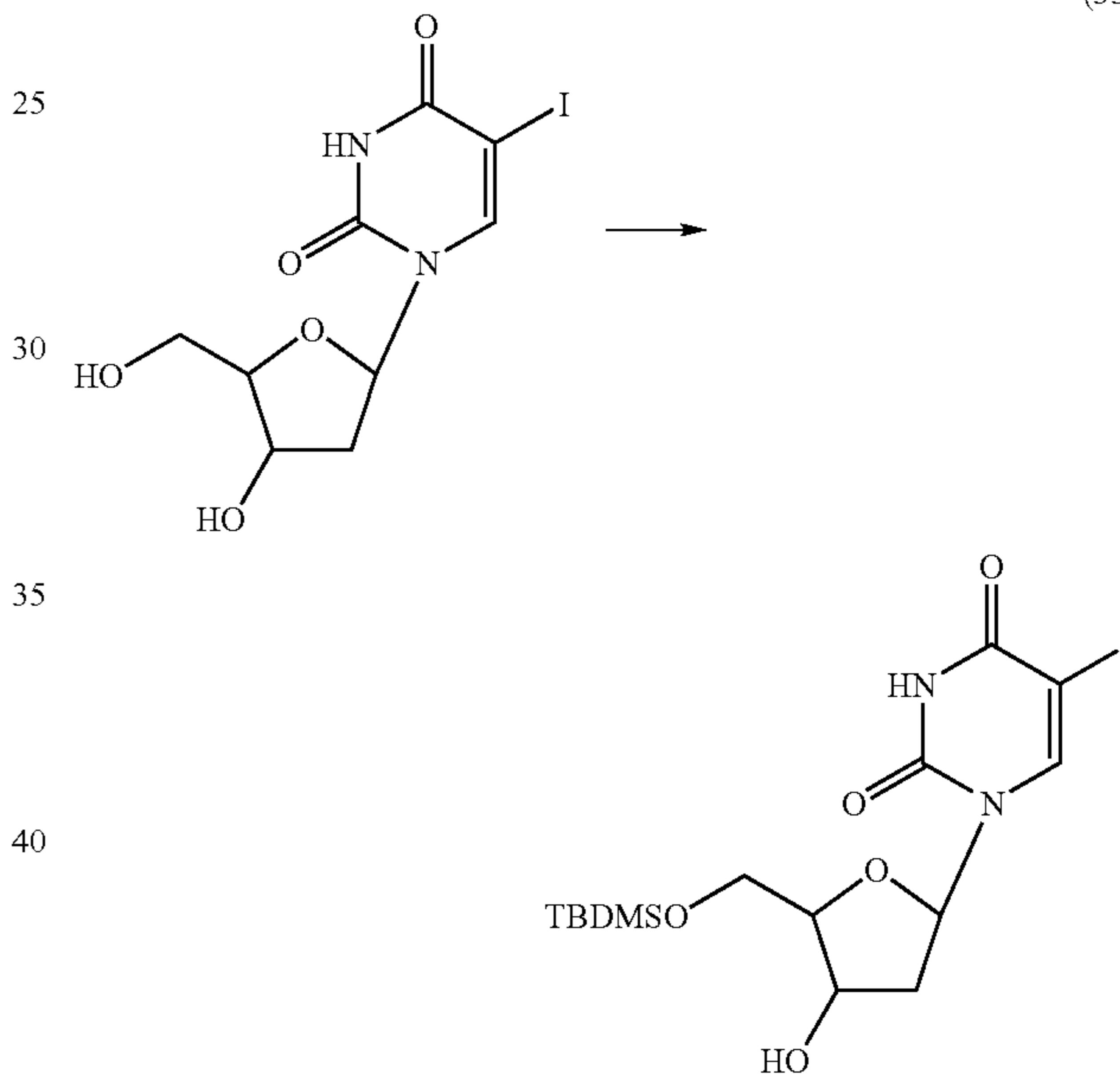
25 5'-O-(t-Butyldimethylsilyl)-5-iodo-2'-deoxyuridine 30 (33)
