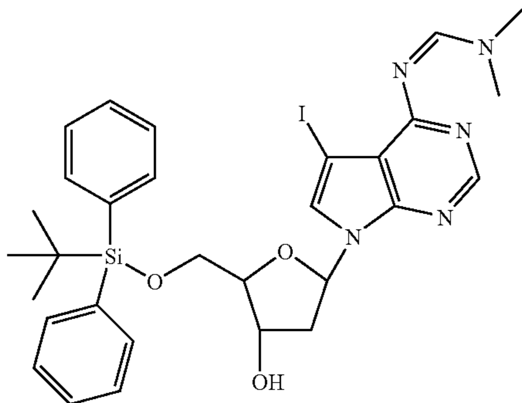
7-Deaza-6-N,N-dimethylformadine-5'-O-diphenylsilyl-7-iodo-2'-deoxyadenosine (50)
