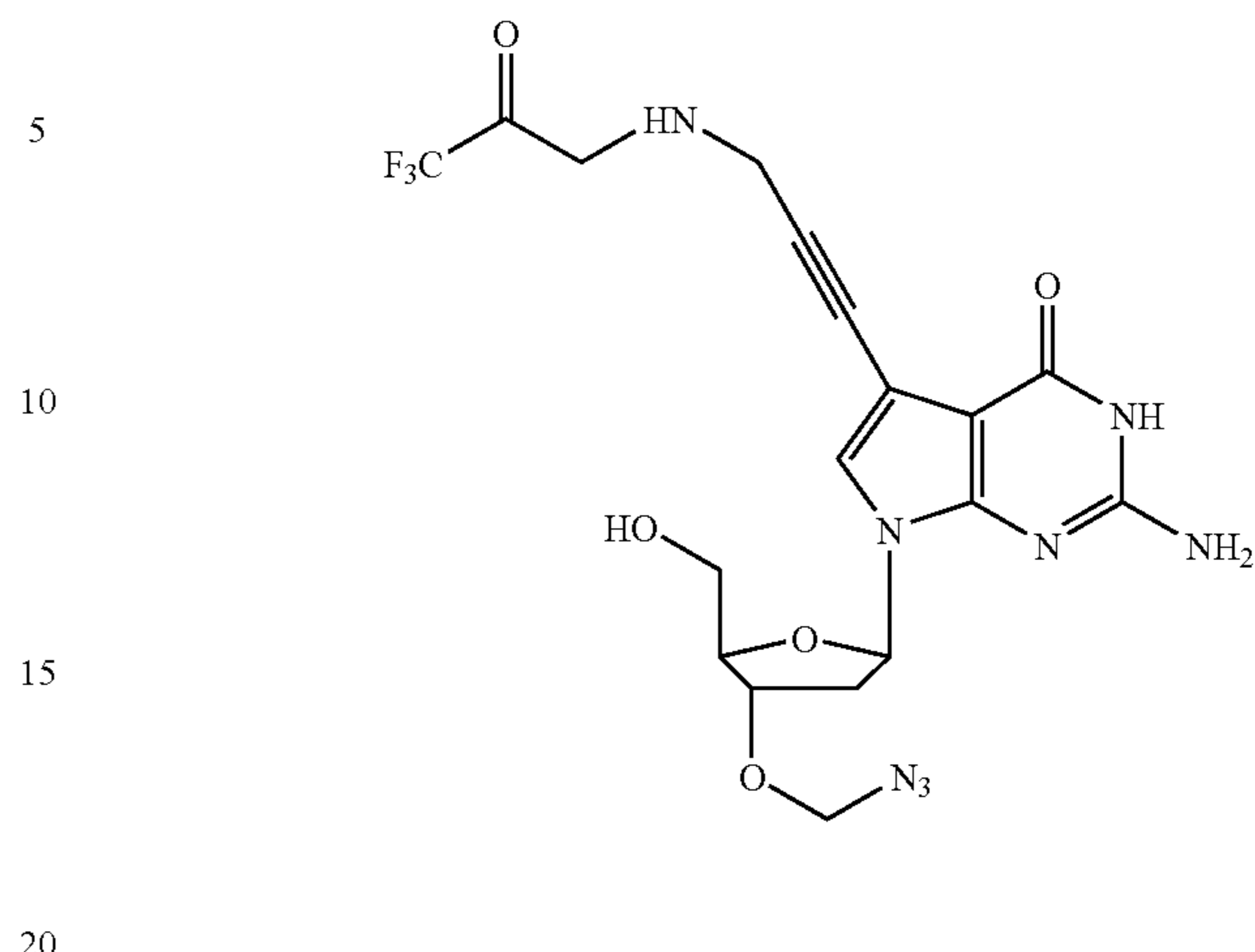
3'-O-Azidomethyl-7-deaza-7-[3-(2,2,2-trifluoroacetamido)-prop-1-ynyl]-2'-deoxyguanosine (22)
