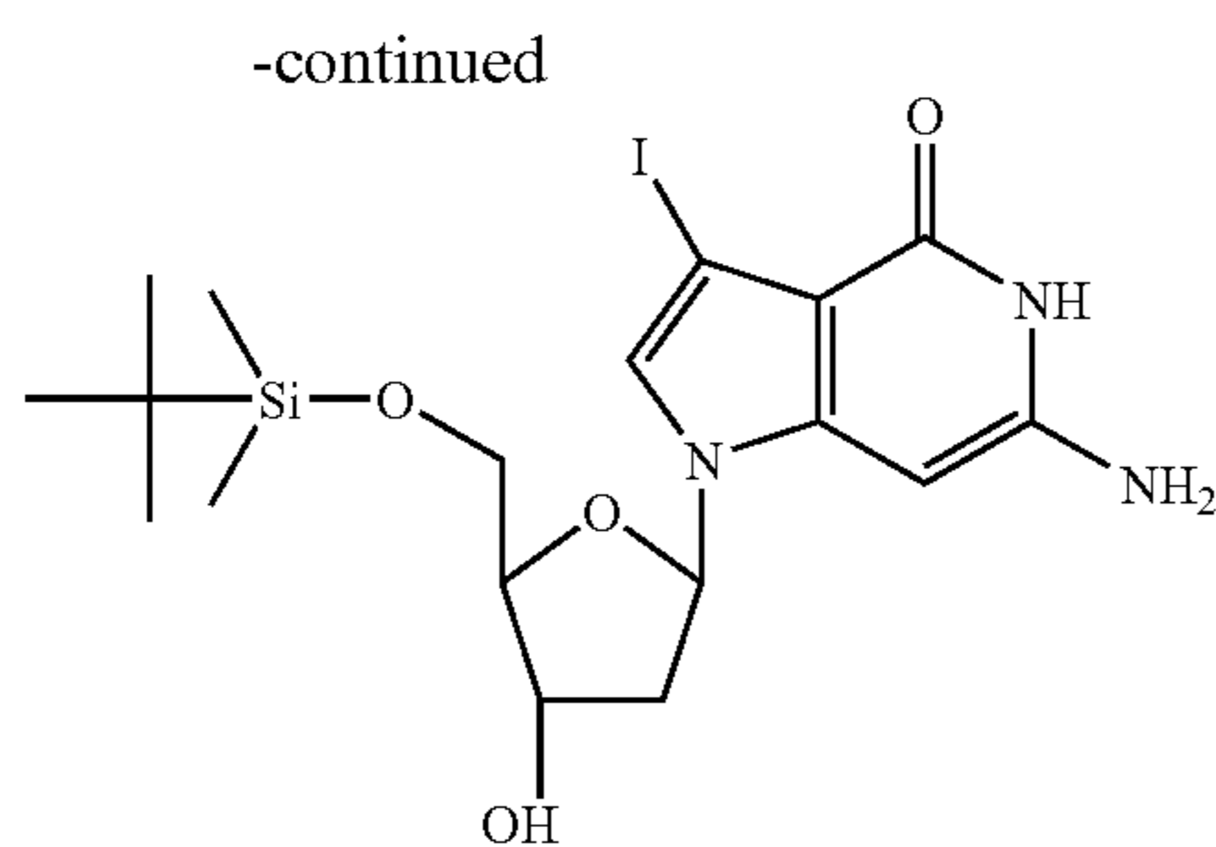
5'-O-(tert-Butyldimethylsilyl)-7-deaza-7-iodo-2'-deoxyguanosine (45)
