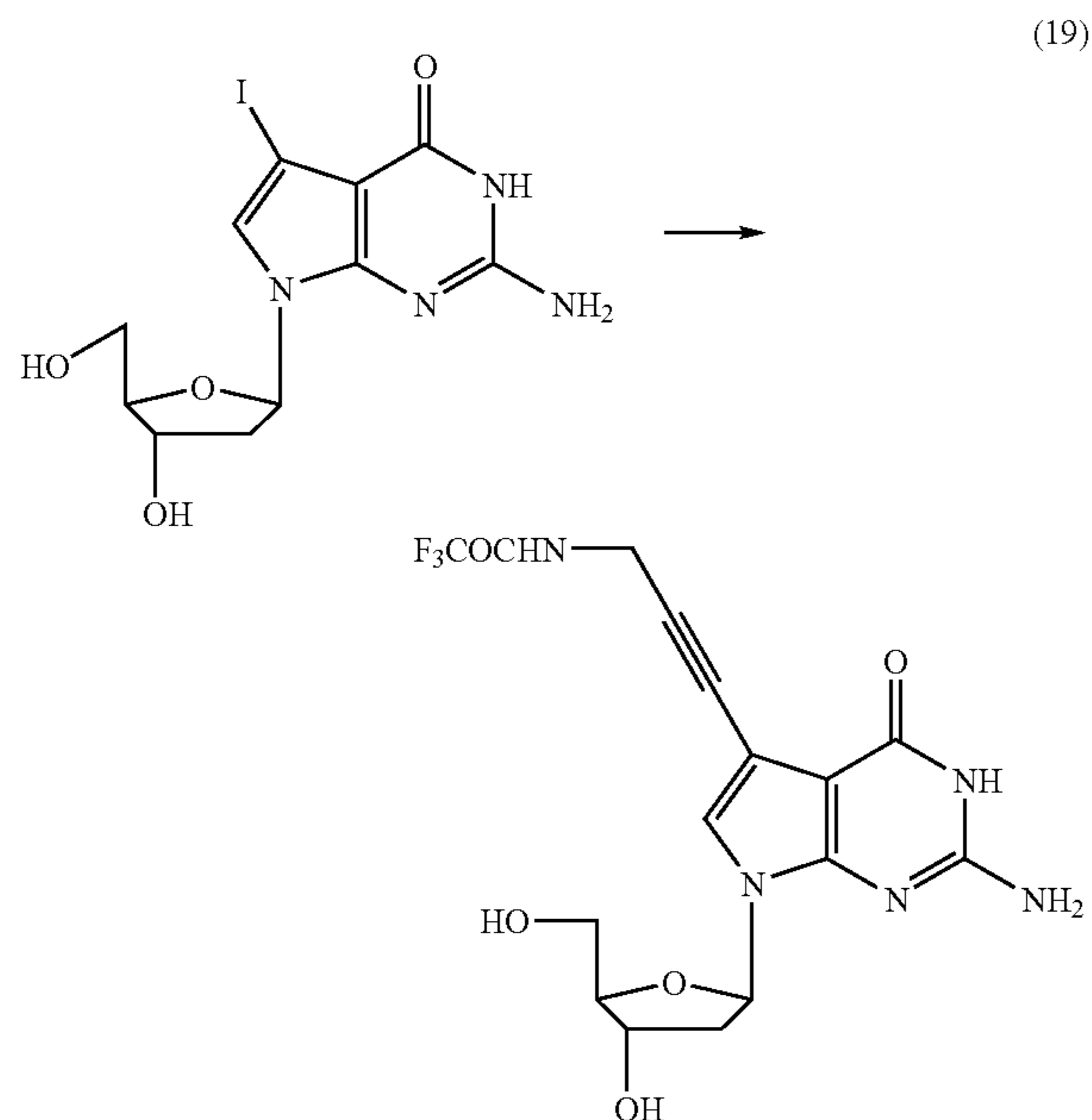
7-Deaza-[3-(2,2,2-trifluoroacetamido)-prop-1-ynyl]- 2'-deoxyguanosine (19)
