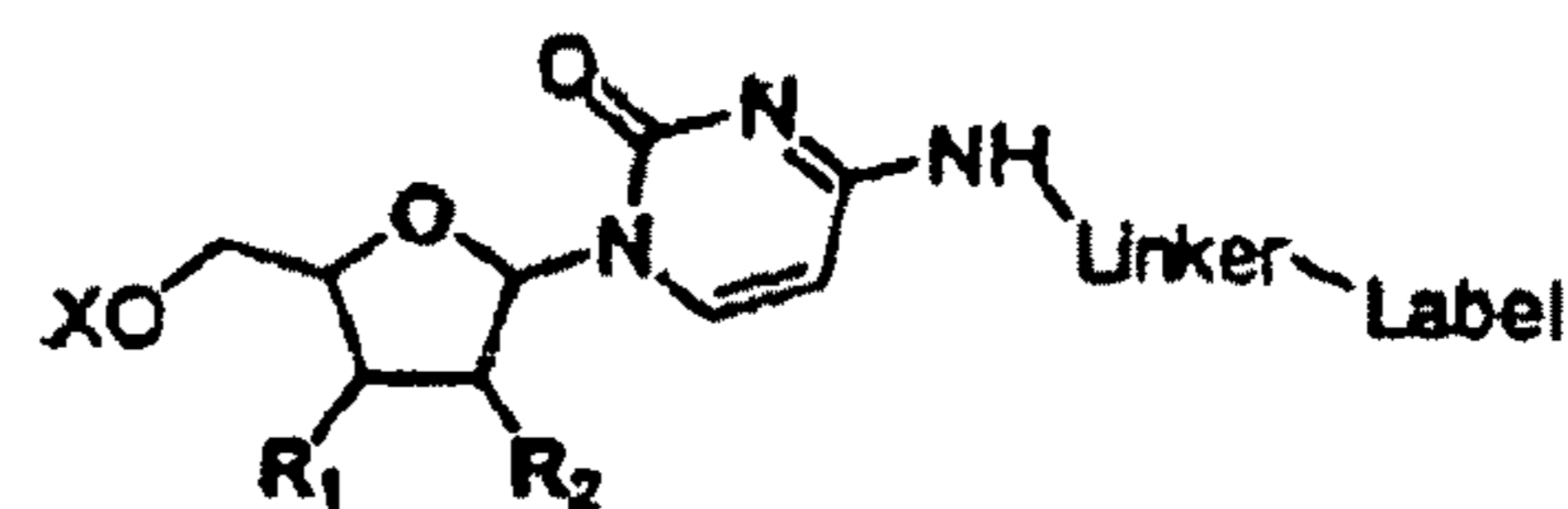
Cytidine N4-linker
