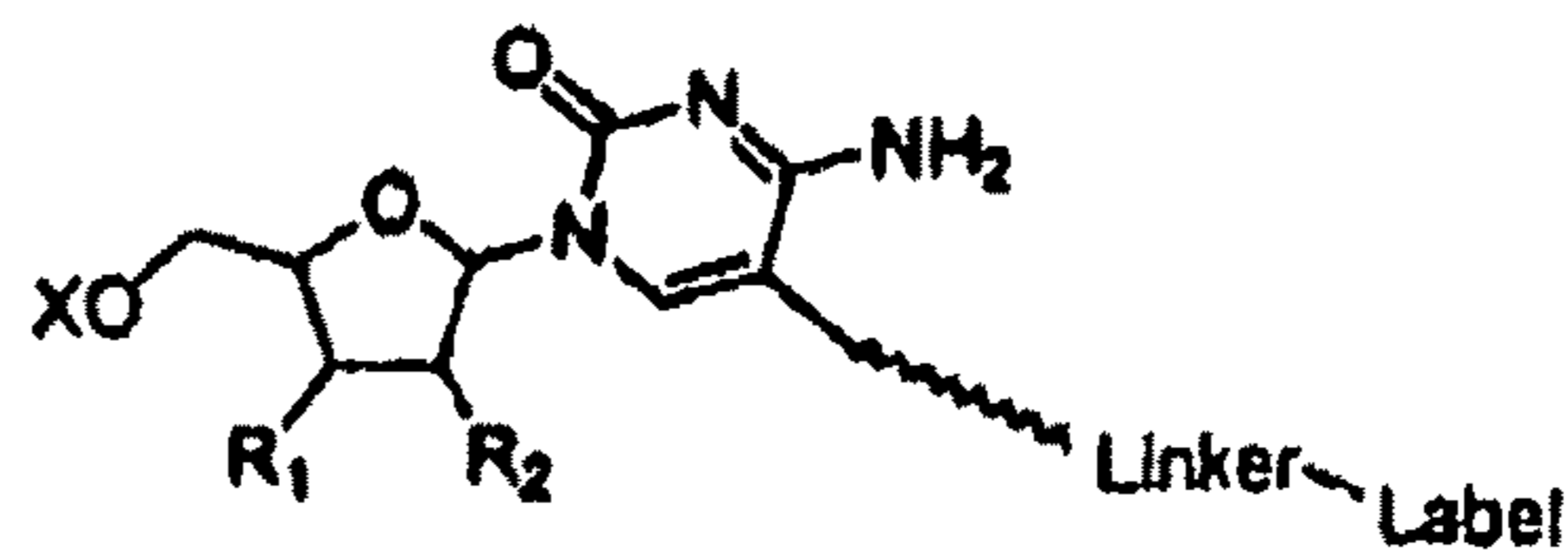
Cytidine C5-linker
