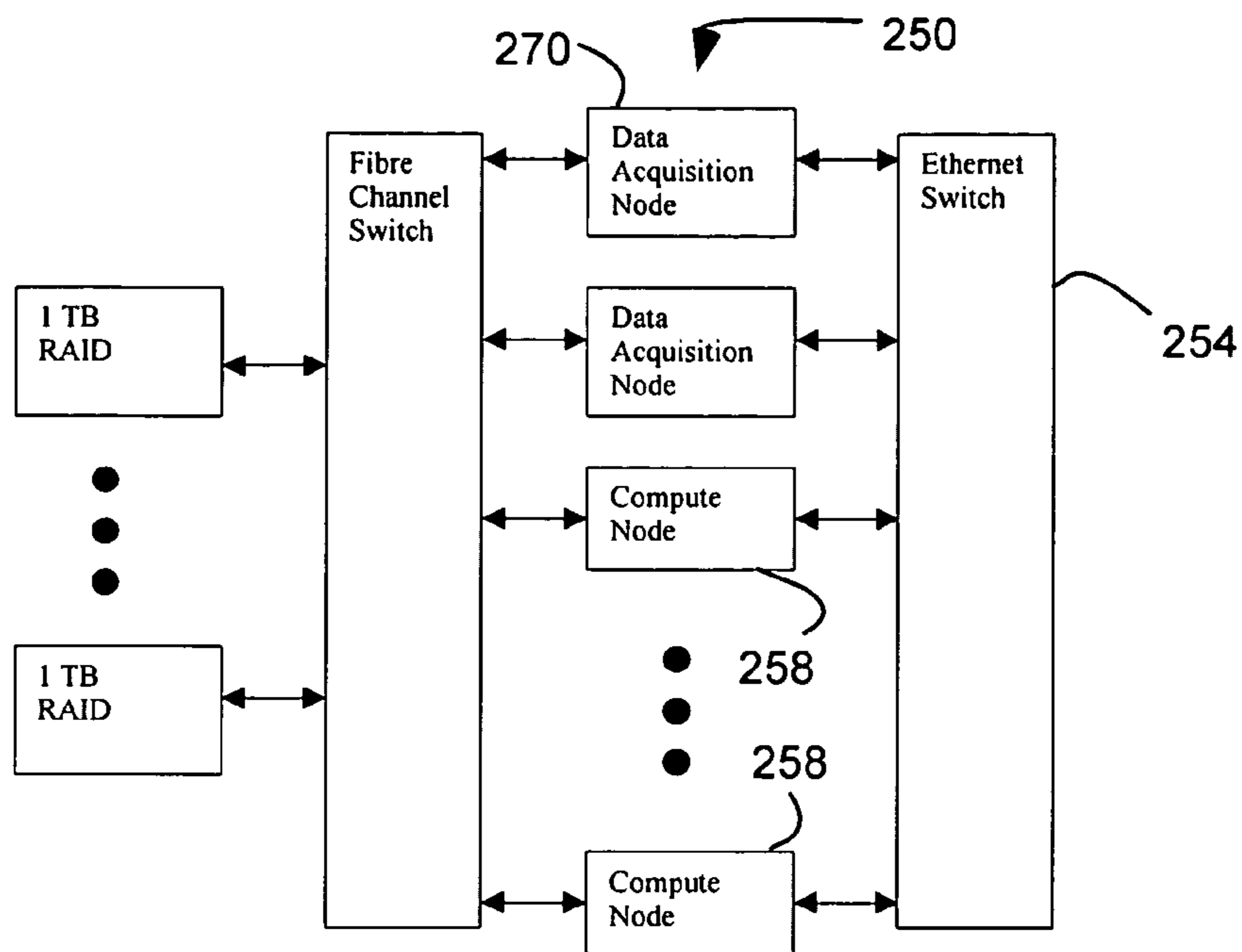
Ultrasound System Block Diagram
