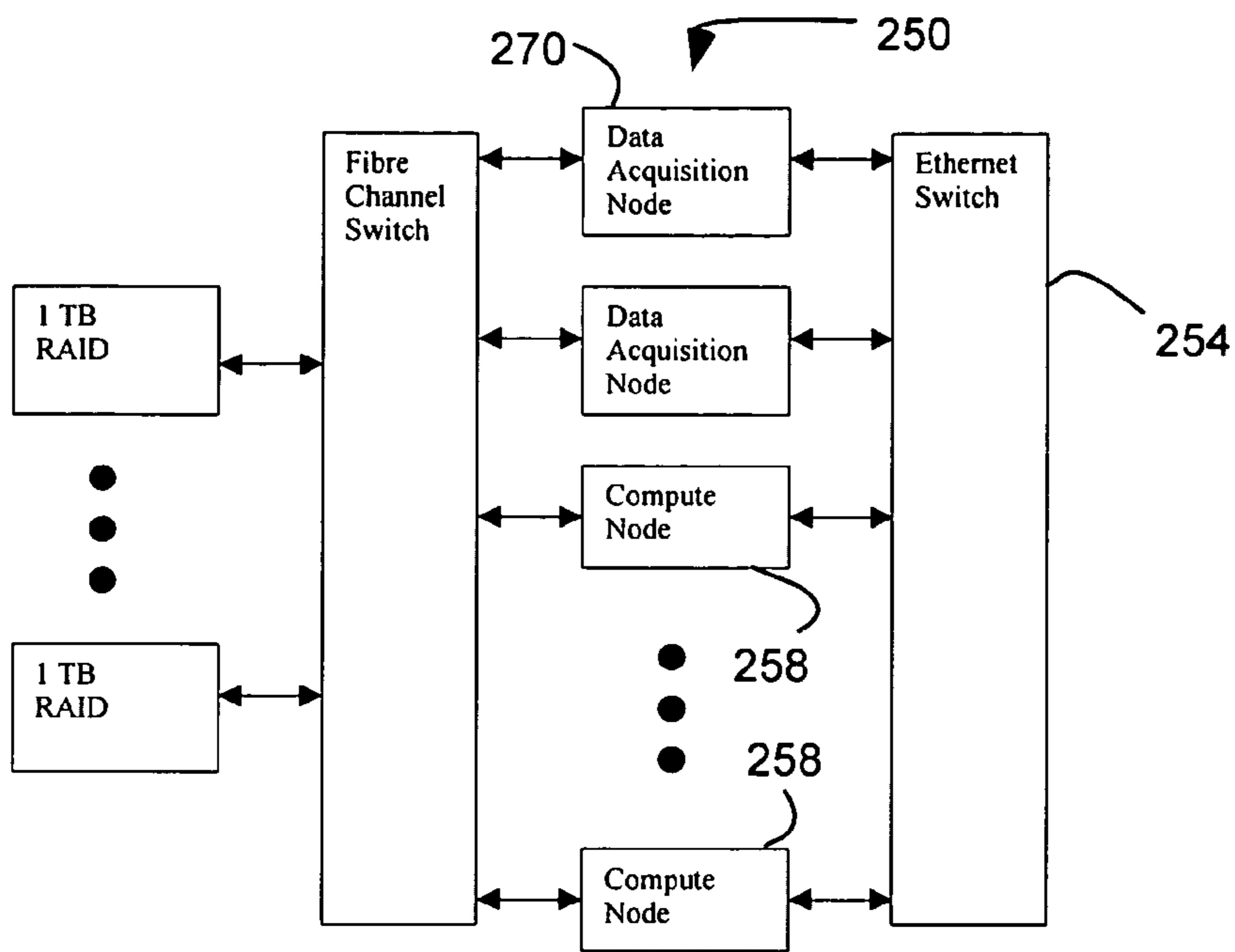
Ultrasound System Block Diagram
