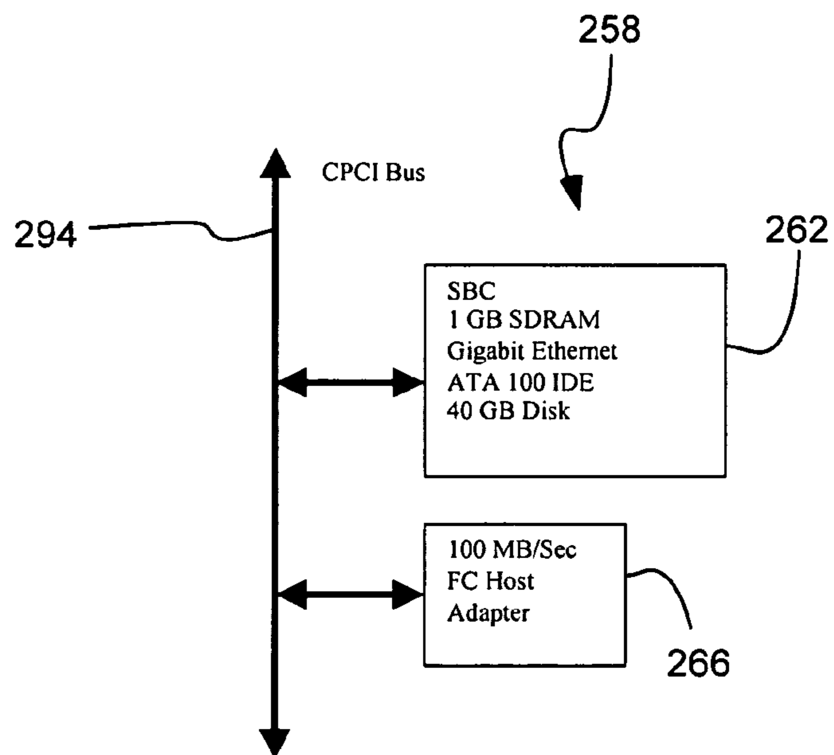
Compute Node Block Diagram
