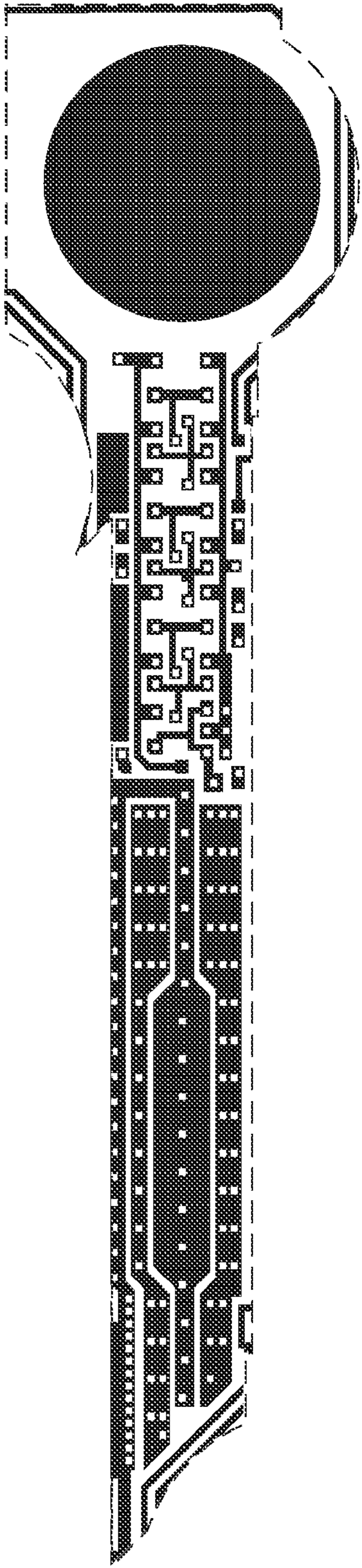
Metal 1 mask
