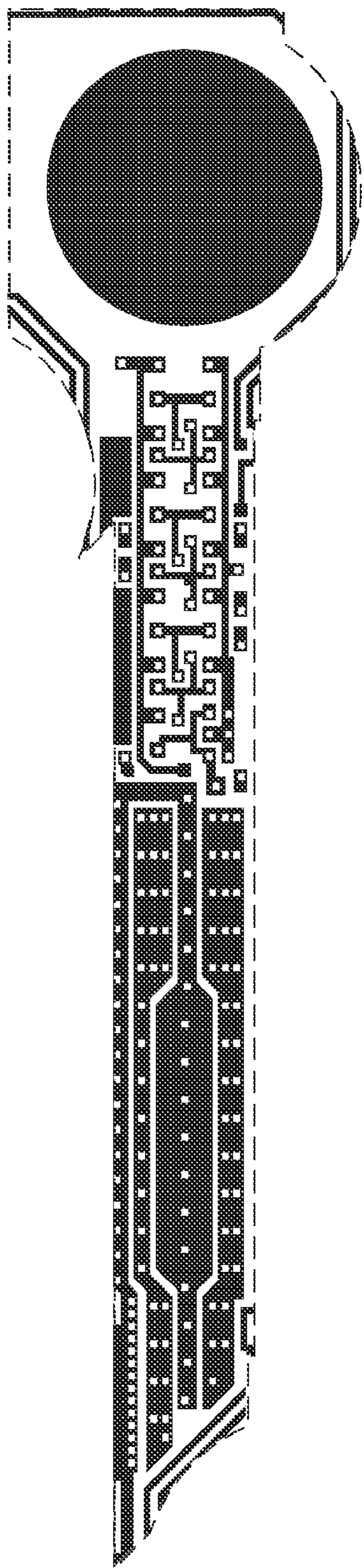
Metal 1 mask
