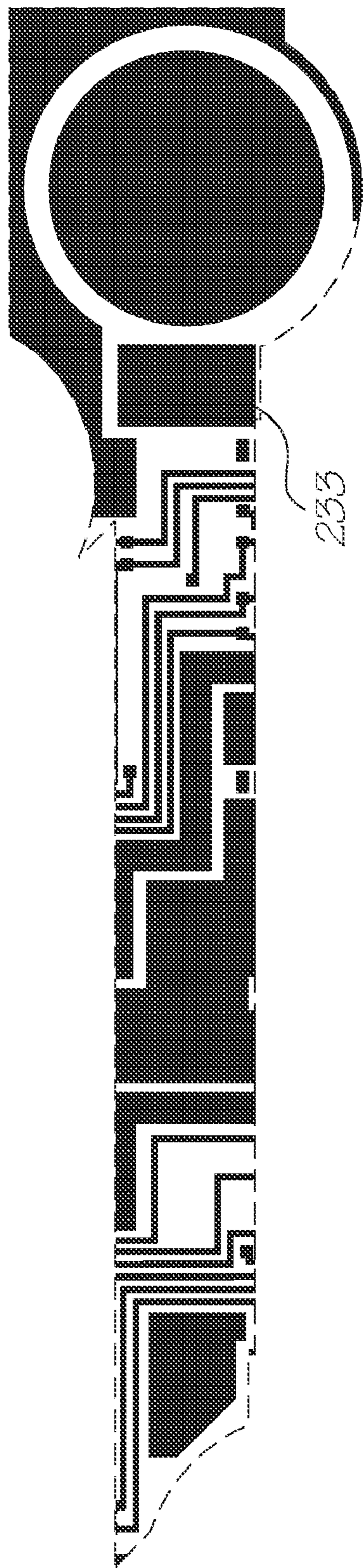
Metal 2 mask
