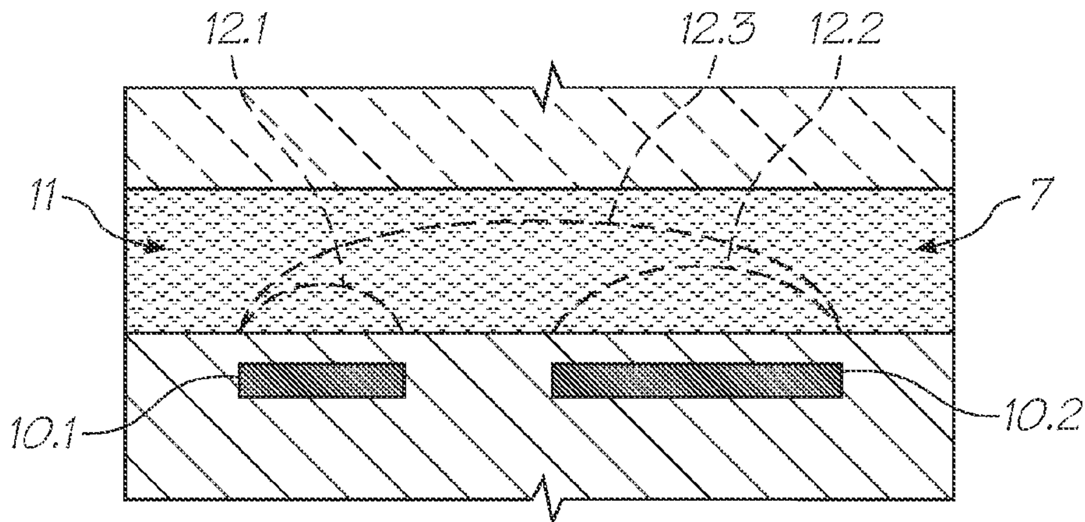
FIG. 52 (PRIOR ART)
