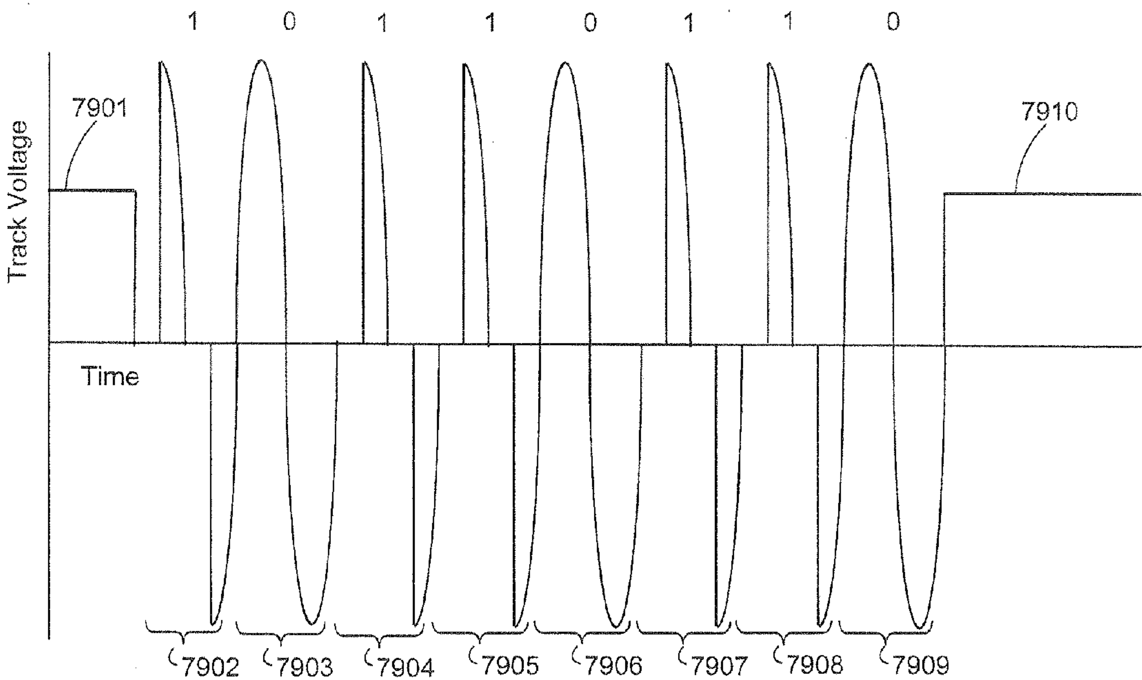
Figure 79 – Type 14 Signaling
