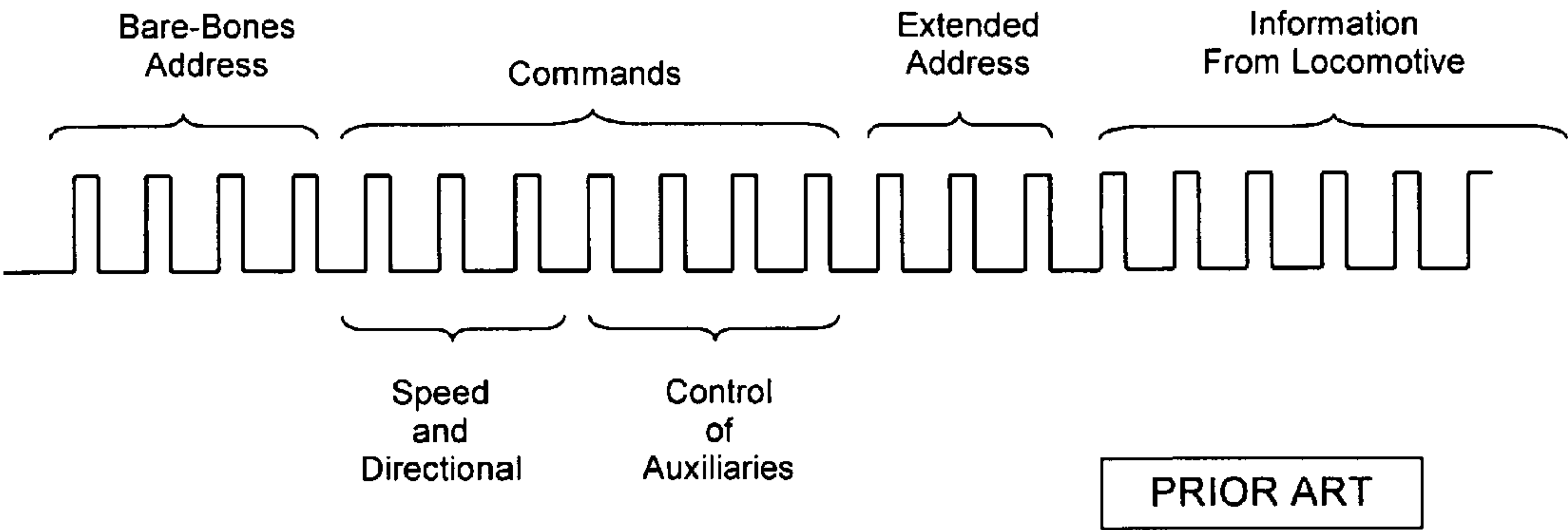
Fig. 17-9 Possible complete digital code.
