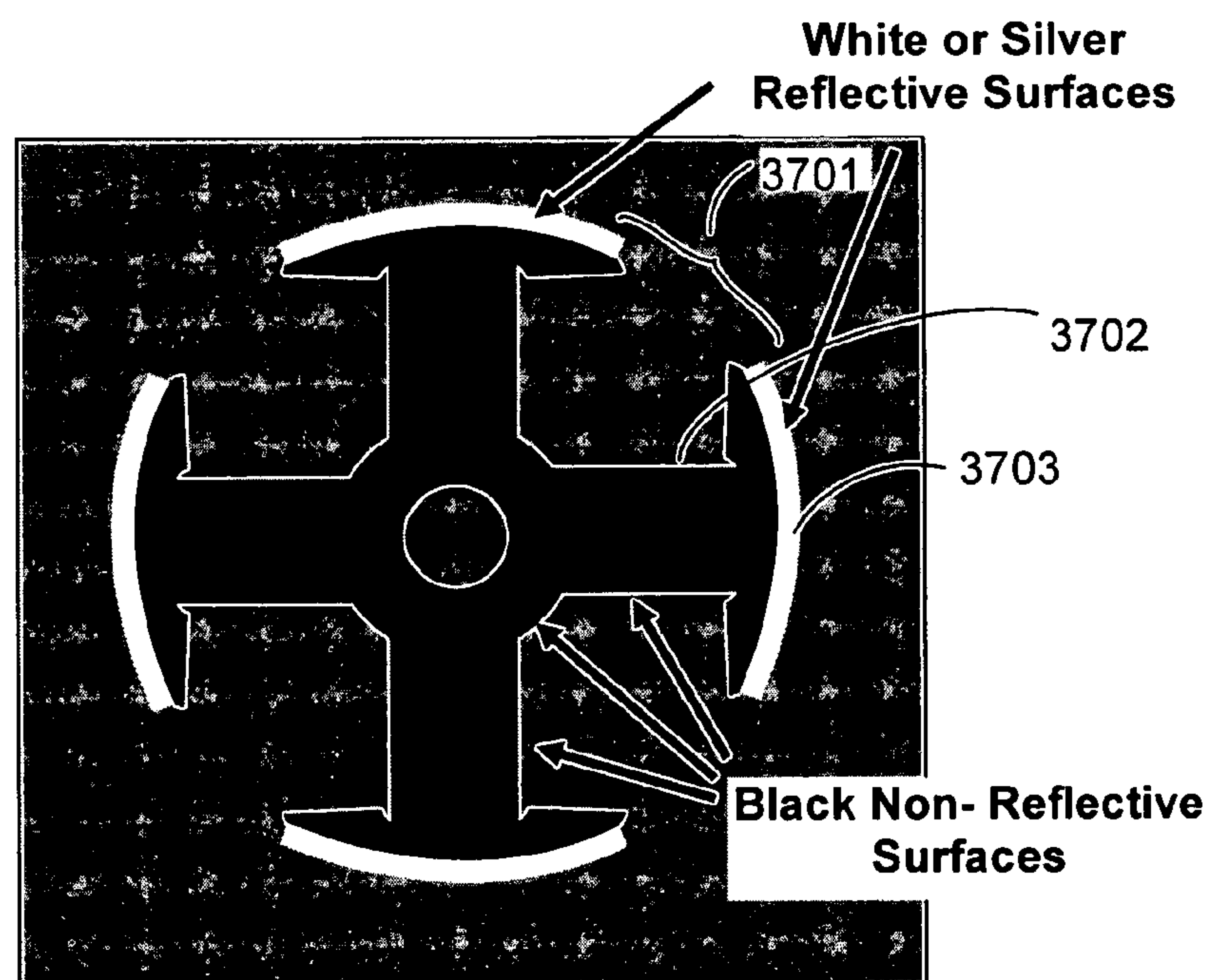
End View of Cylinder Drum
