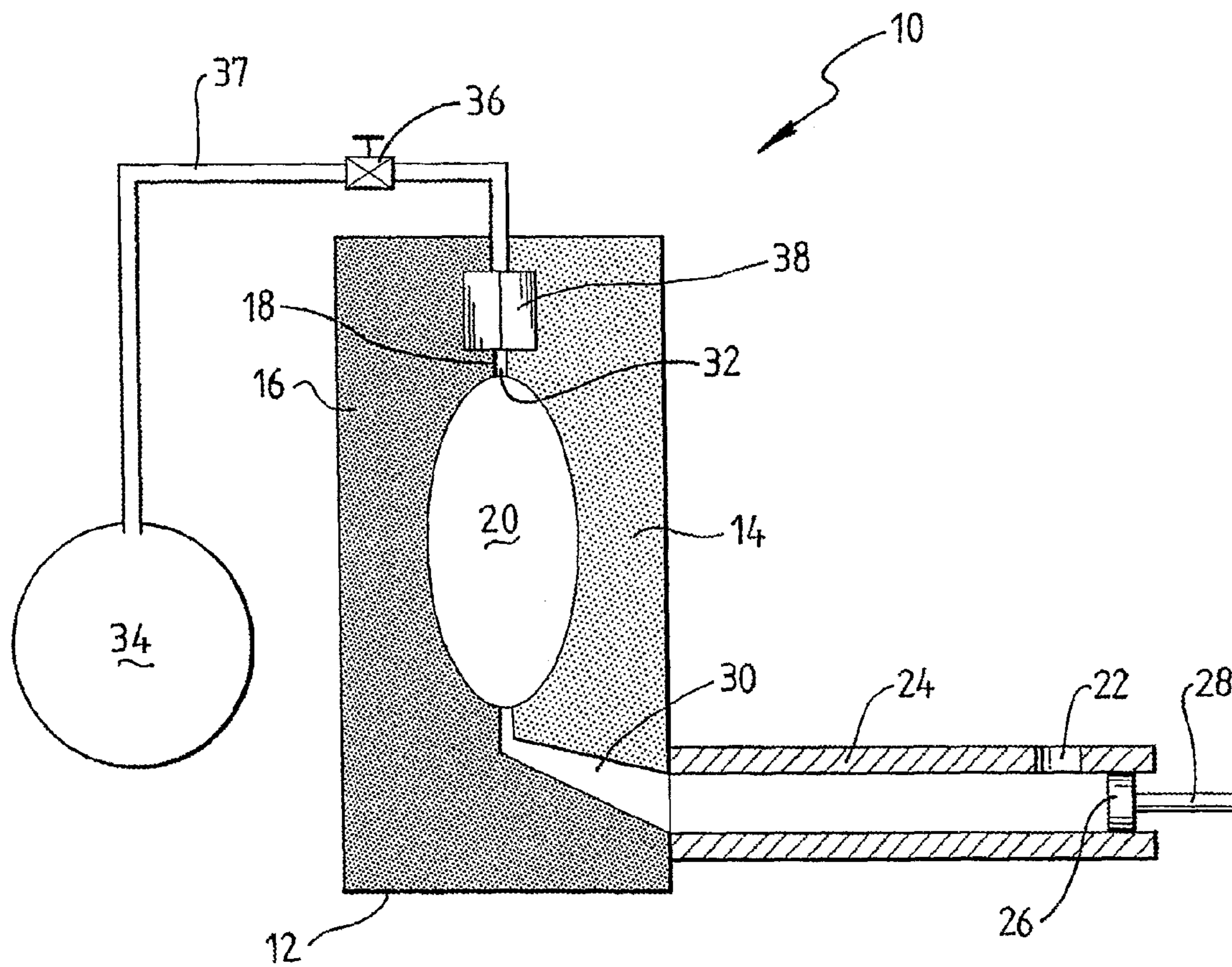
Fig. 1 (PRIOR ART)
