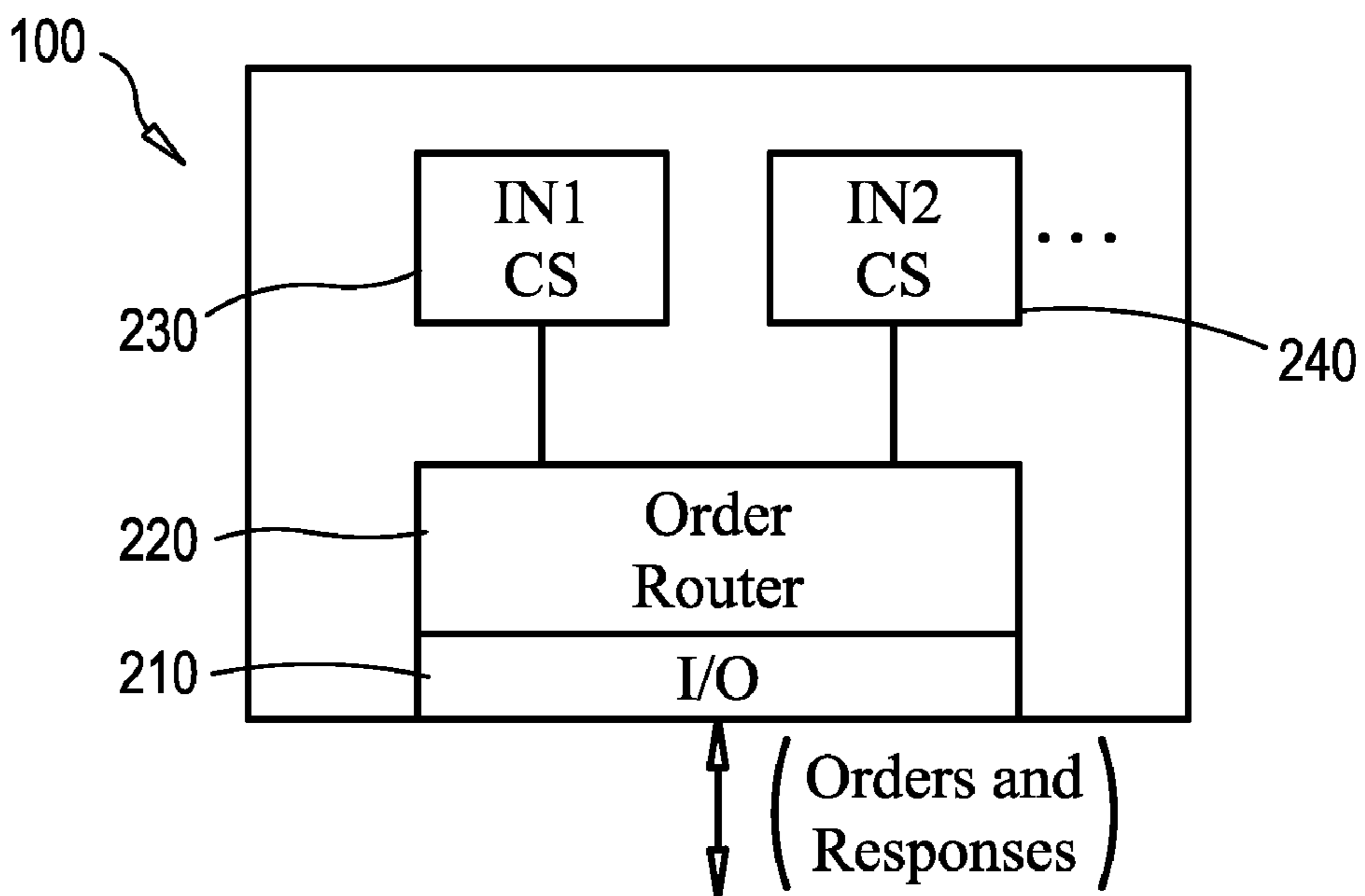
FIG. 2 IN - Instrument
