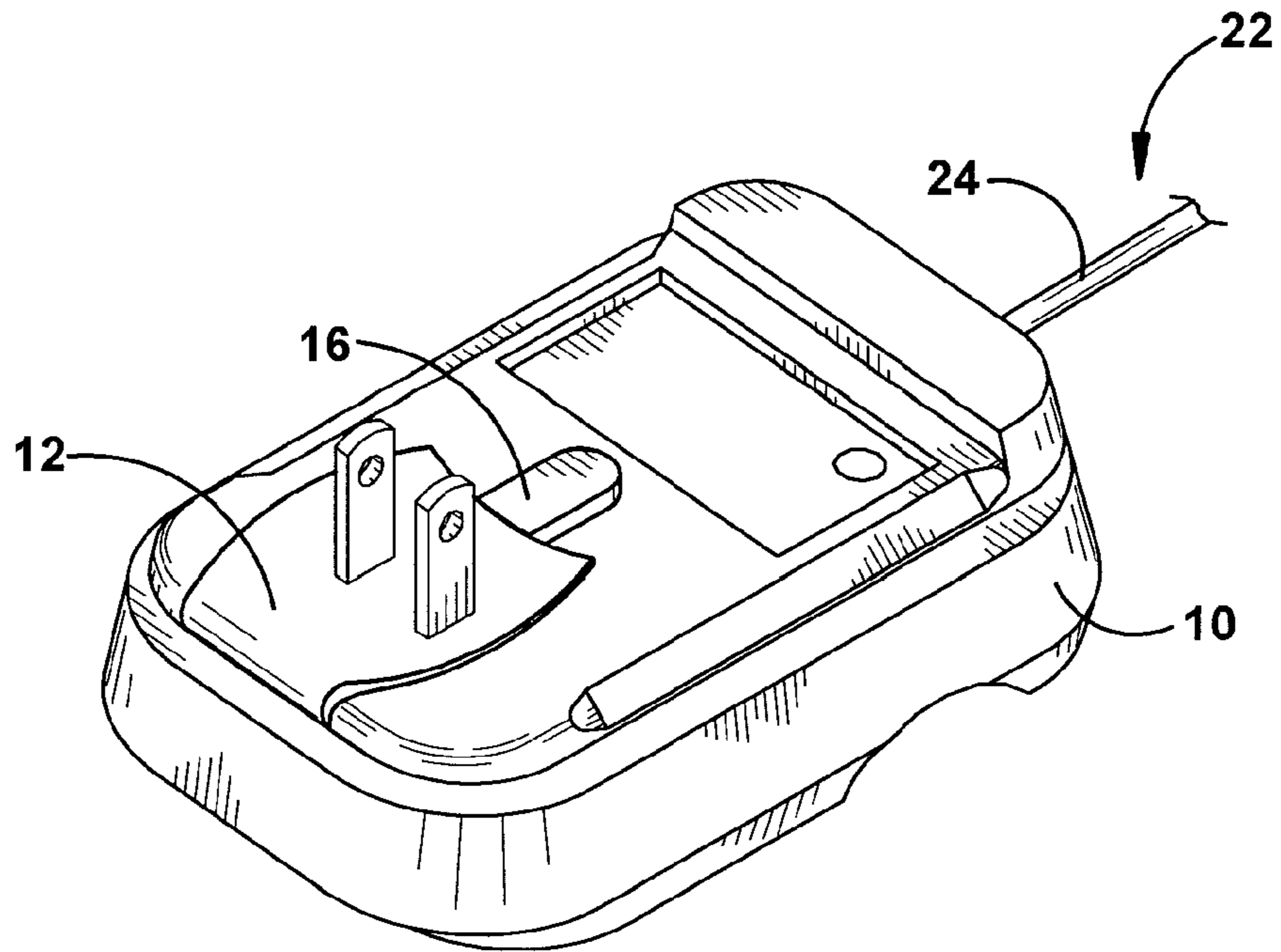
Fig.1 (PRIOR ART)
