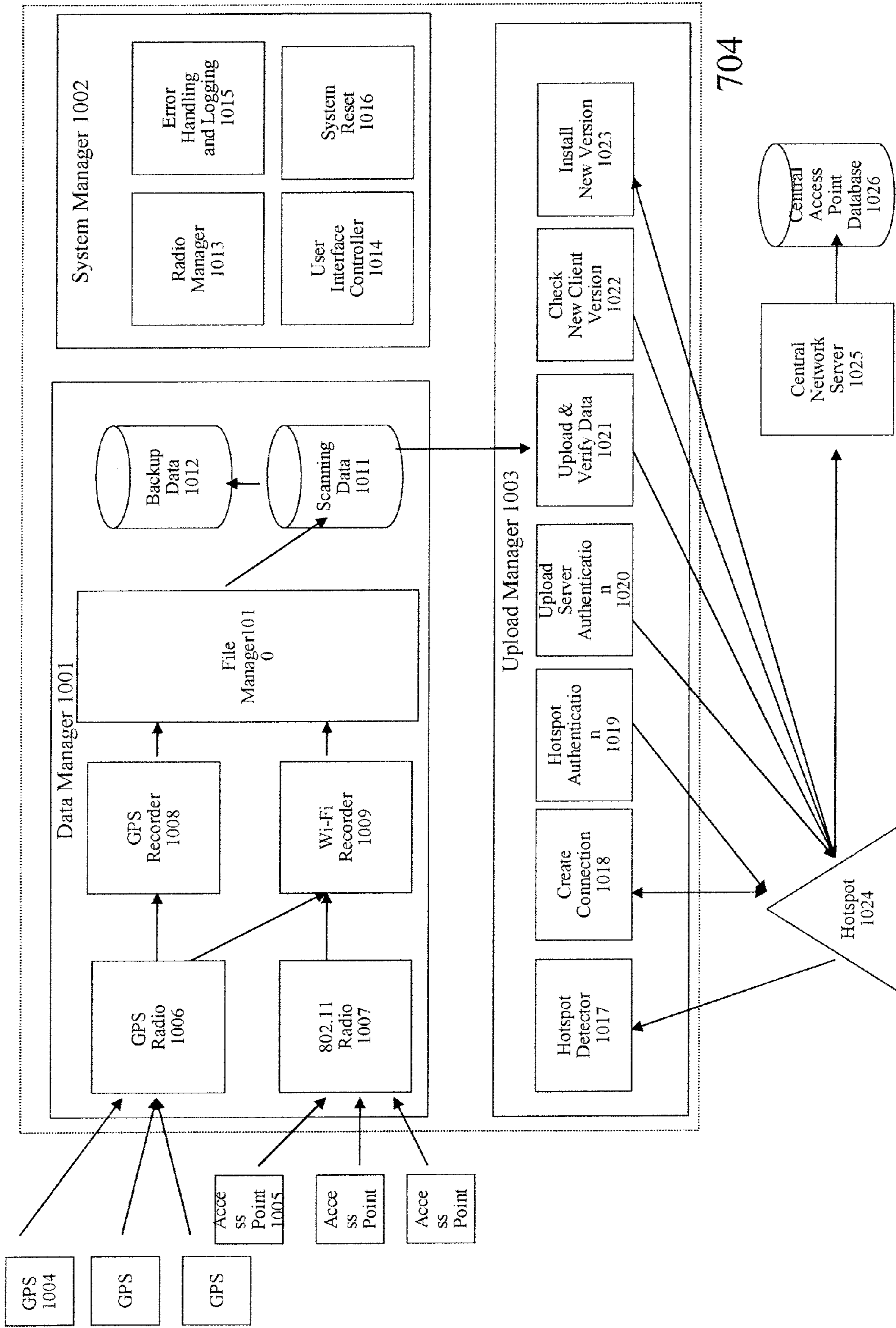
Figure 10: Scanning Client
