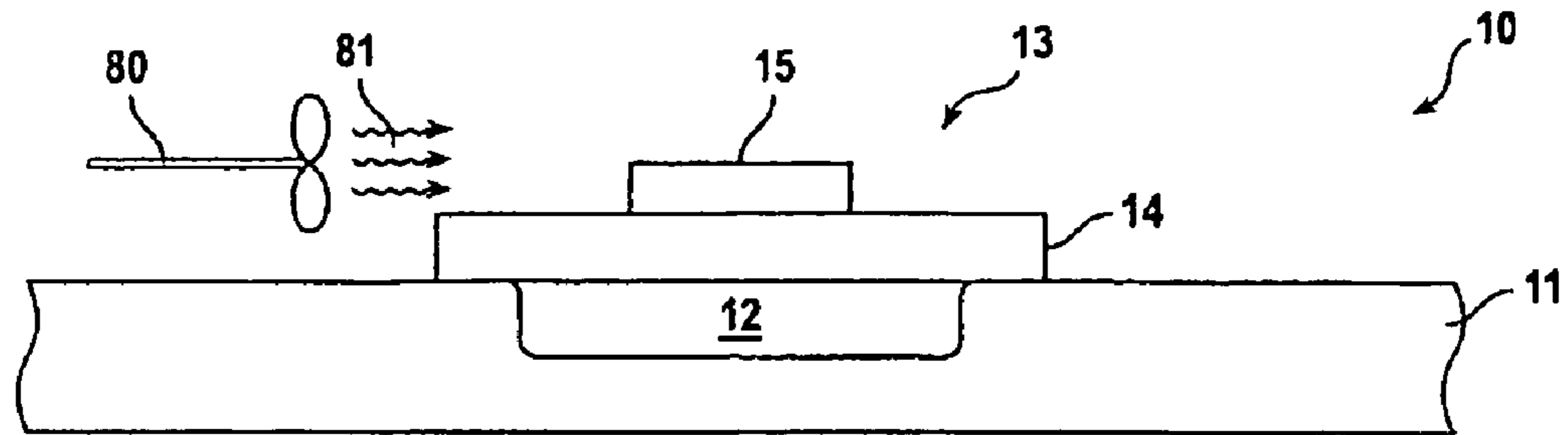
FIG. 1 (PRIOR ART)
