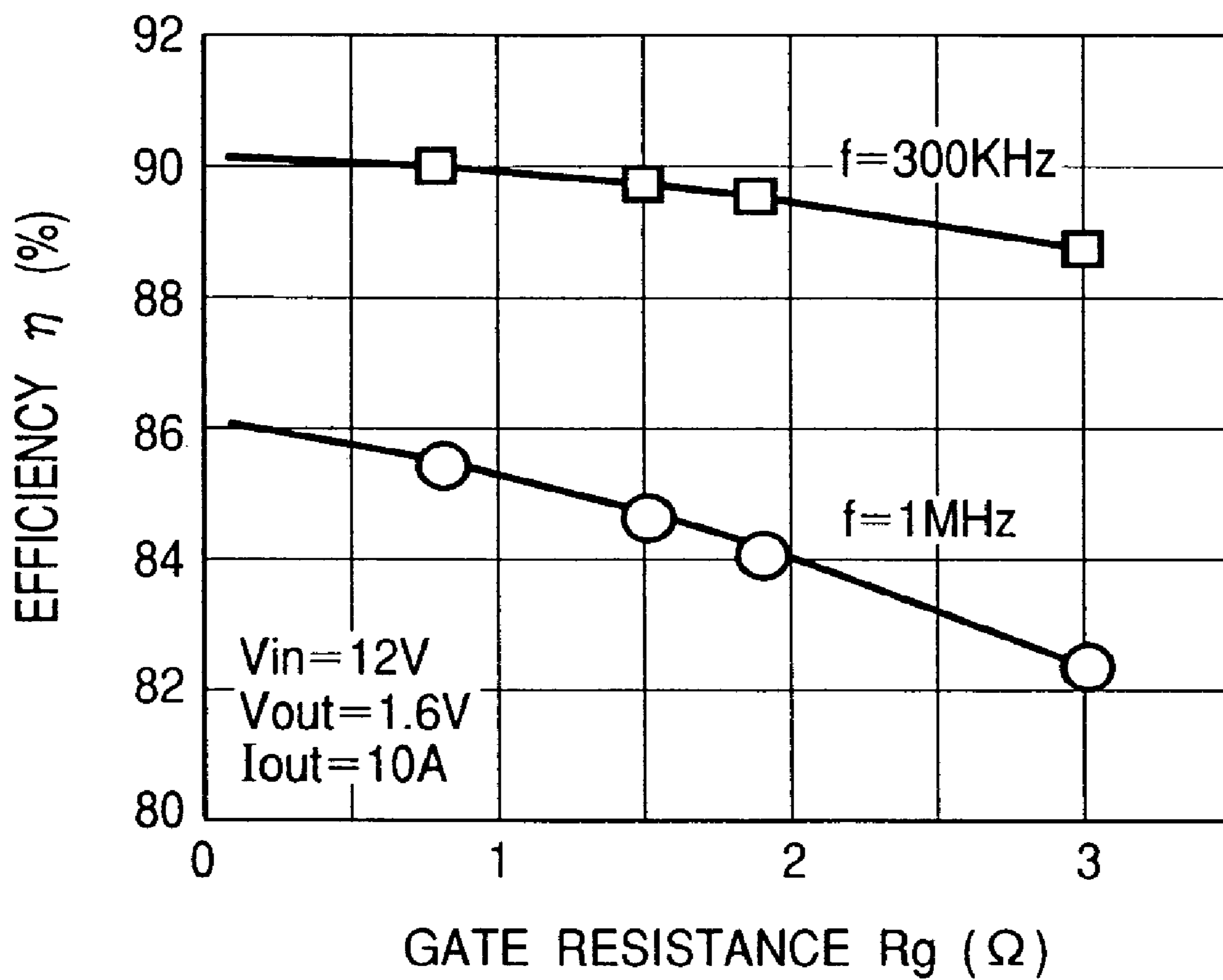
RELATION BETWEEN GATE RESISTANCE AND EFFICIENCY
