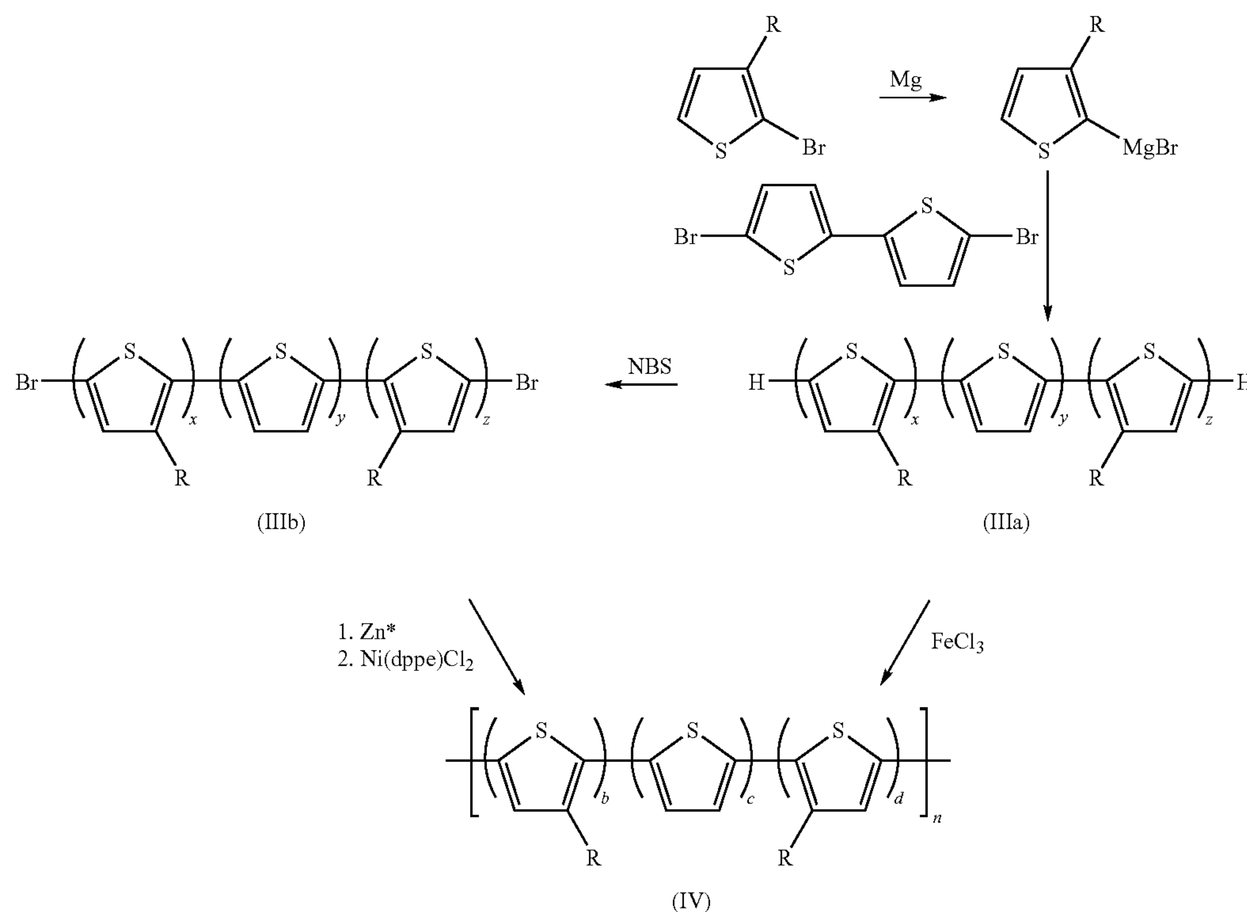
Scheme 1
