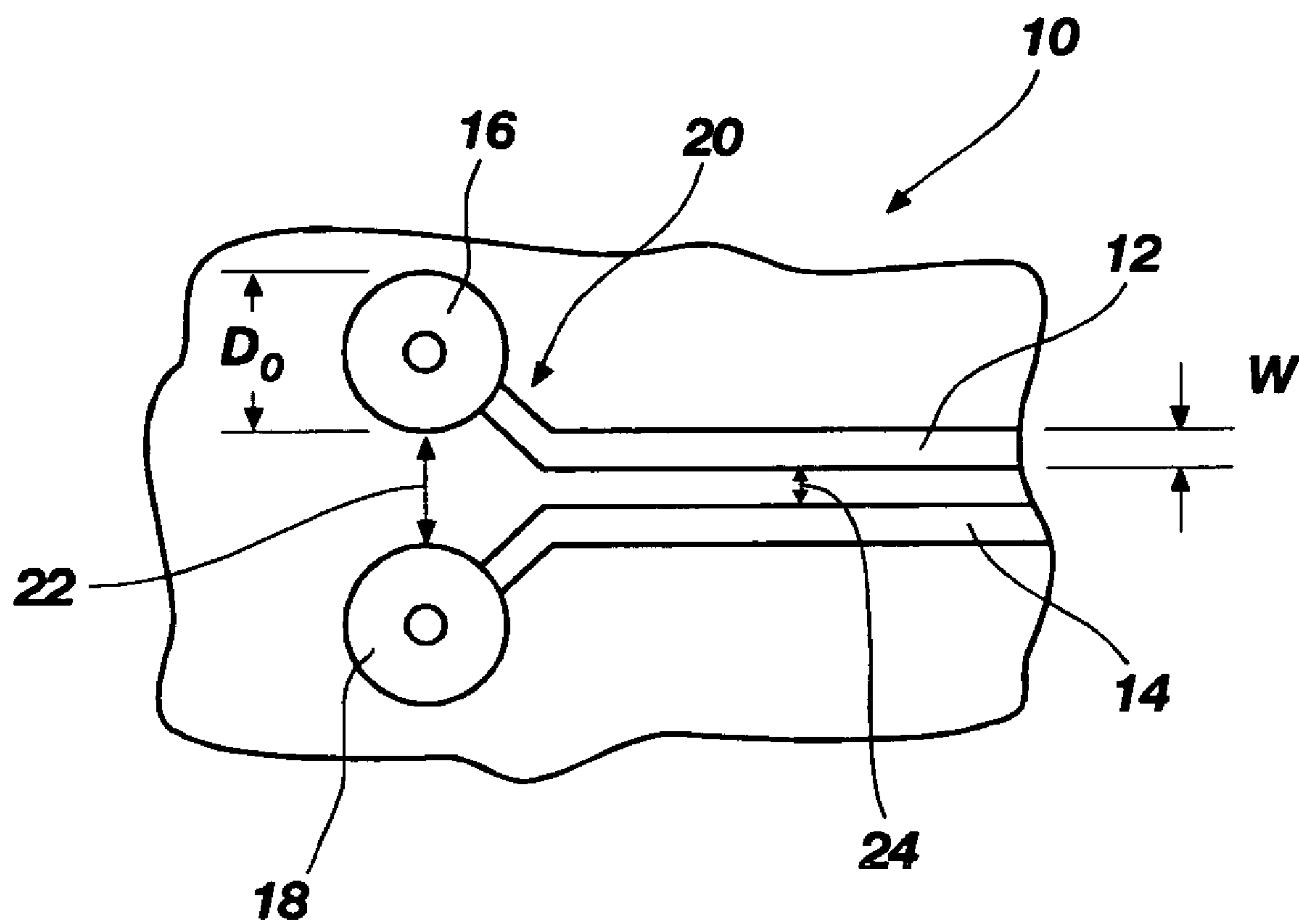
FIG. 1 (PRIOR ART)
