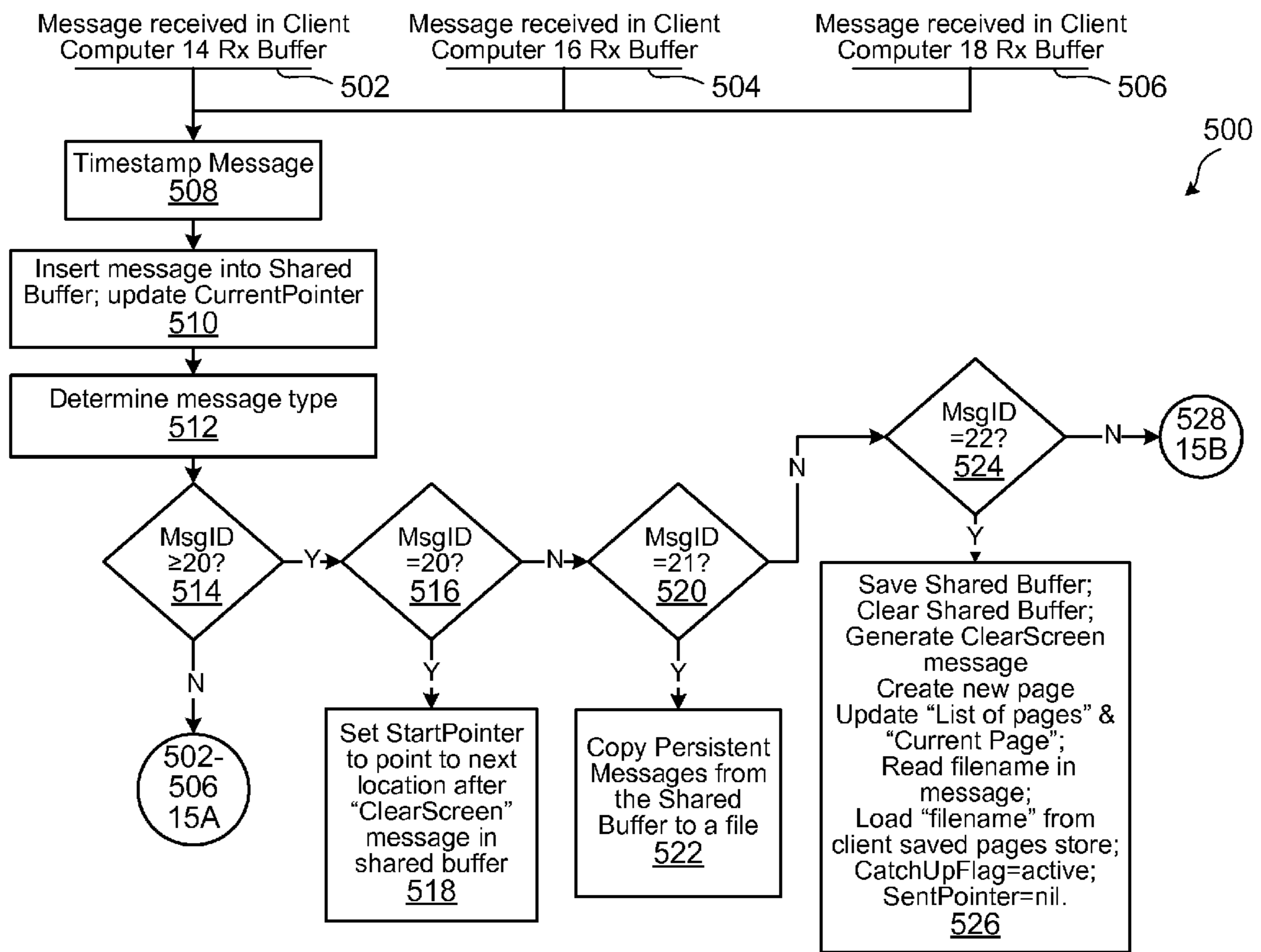
SERVER: Message receive process
