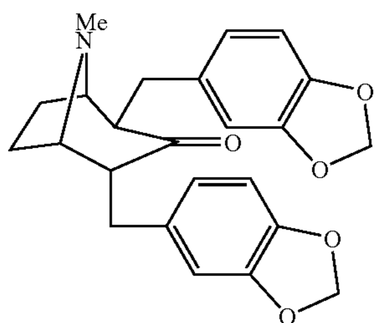
2,4-bis(3,4-methylenedioxybenzyl)-3-tropinone
