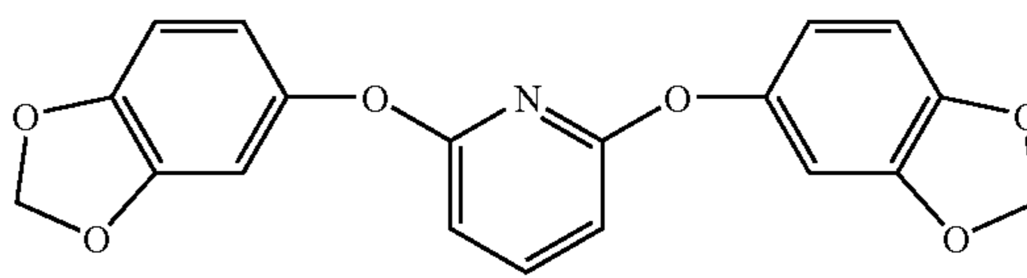
2,6-bis(3,4-methylenedioxyphenoxy) pyridine
