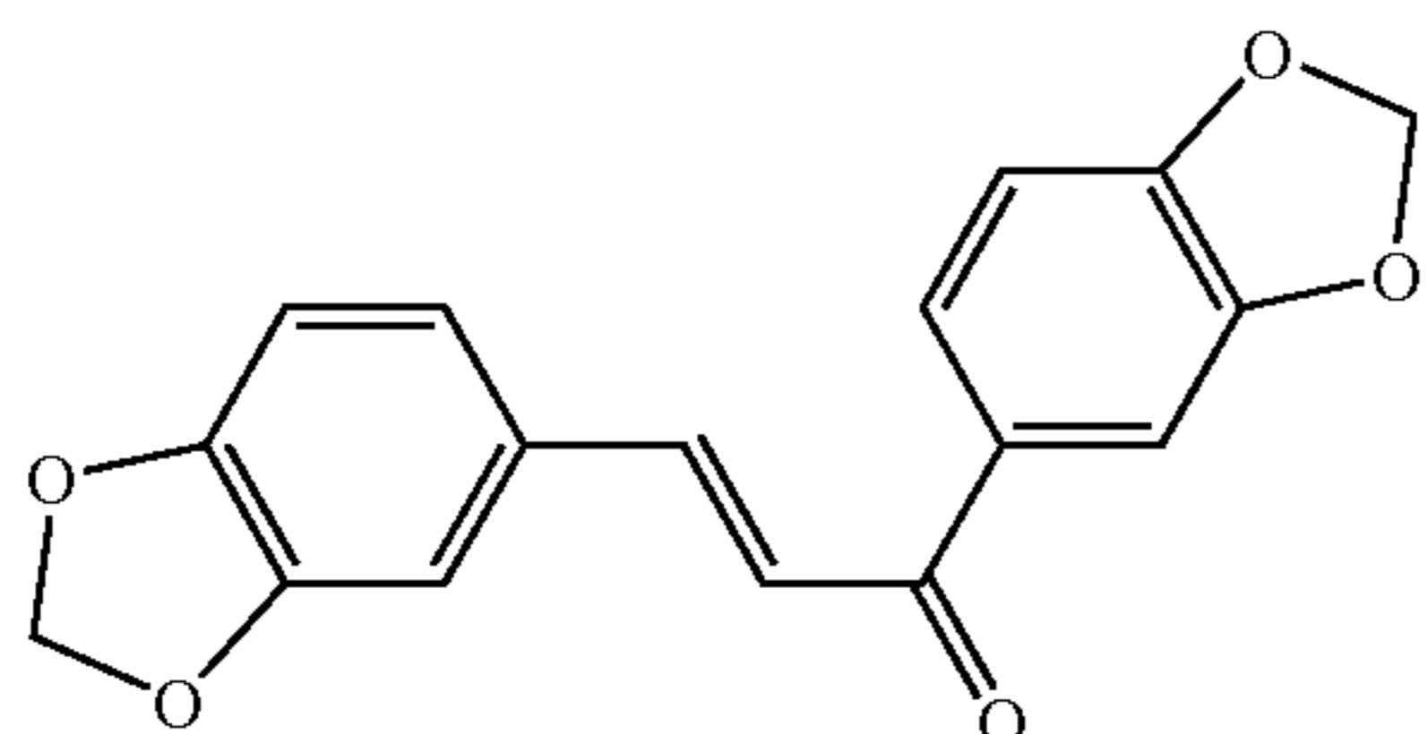
bis(3,4-methylenedioxy)chalcone
