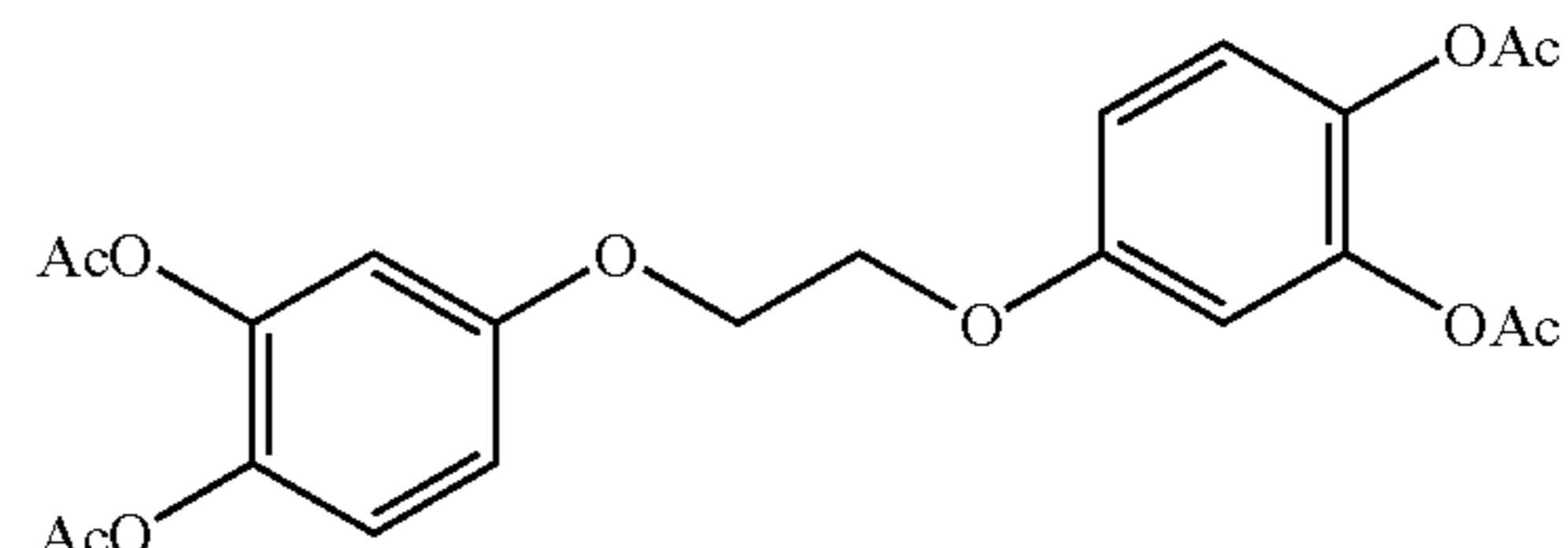
1,2-bis(3,4-diacetoxyphenoxy)ethane
