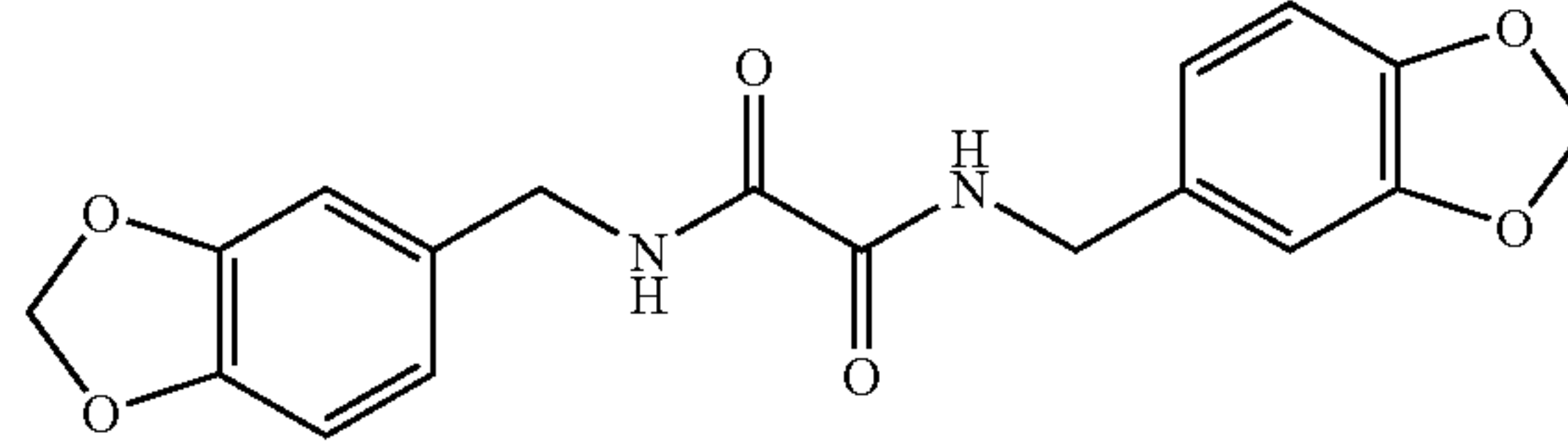
Oxalic acid bis(3,4-methylene- dioxybenzylamide)
