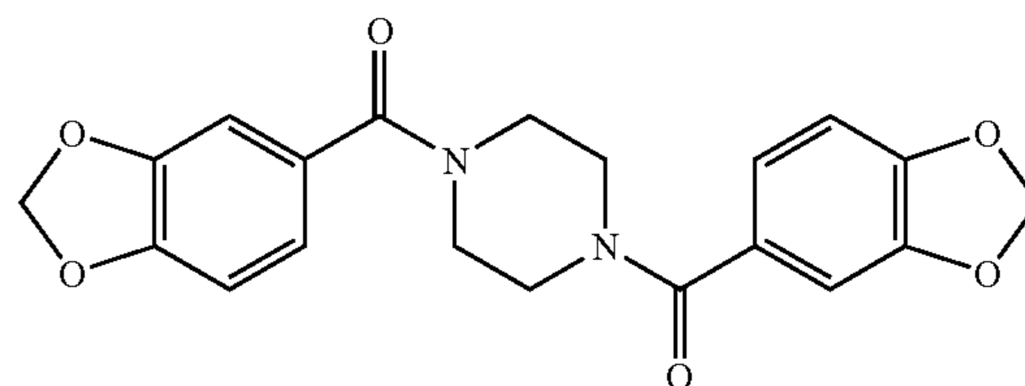
1,4-bis(3,4-methylenedioxybenzoyl)piperazine
