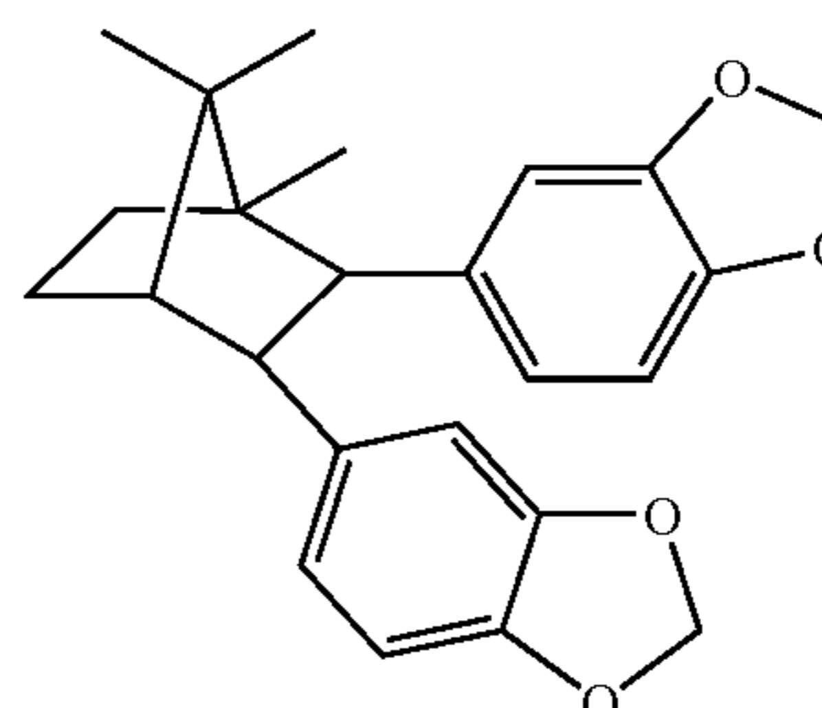
2,3-bis(3,4-methylenedioxyphenyl)-1,7,7-trimethyl-bicyclo[2,2,1]heptane
