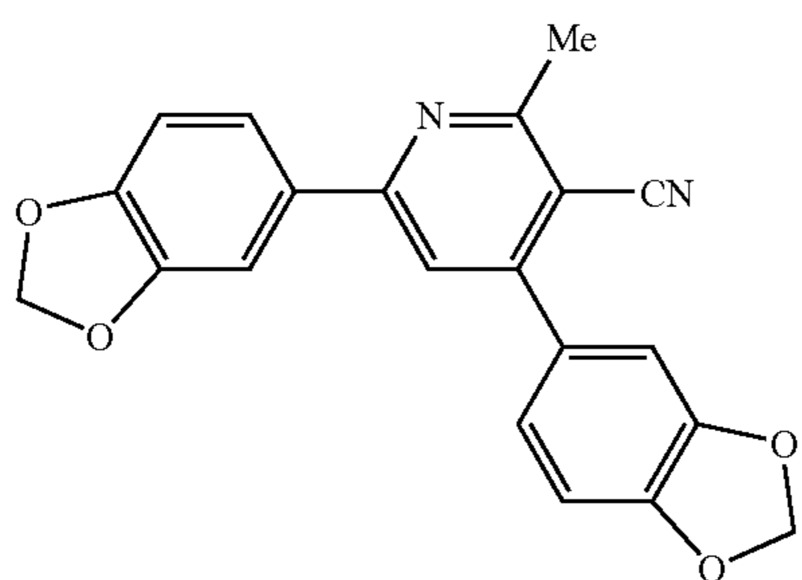
4,6-bis(3,4-methylenedioxyphenyl)- 3-cyano-2-methylpyridine
