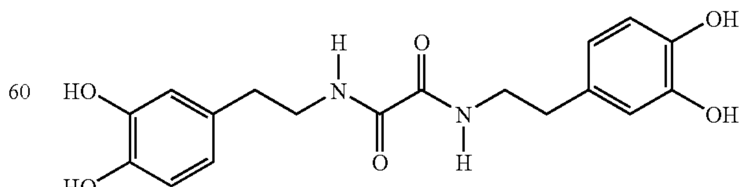
Oxalic acid-bis(3,4-dihydroxyphen(-) ethylamide)
