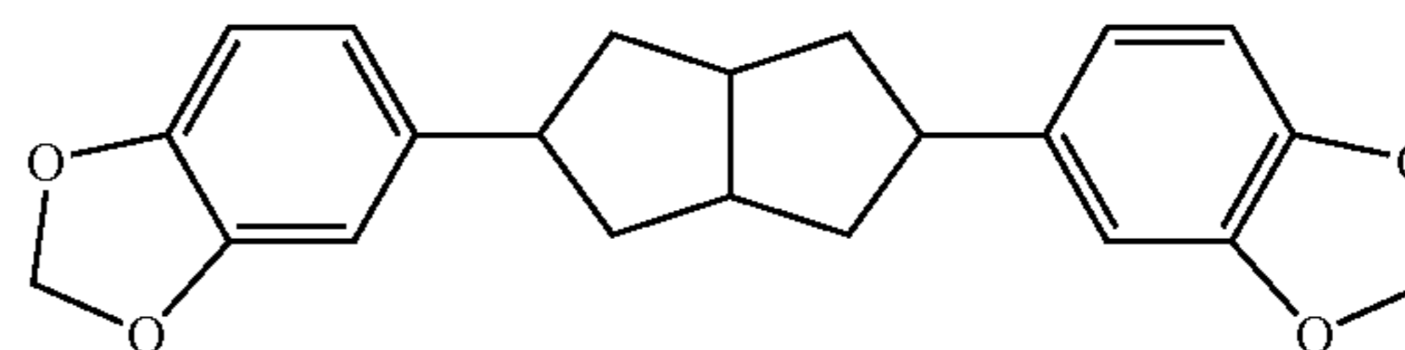
3,7-bis(3,4-methylenedioxyphenyl)bicyclo[3,3,0](-)octane
