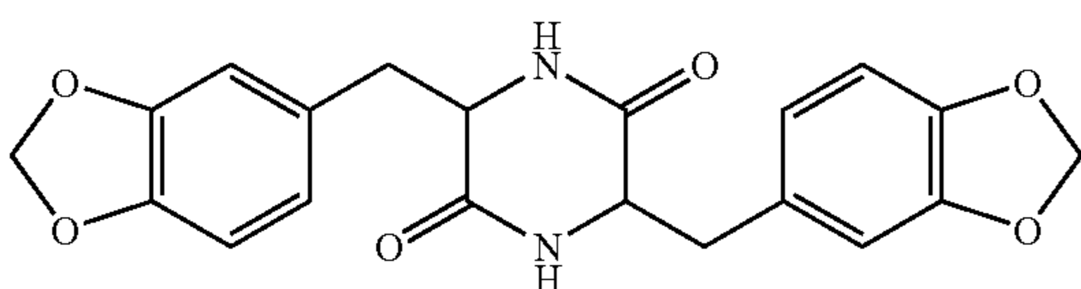
3,6-bis(3,4-methylenedioxybenzyl)-2,5-diketopiperazine
