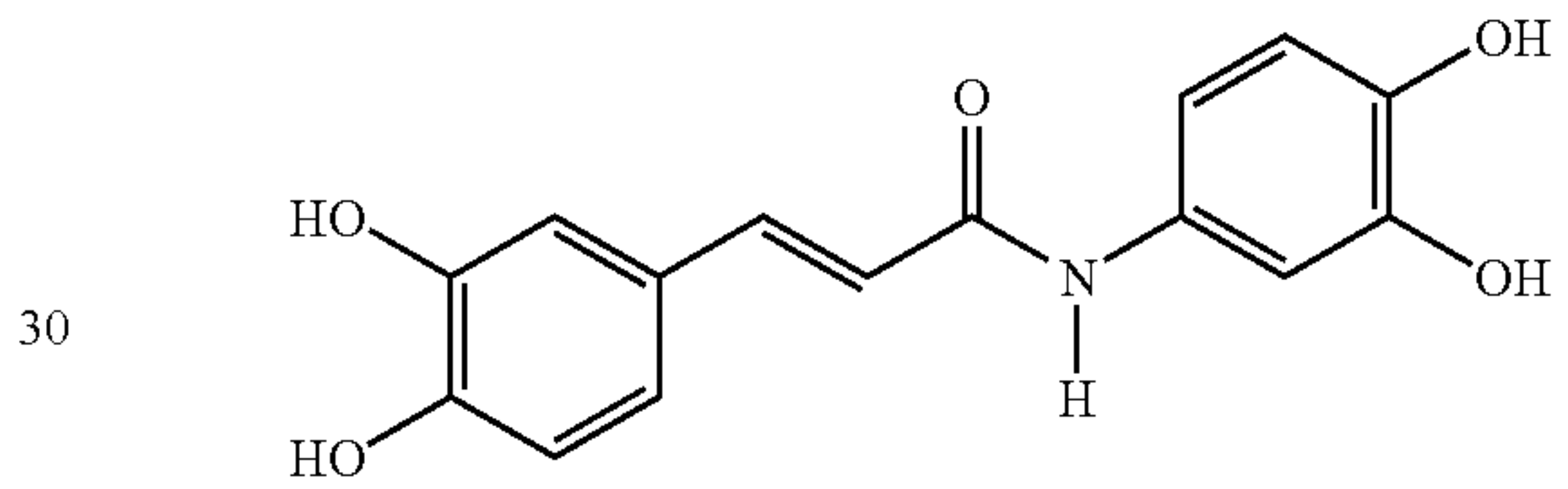
3,4-dihydroxycinnamic acid 3,4-dihydroxyanilide
