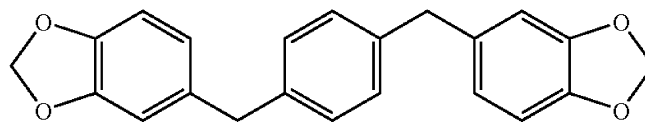
1,4-bis(3,4-methylenedioxybenzyl)benzene
