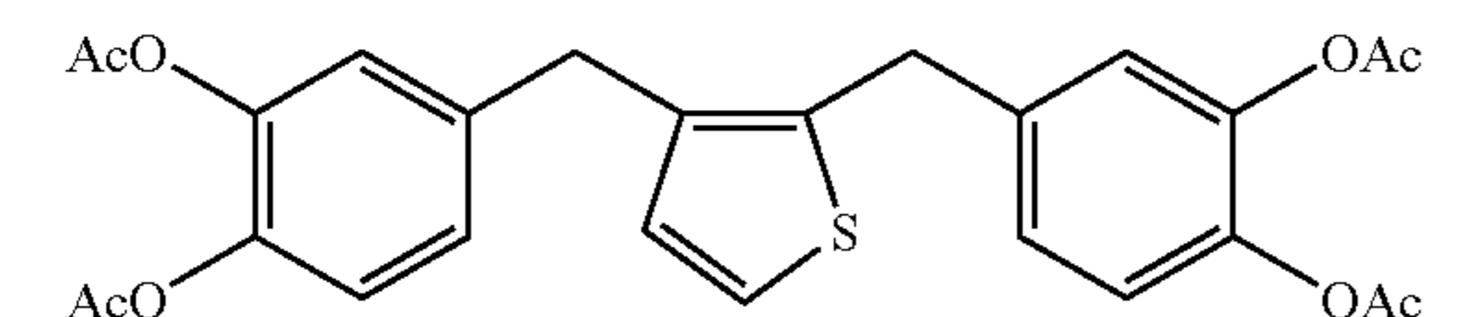
2,3-bis(3,4-diacetoxybenzyl)thiophene
