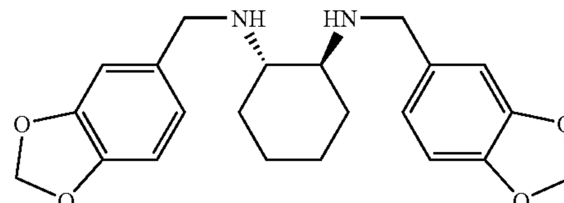
N,N'-bis(3,4-methylenedioxybenzyl)trans- 1,2-diaminocyclohexane
