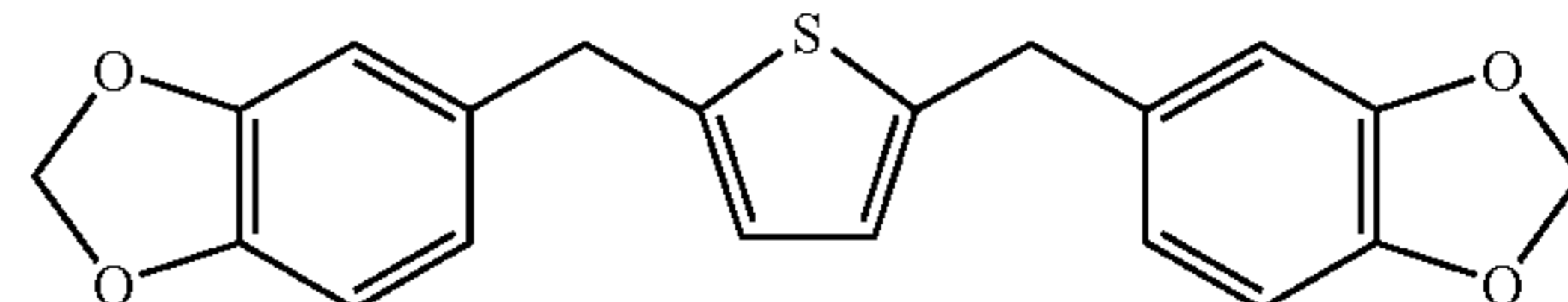
2,5-bis(3,4-methylenedioxybenzyl)-thiophene
