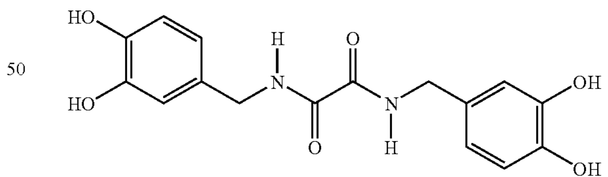
Oxalic acid-bis(3,4-dihydroxybenzyl(-) amide)
