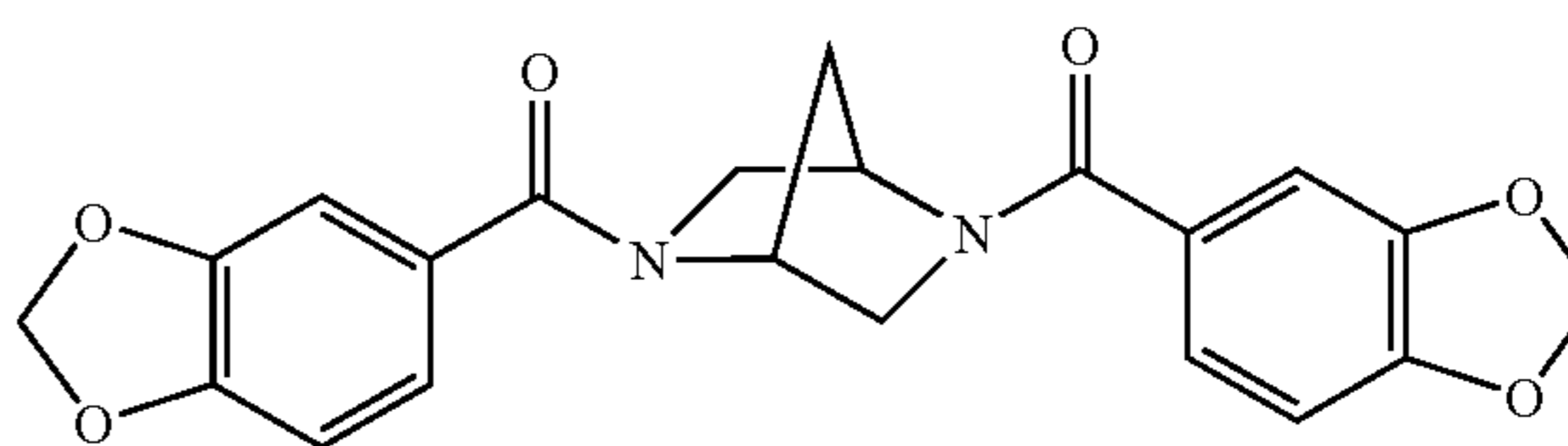
2,5-bis(3,4-methylenedioxybenzoyl)-2,5-diaza[2,2,1]-bicycloheptane
