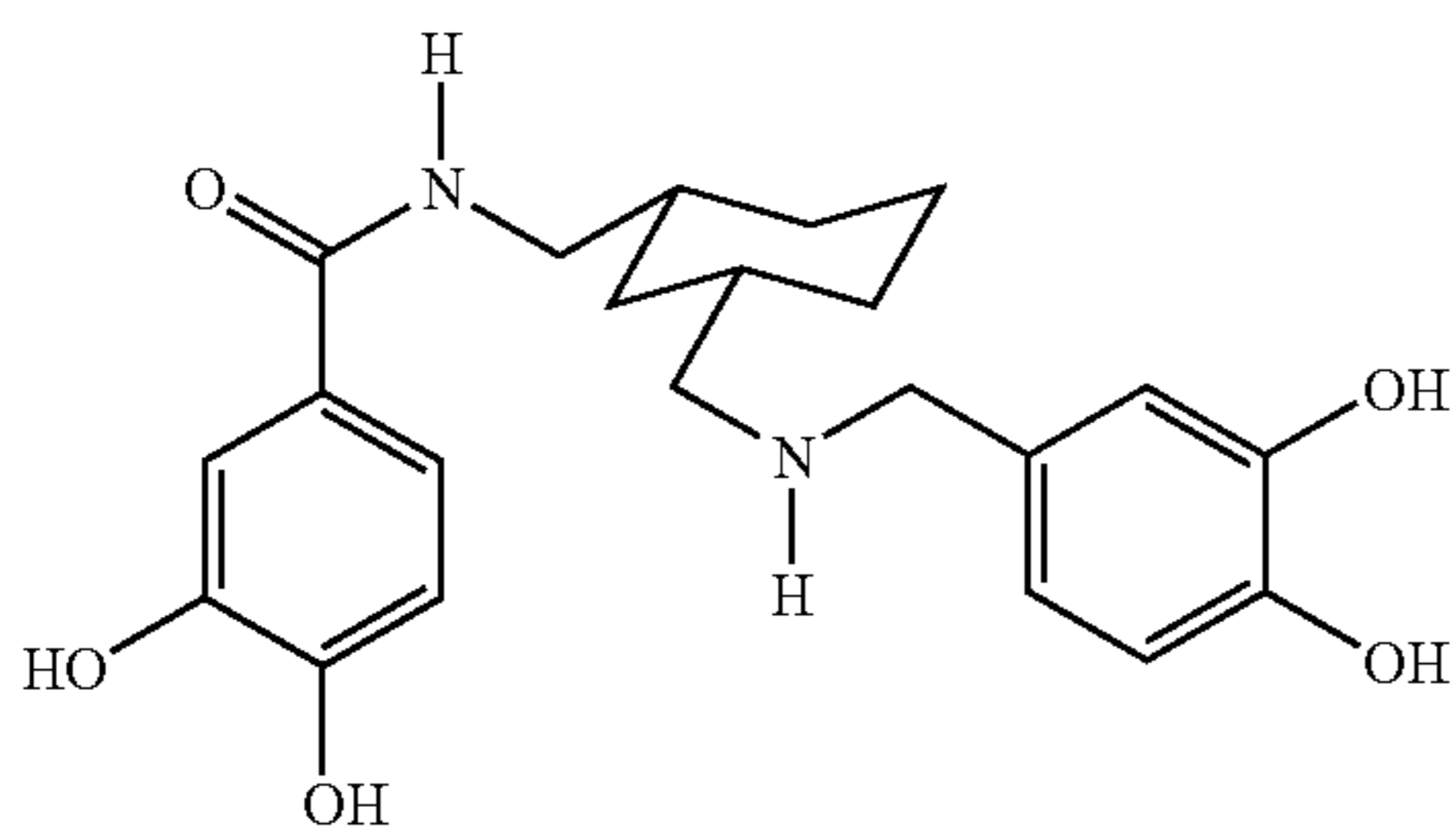
N,N'-bis(3,4-dihydroxybenzoyl)-cis-1,3-bis-aminomethylcyclohexane
