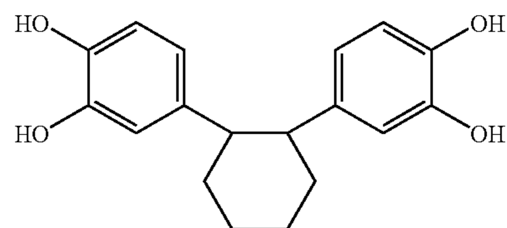
1,2-bis(3,4-dihydroxyphenyl)cyclohexane
