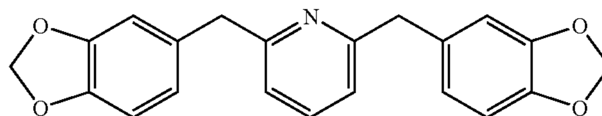
2,6-bis(3,4-methylenedioxybenzyl)pyridine
