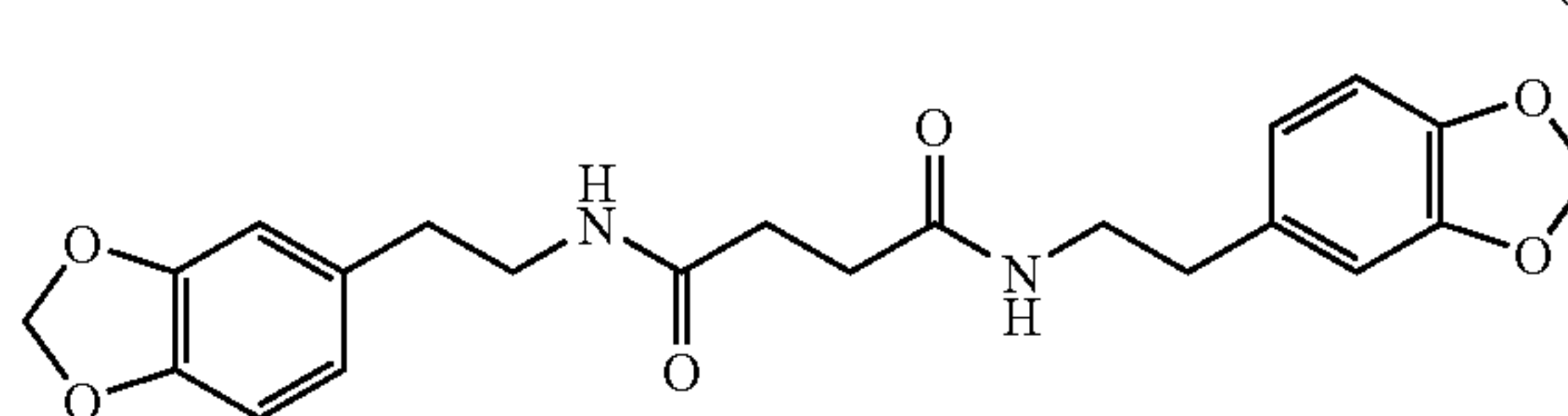
Succinic acid bis(3,4-methylene- dioxyphenethylamide)
