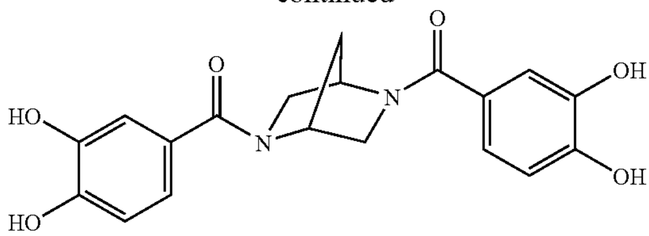
2,5-bis(3,4-dihydroxybenzoyl)-2,5-diaza-[2.2.1]-bicycloheptane
