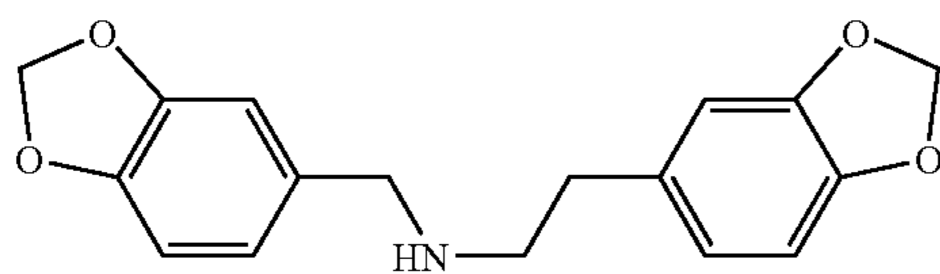
N-(3,4-methylenedioxybenzyl)-3,4-methylenedioxyphenethylamine
