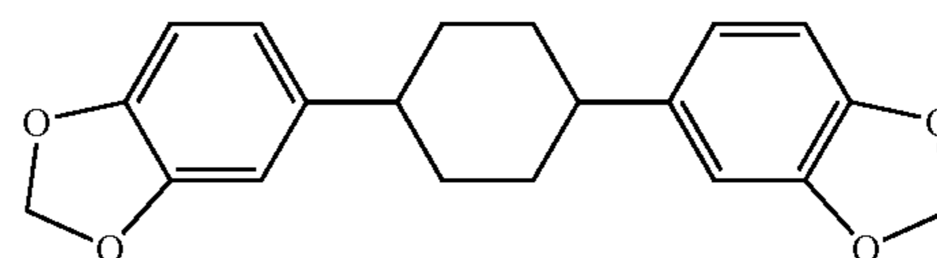
1,4-bis(3,4-methylenedioxyphenyl)cyclohexane
