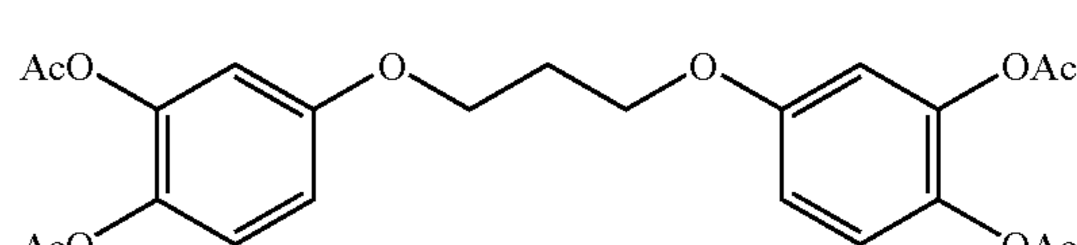
1,3-bis(3,4-diacetoxyphenoxy)propane
