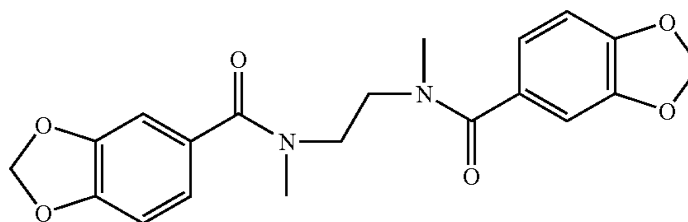
N,N'-bis(3,4-methylenedioxybenzoyl)-N,N'-dimethyl(-)ethylenediamine
