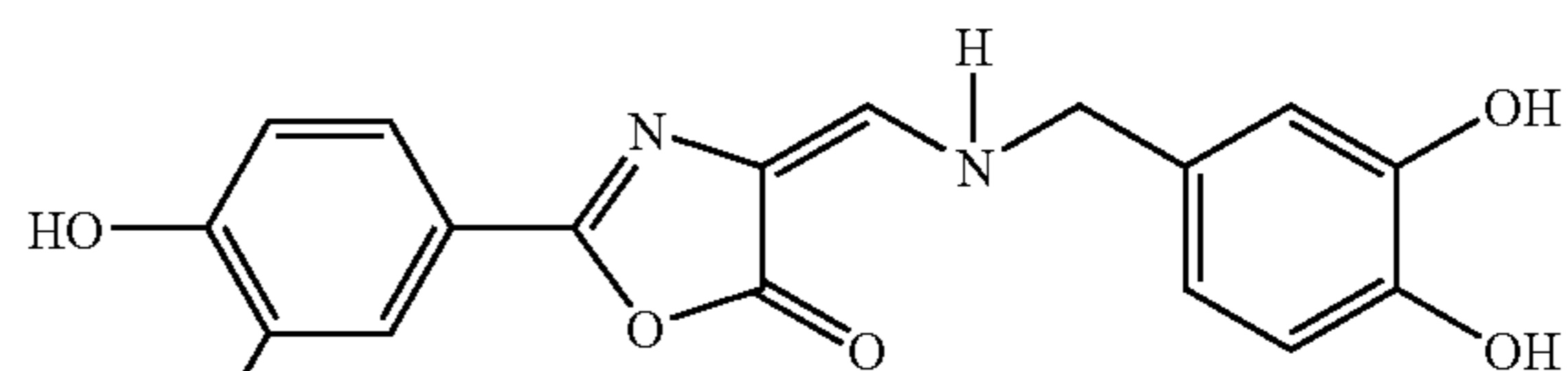
4-(3,4-dihydroxybenzylaminomethylene)-2-(3,4-dihydroxyphenyl)oxazolin-5-one
