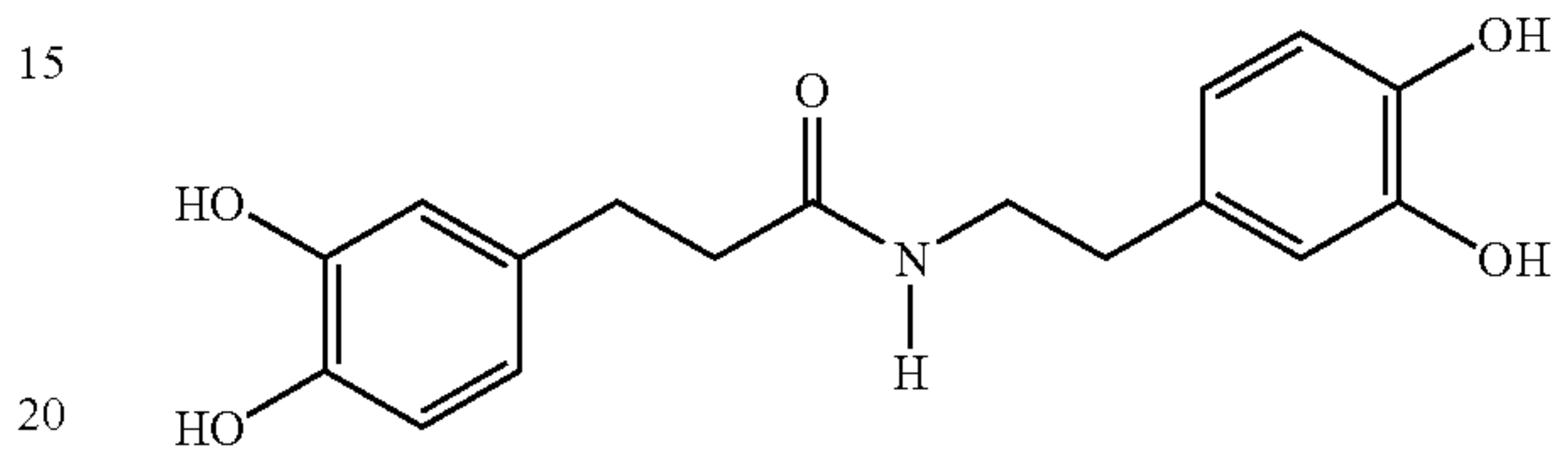
3-(3,4-dihydroxyphenyl)propionic acid 3,4-dihydroxyphenethylamide
