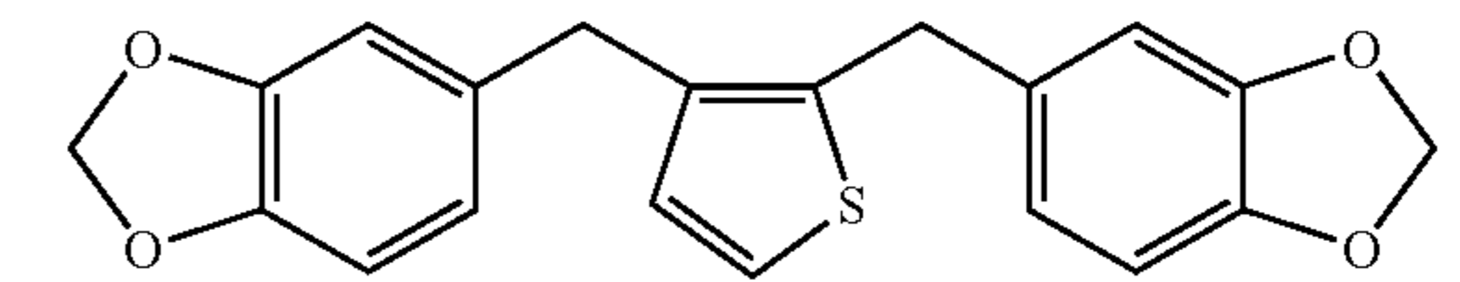
2,3-bis(3,4-methylenedioxybenzyl)-thiophene
