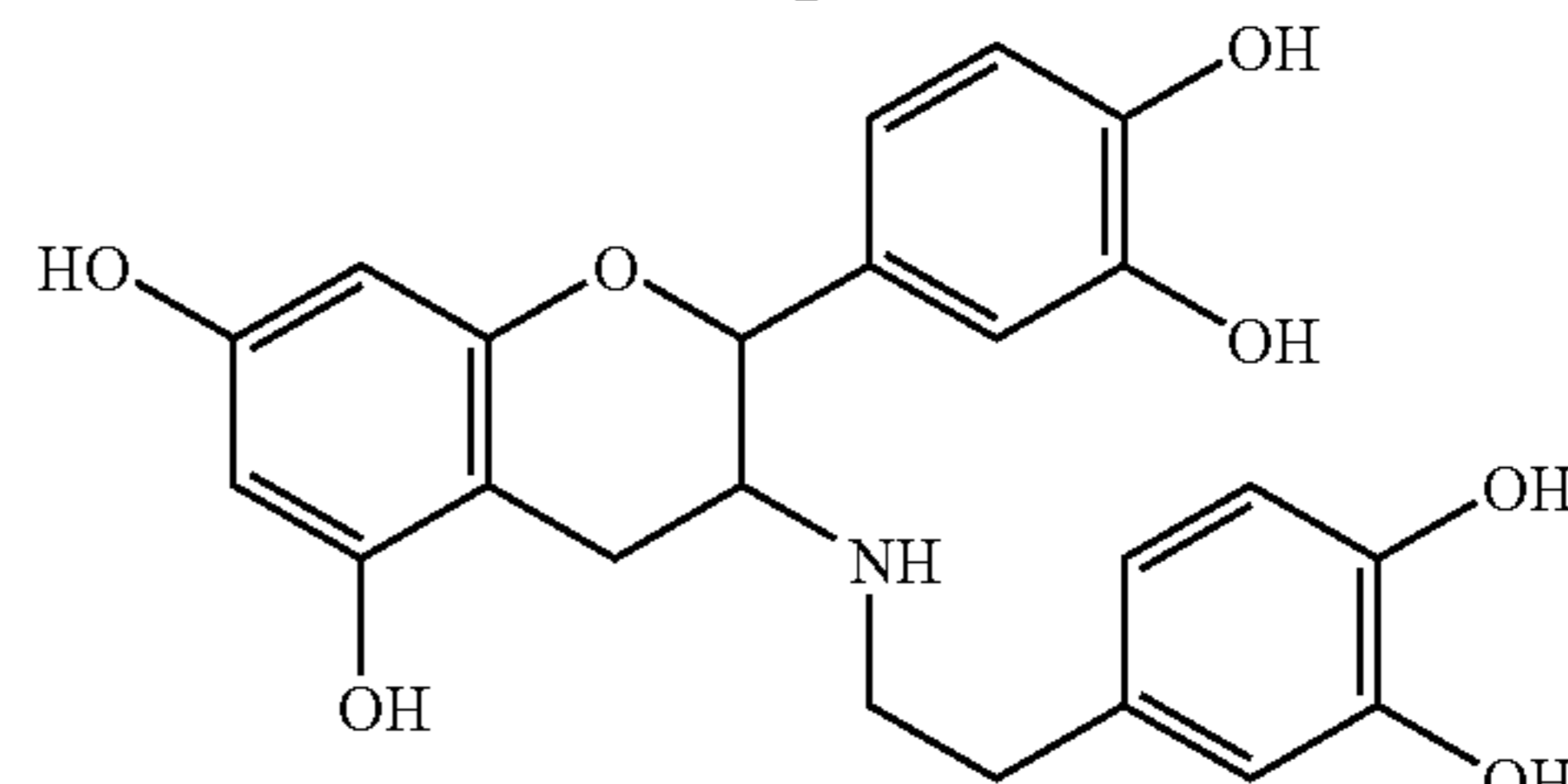
3-deoxy-3-(3,4-dihydroxyphenethyl)(-)amino-epicatechin
