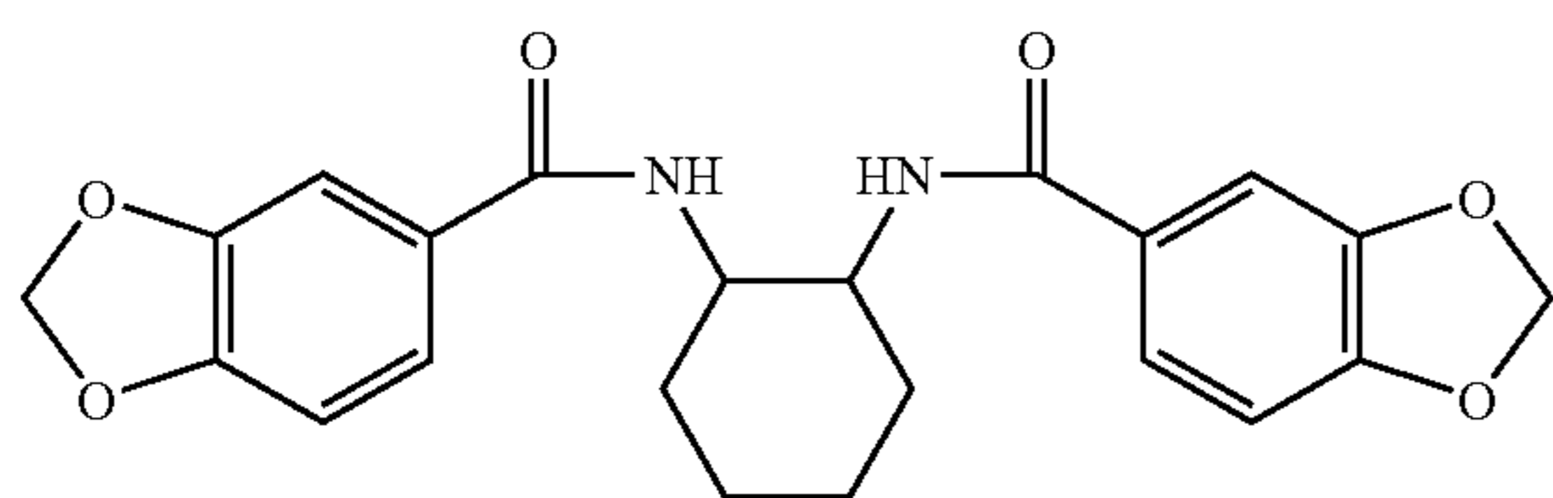
N,N'-bis(3,4-methylenedioxybenzoyl)-trans-diaminocyclohexane
