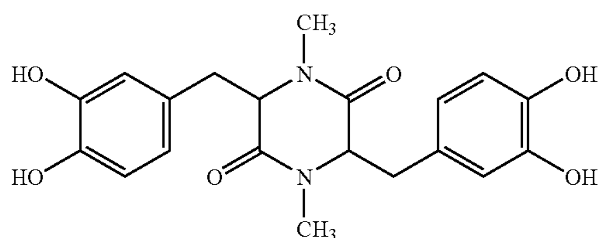
3,6-bis(3,4-dihydroxybenzylidene)-1,4-dimethyl-2,5-diketopiperazine
