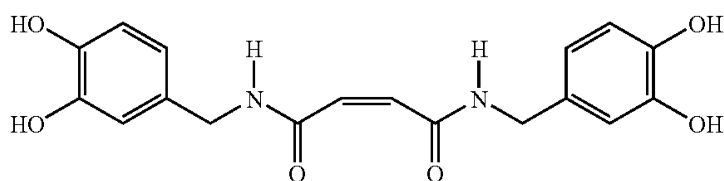
Maleic acid bis-(3,4-dihydroxybenzyl anilide)
