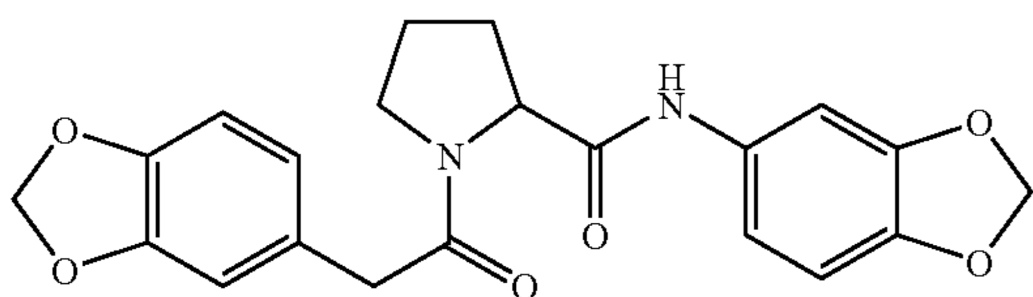
N-(3,4-methylenedioxyphenylacetyl)-proline-3,4-methylenedioxyanilide
