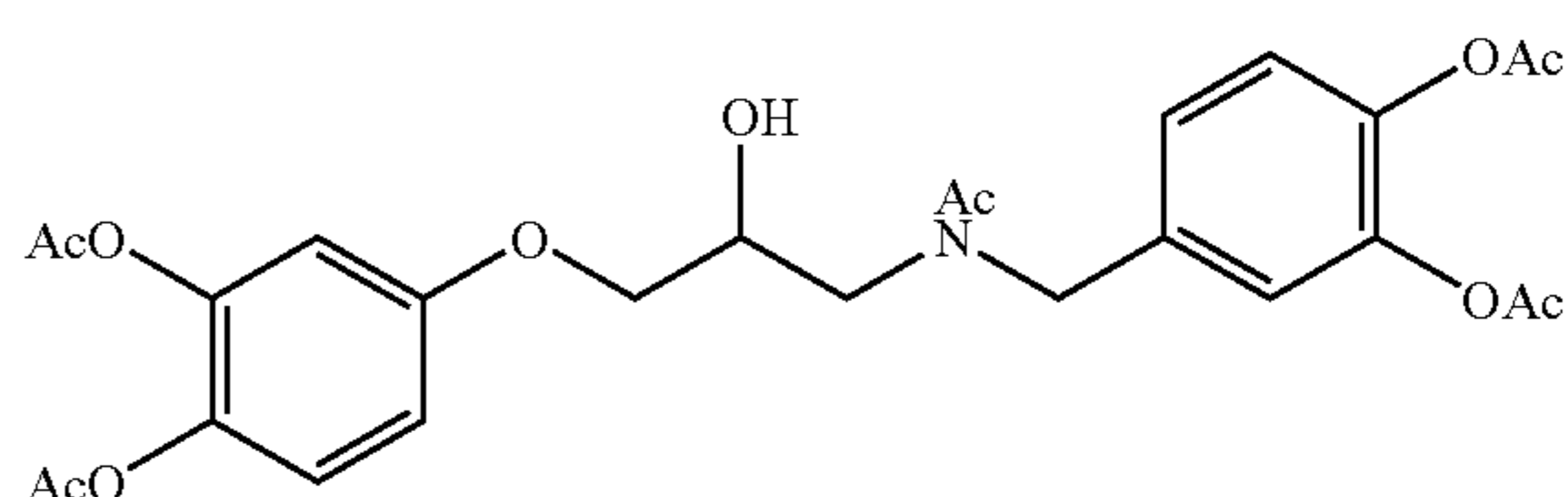
N-acetyl-N-(3,4-diacetoxybenzyl)-3-(3,4-diacetoxy(-)phenoxy)-2-hydroxypropylamine
