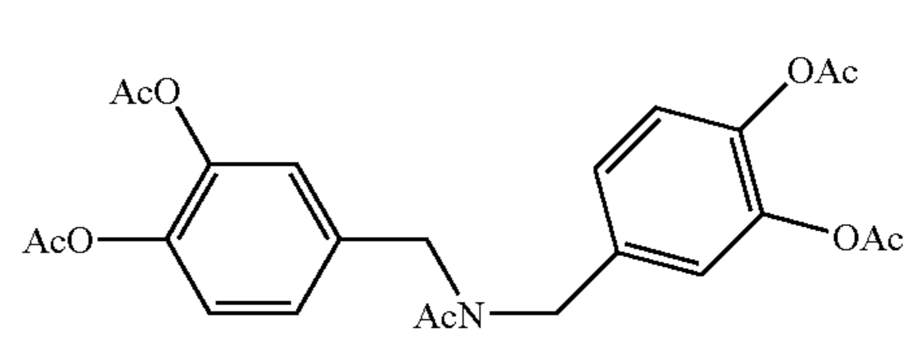
N-acetyl-bis-(3,4-diacetoxybenzyl)-amine
