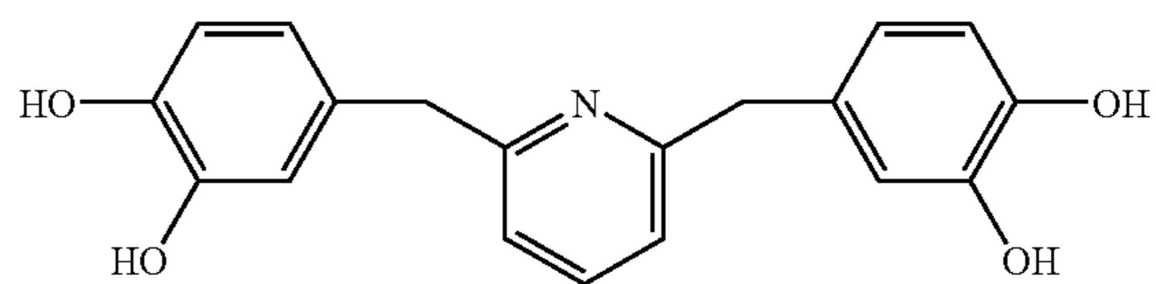
2,6-bis(3,4-dihydroxybenzyl)pyridine
