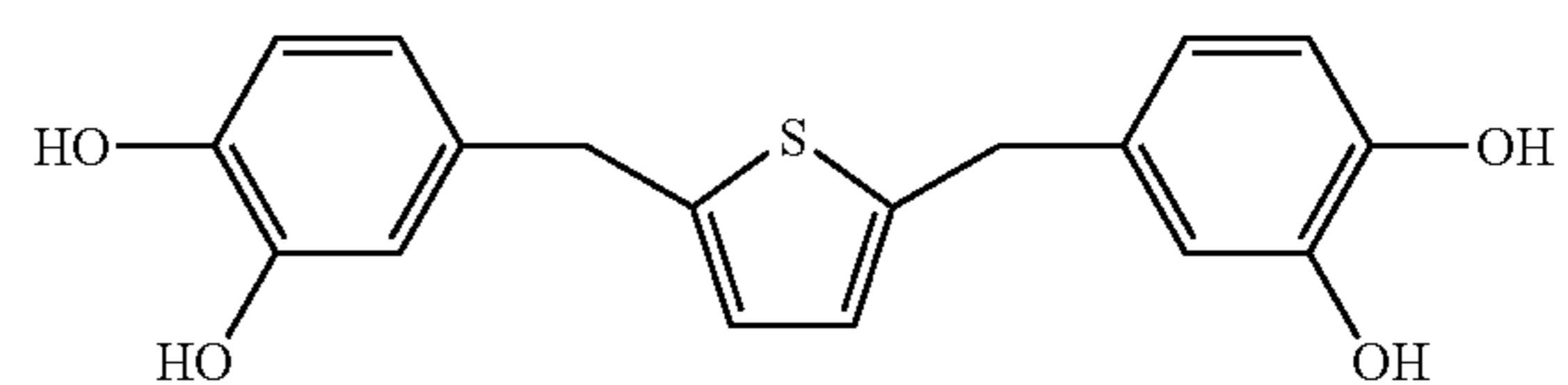
2,5-bis(3,4-dihydroxybenzyl)thiophene
