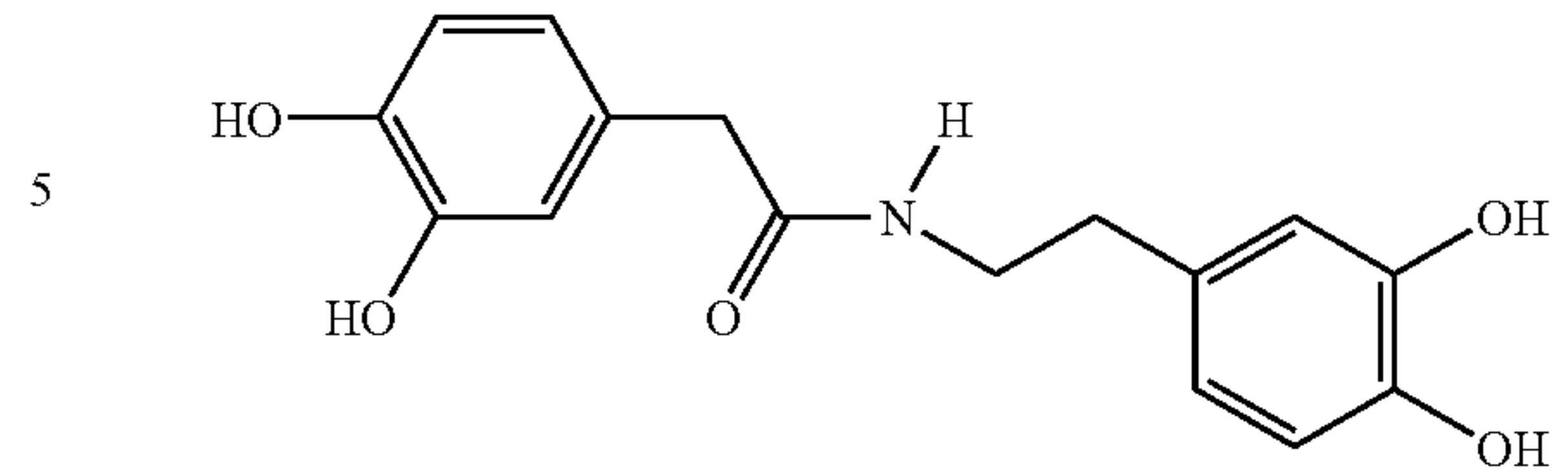
3,4-dihydroxyphenylacetic acid 3,4-dihydroxyphenethylamide
