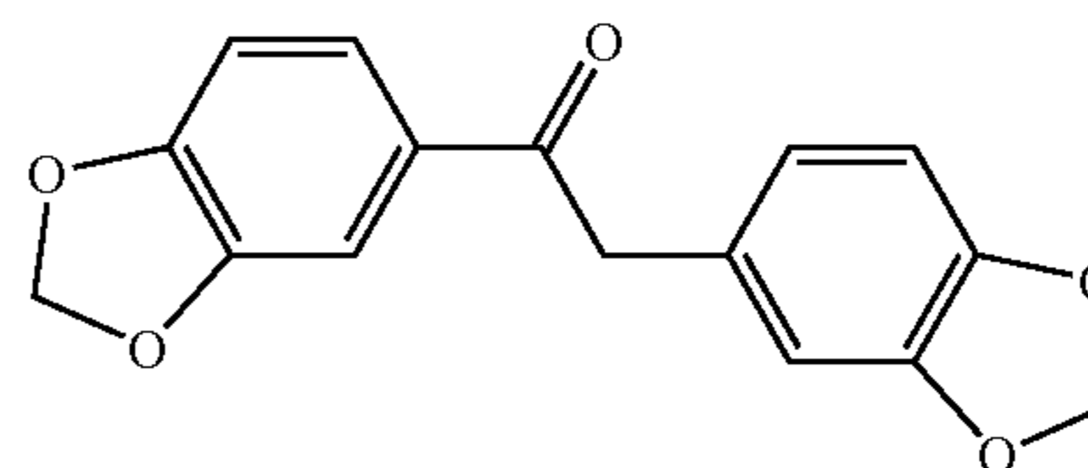
bis(3,4-methylenedioxy)desoxybenzoil
