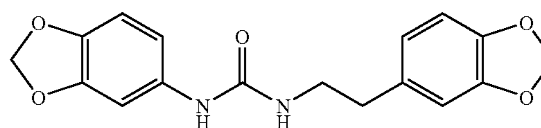
1-(3,4-methylenedioxyphenyl)-3-(3,4-methylenedioxyphenethyl) urea
