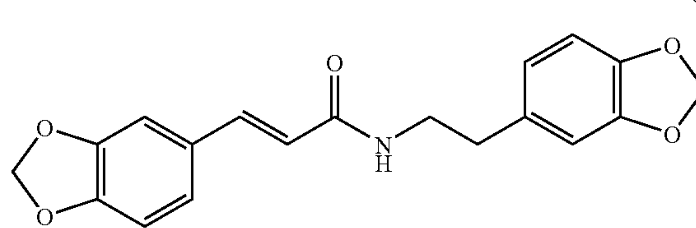
3,4-methylenedioxycinnamic acid 3,4-methylenedioxyphenethylamide
