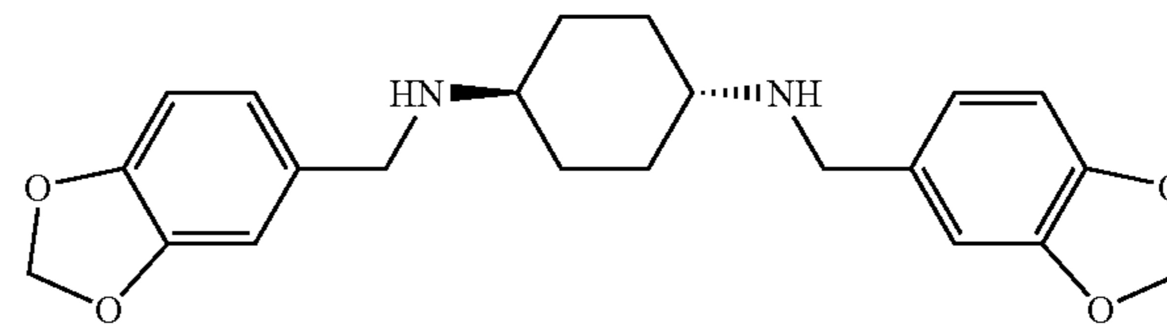
N,N'-bis(3,4-methylenedioxybenzyl)trans- 1,4-diaminocyclohexane
