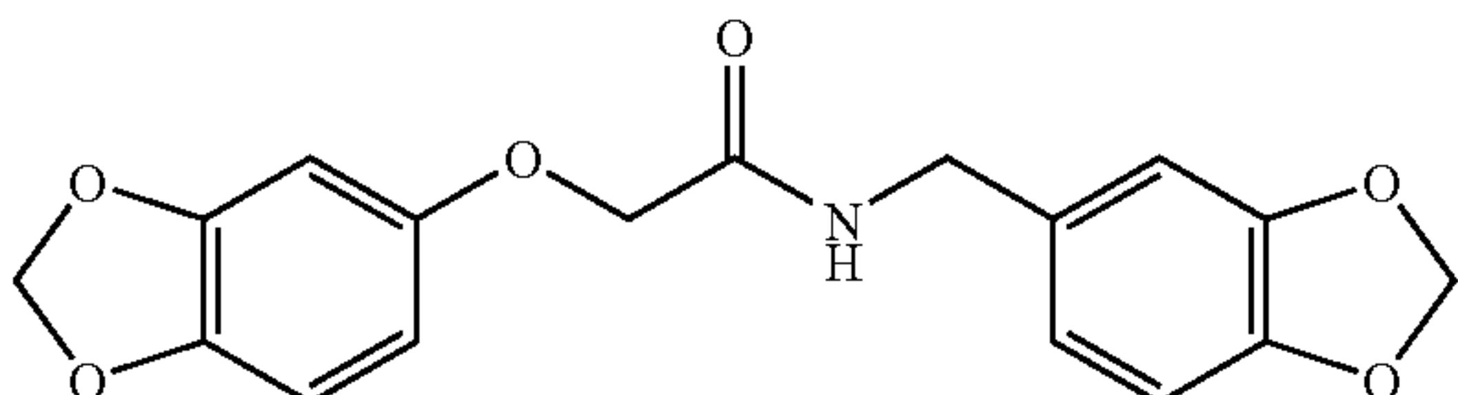
3,4-methylenedioxyphenoxyacetic acid 3,4-methylenedioxybenzylamide
