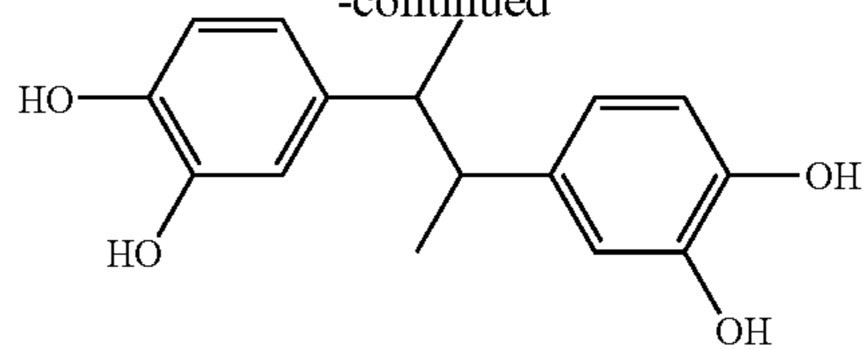
2,3-bis(3,4-dihydroxyphenyl)butane
