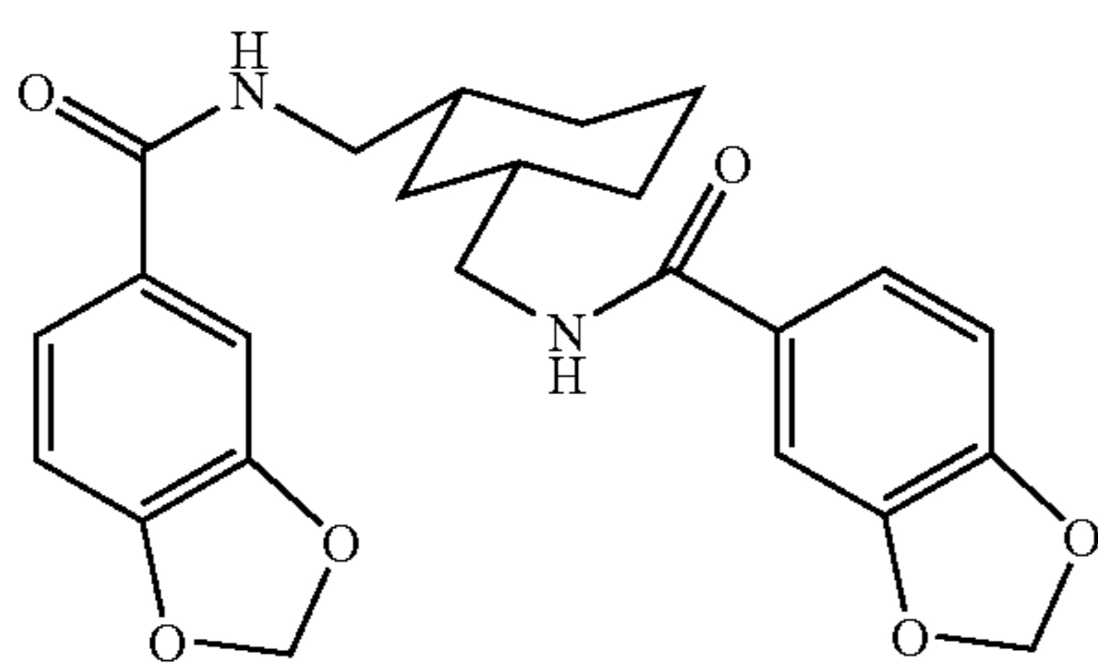
N,N'-bis(3,4-methylenedioxybenzoyl)-cis-1,3-bis-aminomethylcyclohexane
