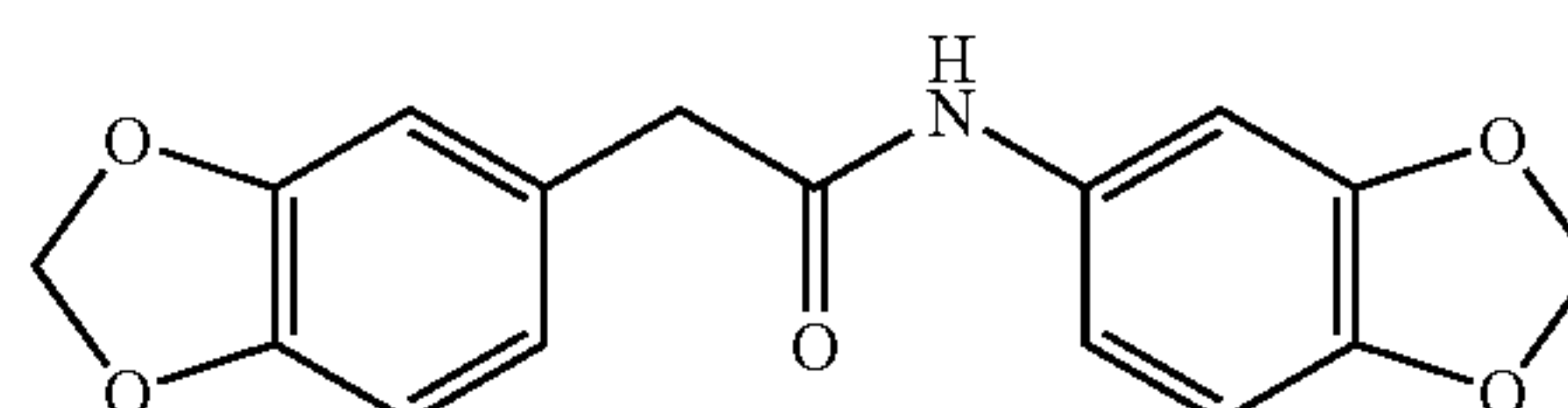
3,4-methylenedioxyphenylacetic acid 3,4-methylenedioxyanilide
