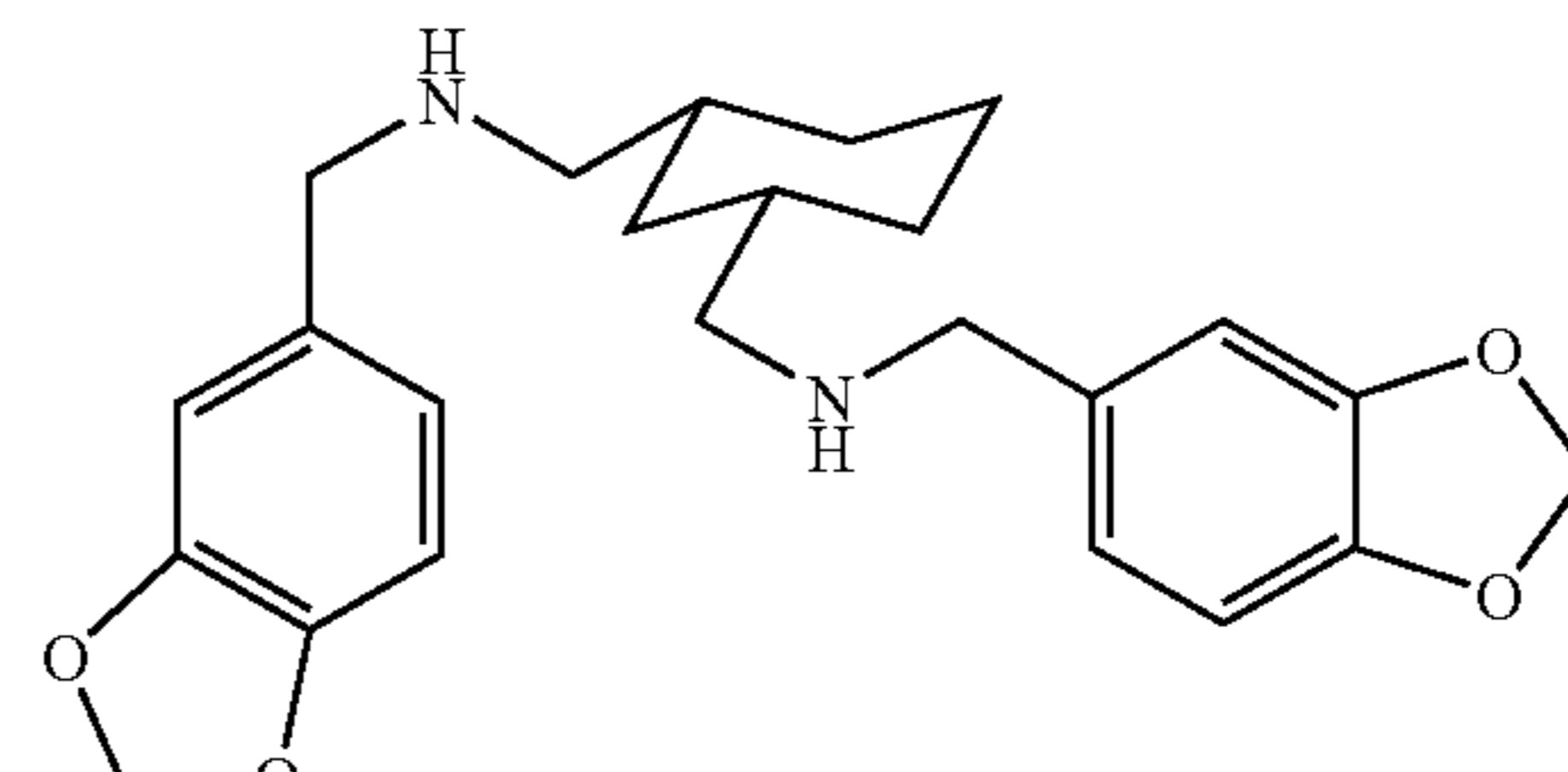
N,N'-bis(3,4-methylenedioxybenzyl)-cis- 1,3-bis-aminomethylcyclohexane
