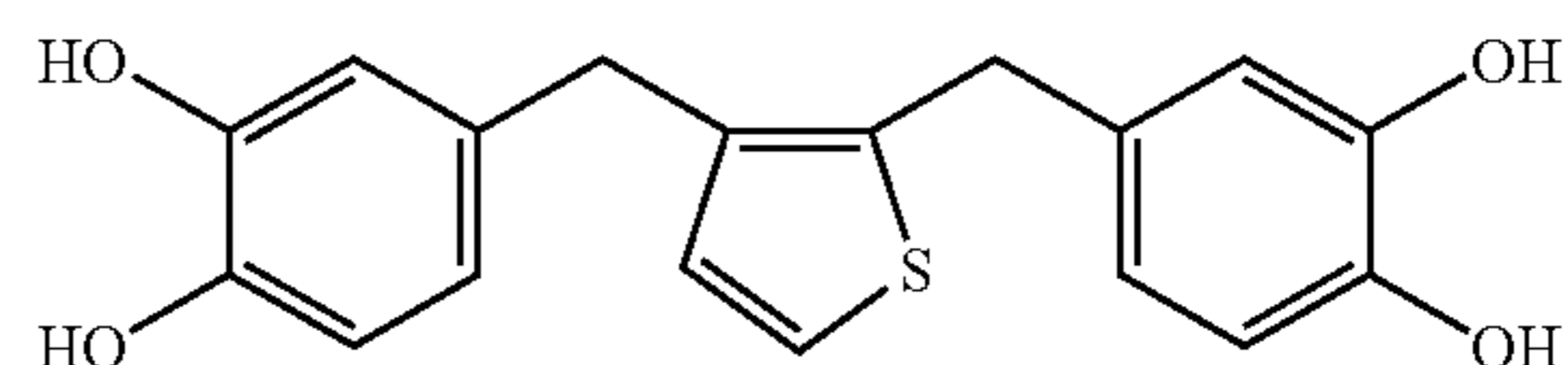
2,3-bis(3,4-dihydroxybenzyl)thiophene
