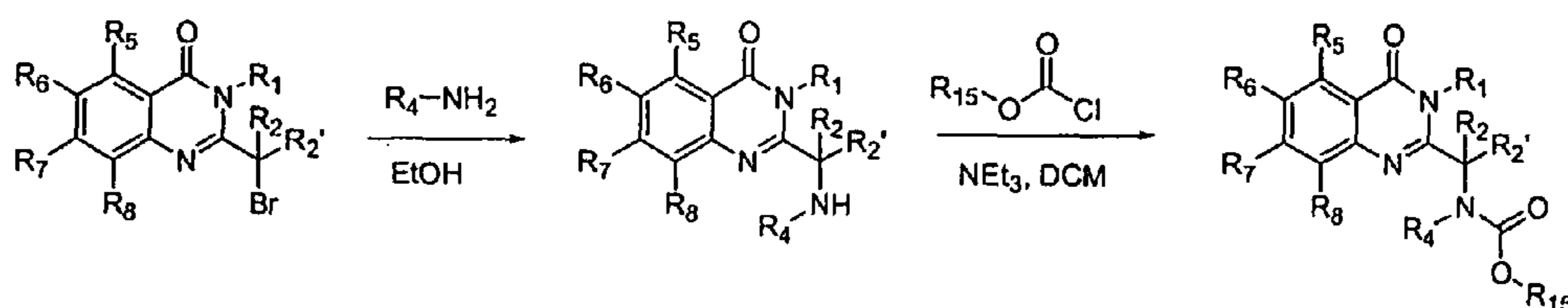
Figure 5c: Urea Synthesis
