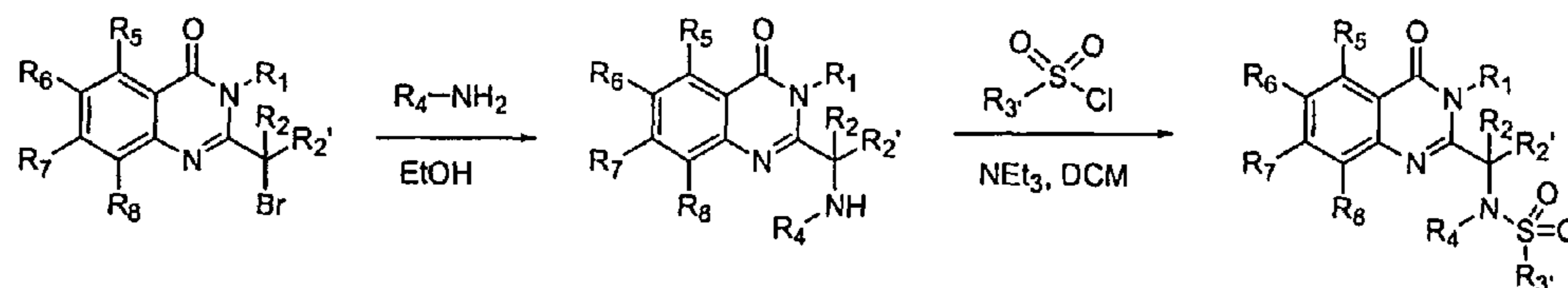
Figure 5a: Sulfonamide Synthesis
