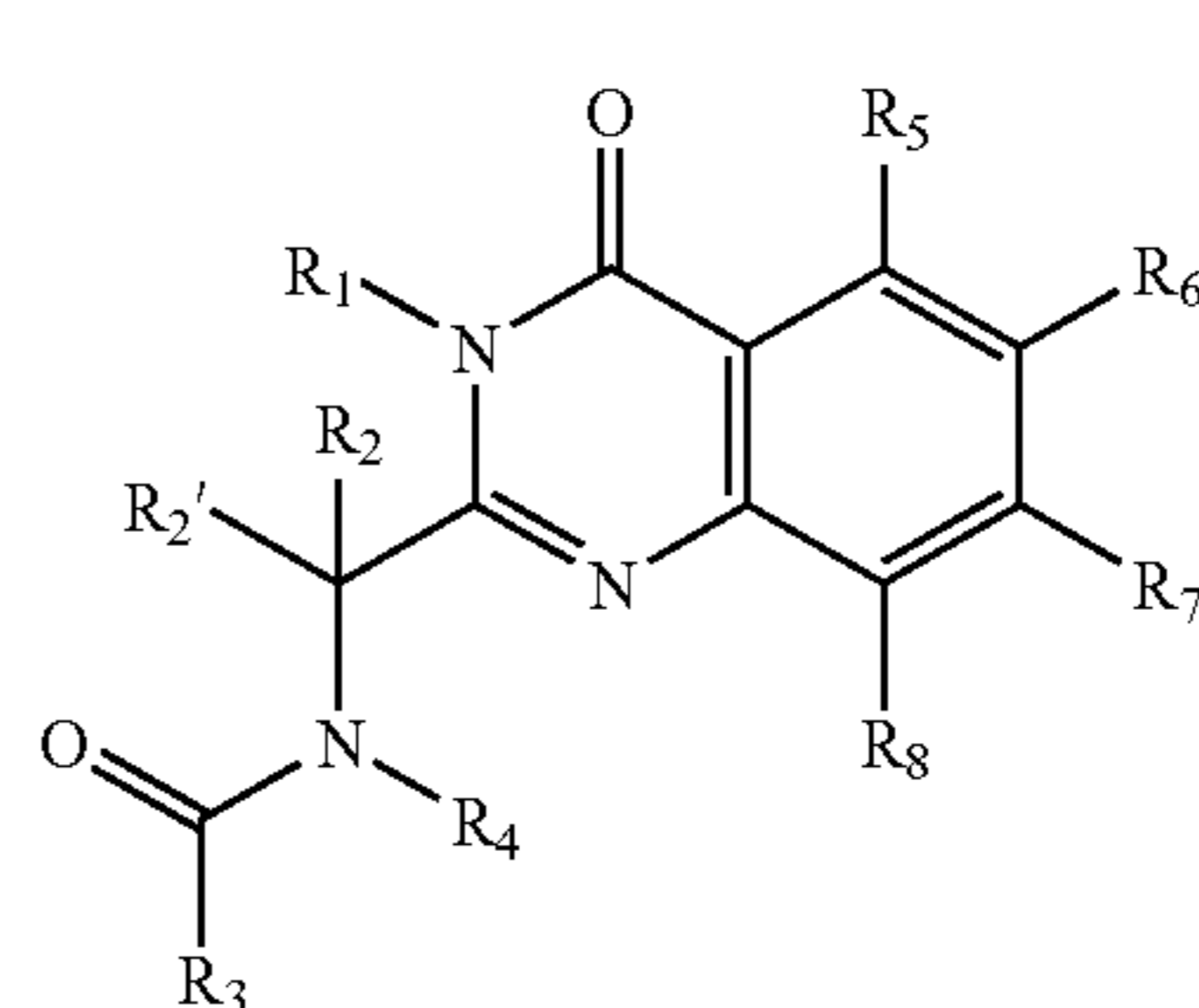
quinazolinone sulfonamides of formula 1b
