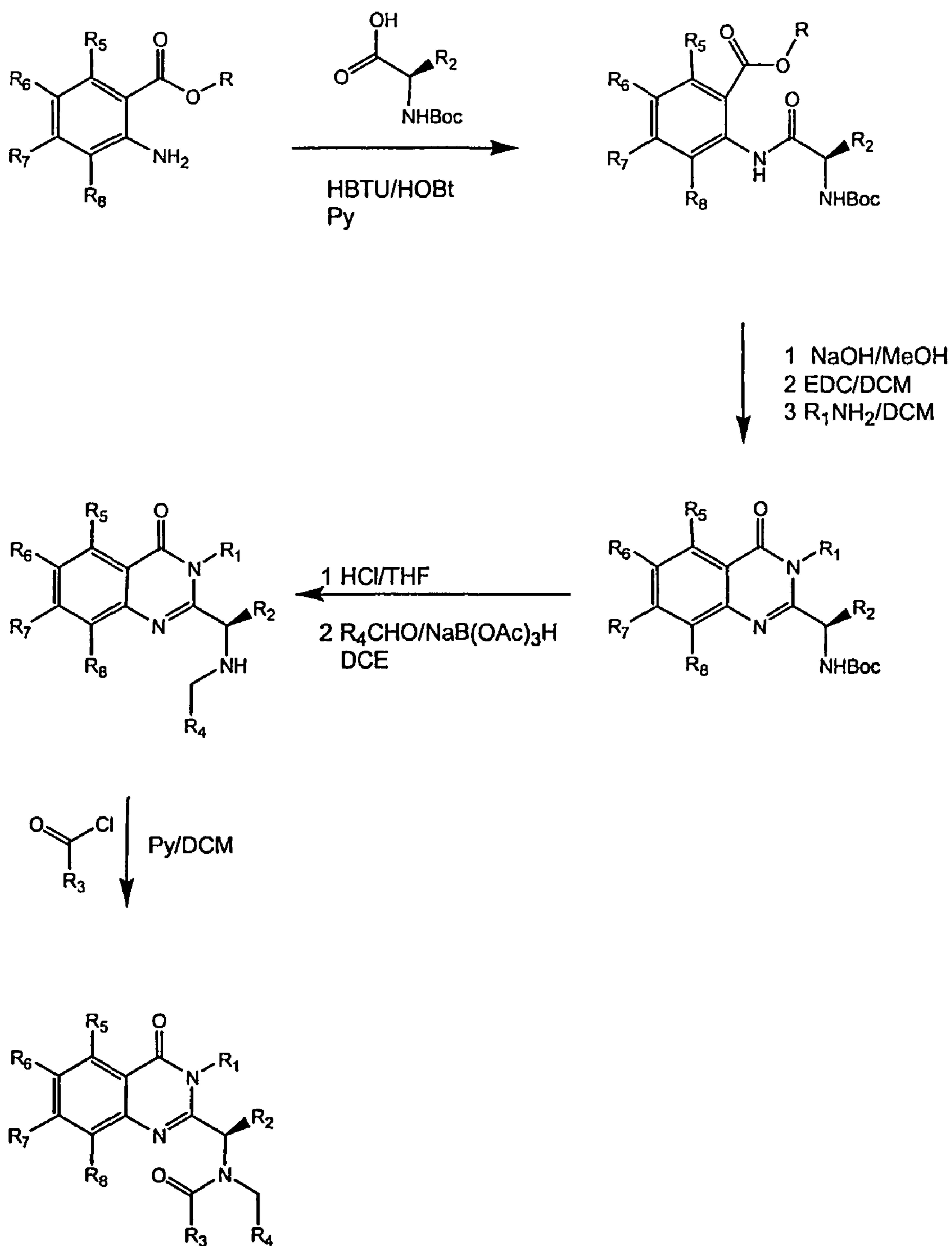
Figure 4: Asymmetric Synthesis
