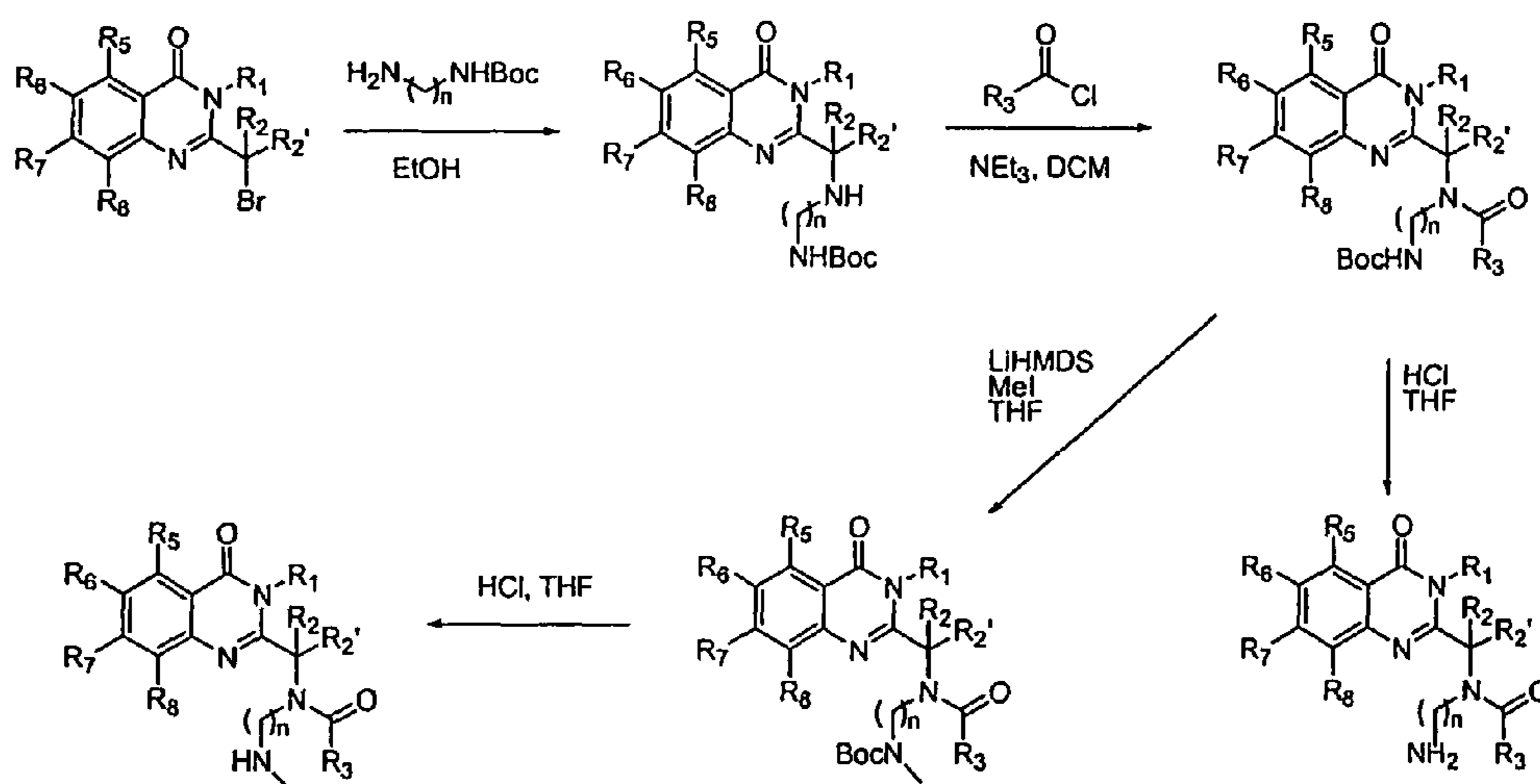
15 Figure 5d: Primary and Secondary Amine R4 Synthesis
