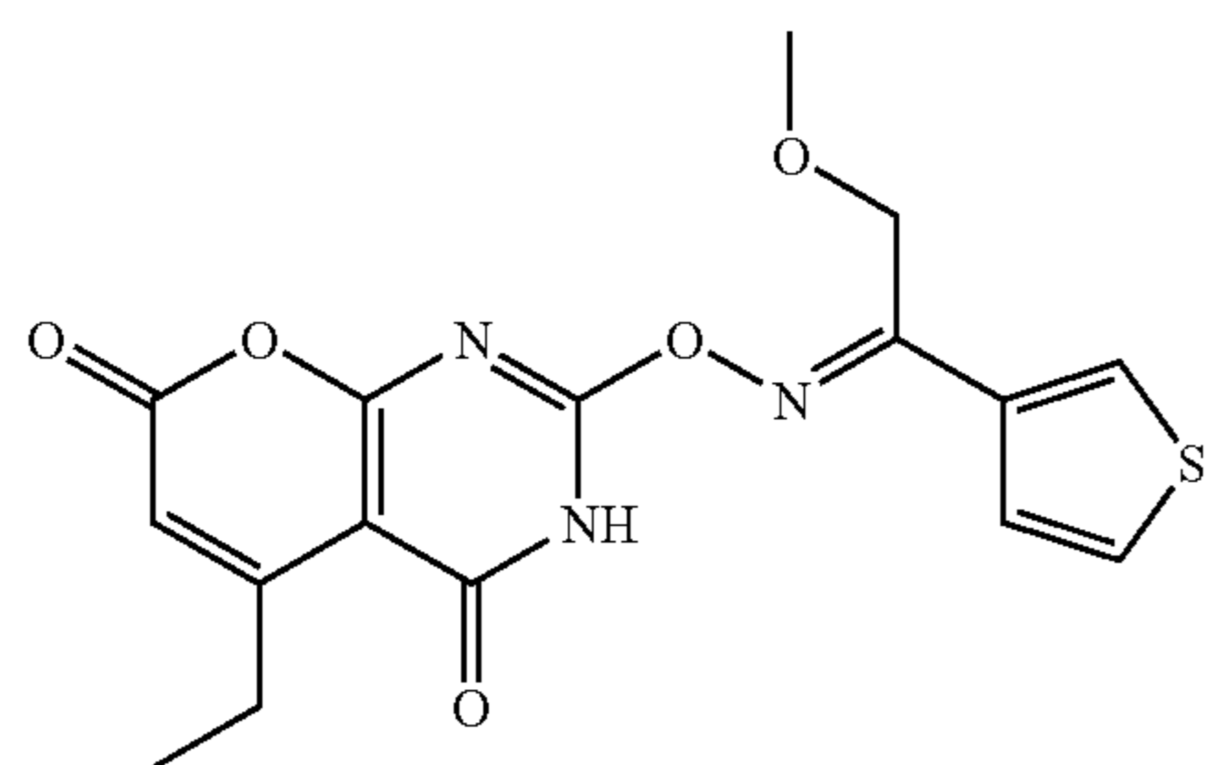
Compound 44:
