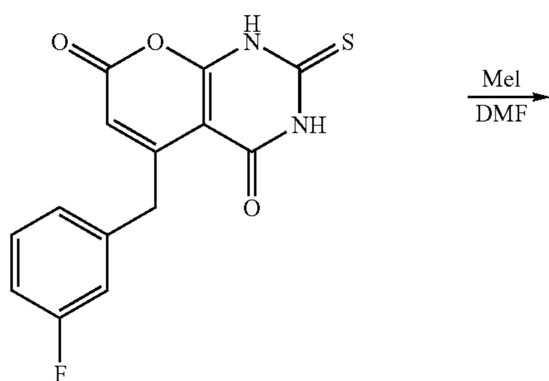
Compound 101b
