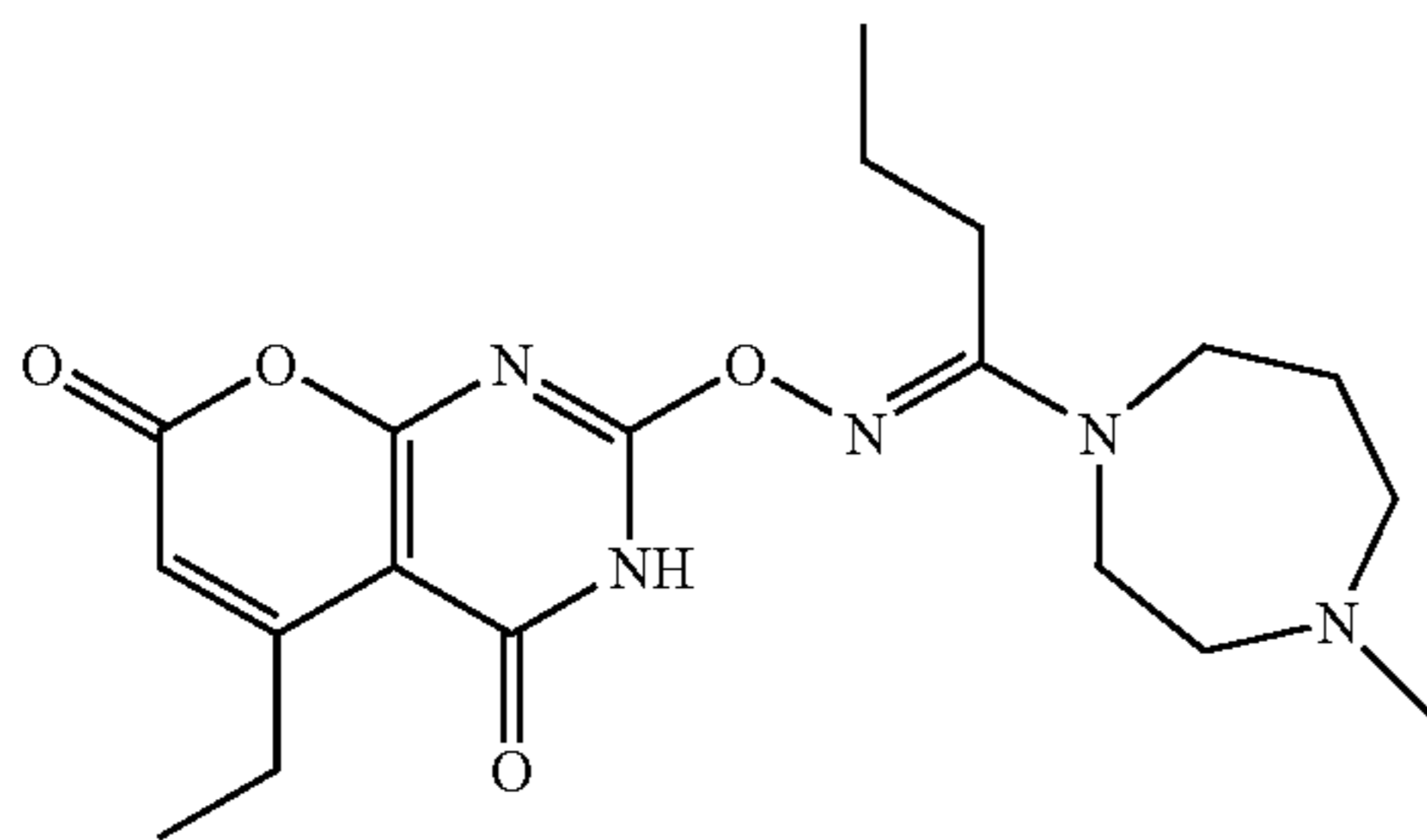
Compound 18:
