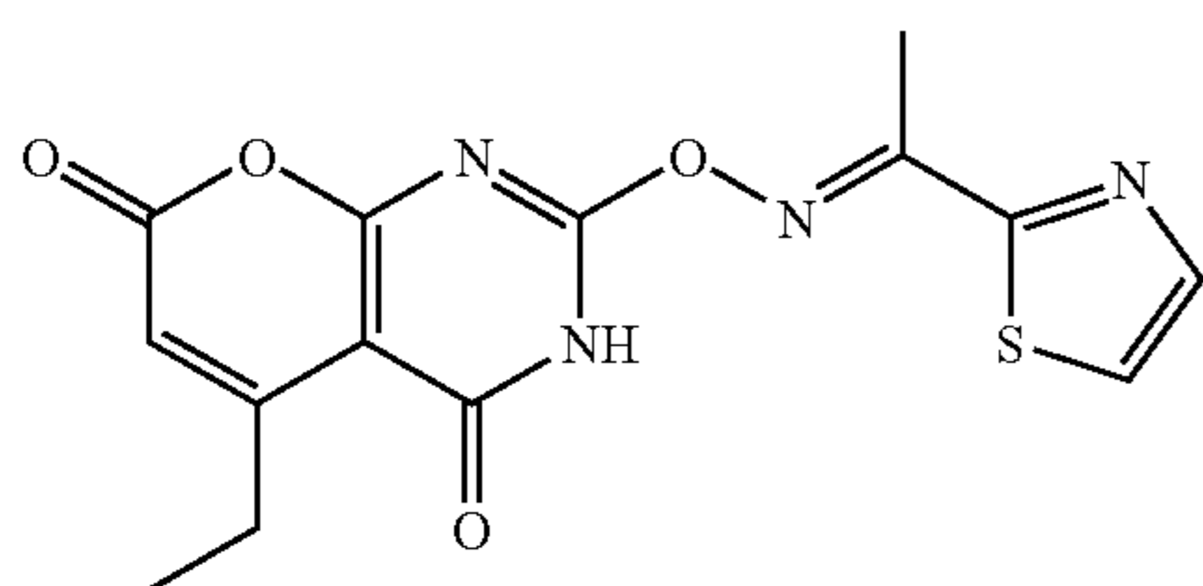
40, Isomers A and B
