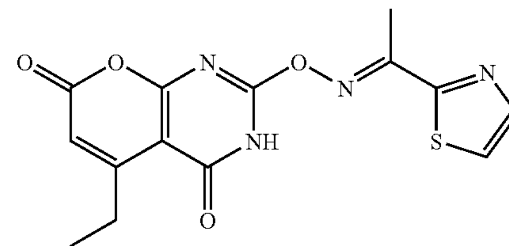
Compound 41, isomer A
