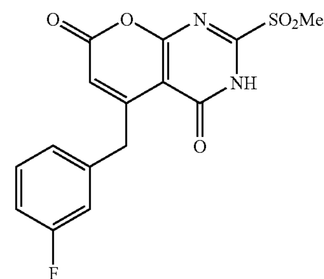
Compound 101d
