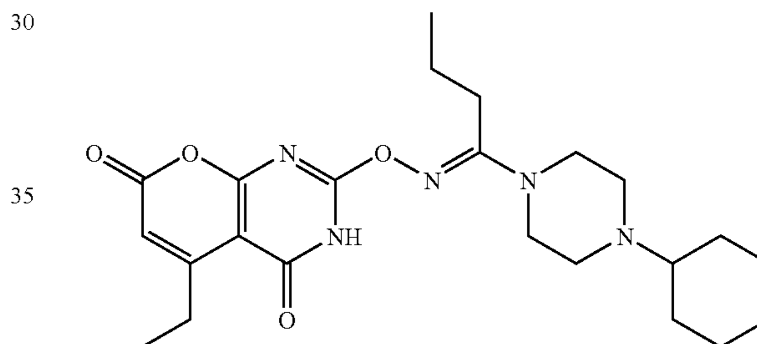
Compound 14:
