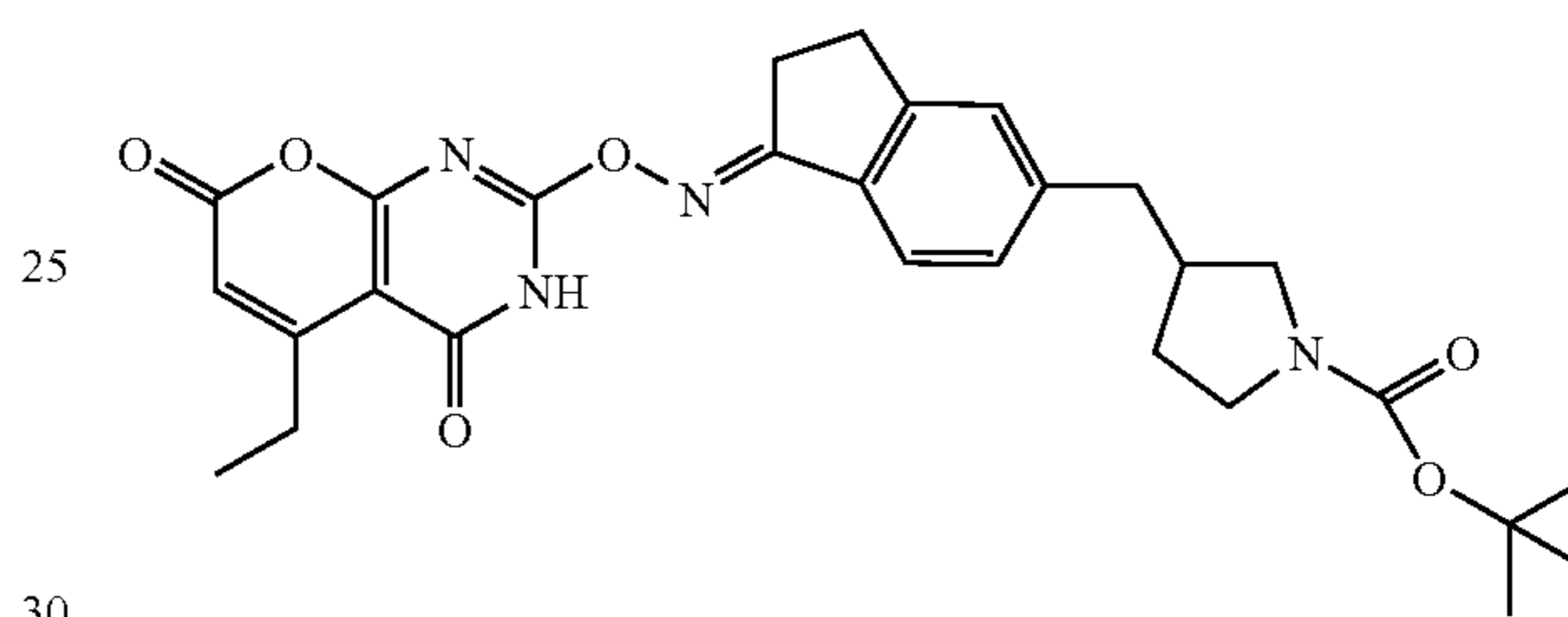
Compound 47:
