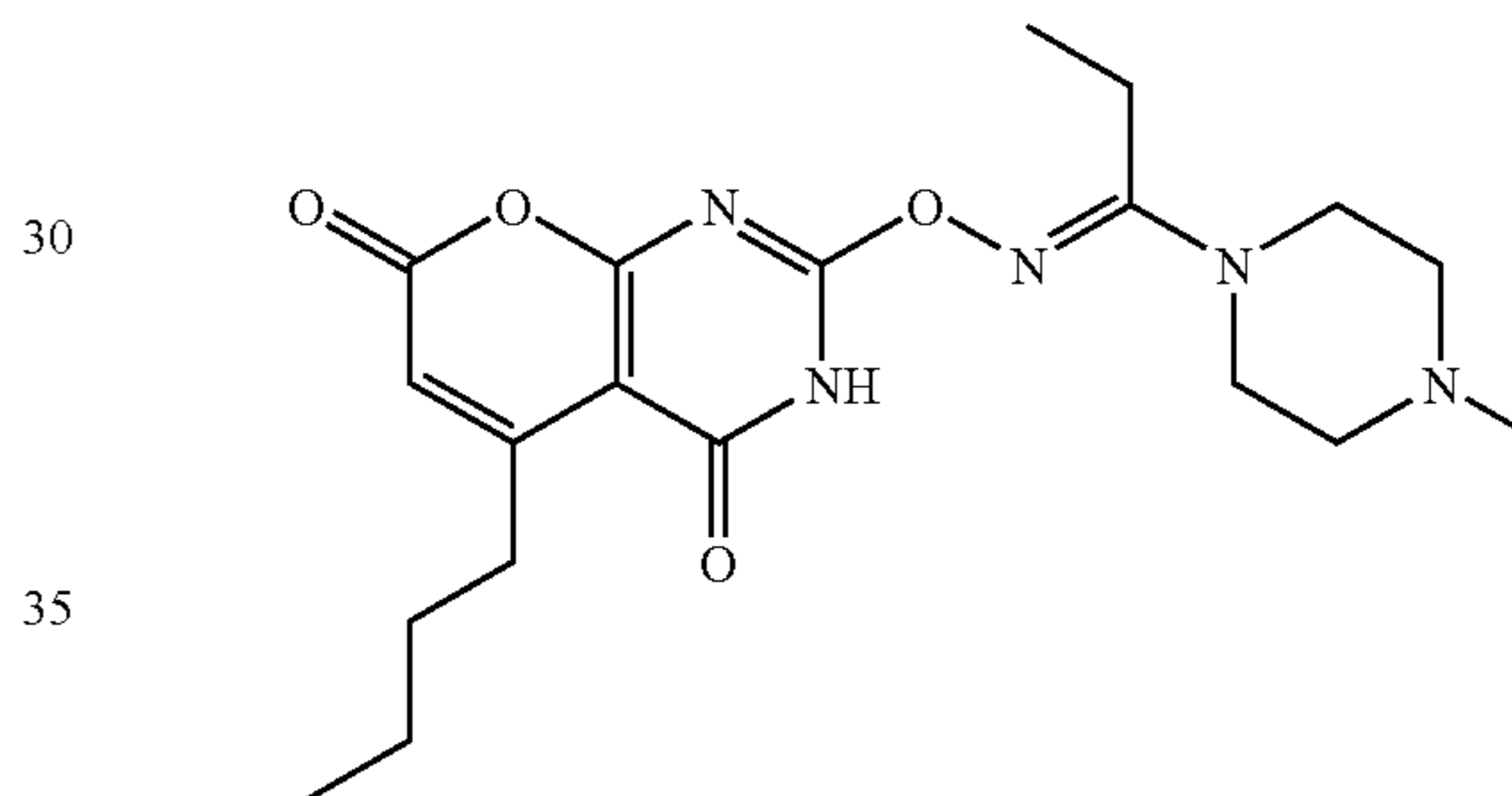
Compound 20:
