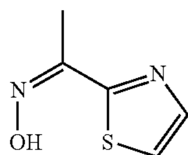
40b, isomer B
