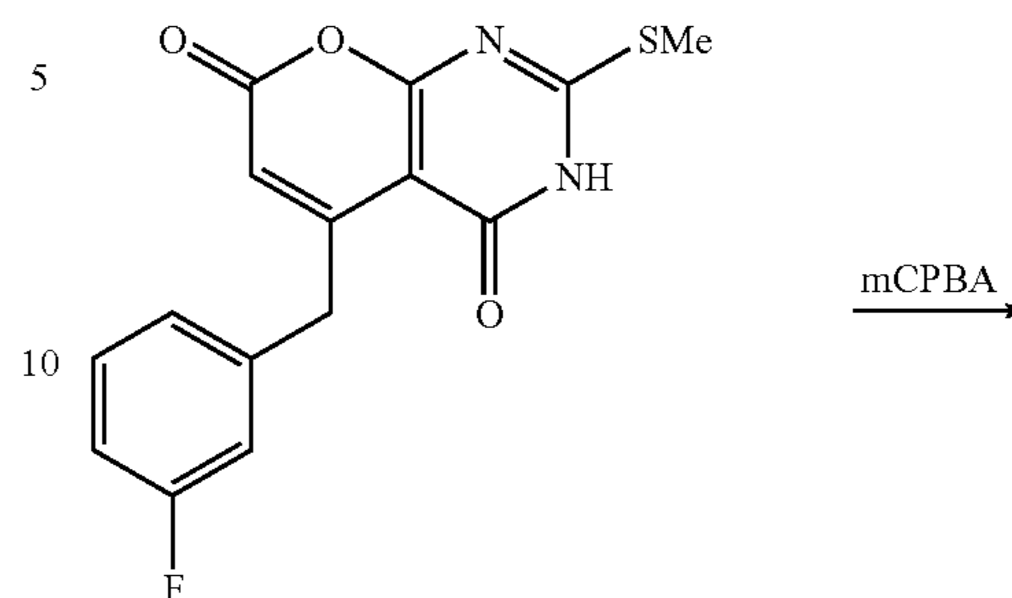
Compound 101c
