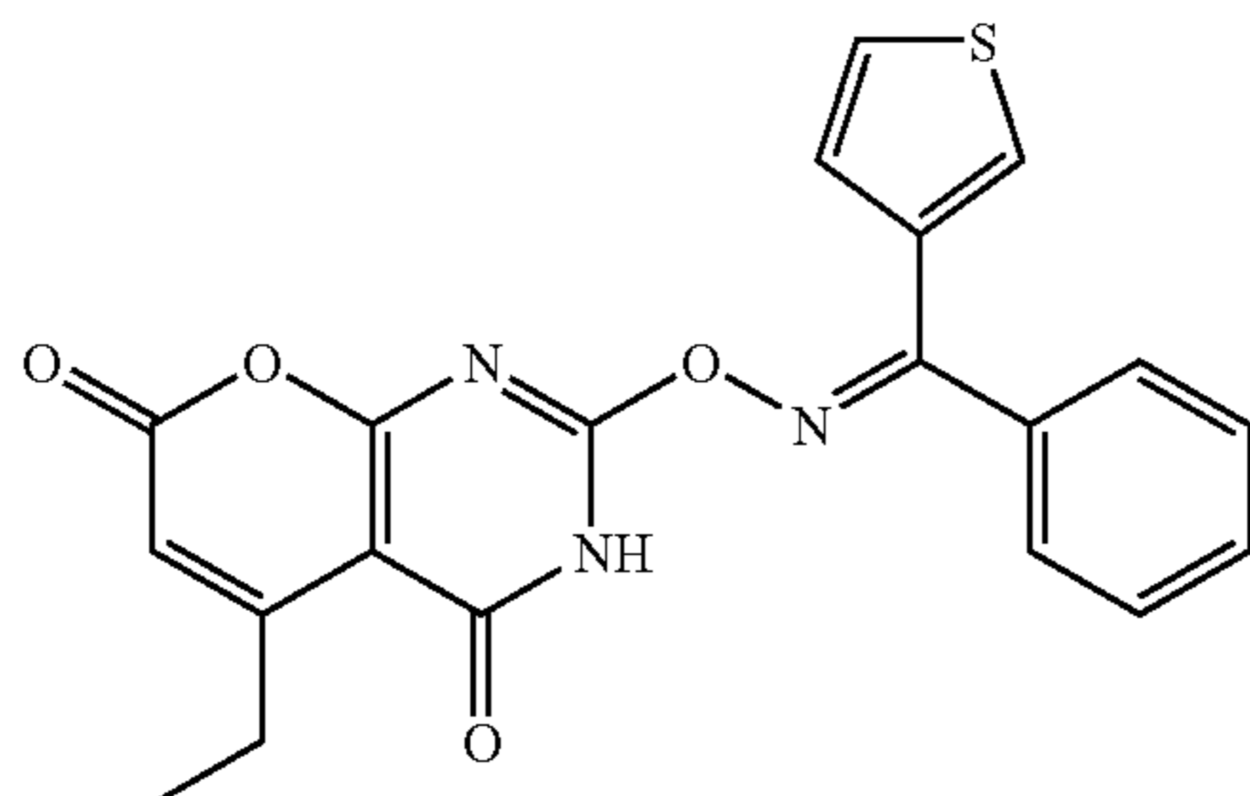
Compound 43:
