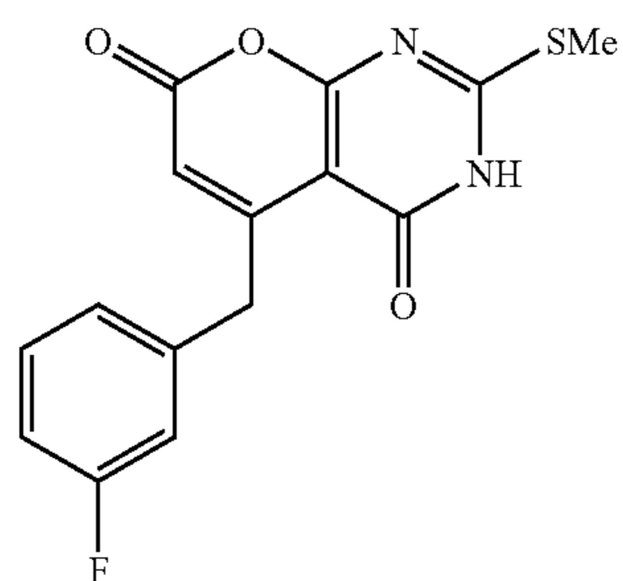
Compound 101c
