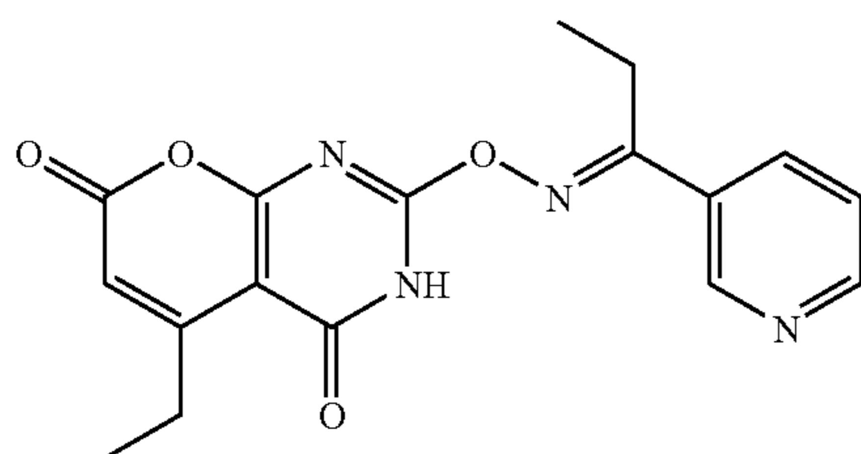
Compound 45:
