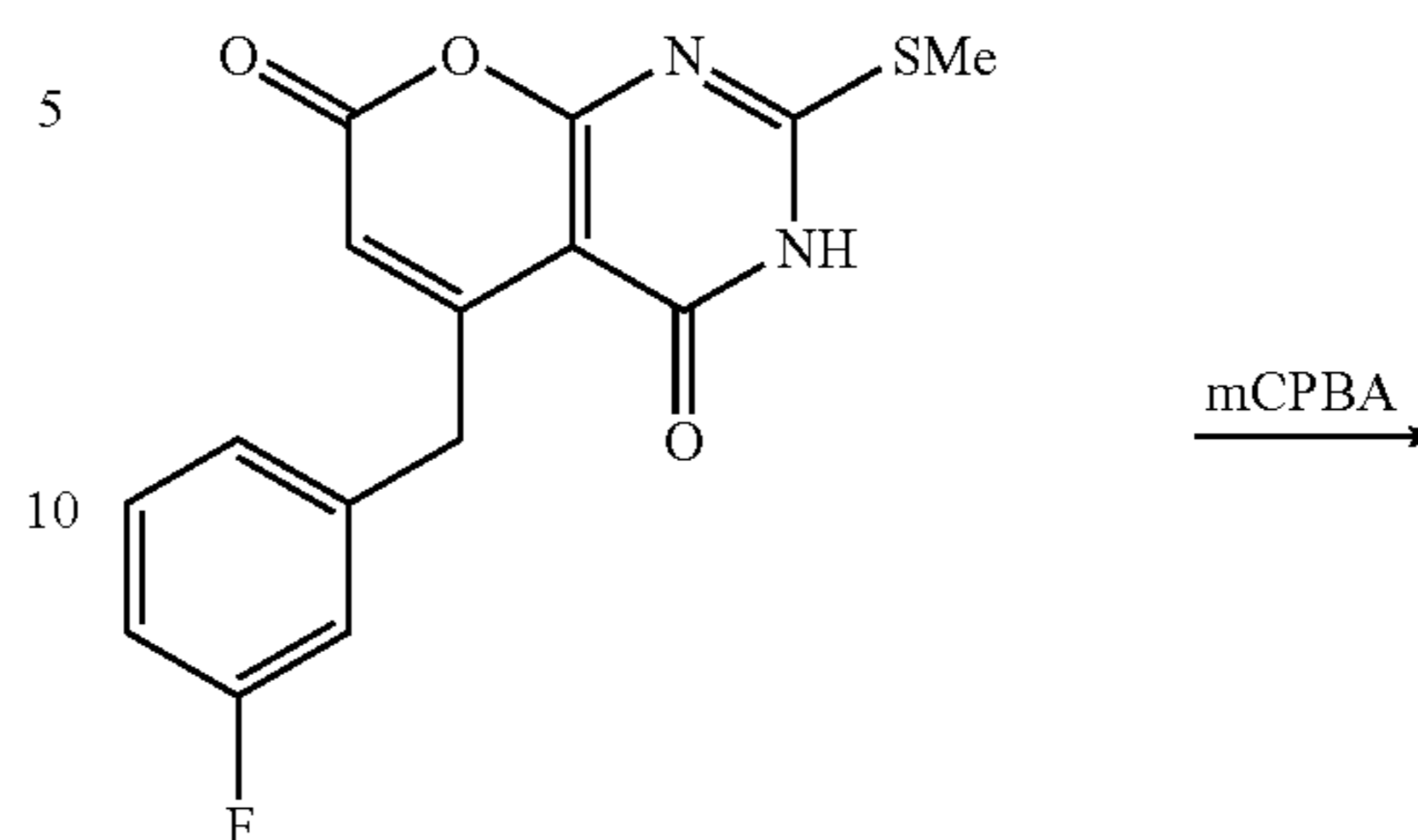
Compound 101c
