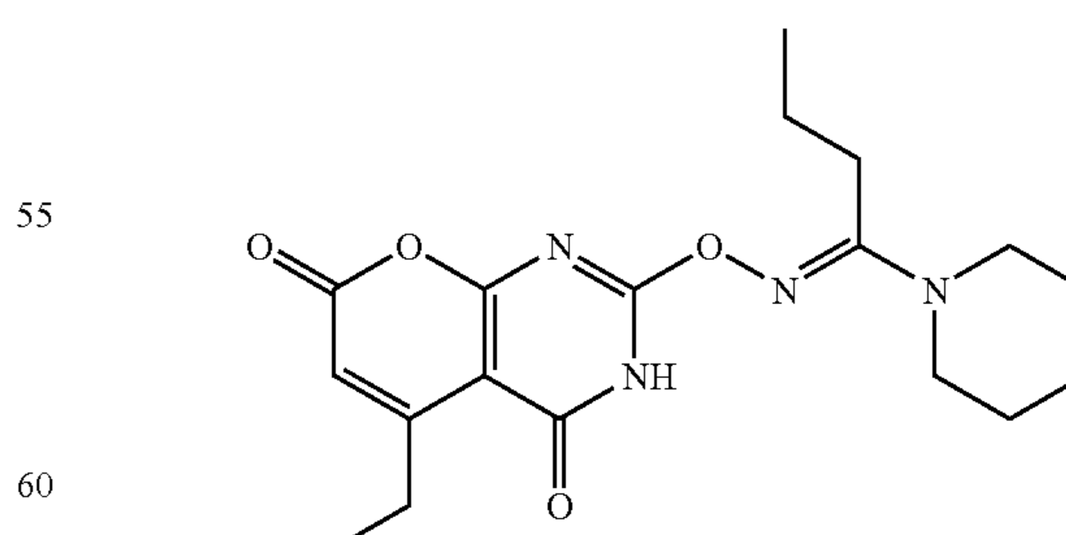
Compound 15:
