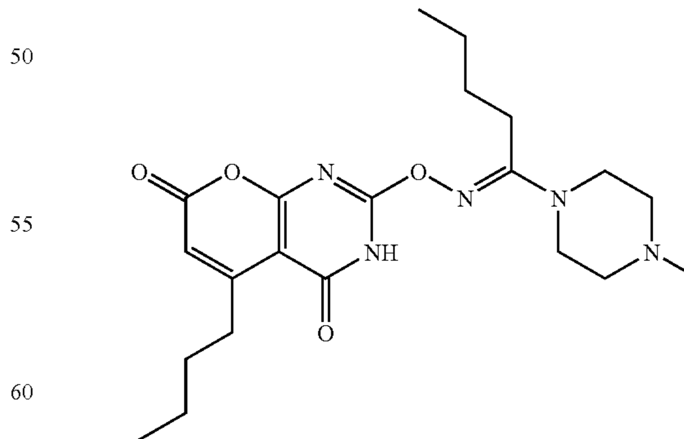
Compound 21:
