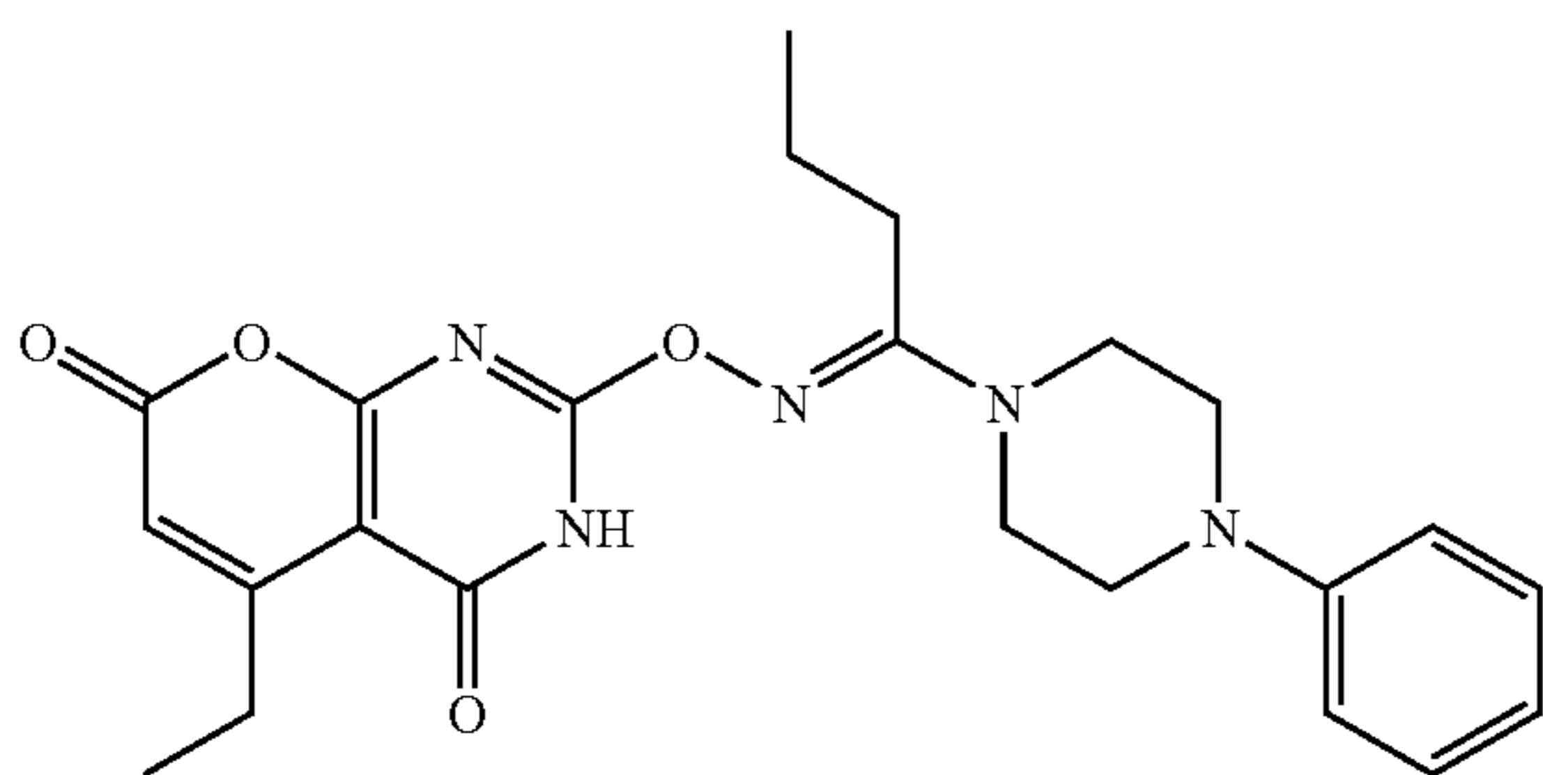
Compound 11:
