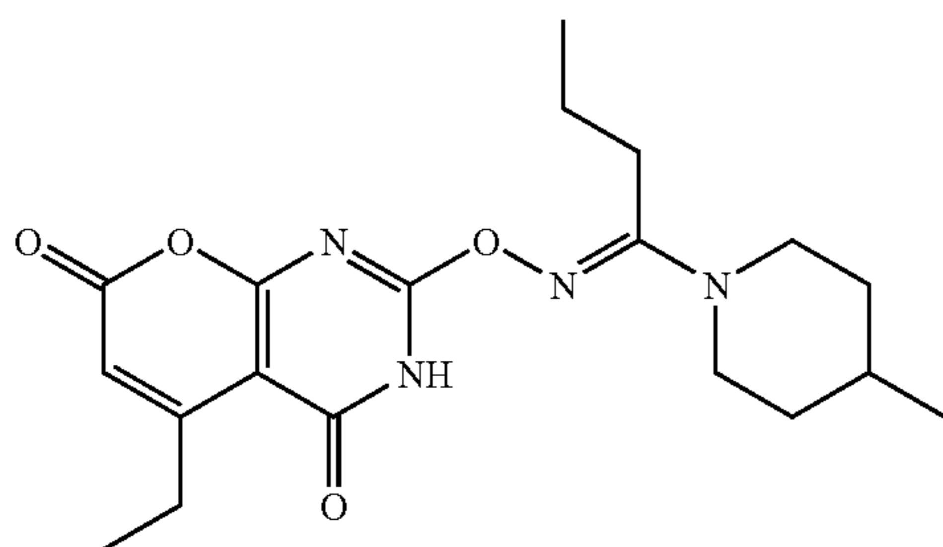
Compound 16:
