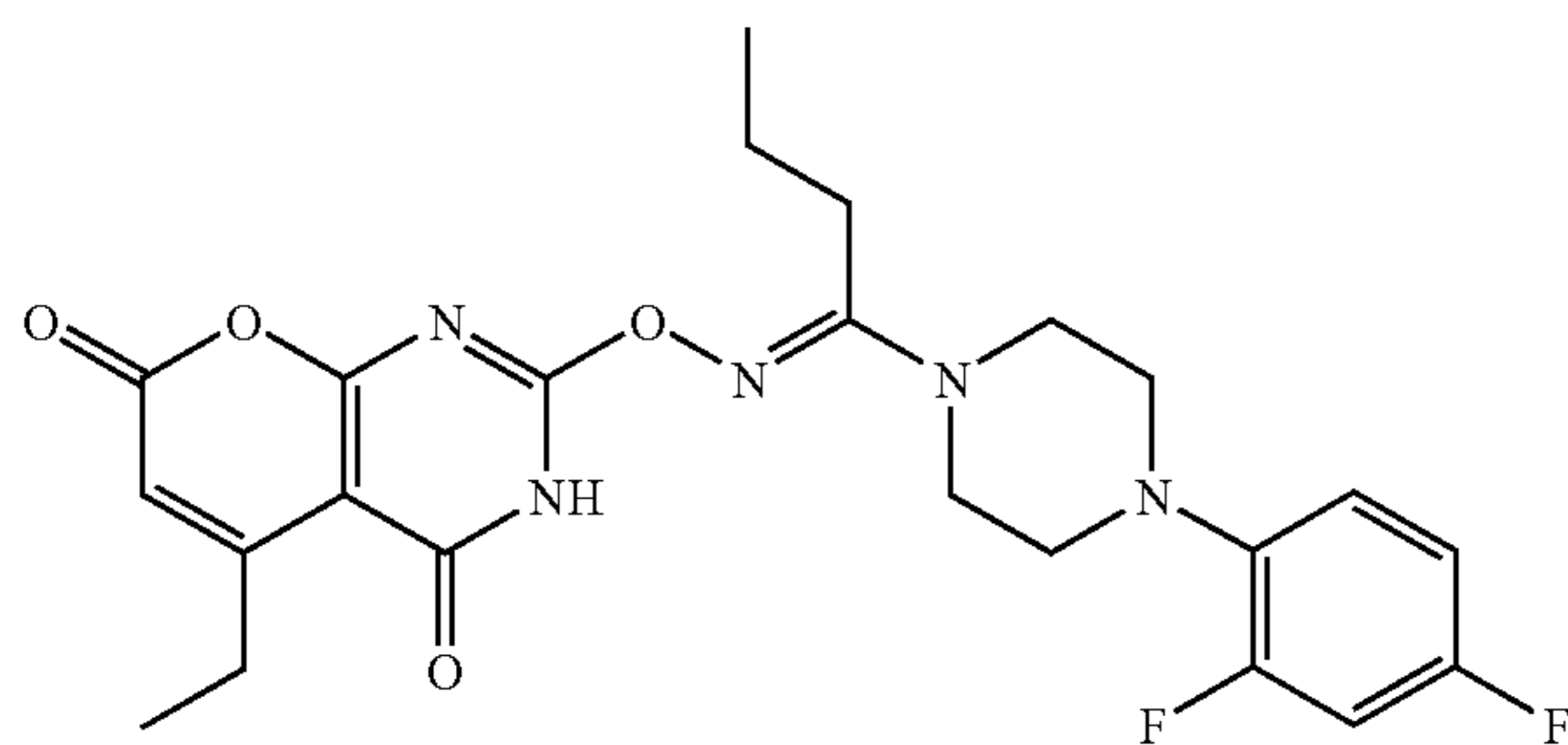
Compound 10:
