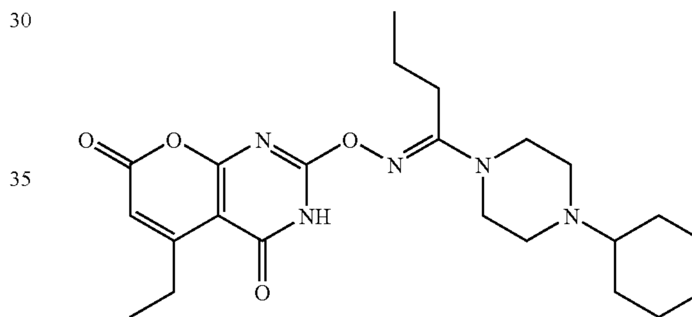
Compound 14:
