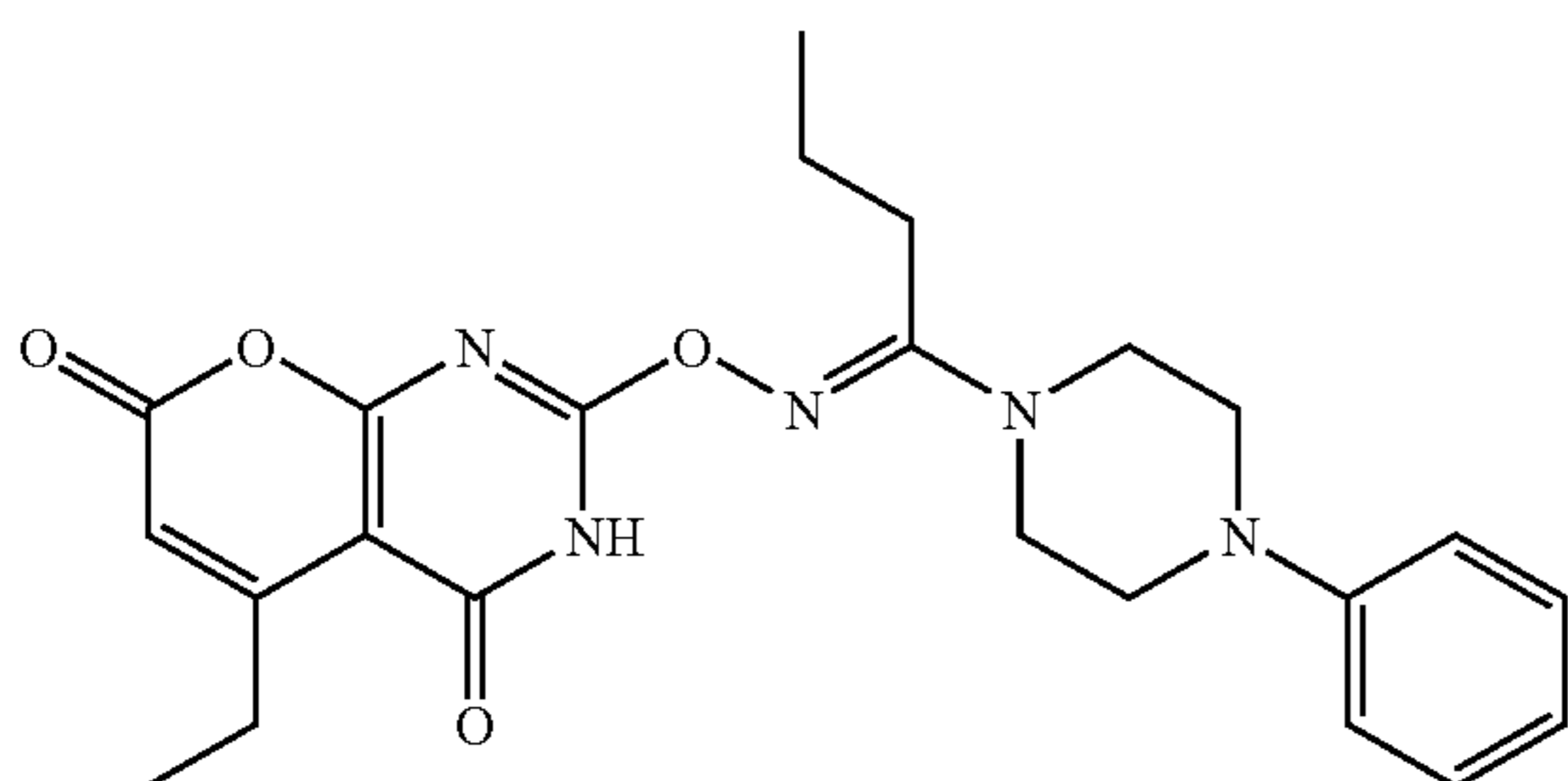
Compound 11:
