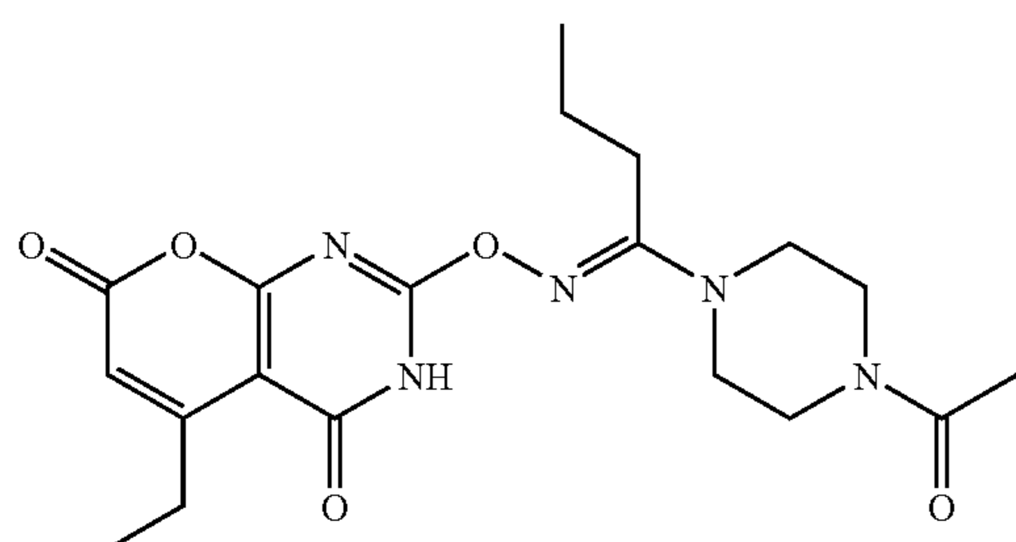
Compound 12:
