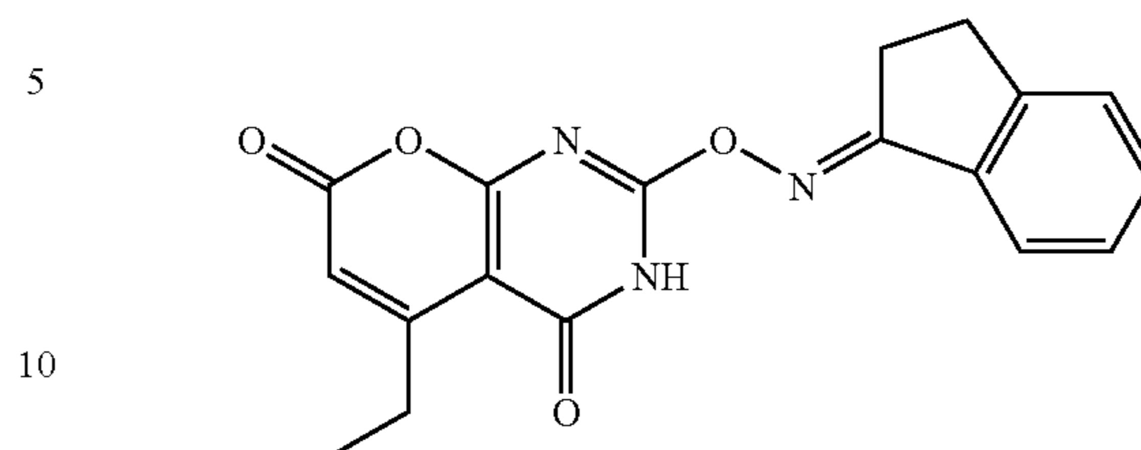
Compound 46:
