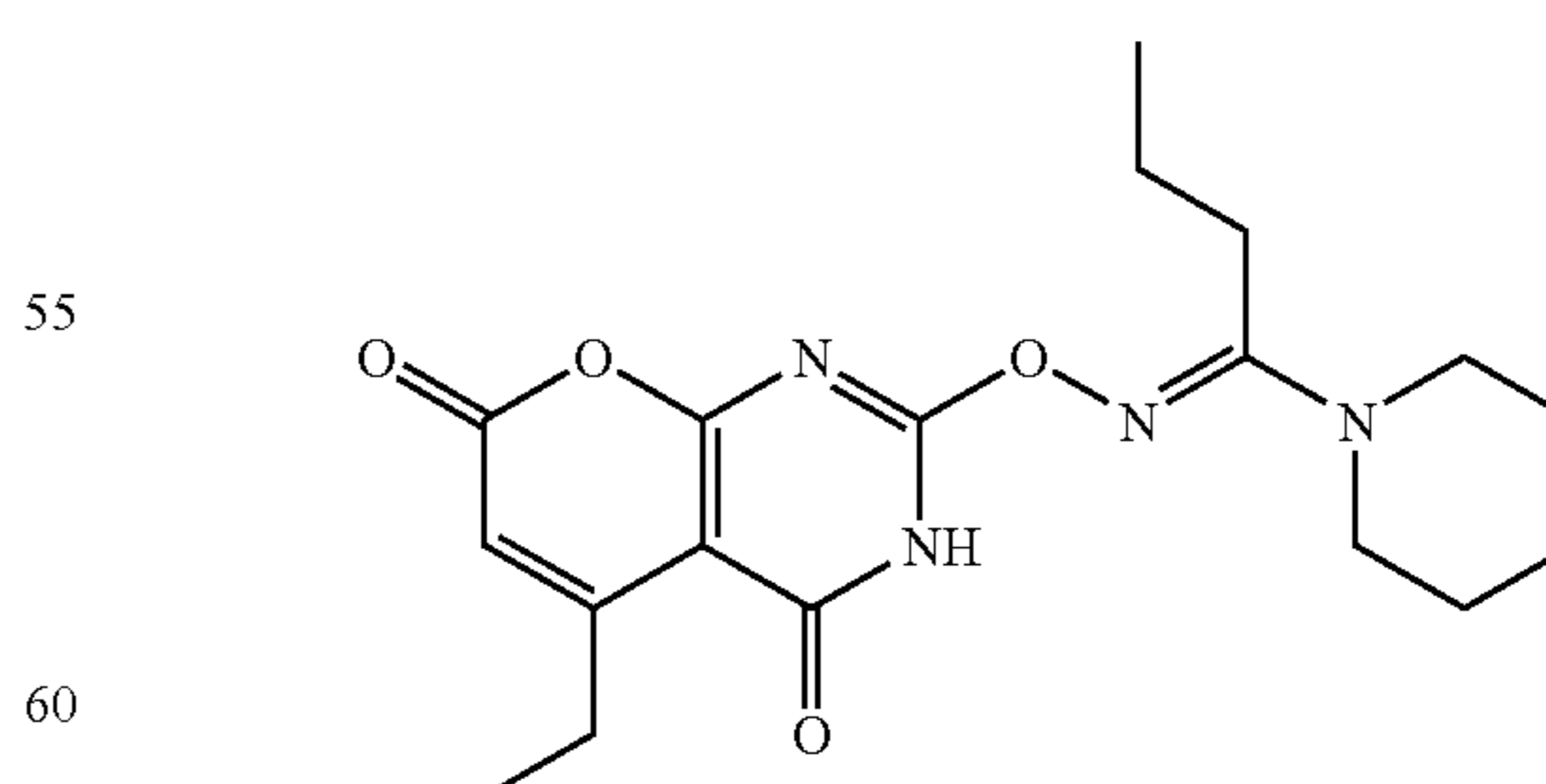
Compound 15:
