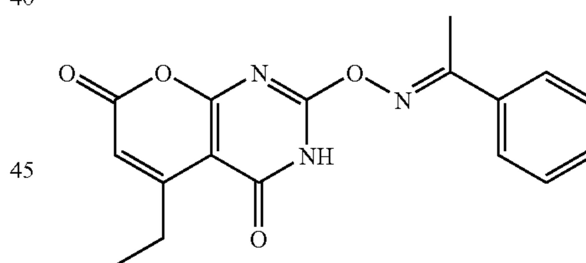
Compound 48:
