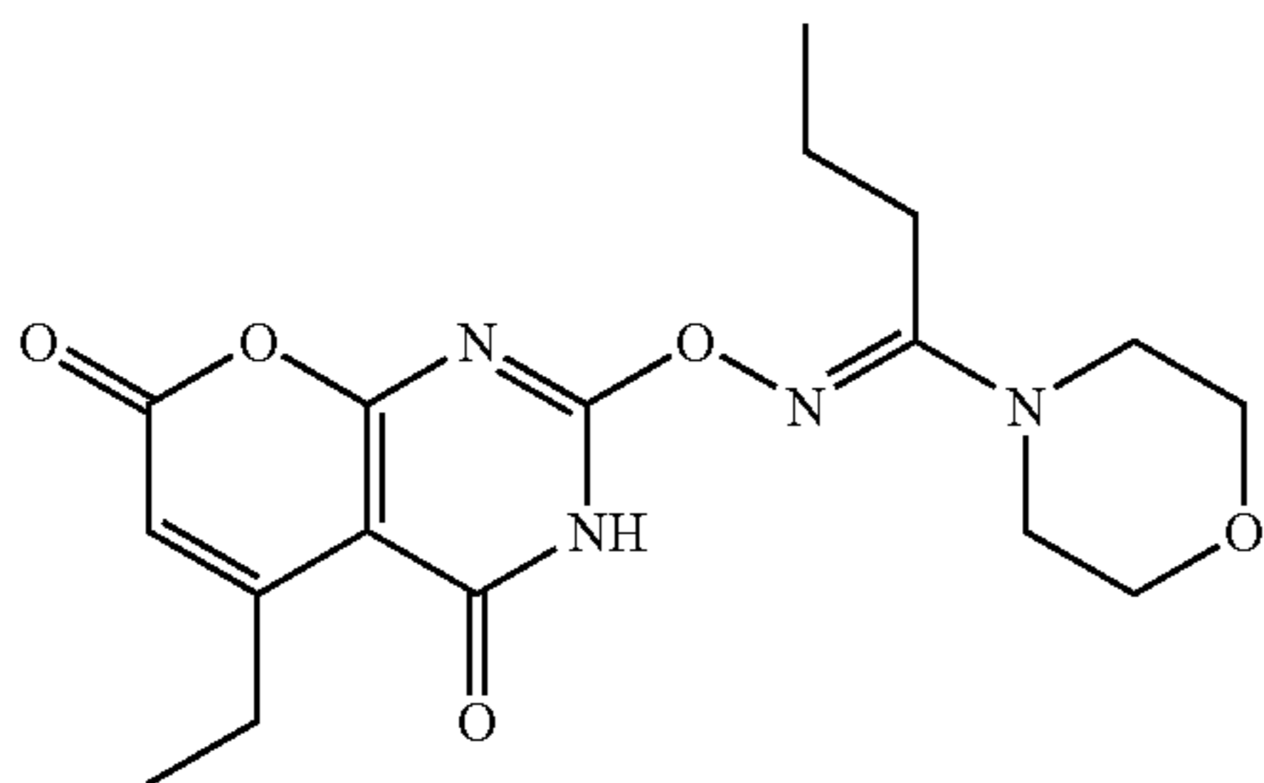
Compound 17:
