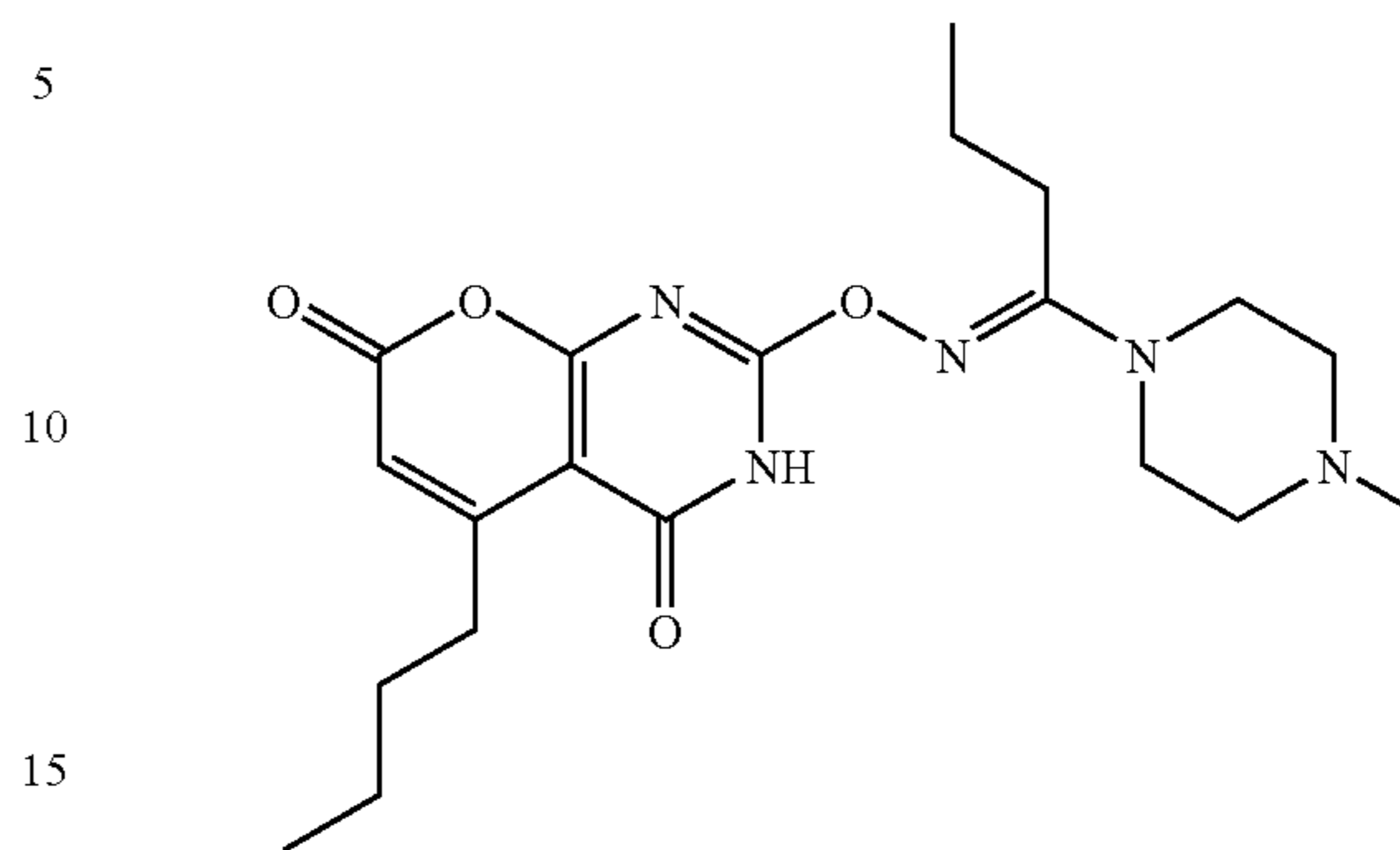
Compound 19:
