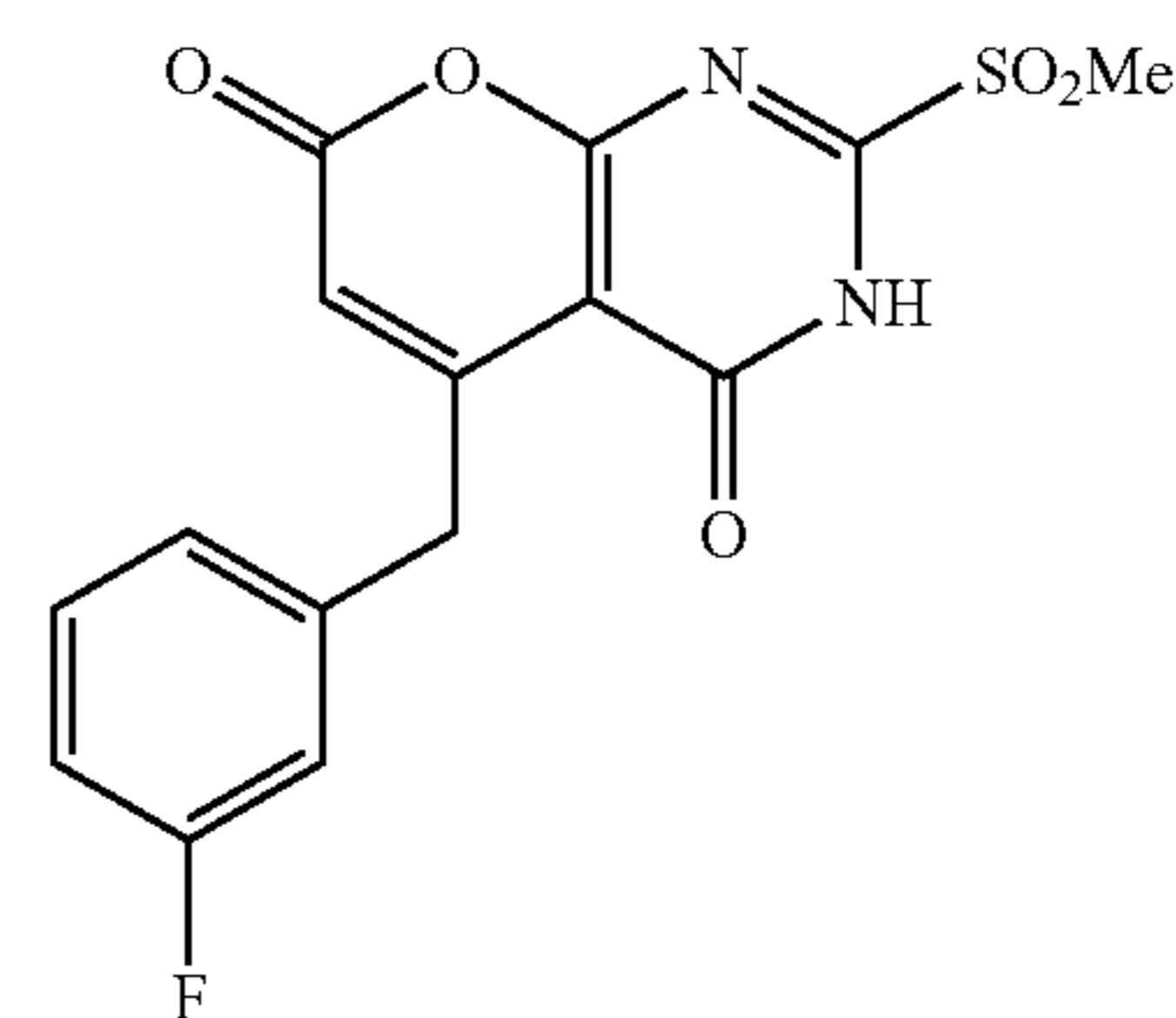
Compound 101d
