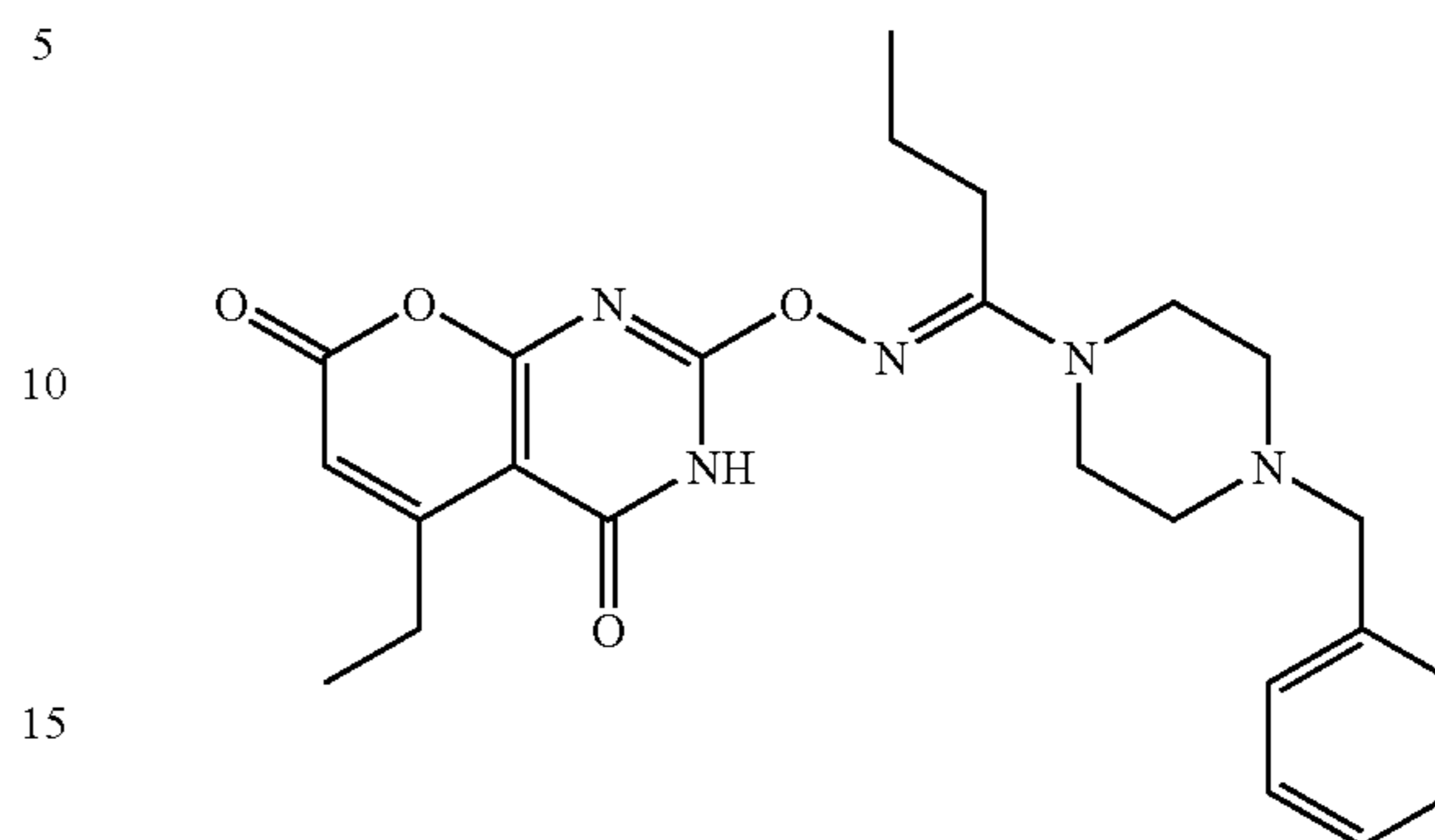
Compound 13:
