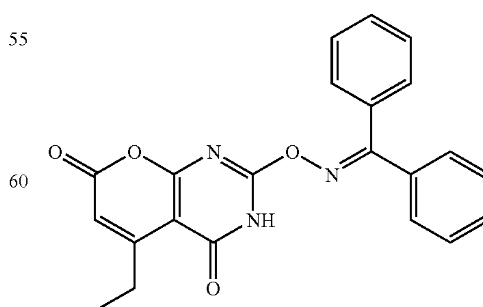
Compound 49:
