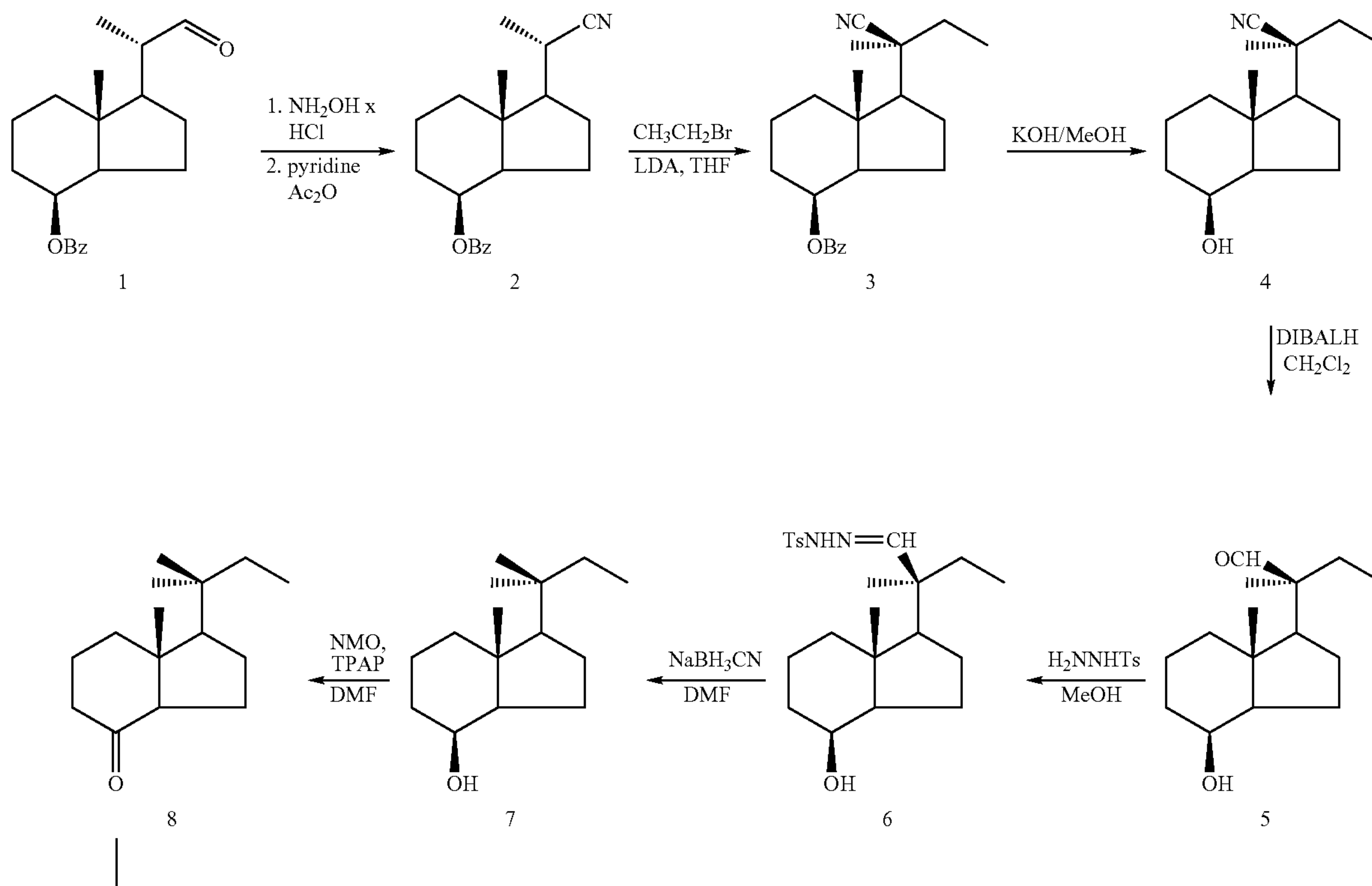
SCHEME I
