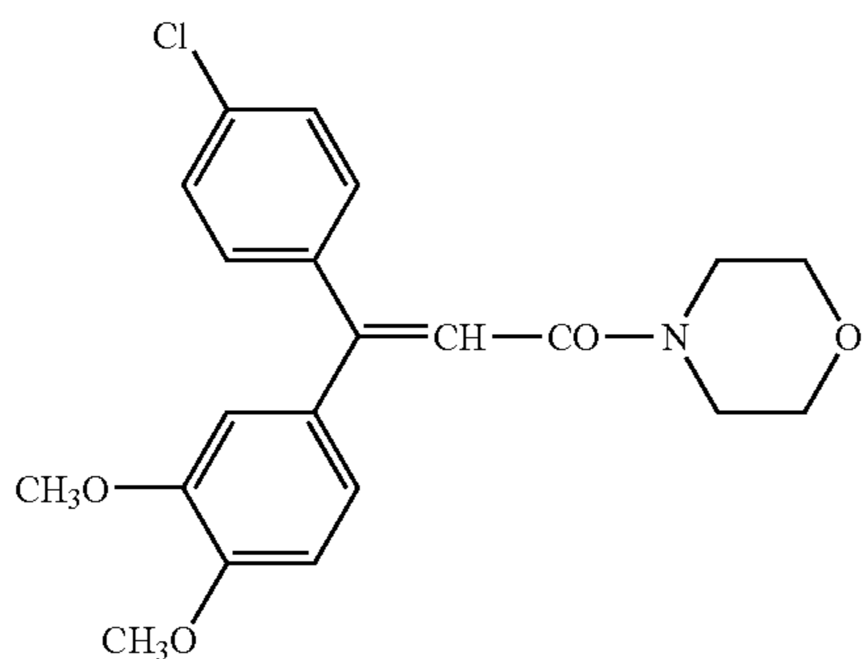
(DIMETHOMORPH)
