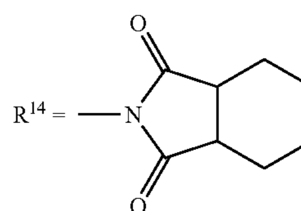
(CAPTAN)
