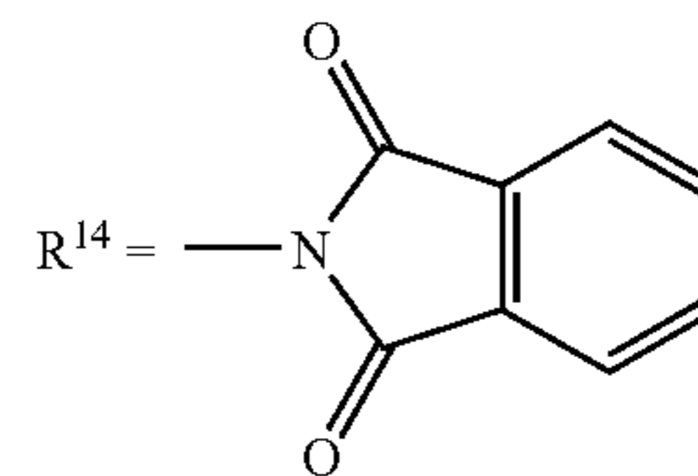
(FOLPET)
