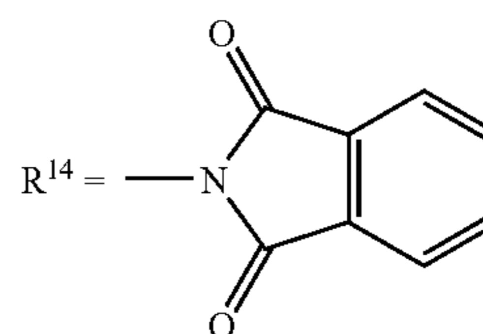
(FOLPET)
