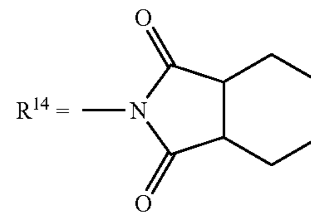
(CAPTAN)
