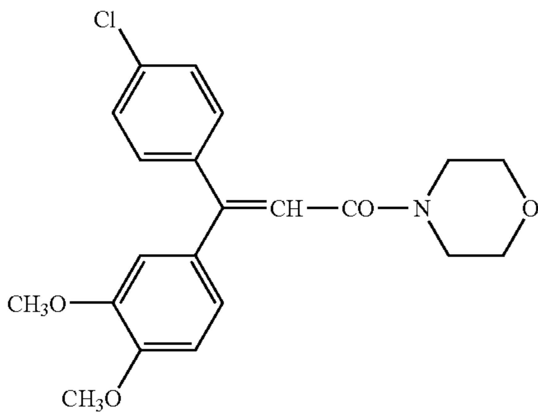
(DIMETHOMORPH)
