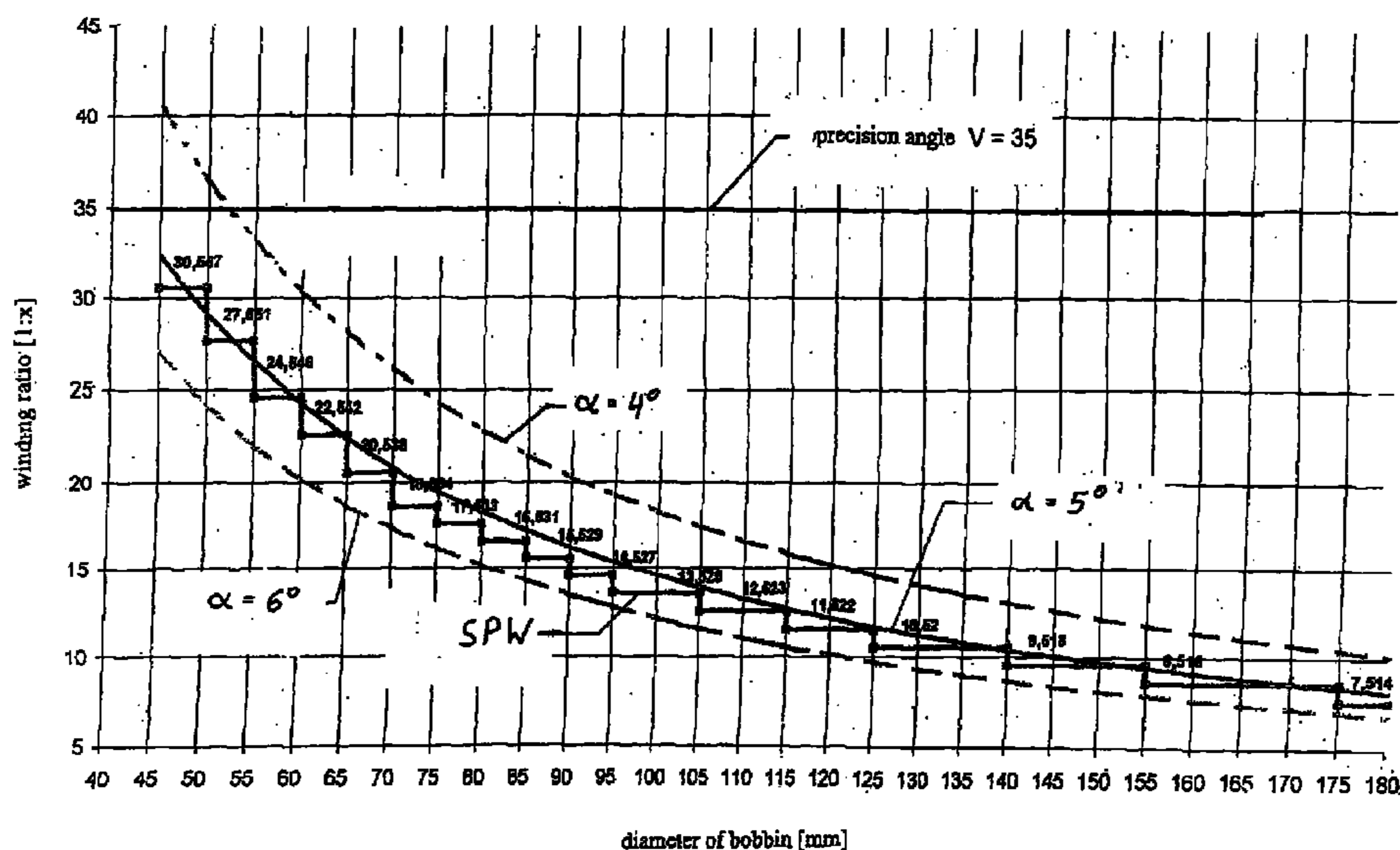
Winding ratios in the winding angle limit range of between 4° and 6°
