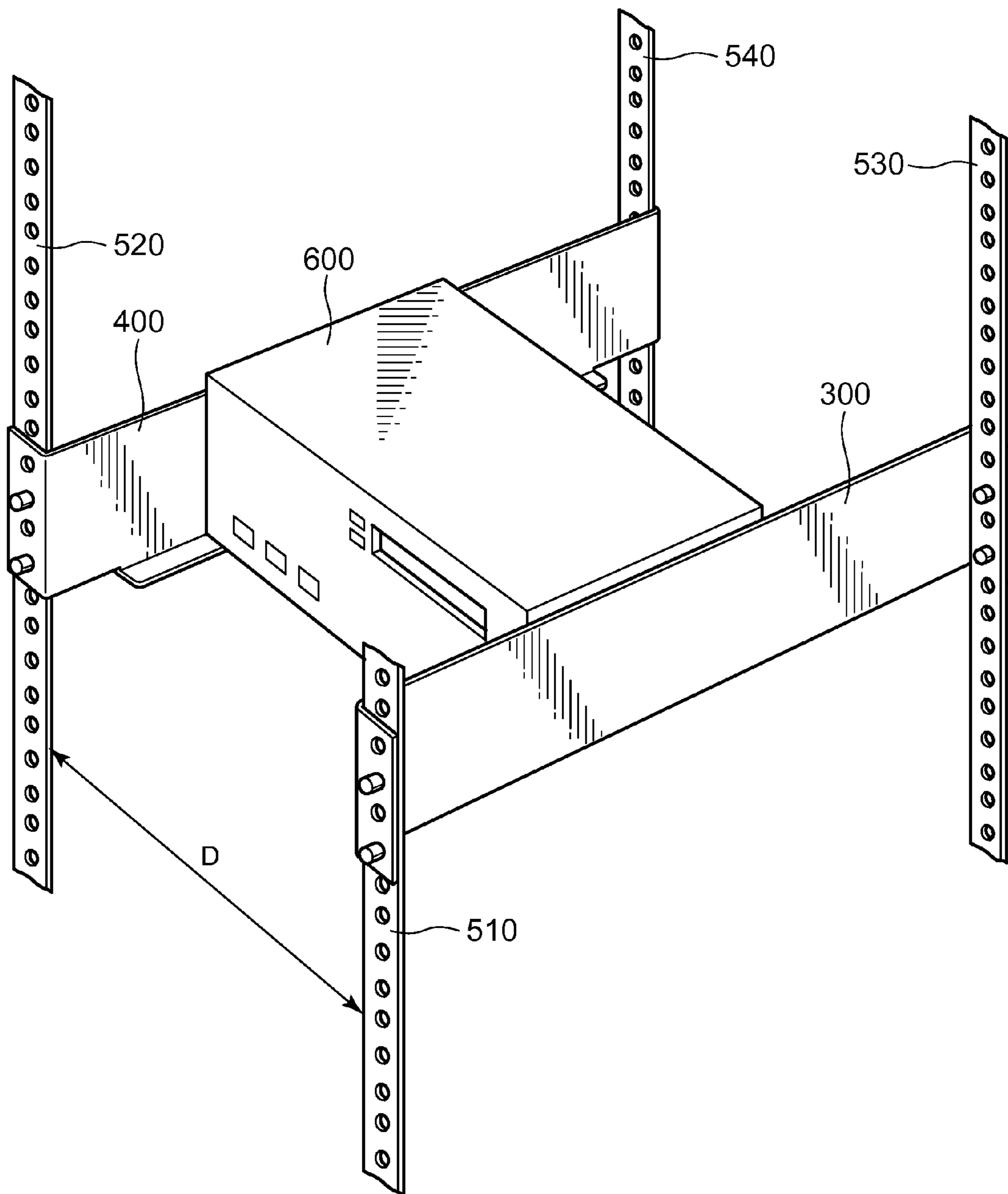
FIG. 7 PRIOR ART
