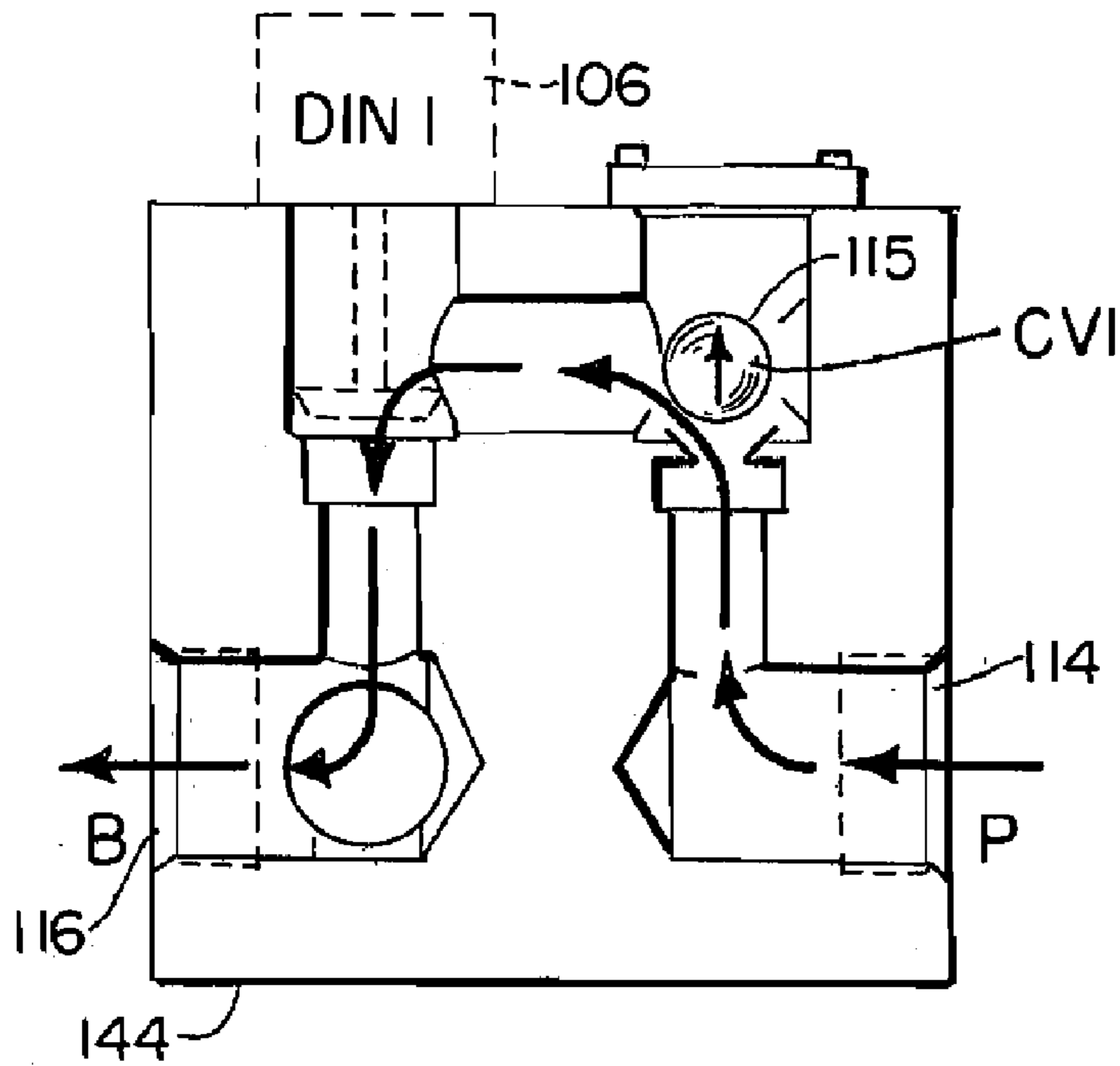
FIG. 40. UP STROKE
