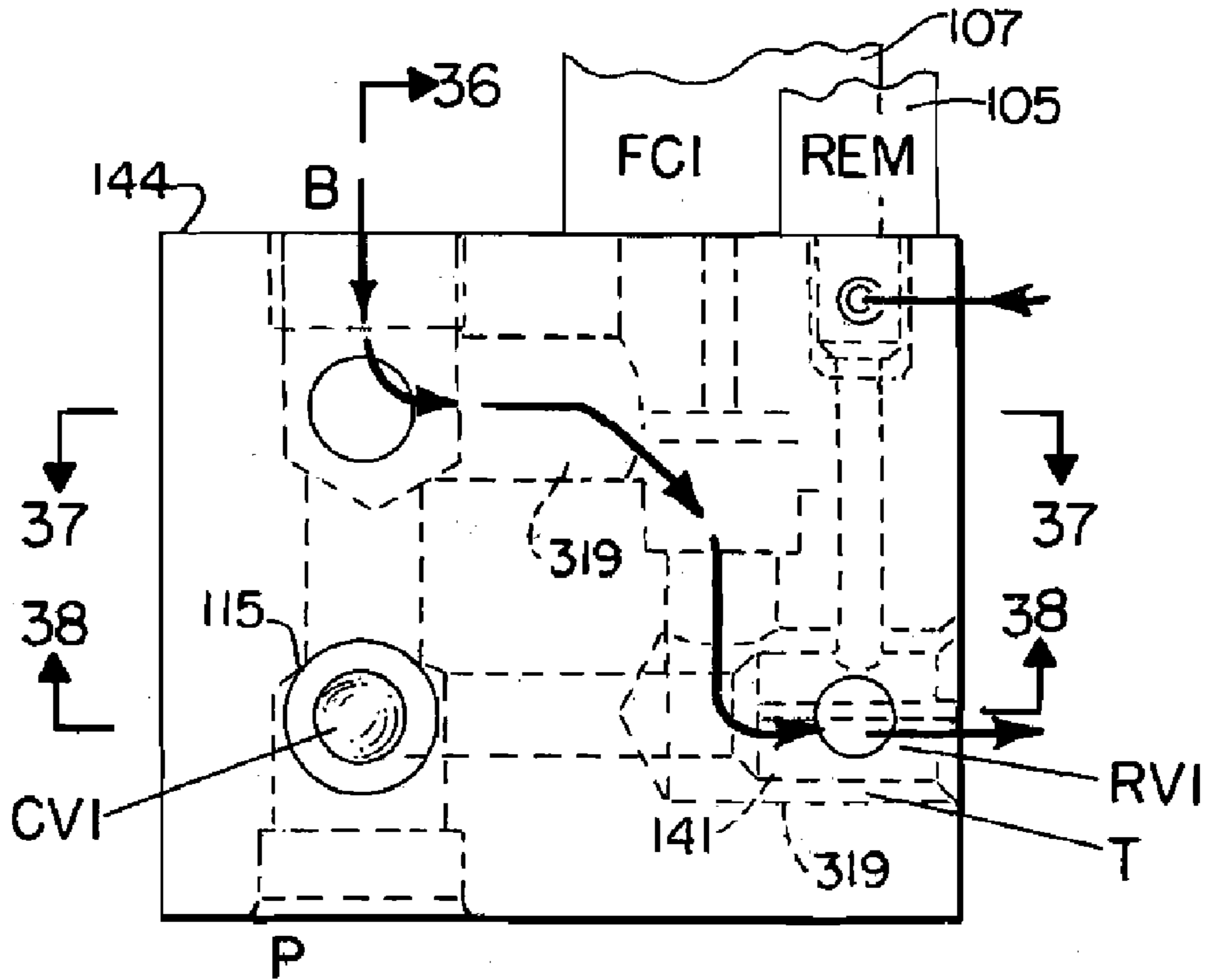
FIG. 35. DOWN STROKE
