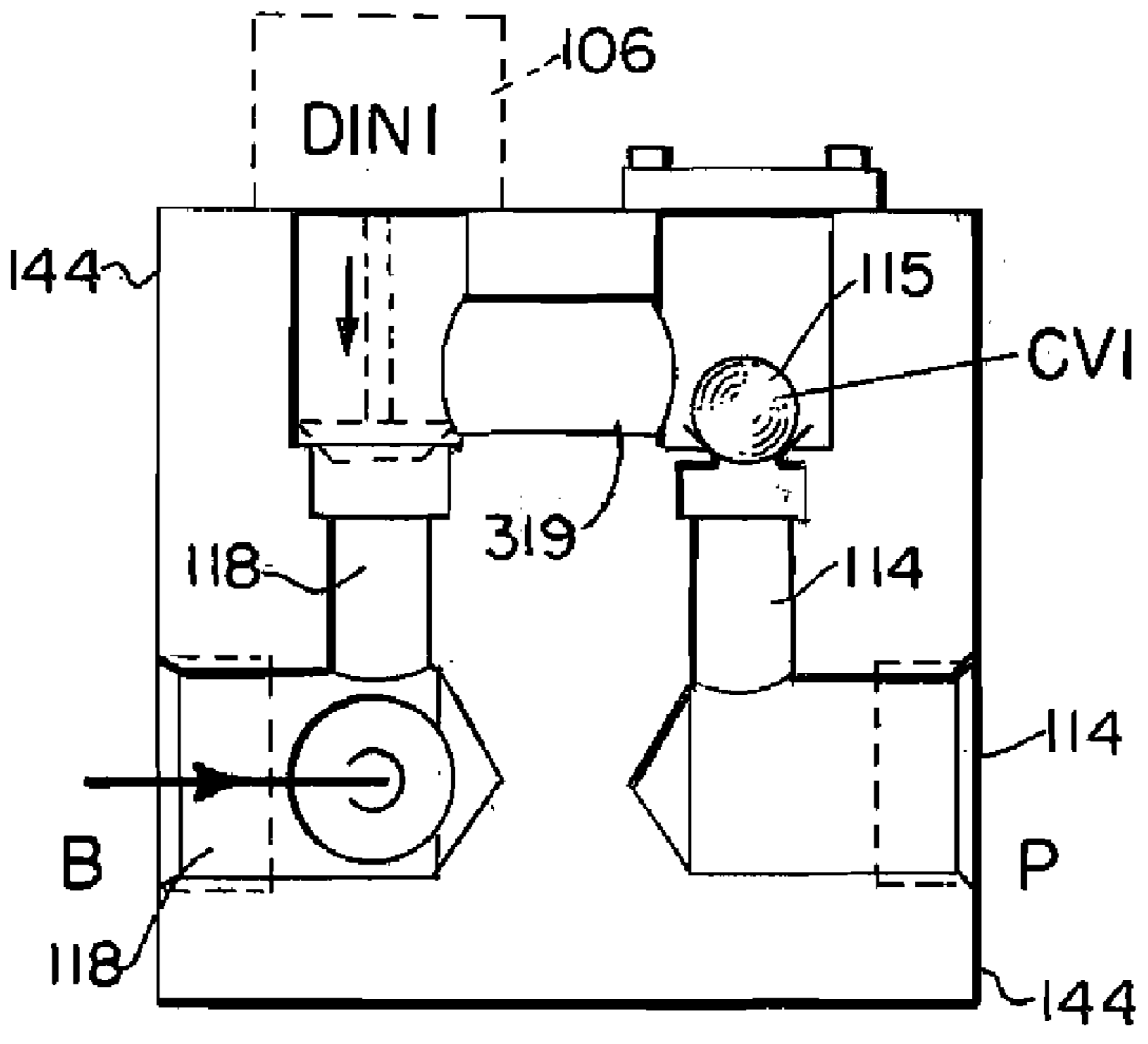
FIG. 35. DOWN STROKE
