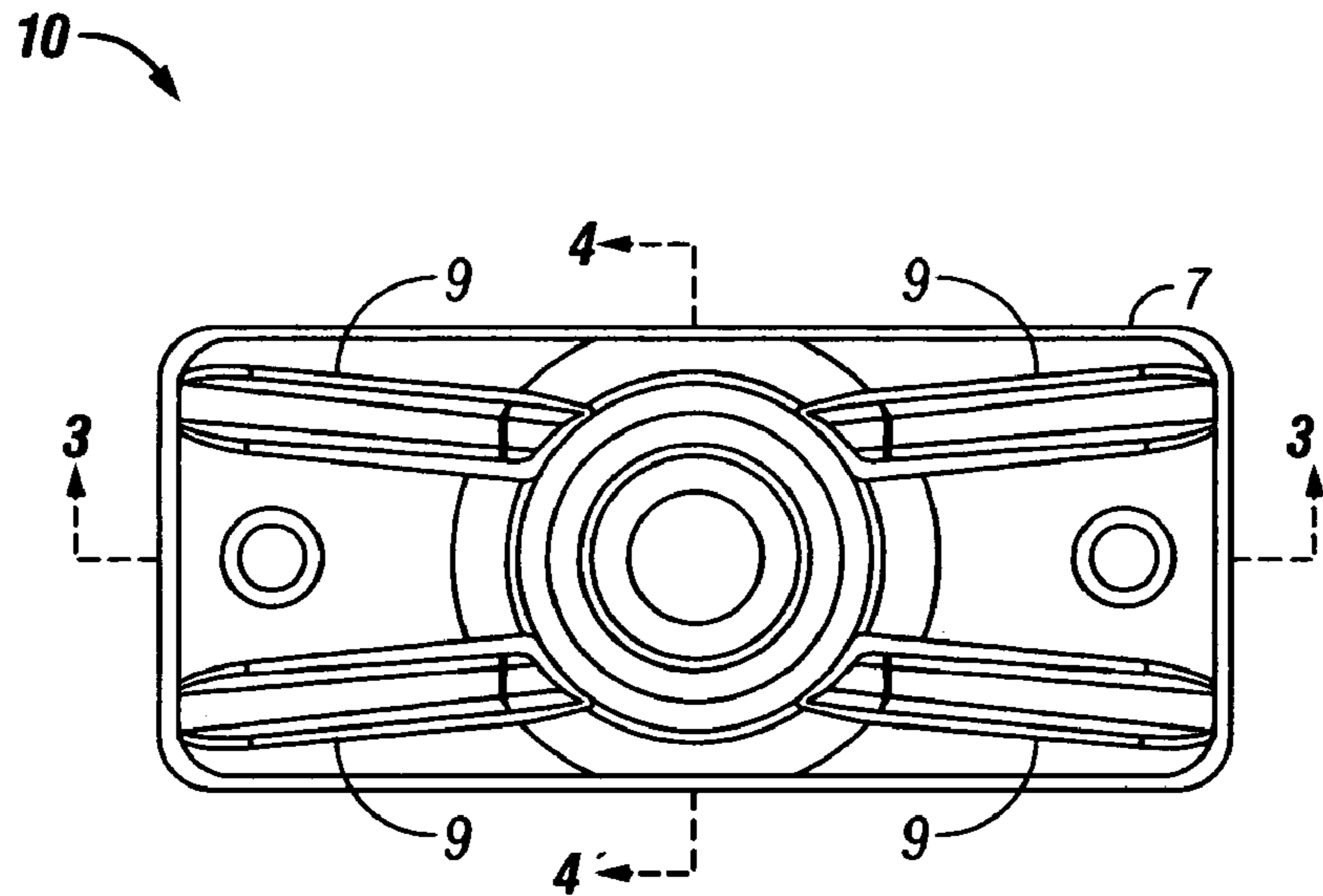
FIG. 2 (Prior Art)
