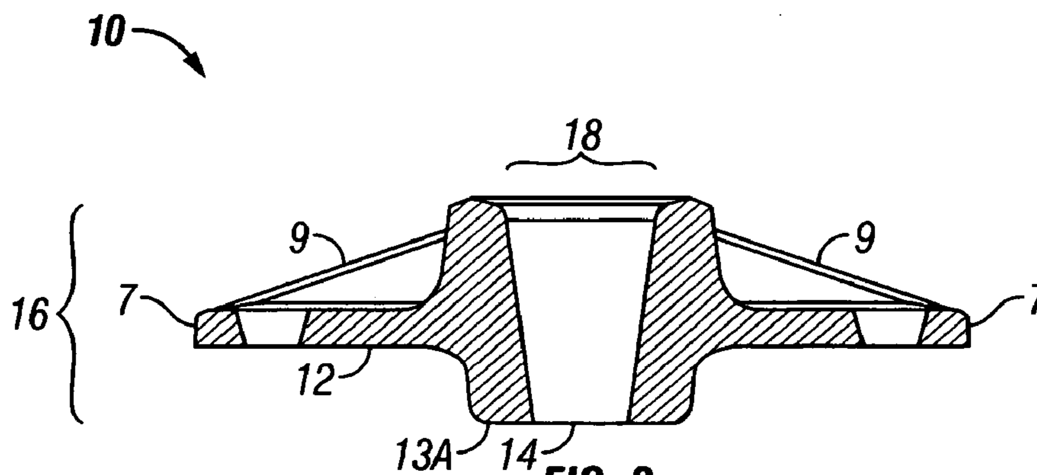
FIG. 3 (Prior Art)
