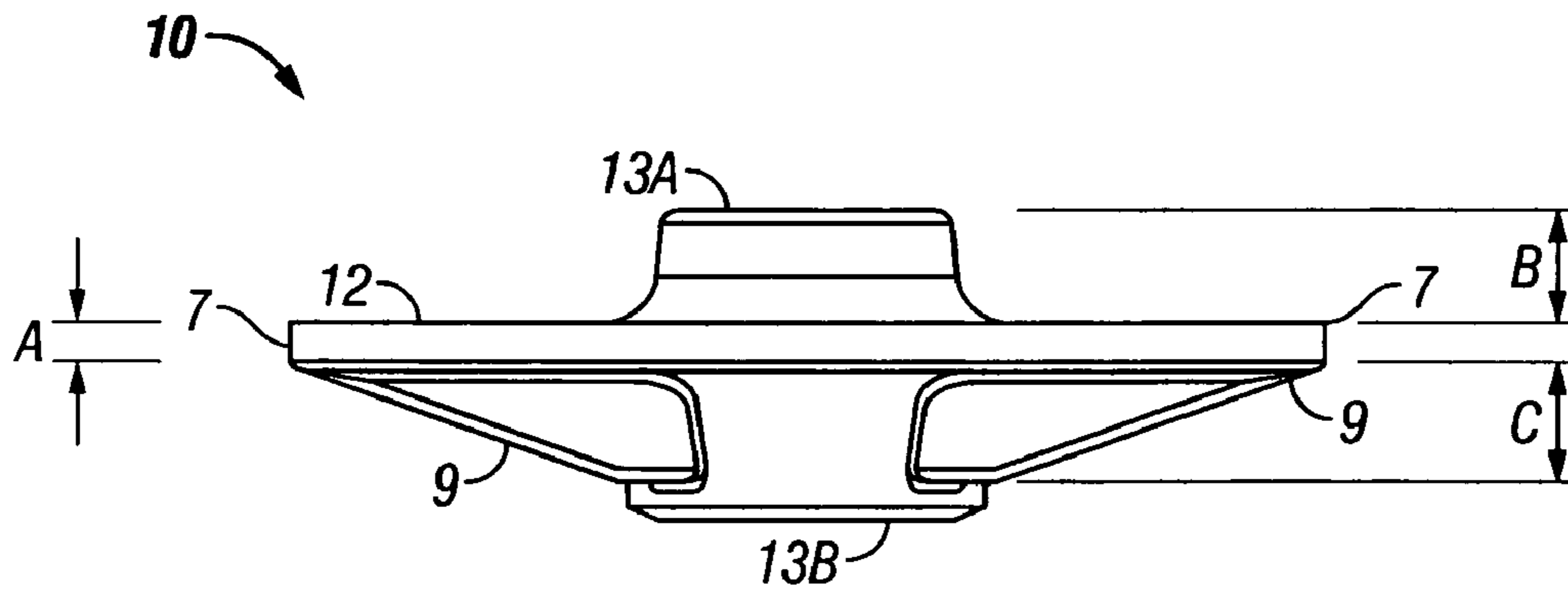
FIG. 1 (Prior Art)
