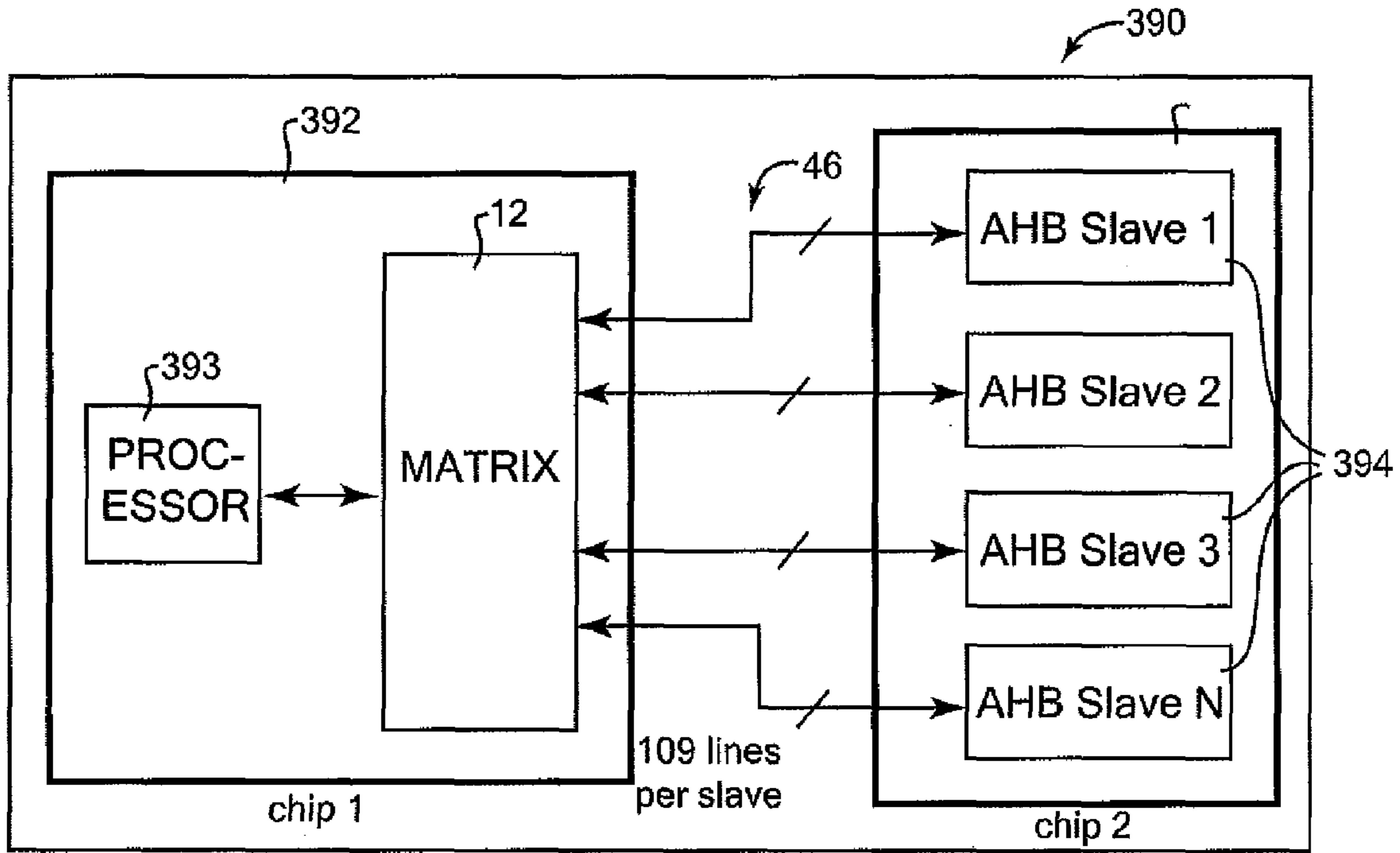
FIG. 14 (PRIOR ART)
