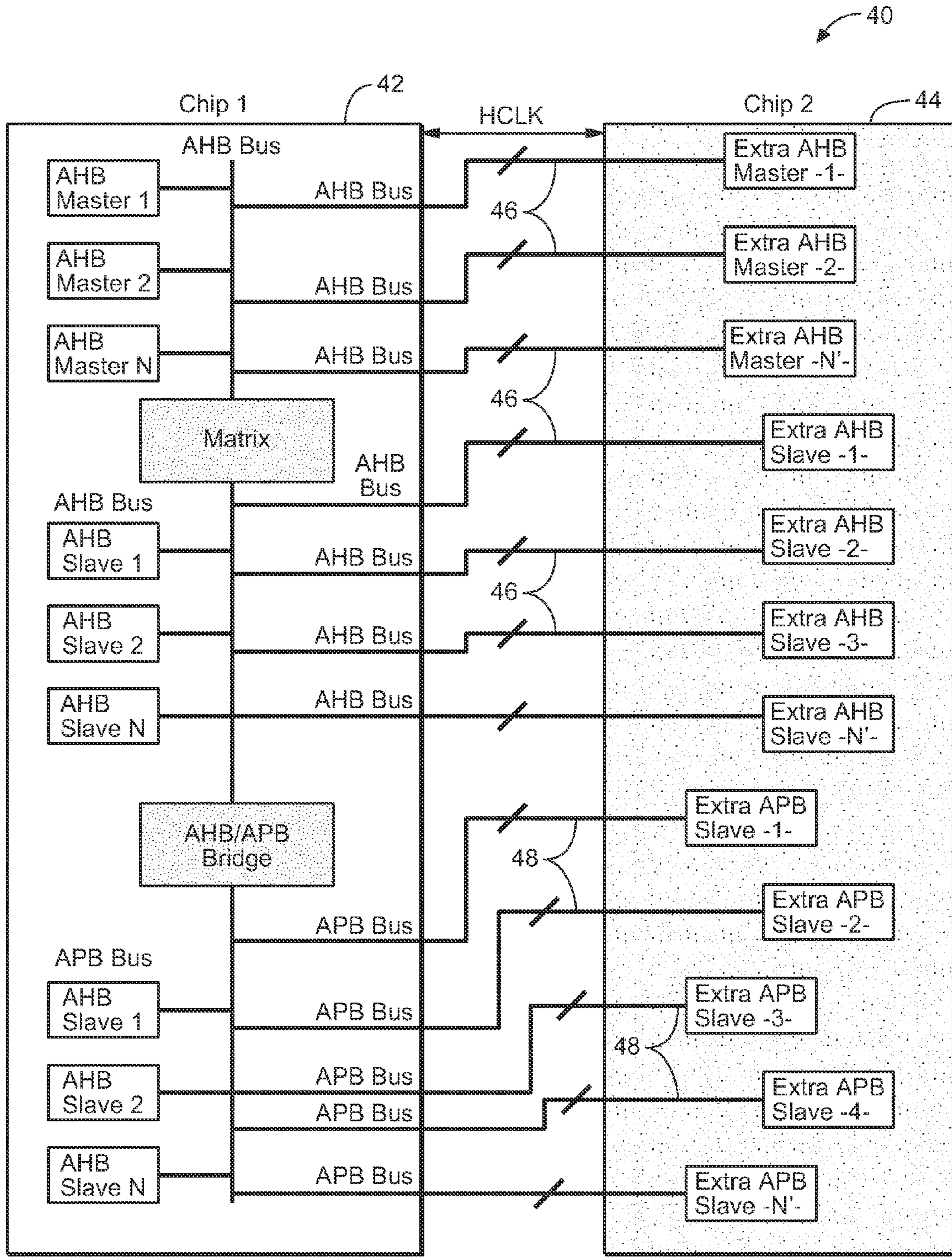
AMBA Base System in Chip 1
