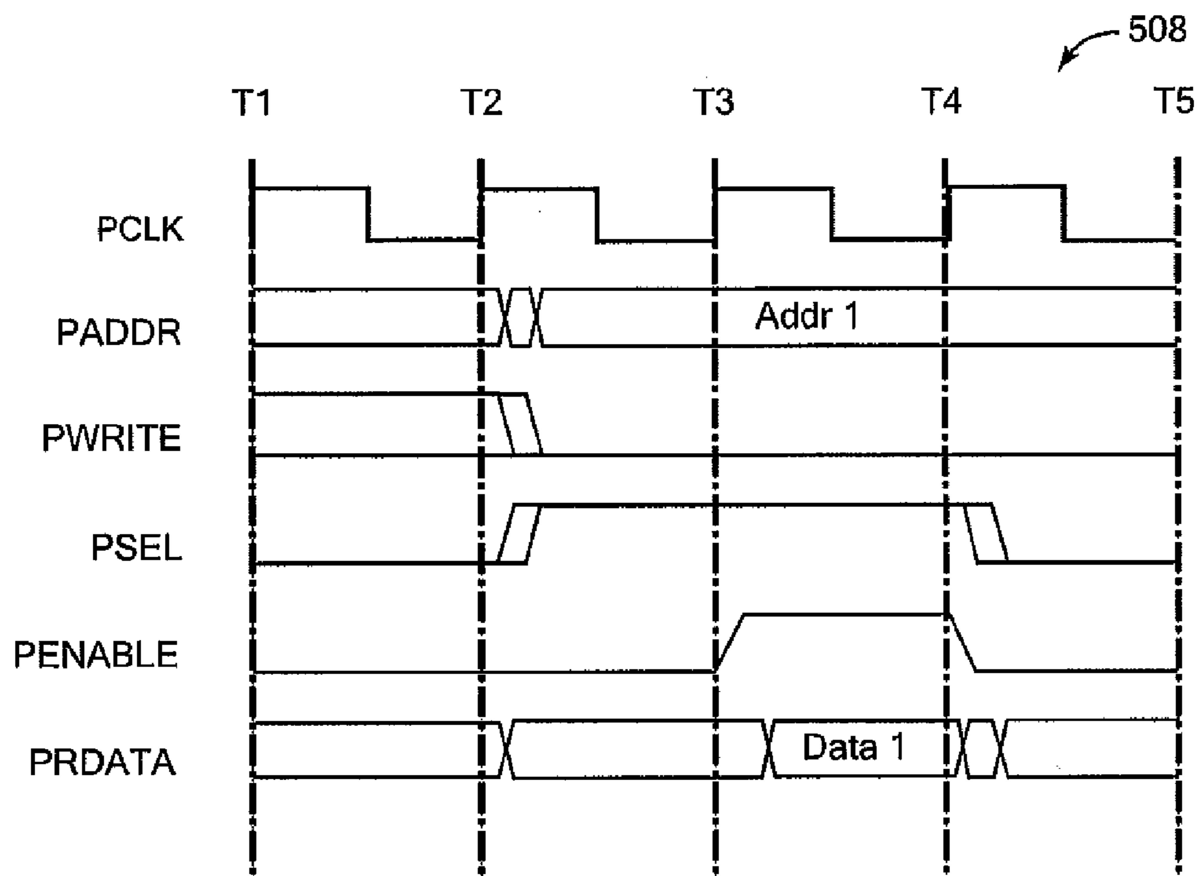
FIG. 20C (PRIOR ART)
