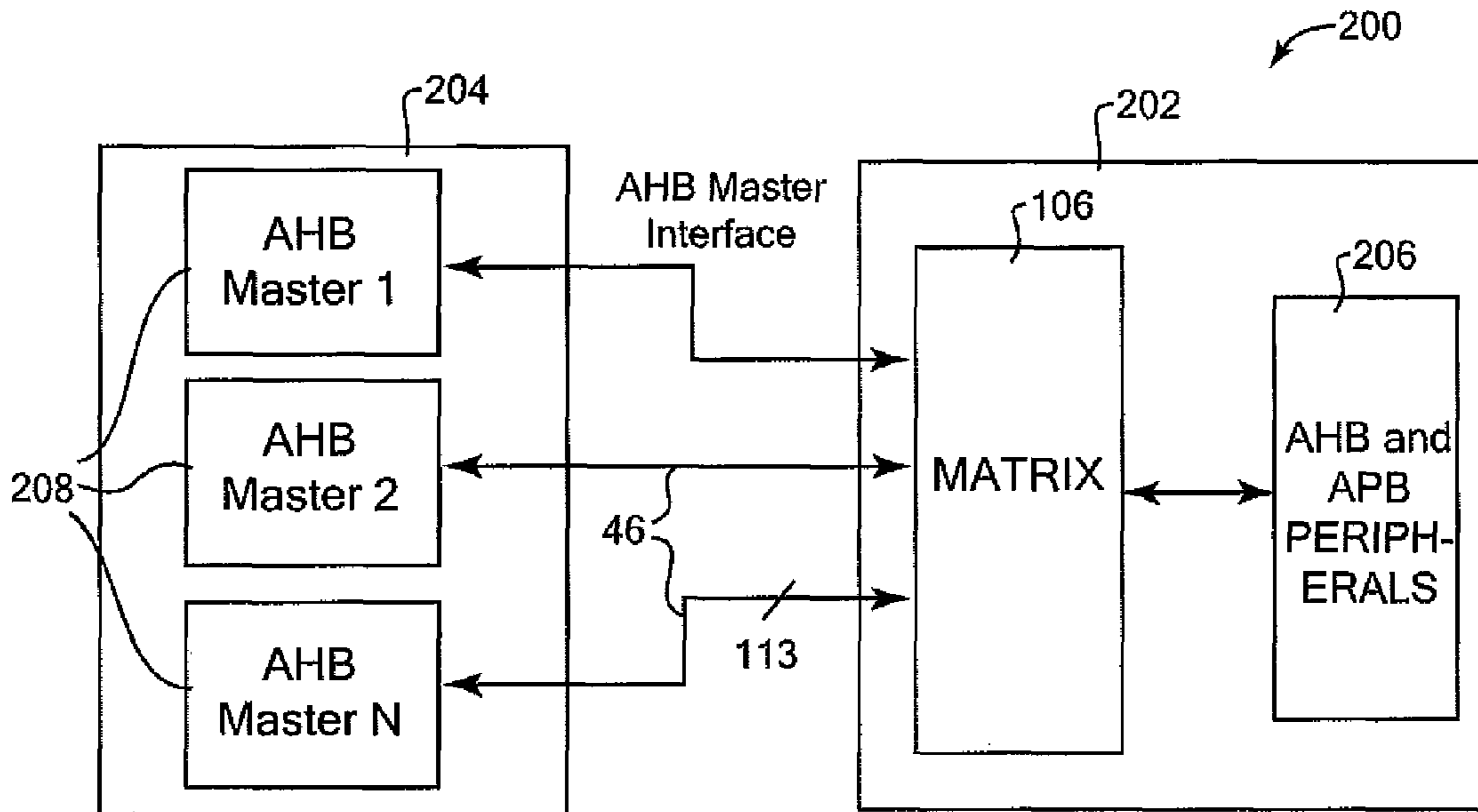
FIG. 6 (PRIOR ART)
