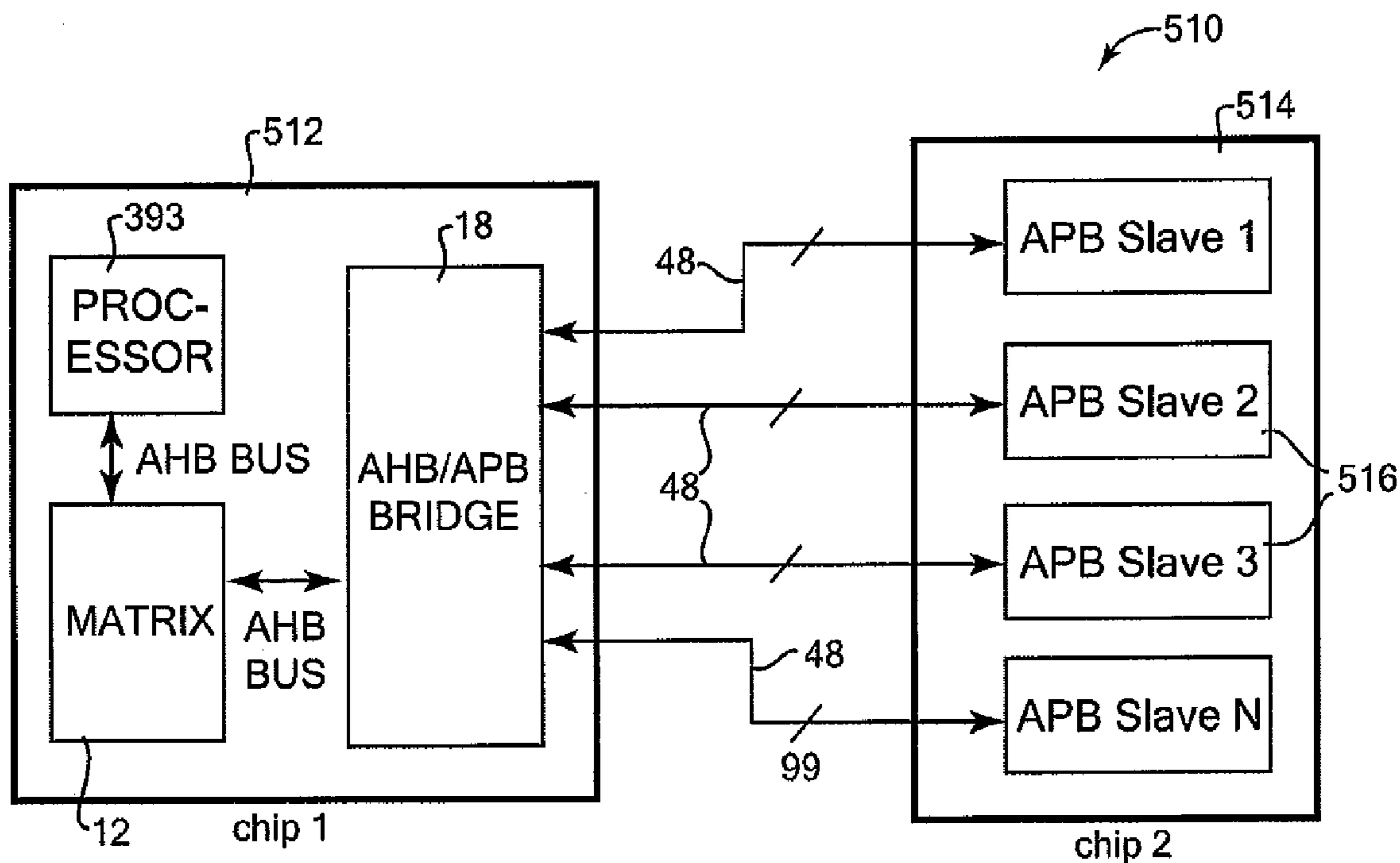
FIG. 21 (PRIOR ART)
