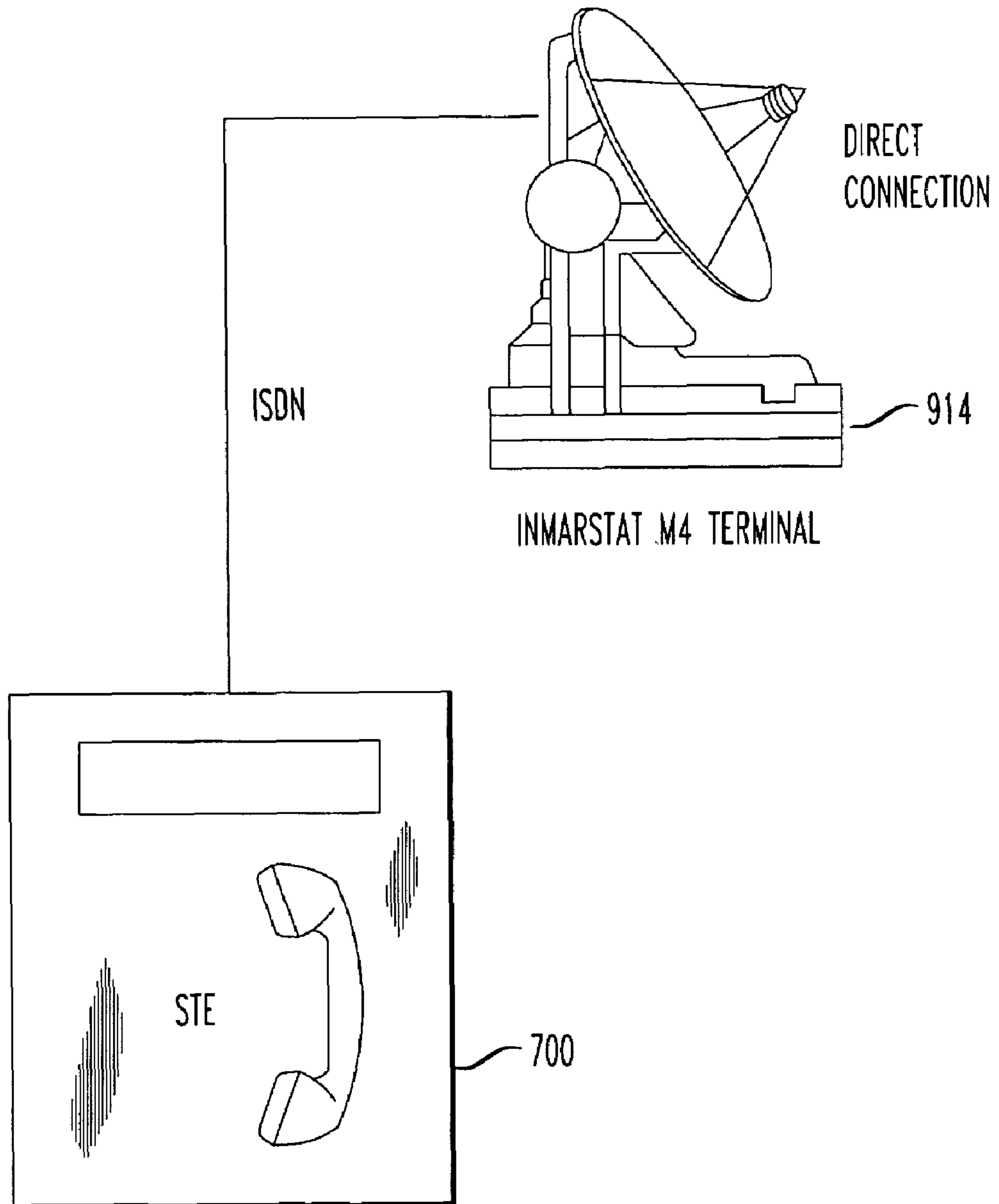
FIG. 24 (PRIOR ART)
