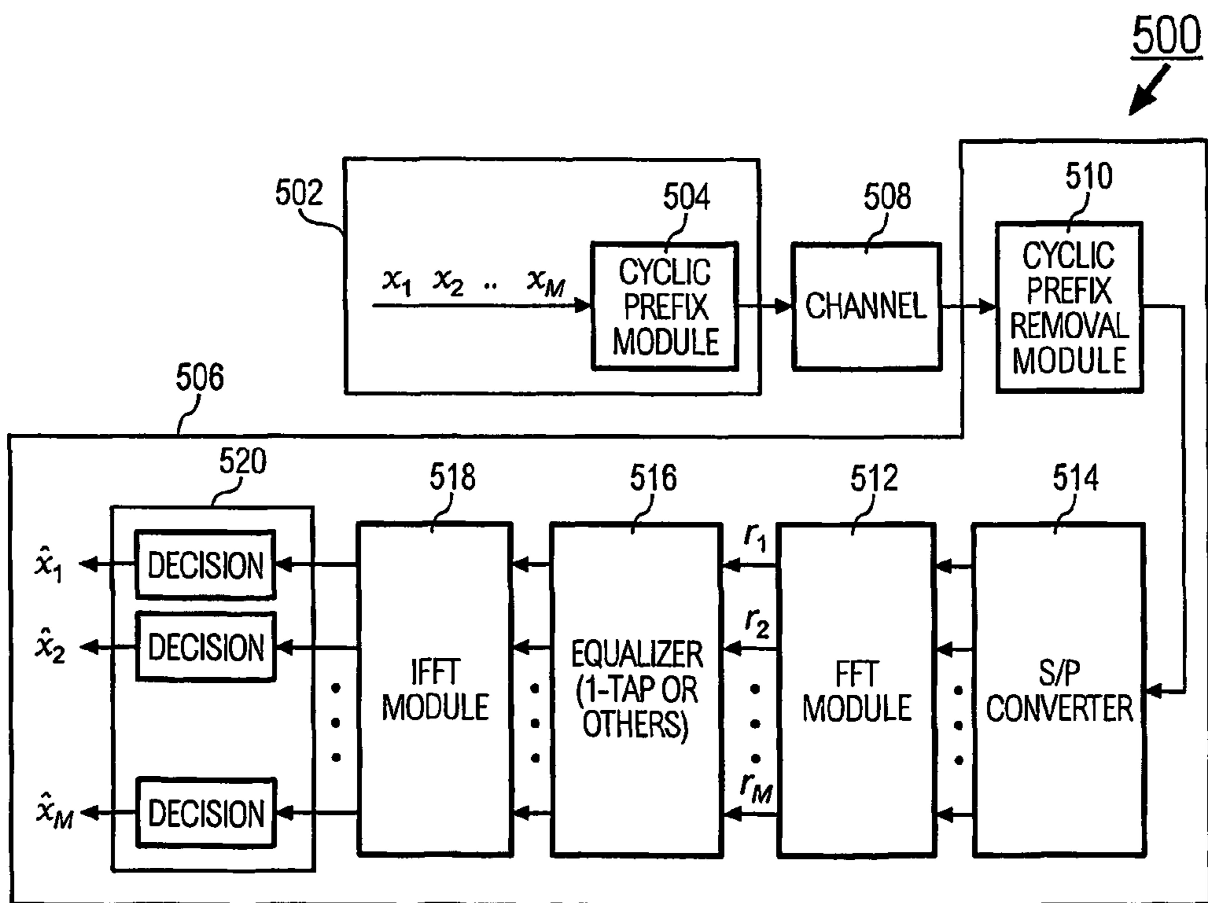
FIG. 7 (PRIOR ART)
