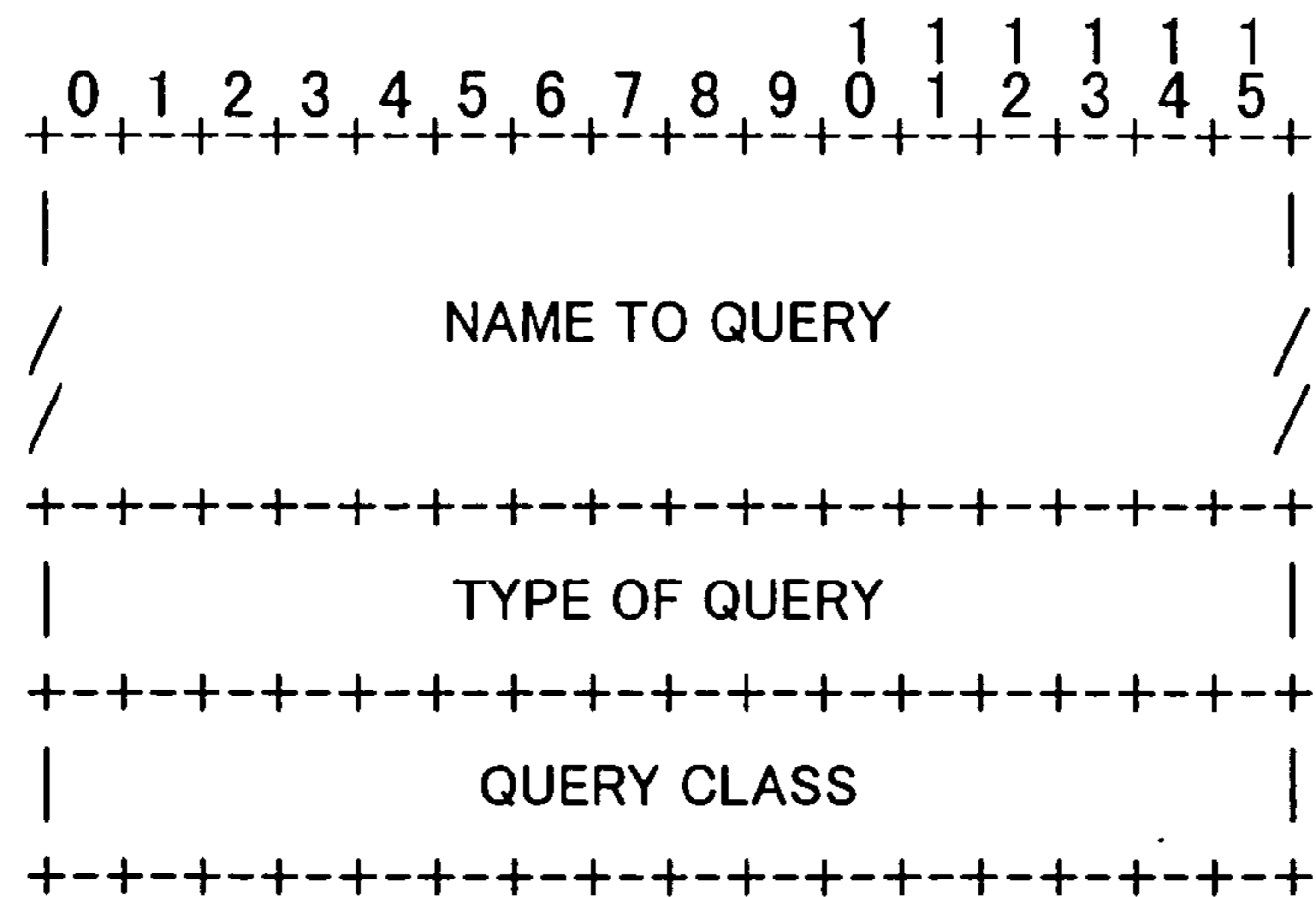
DNS query part, in FIG.54 message format
