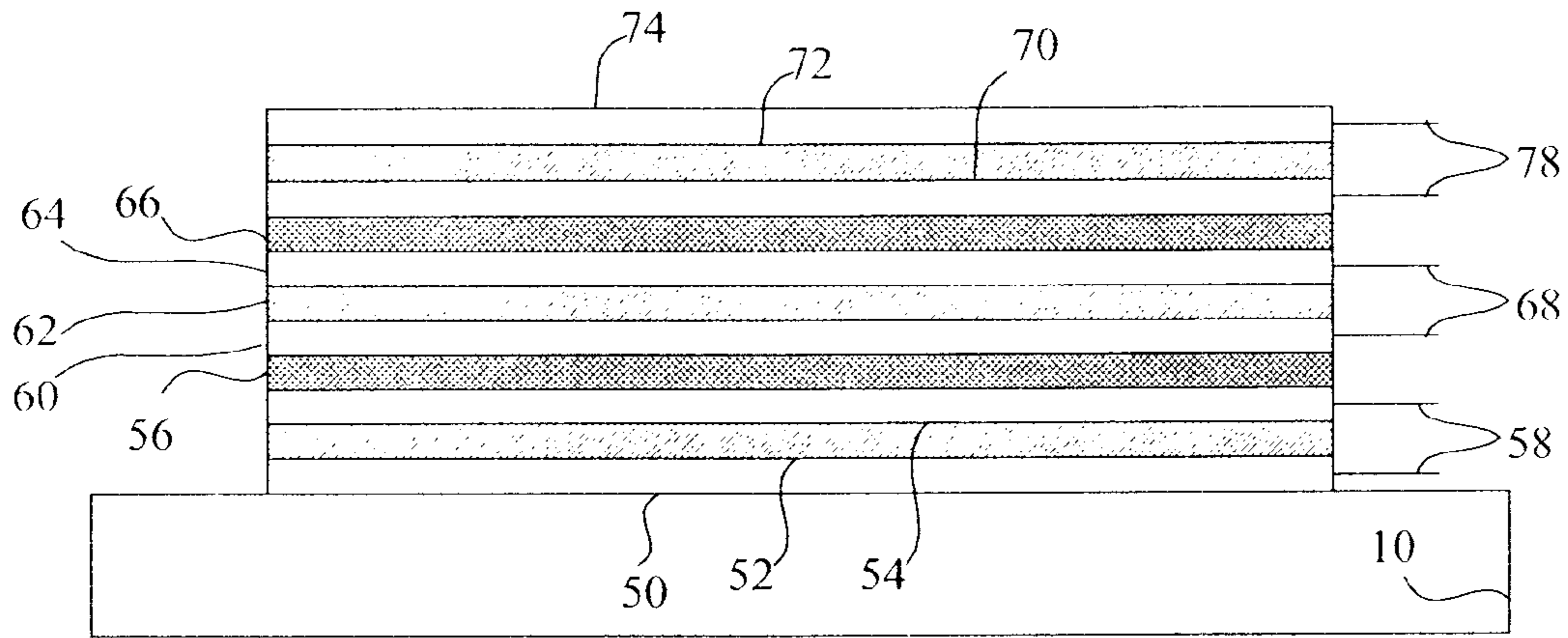
Fig. 5 - Prior art
