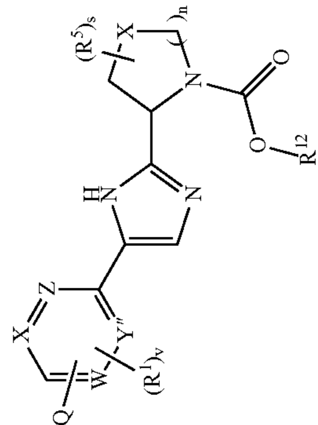
Scheme 11: Substituted Phenylglycine Derivatives.
