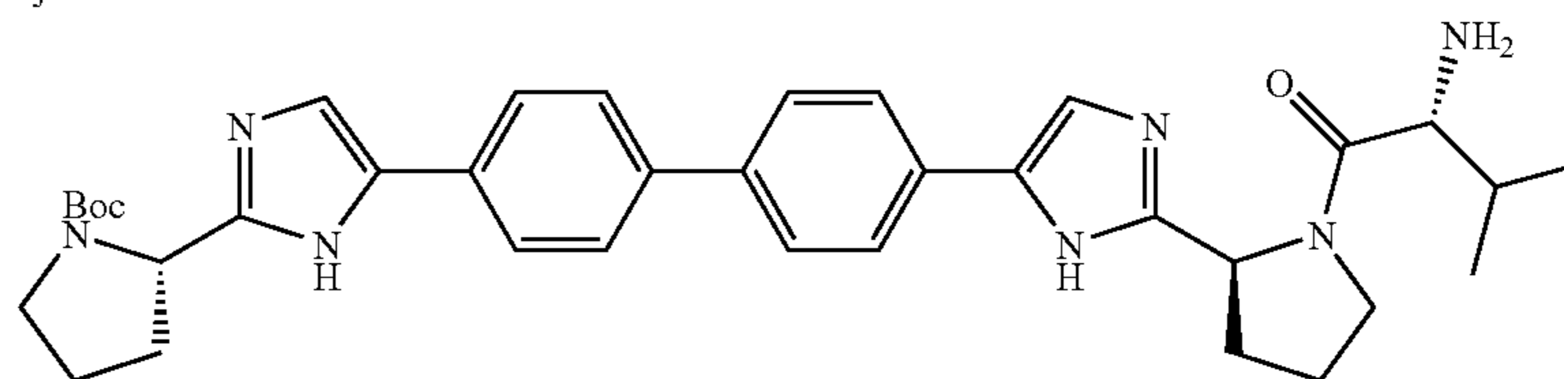
cj-3
