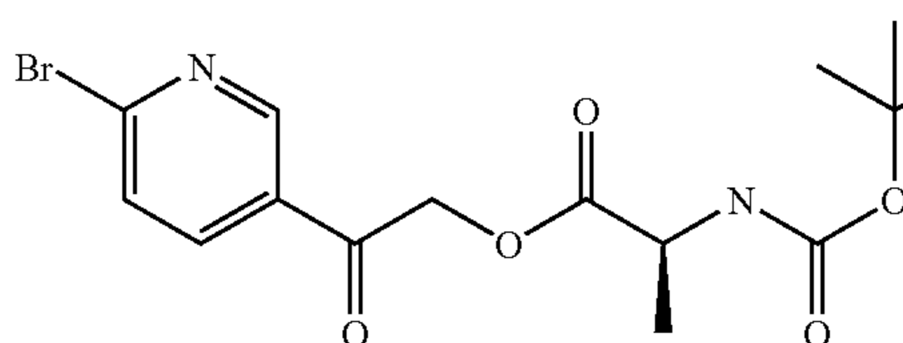
Example 152c-2
