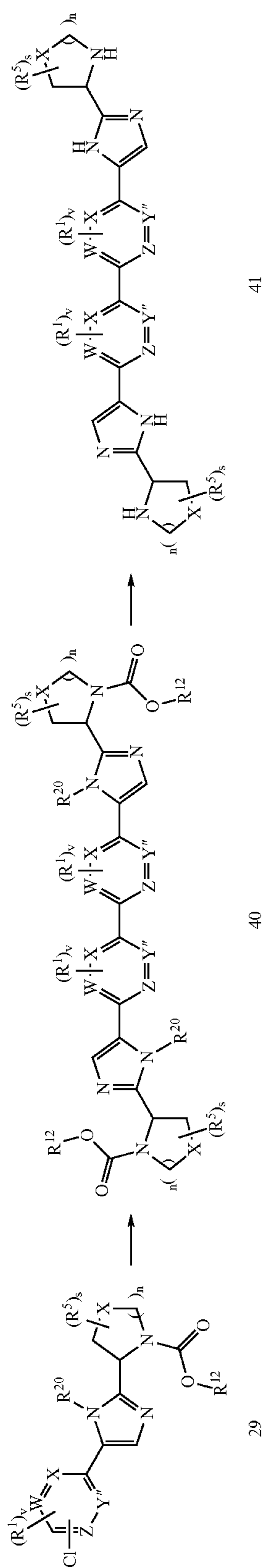
Scheme 9: Symmetric Cap Substituted Heteroaryls
