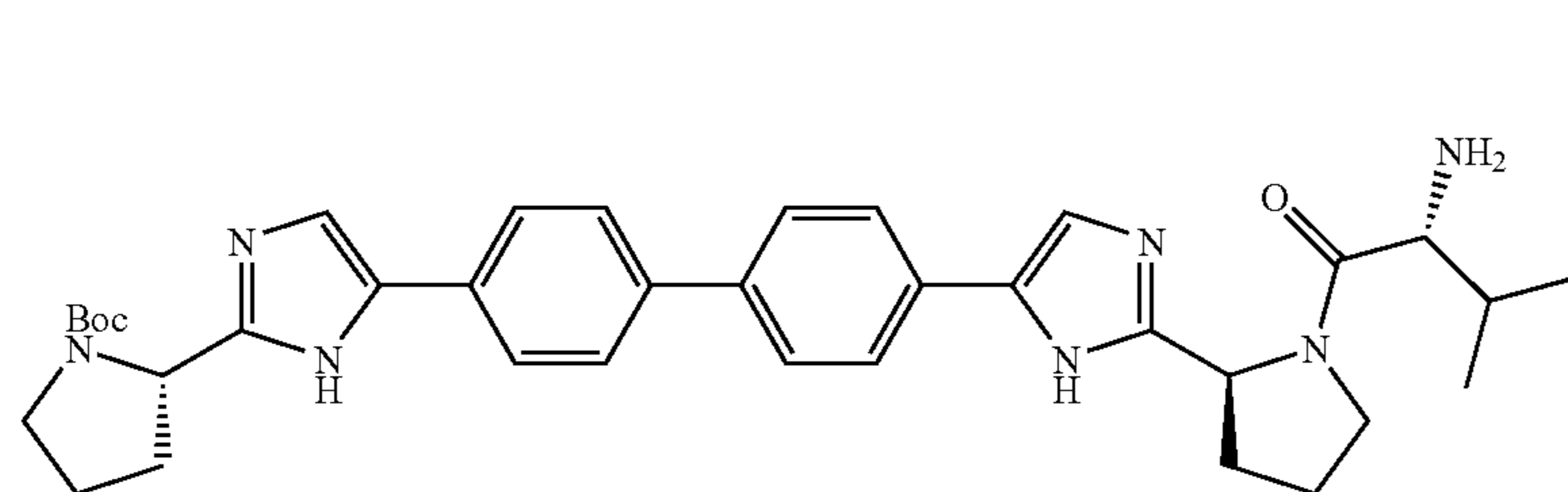
cj-3
