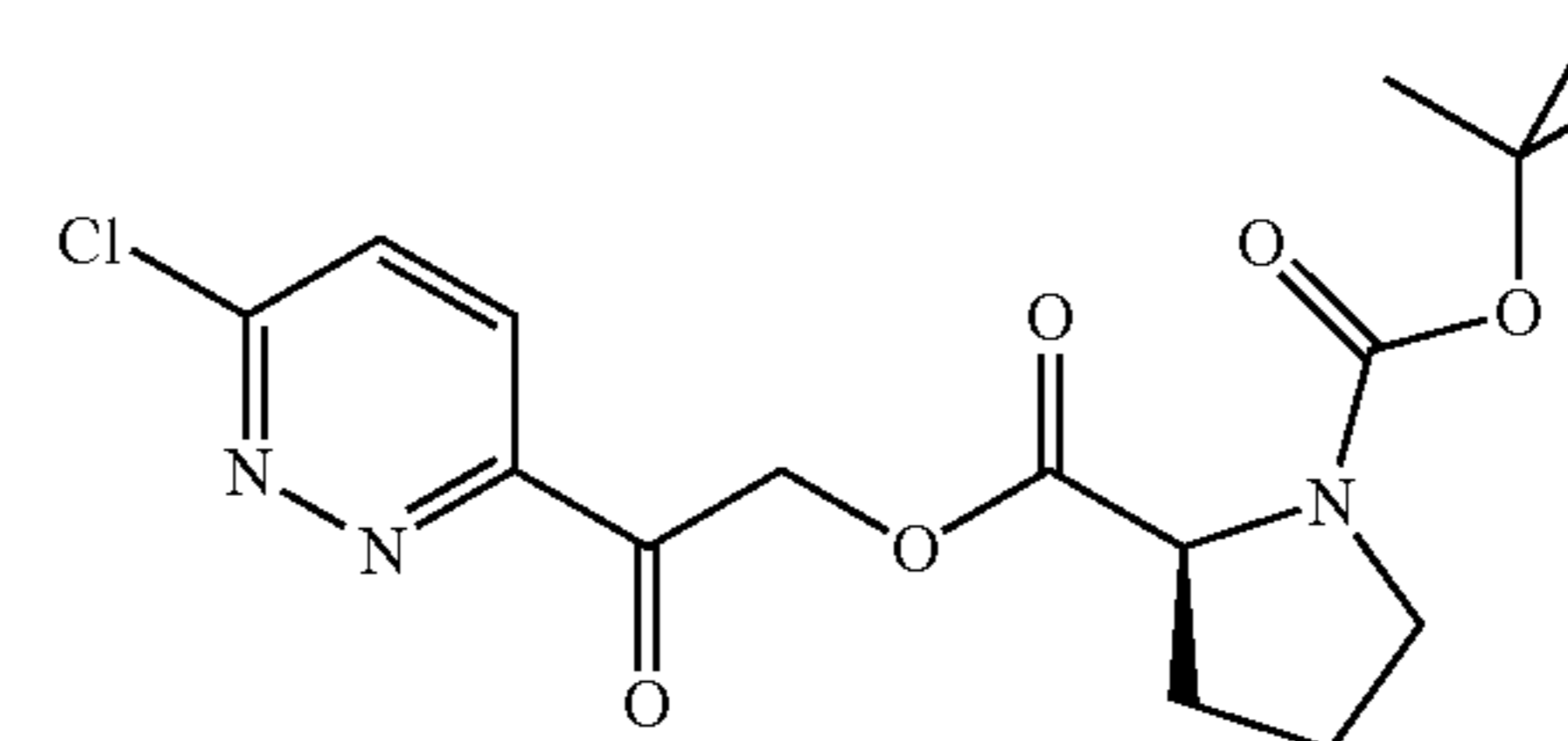
Example 152c-3a
