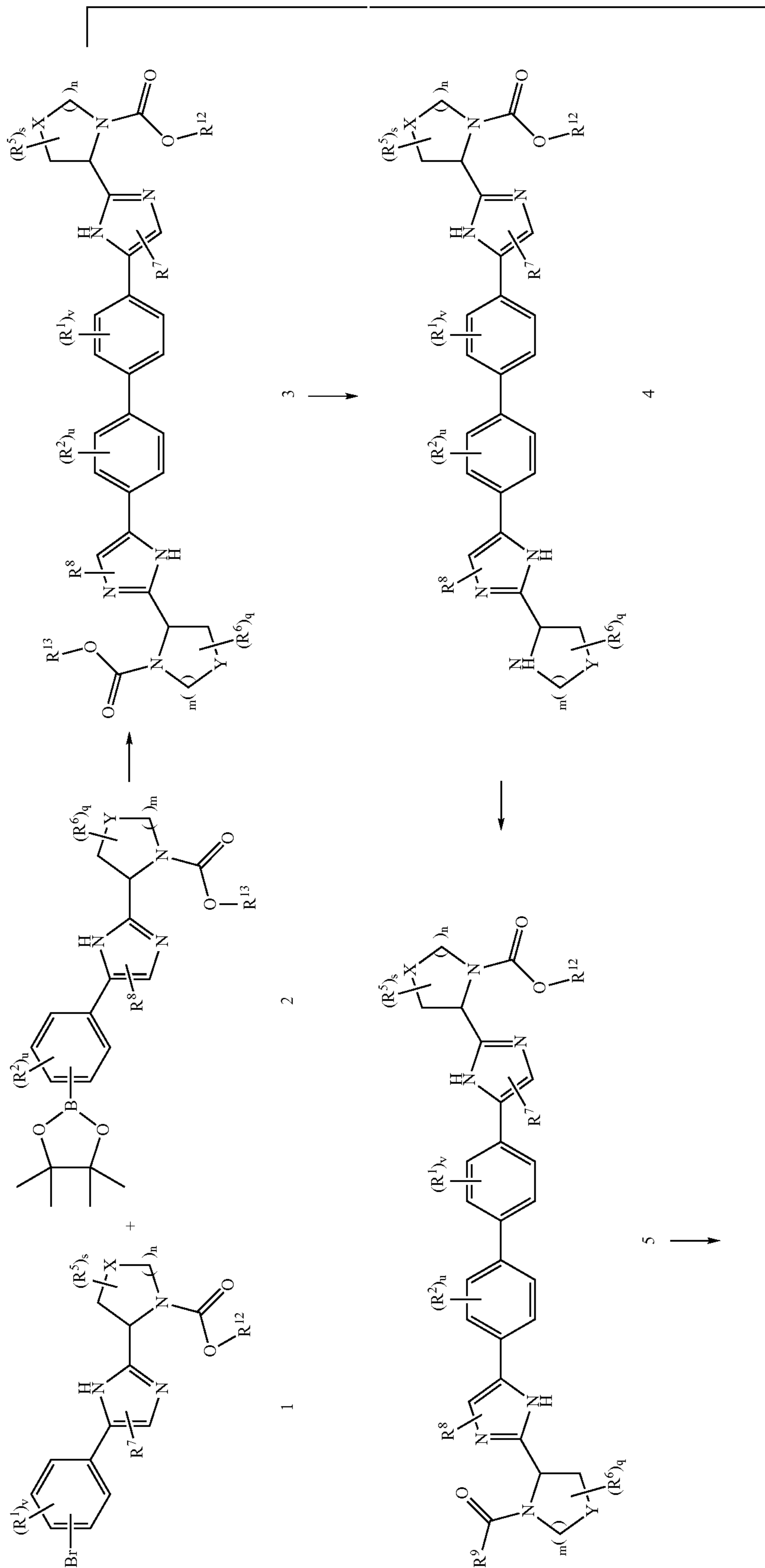
Scheme 2: Asymmetrically Capped Biphenyls
