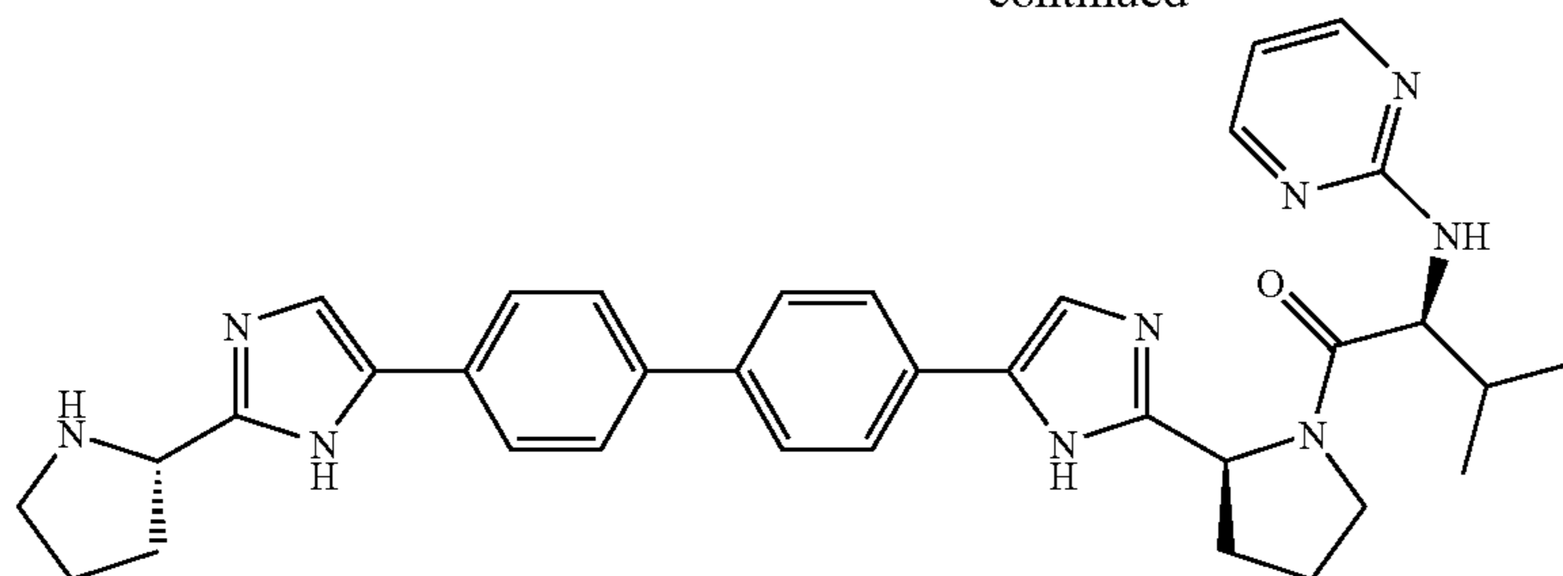
cj-10a
