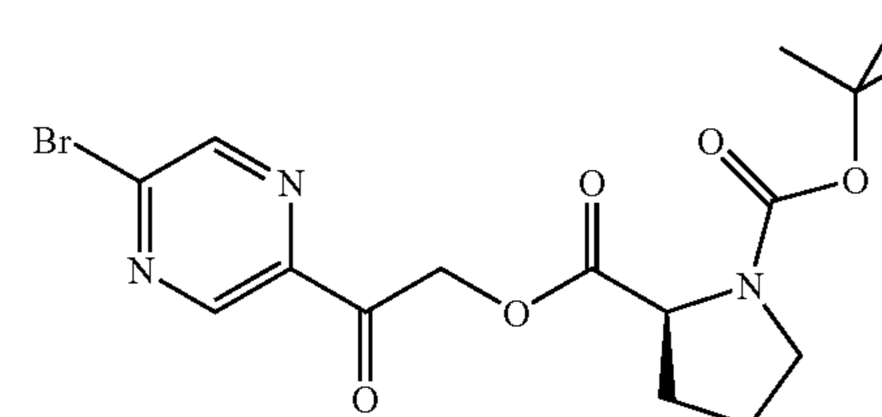
Example 152c-4
