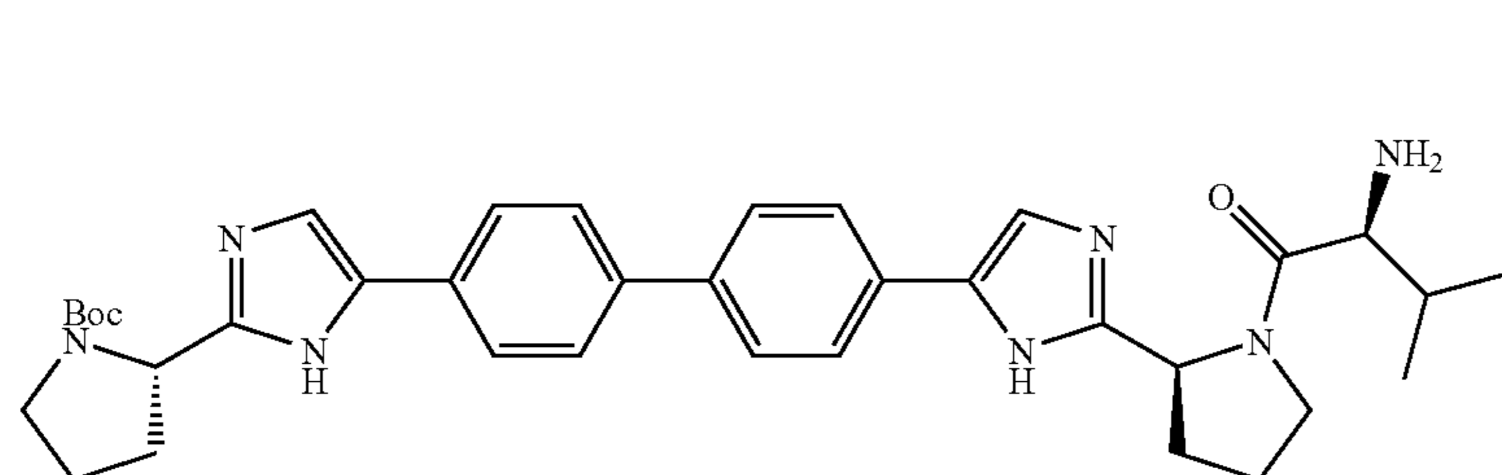
cj-2
