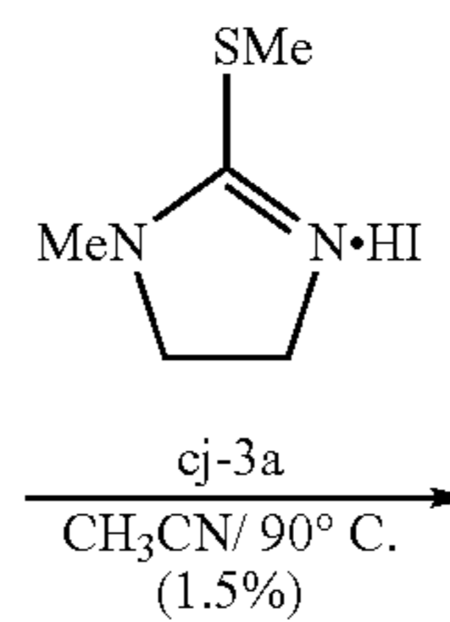
cj-6
