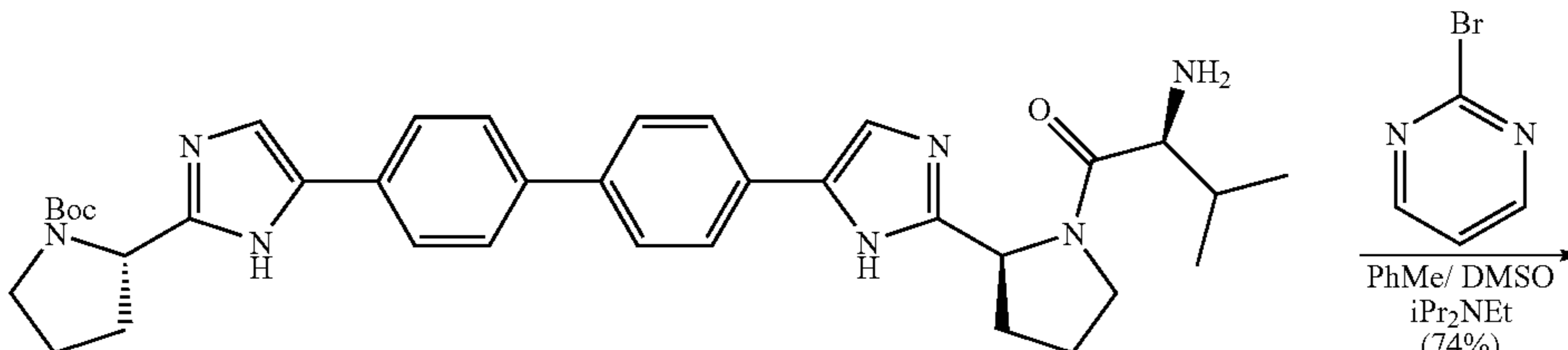
cj-2
