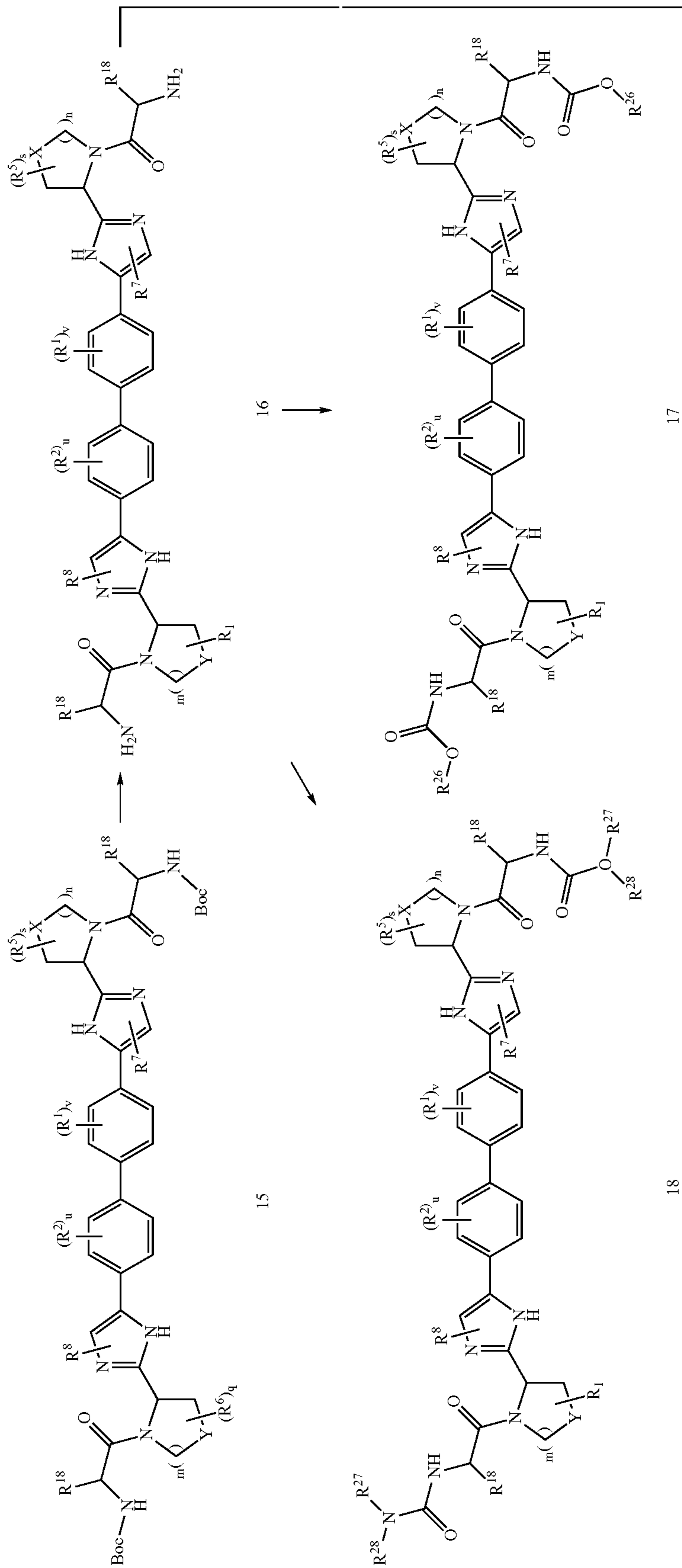
Scheme 4: Symmetric Biphenyls
