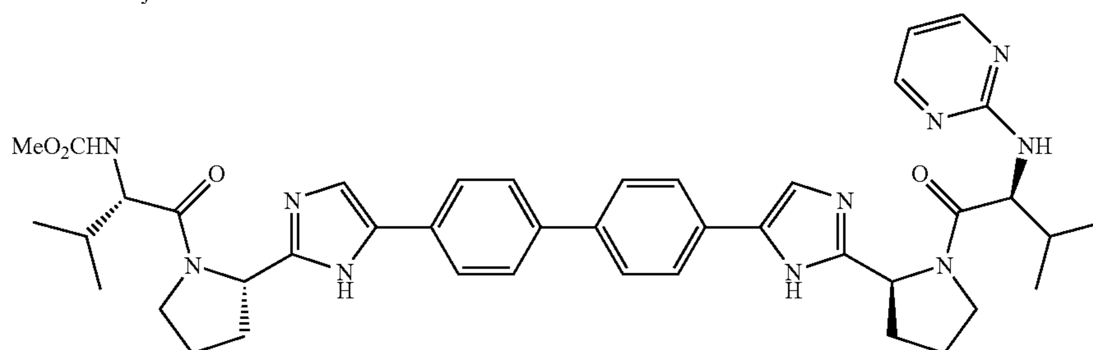
cj-10a
