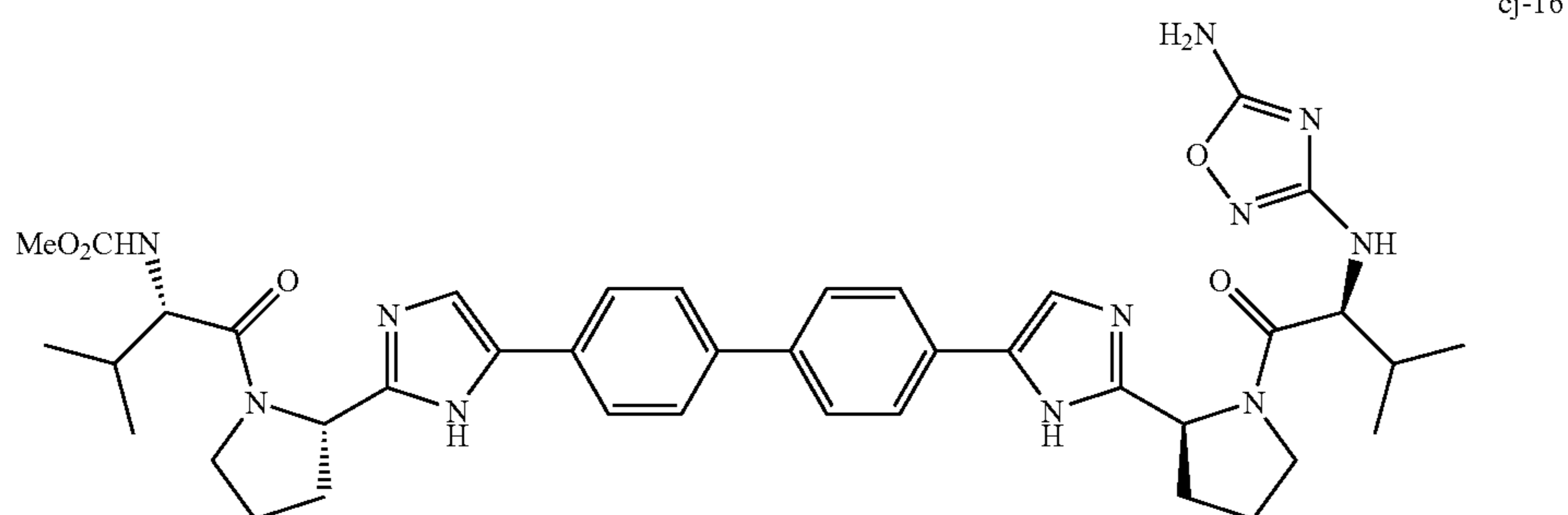
cj-16
