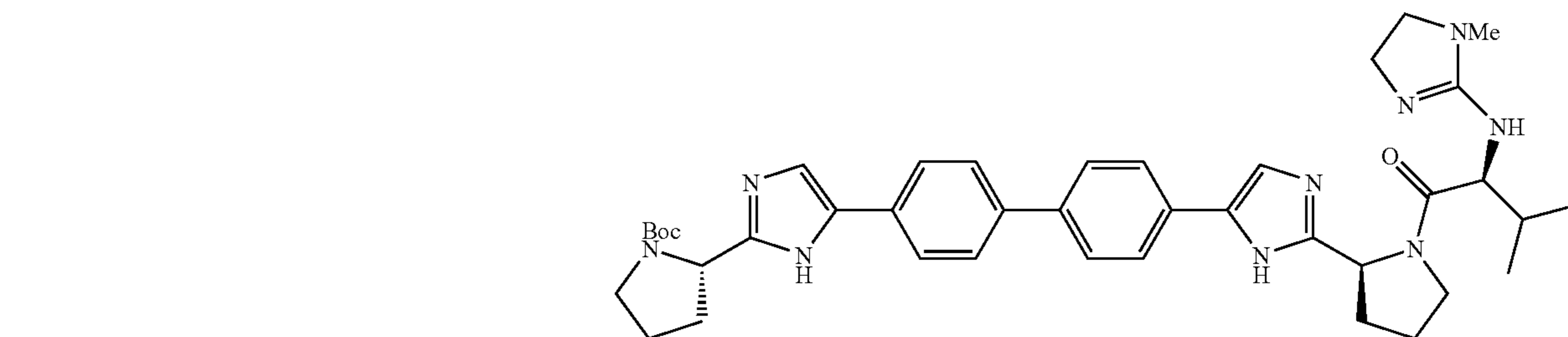
cj-6
