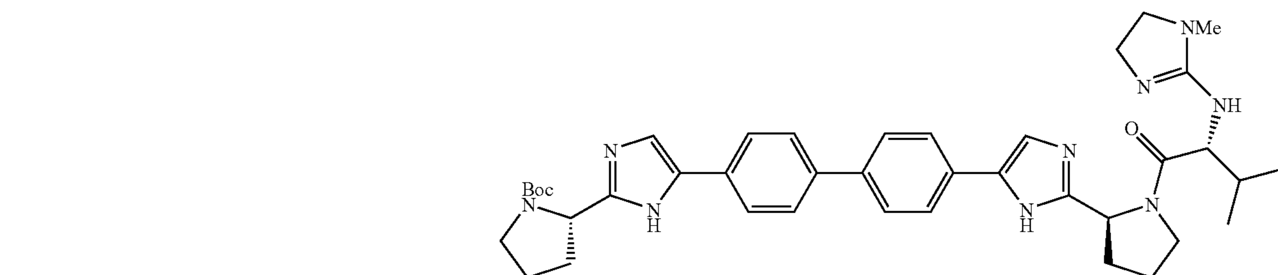
cj-7
