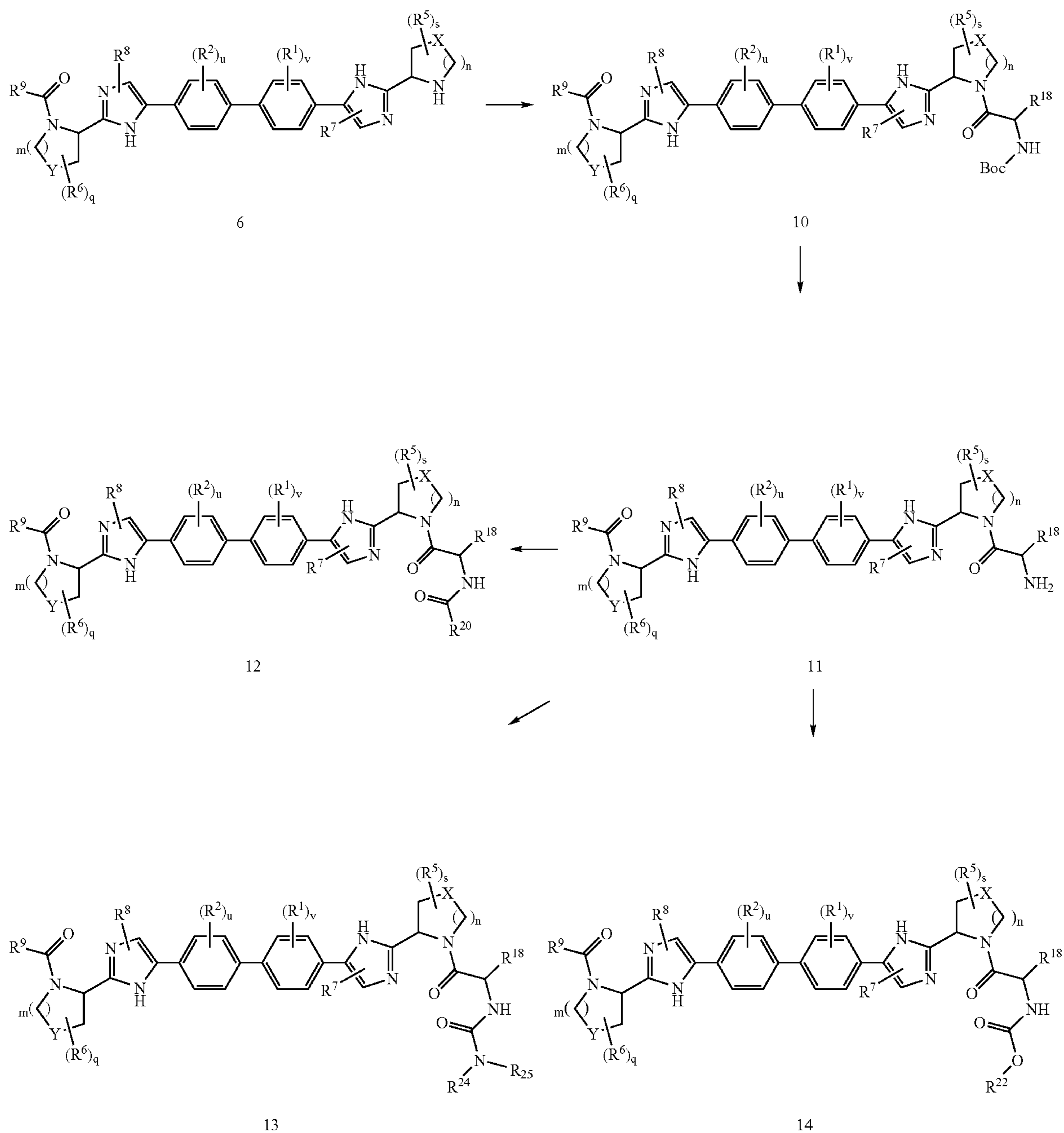
Scheme 3: Symmetric Cap Elaborated Biphenyls
