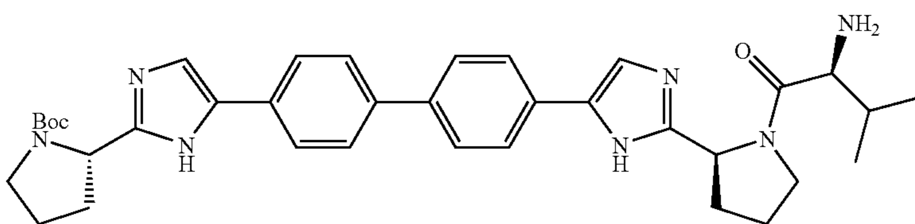
cj-2
