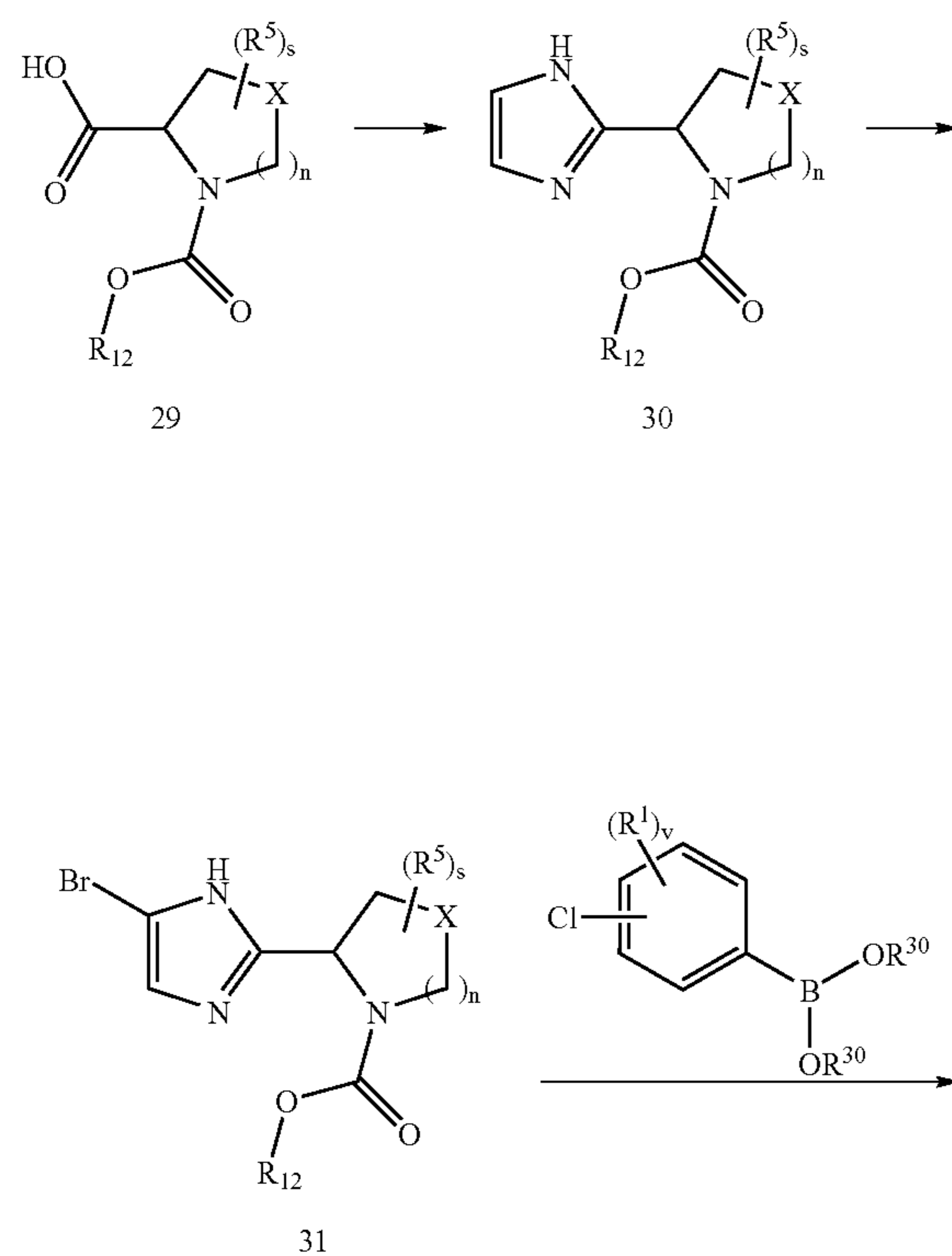
Scheme 7: Heteroaryls
