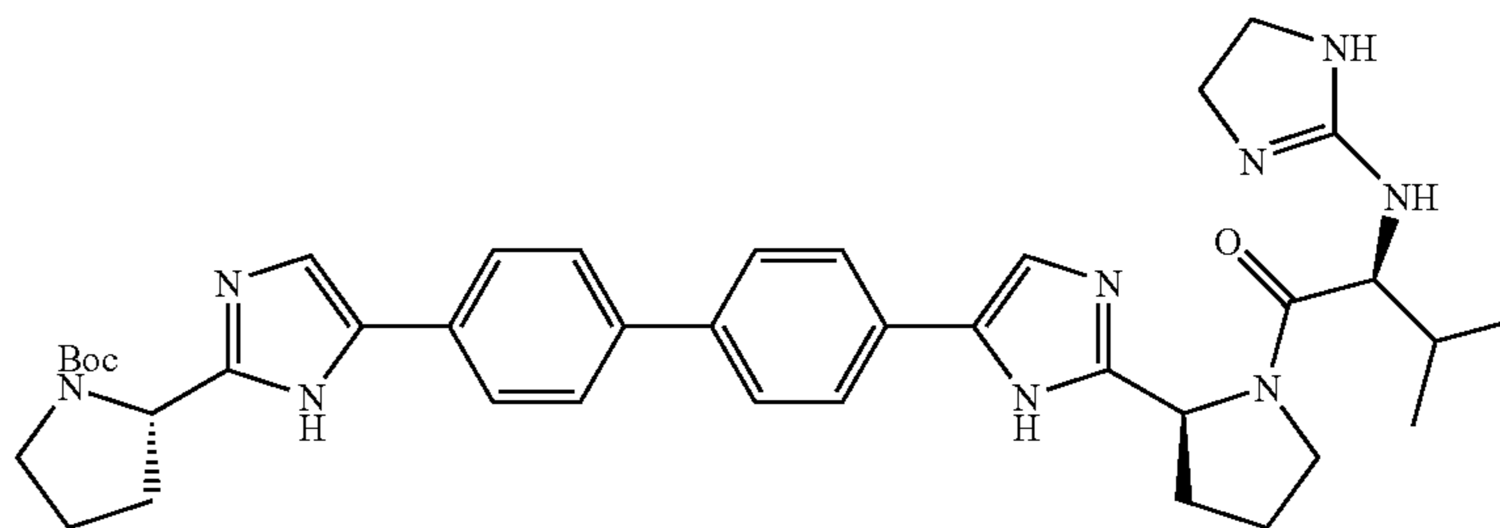
cj-8
