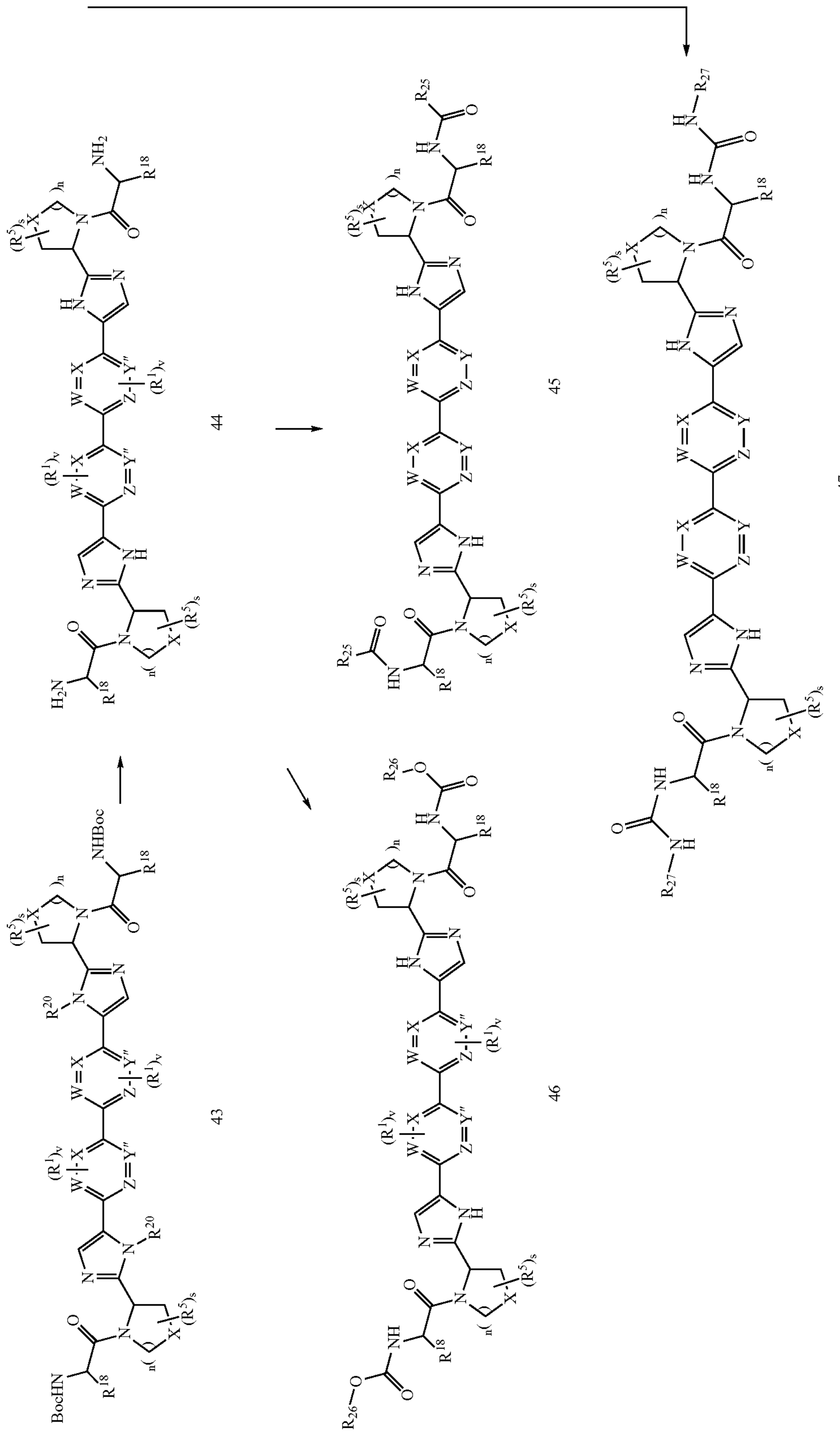
Scheme 10: Starting Material 29
