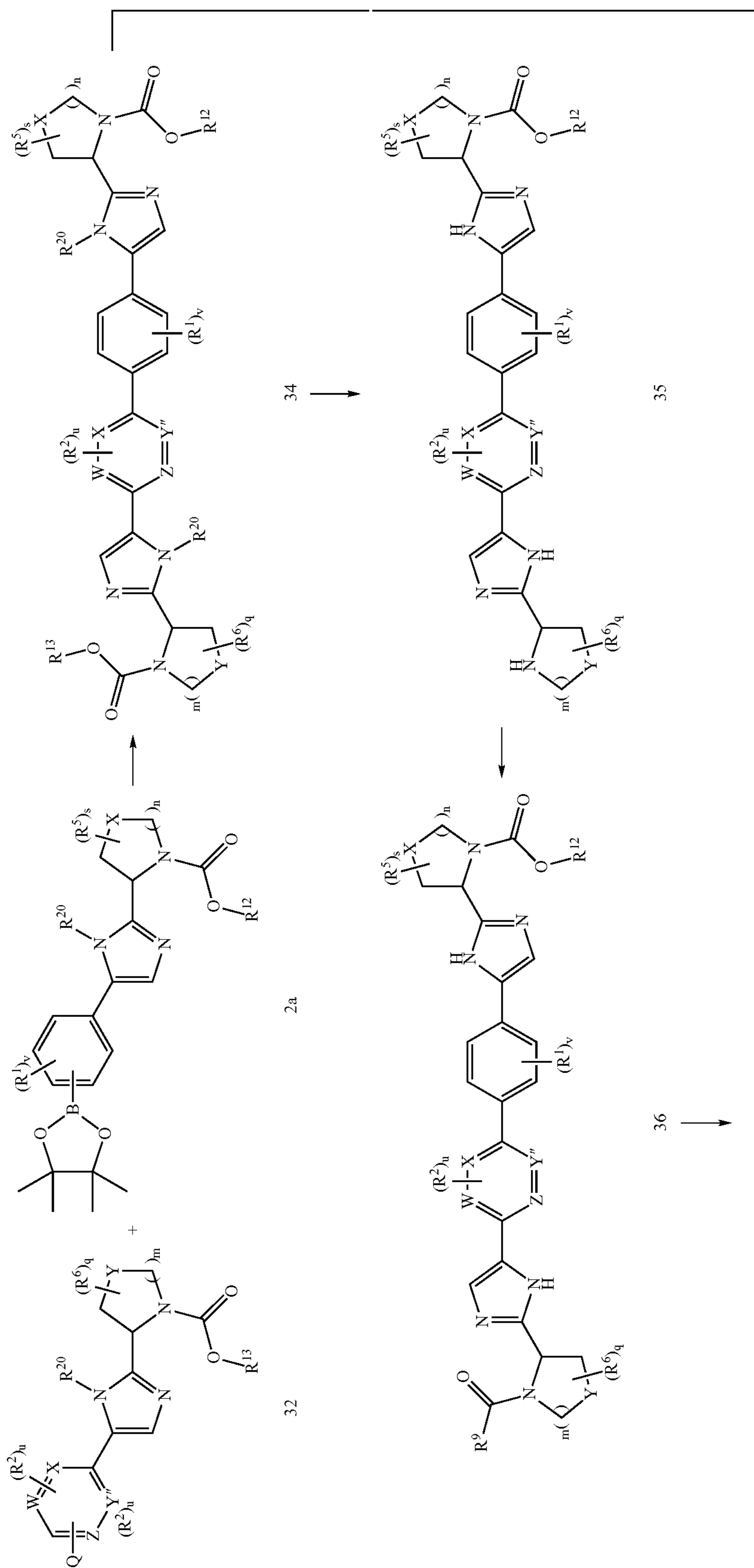
Scheme 8
