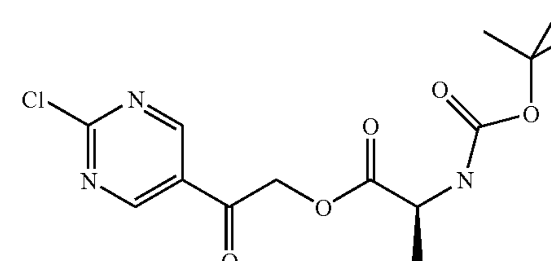
Example 152c-5
