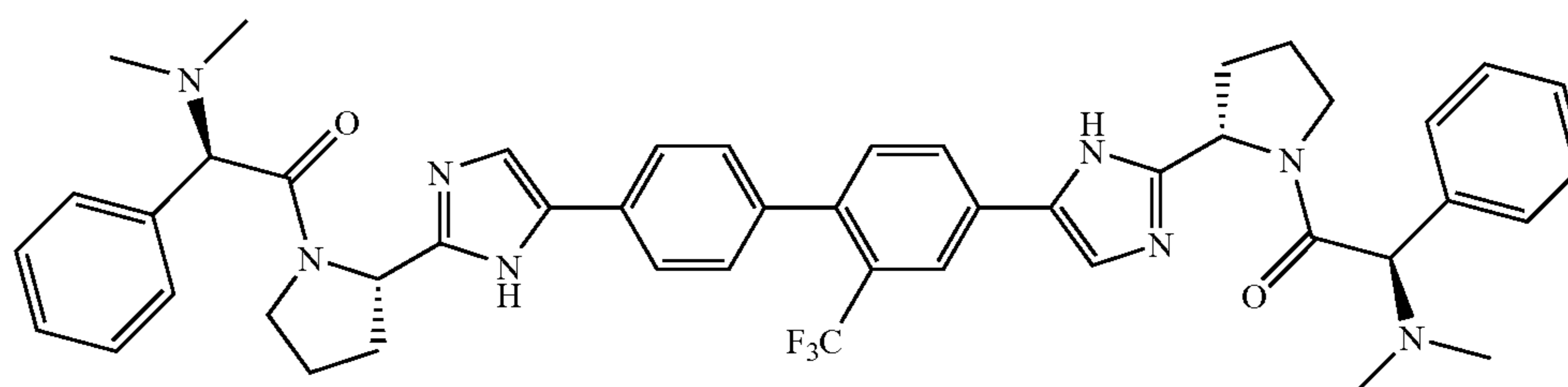
Example 130
