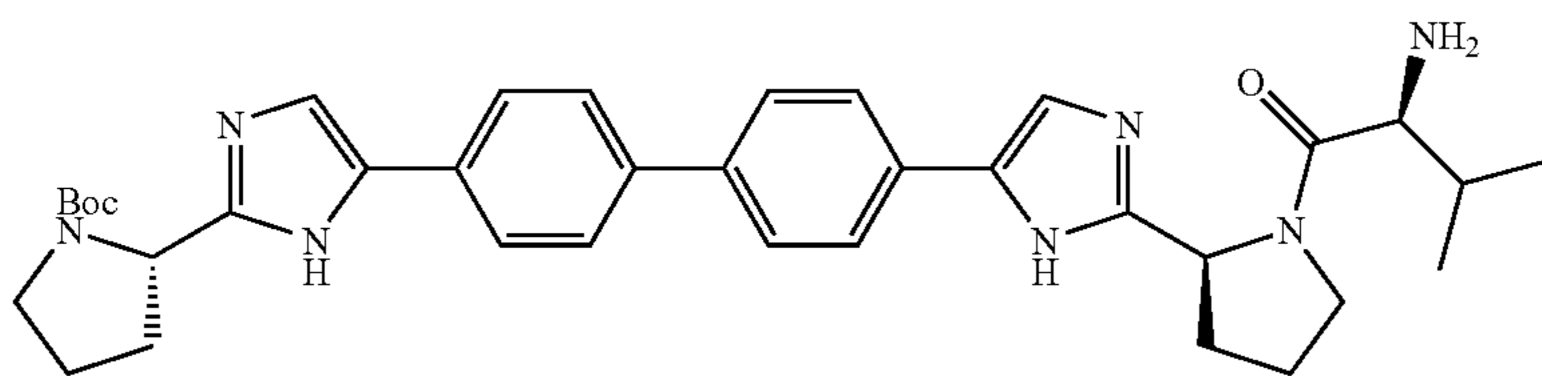
cj-2
