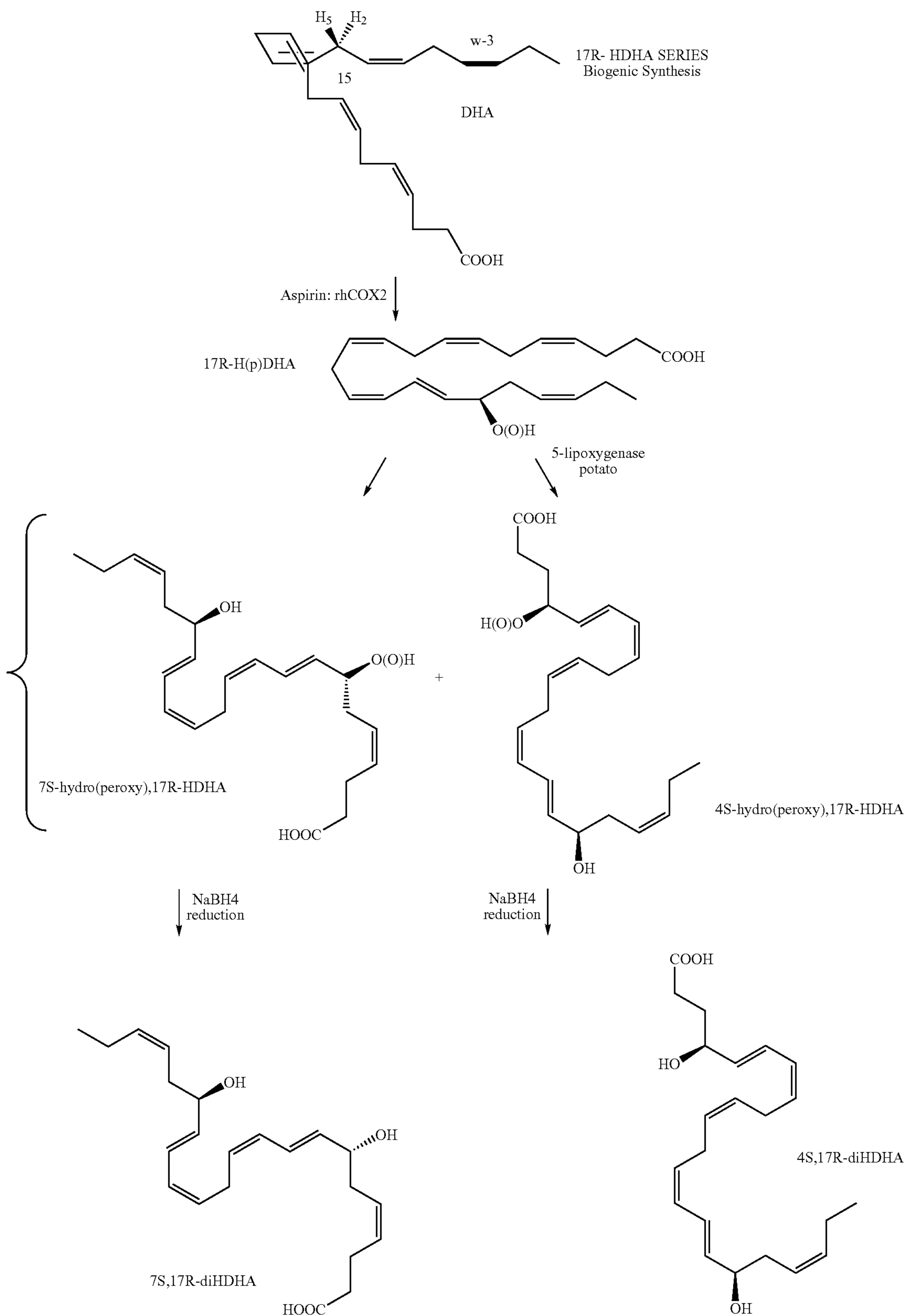
Scheme A
