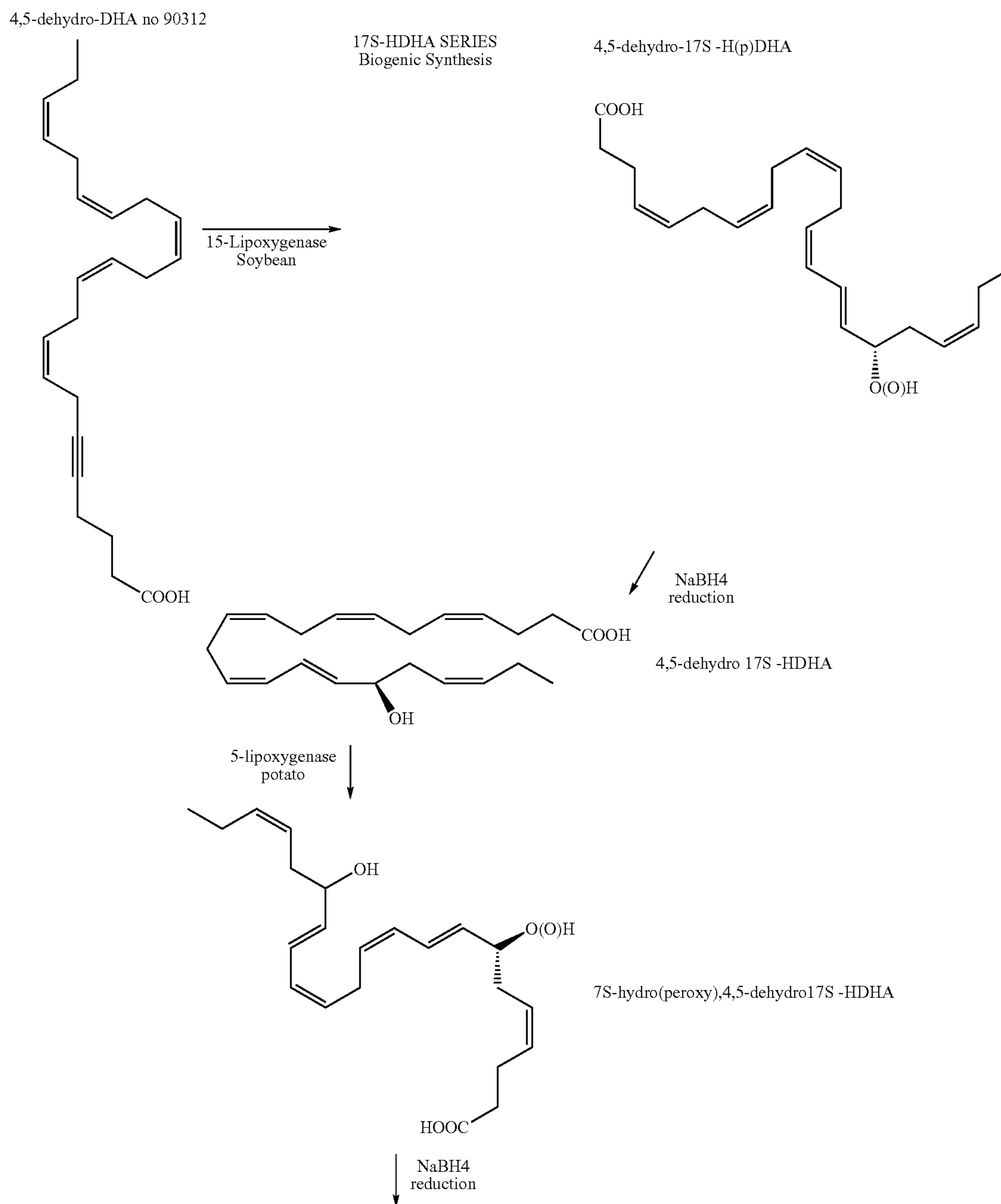
Scheme B
