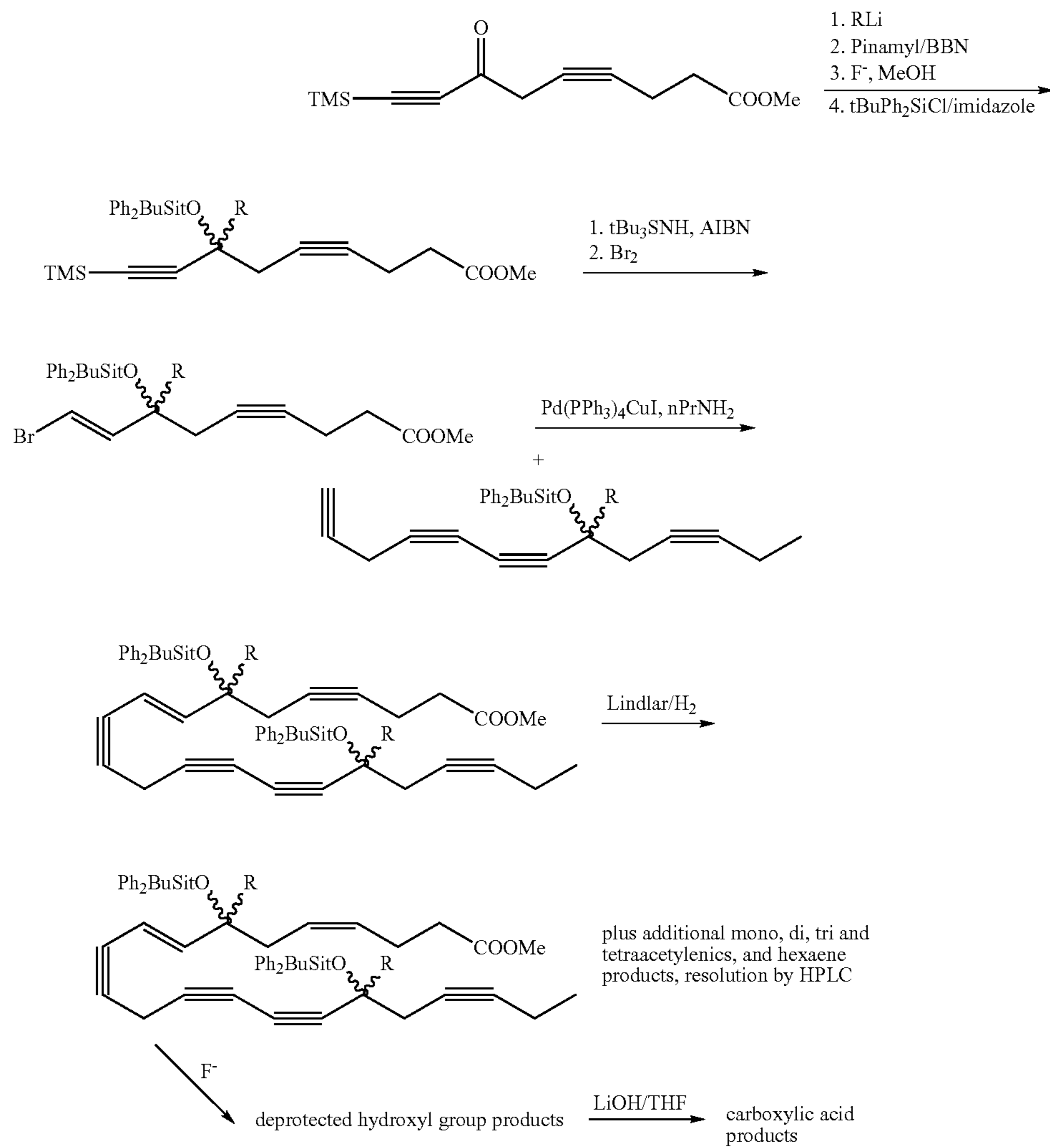
Scheme V
