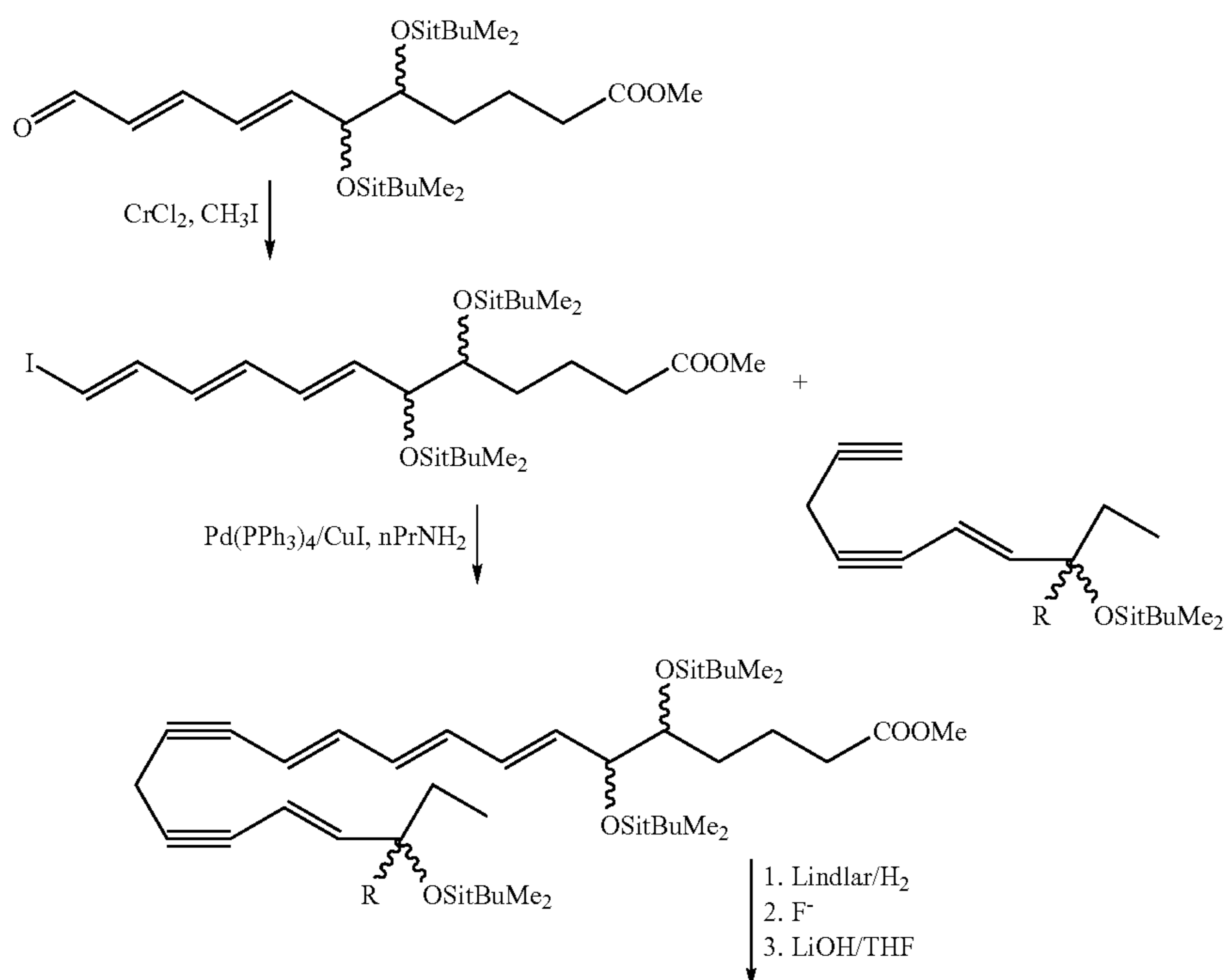
Scheme VIII
