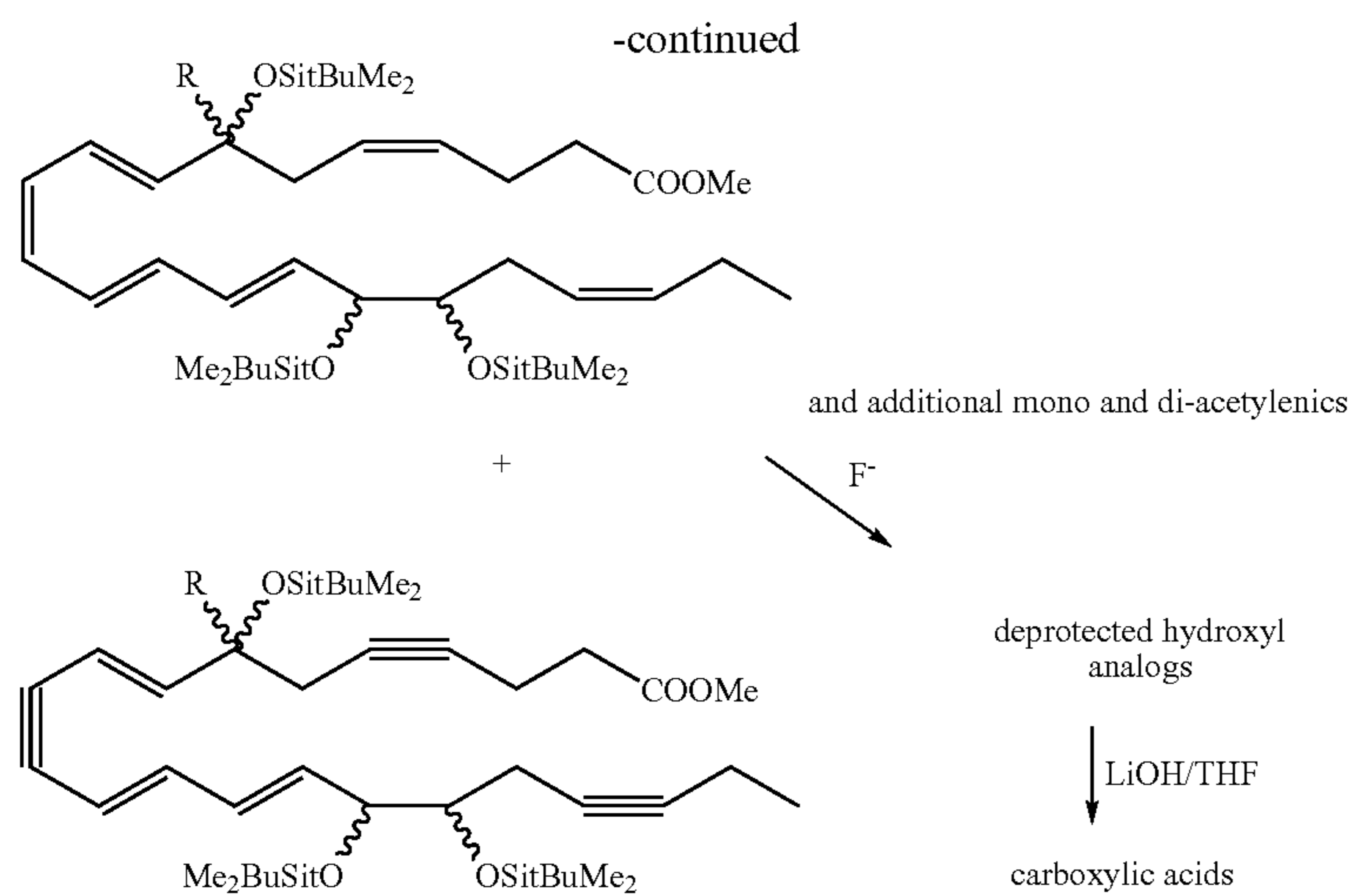
Scheme II
