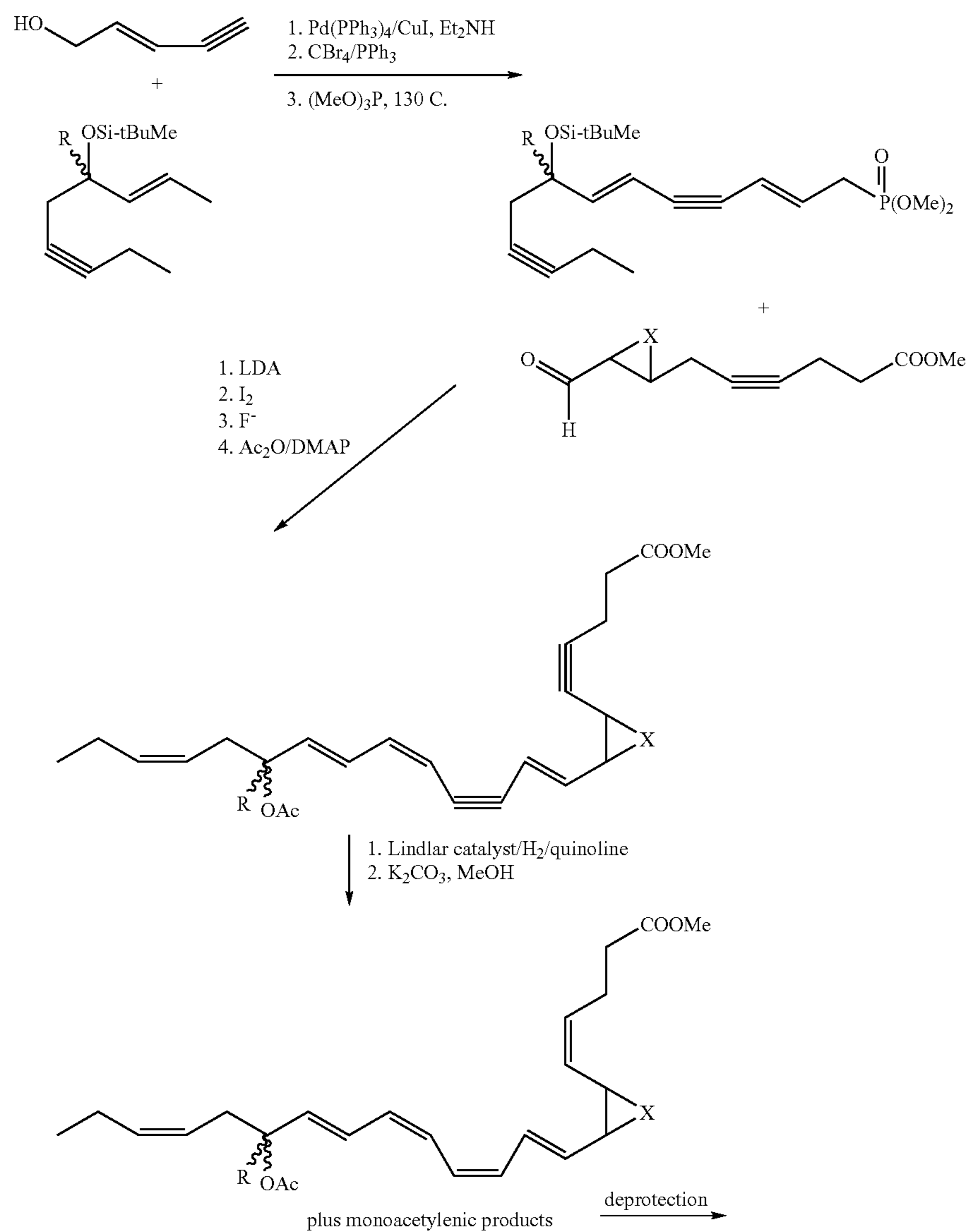
Scheme II
