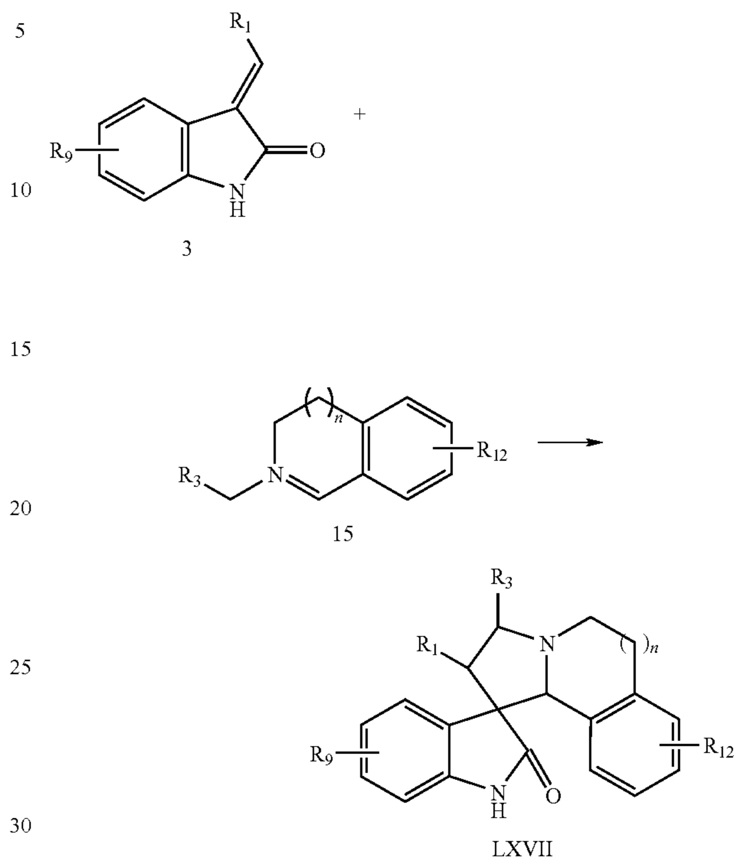
Scheme 4.
