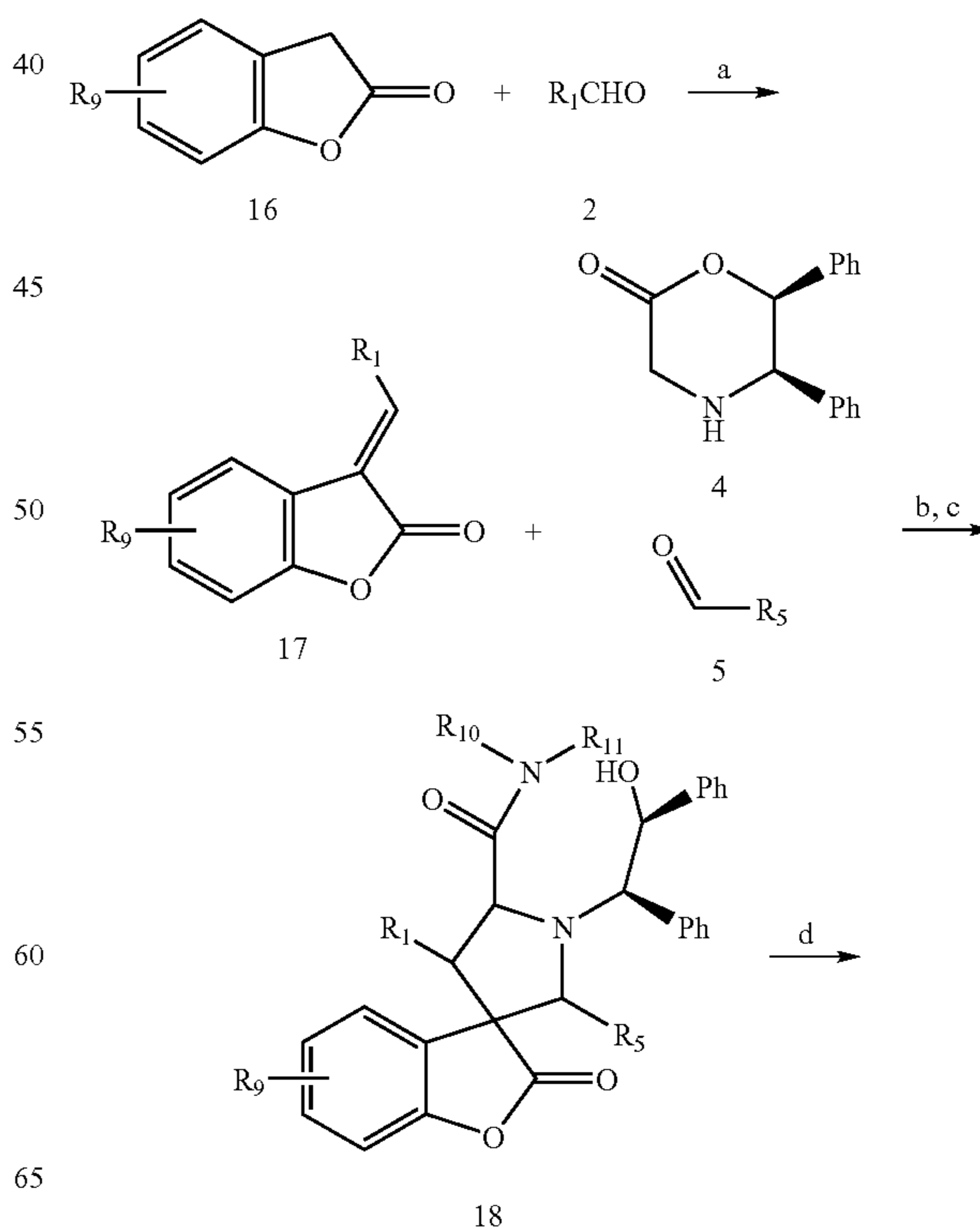
Scheme 5.
